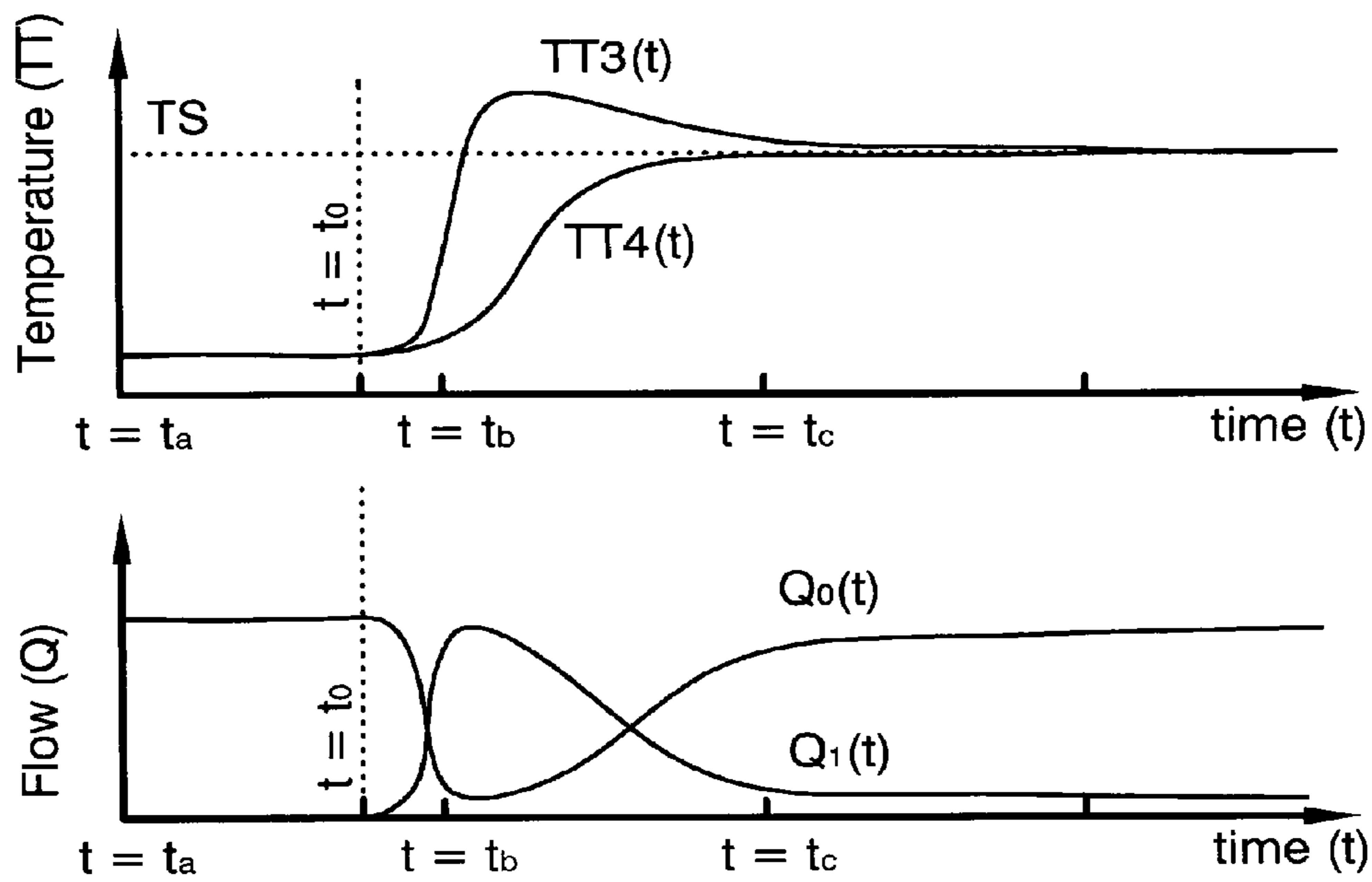
FIG. 2D
