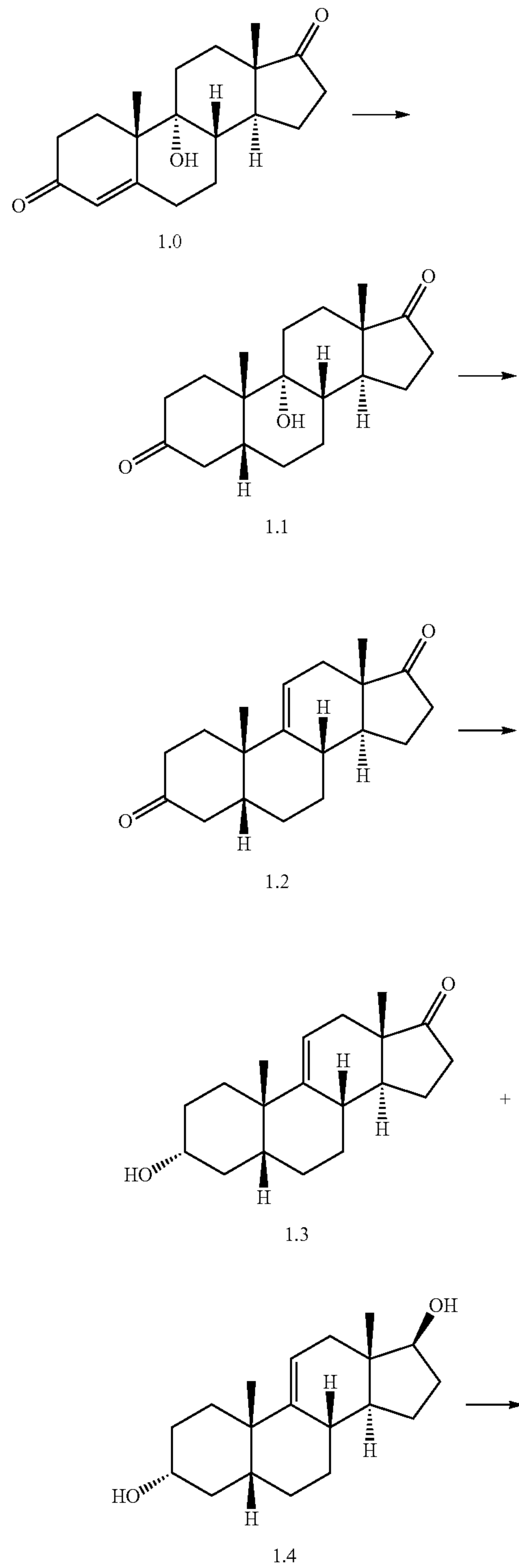
Scheme 1. Synthesis of Deoxycholic Acid (DCA)
