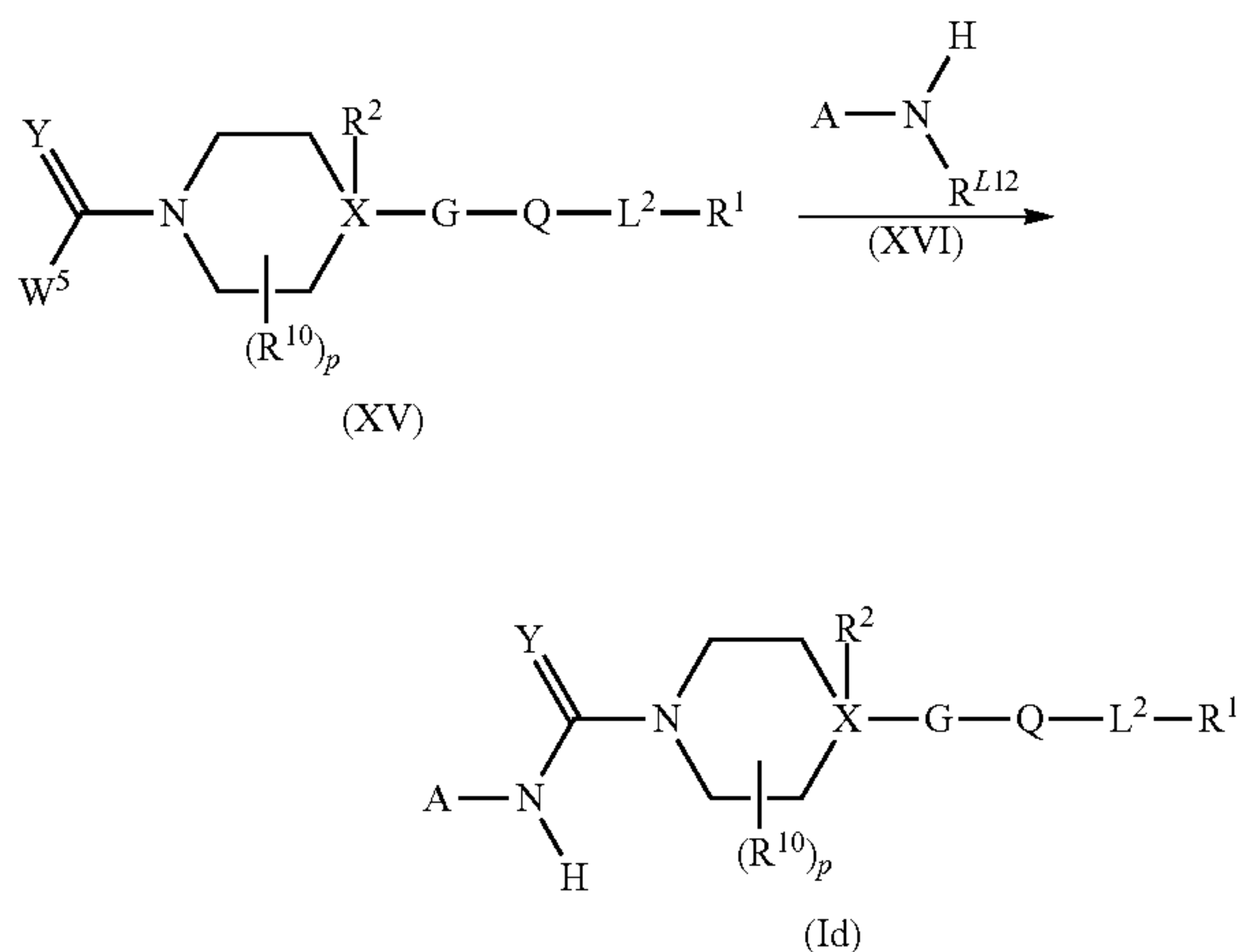
Scheme 11: Process J
