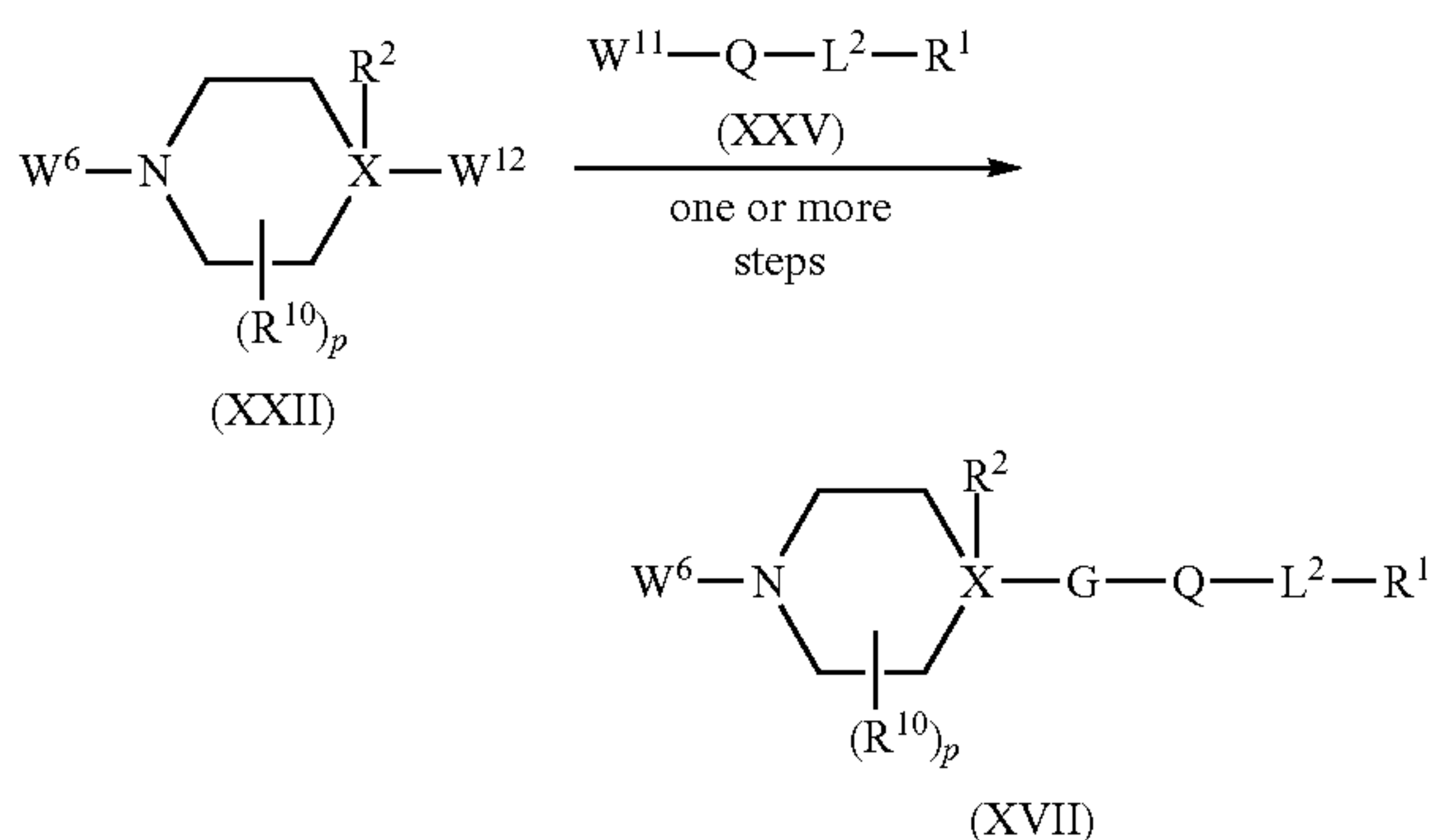
Scheme 13: Process L
