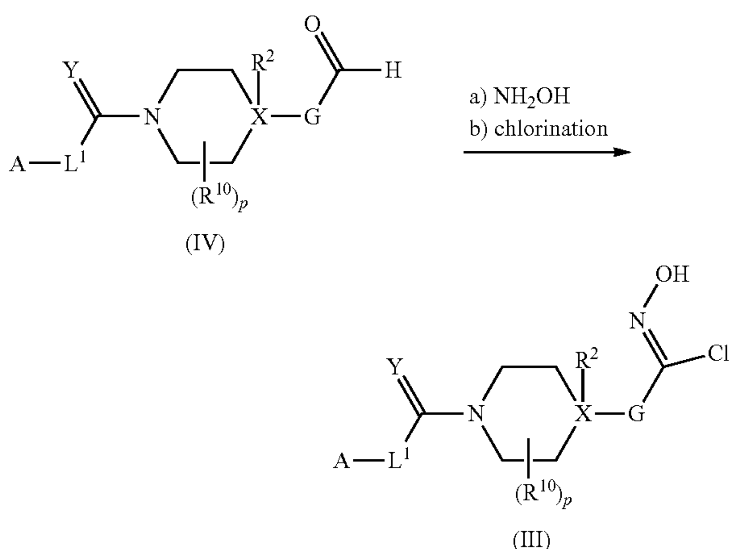
Scheme 3: Process C
