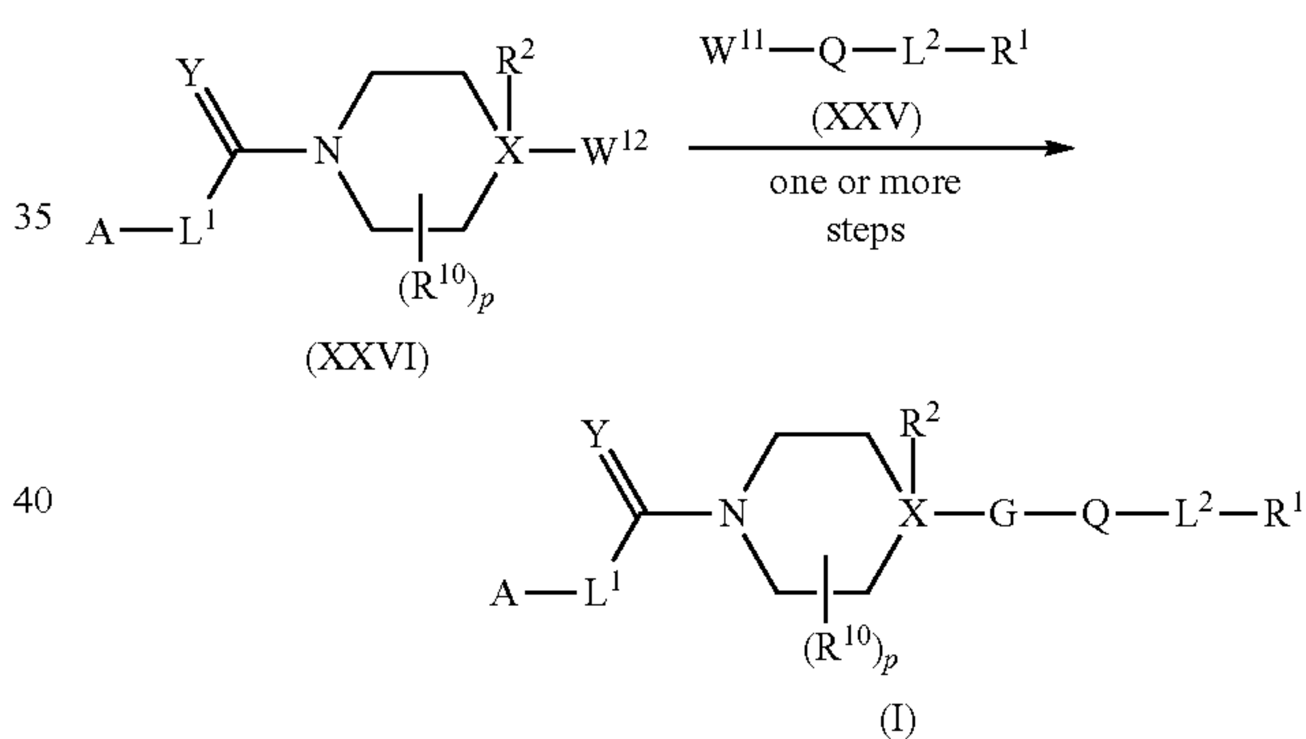
Scheme 4: Process D
