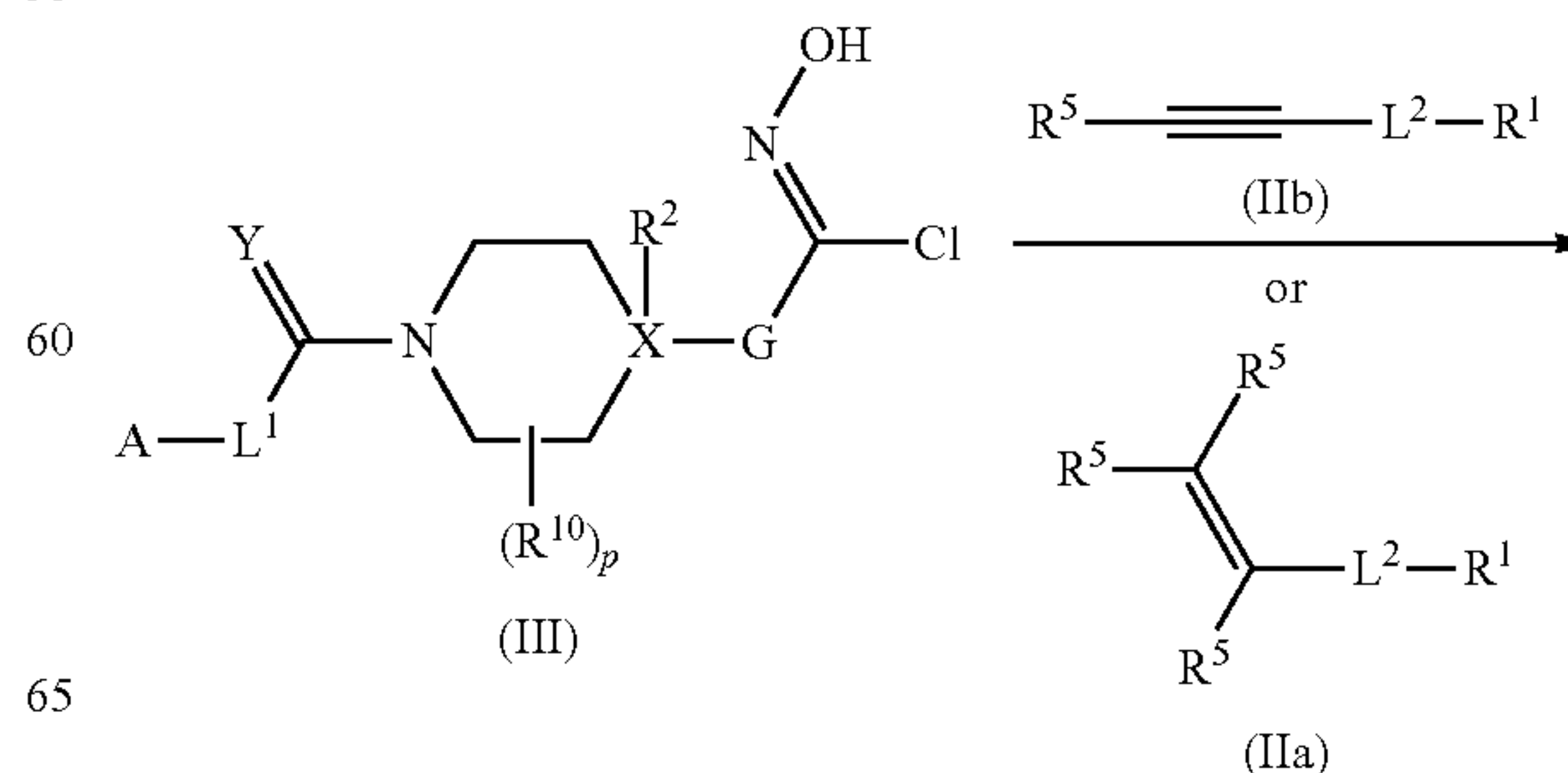
Scheme 2: Process B
