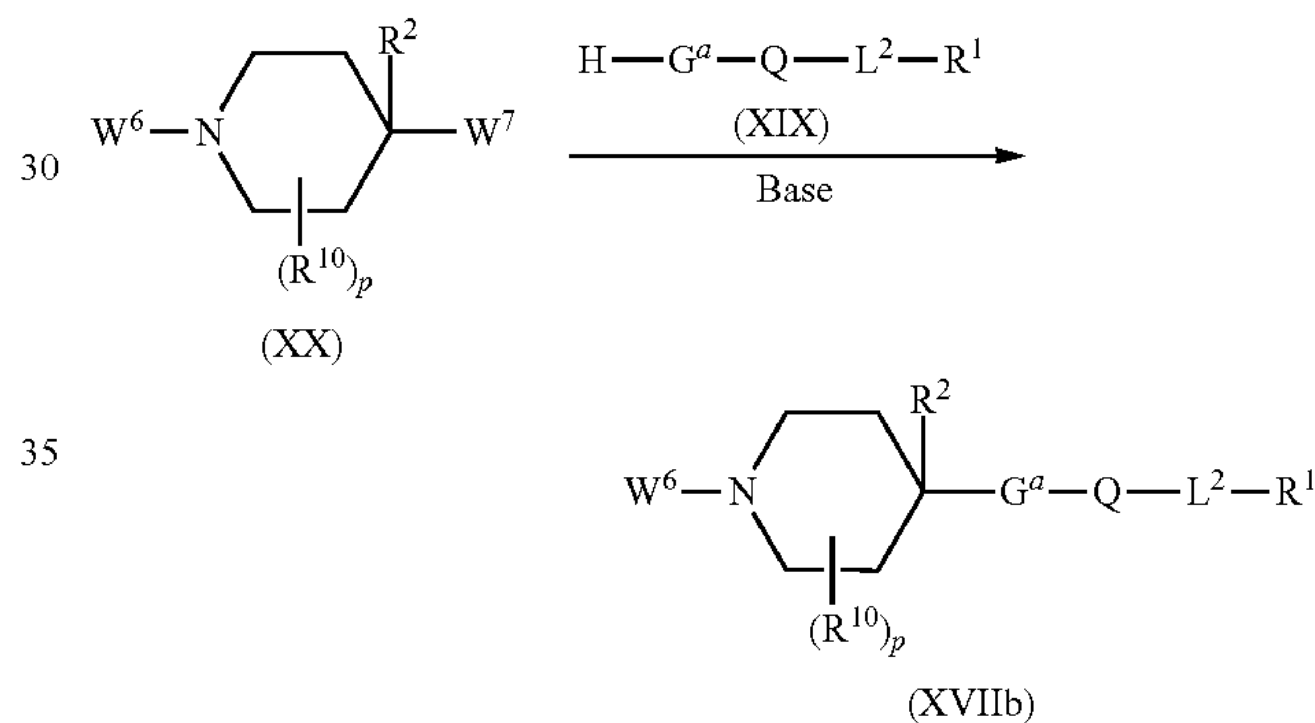
Scheme 15: Process N
