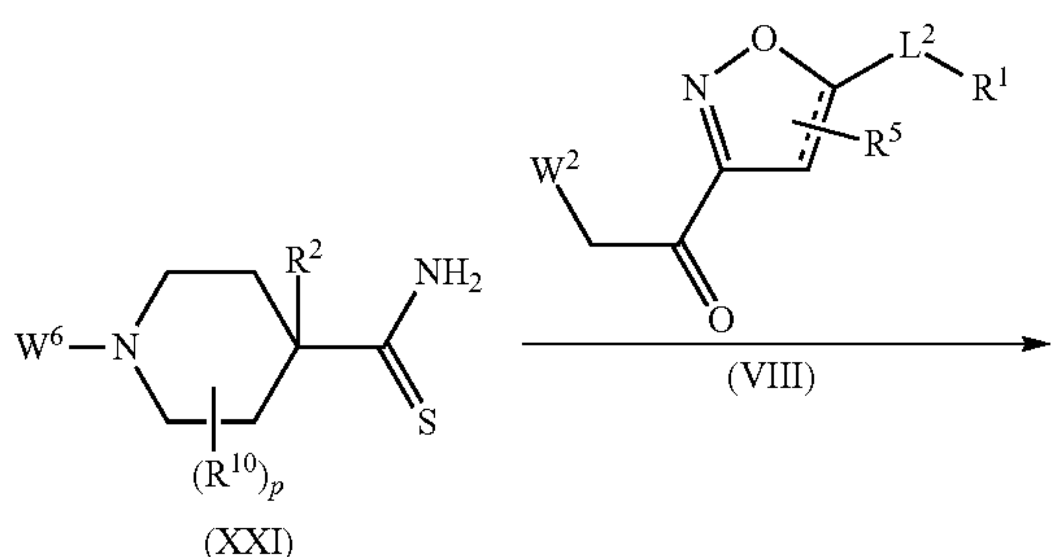
Scheme 14: Process M
