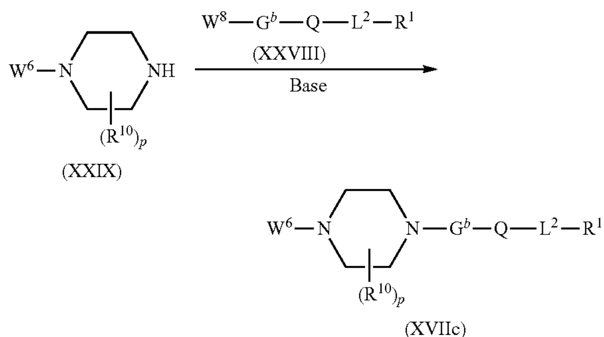
Scheme 16: Process O
