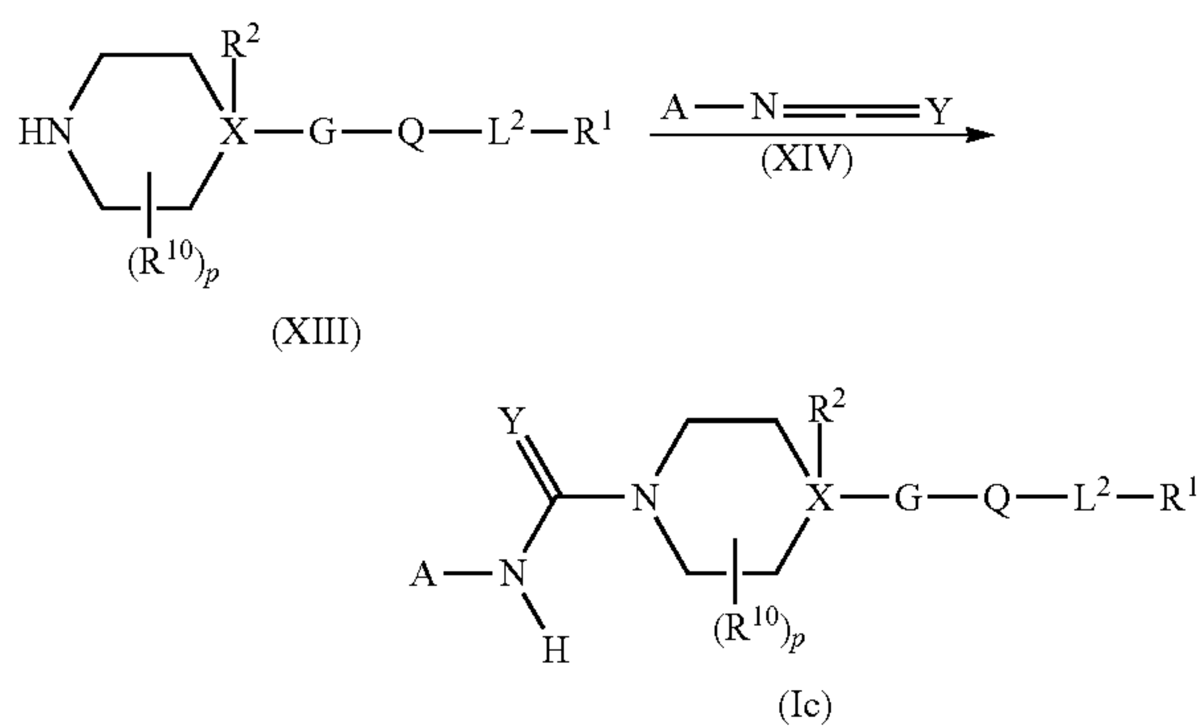
Scheme 10: Process I
