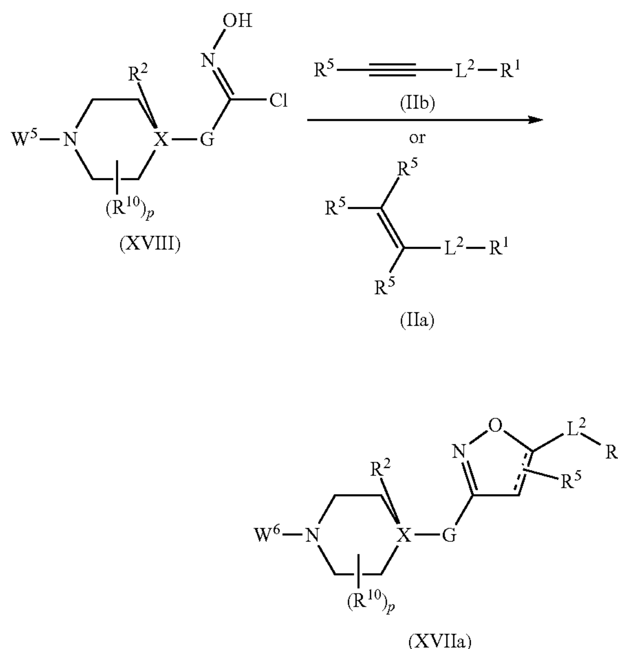
Scheme 18: Process Q
