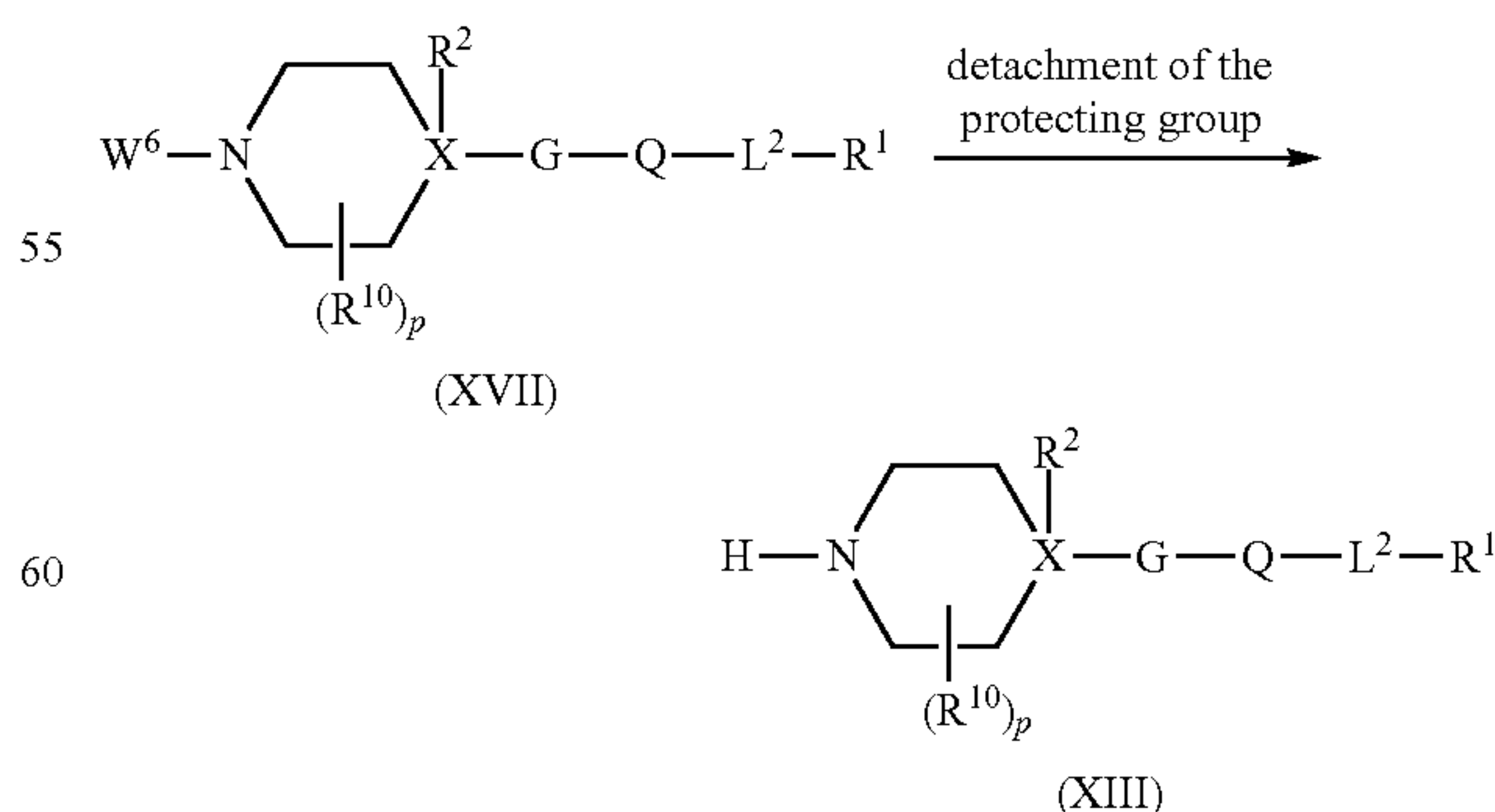
Scheme 12: Process K
