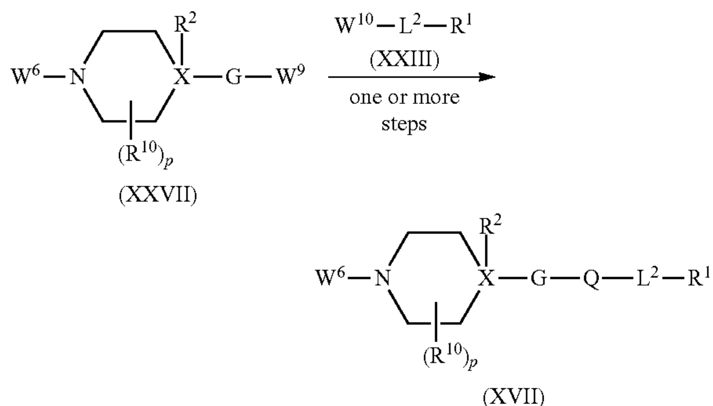
Scheme 17: Process P
