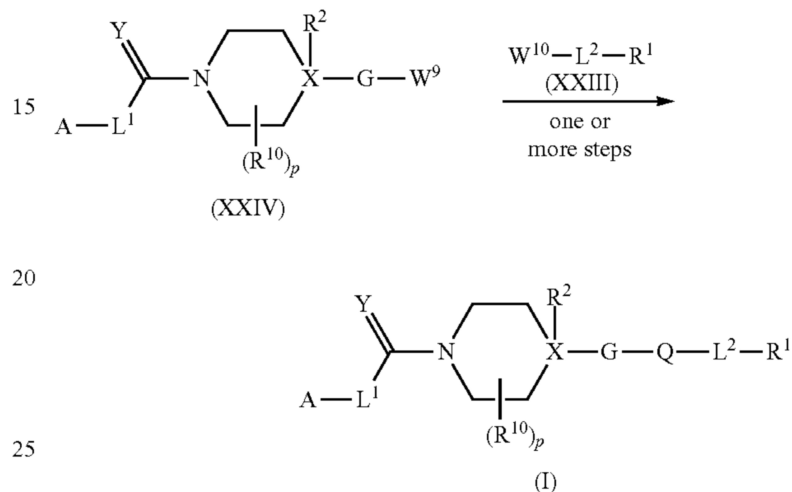
Scheme 1: Process A
