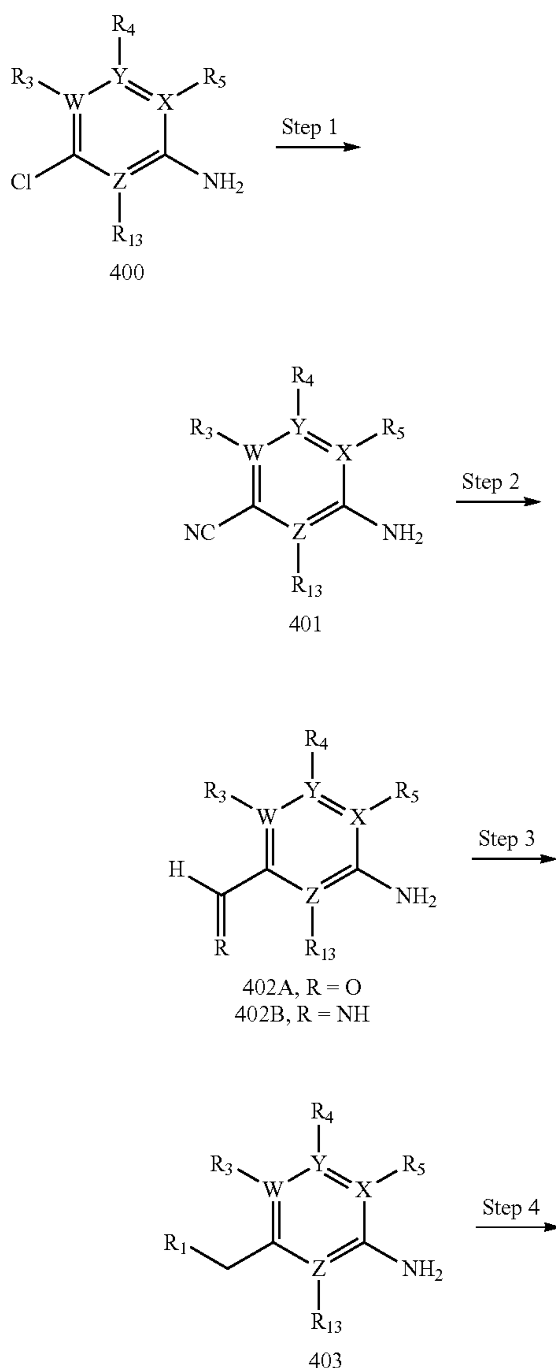
Reaction Scheme 4
