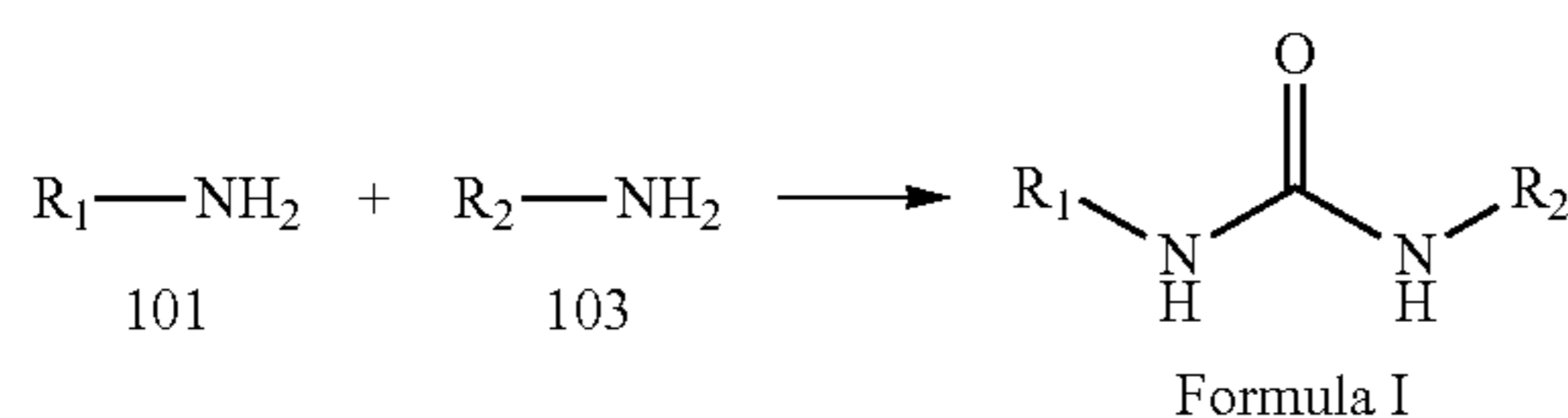
REACTION SCHEME 1
