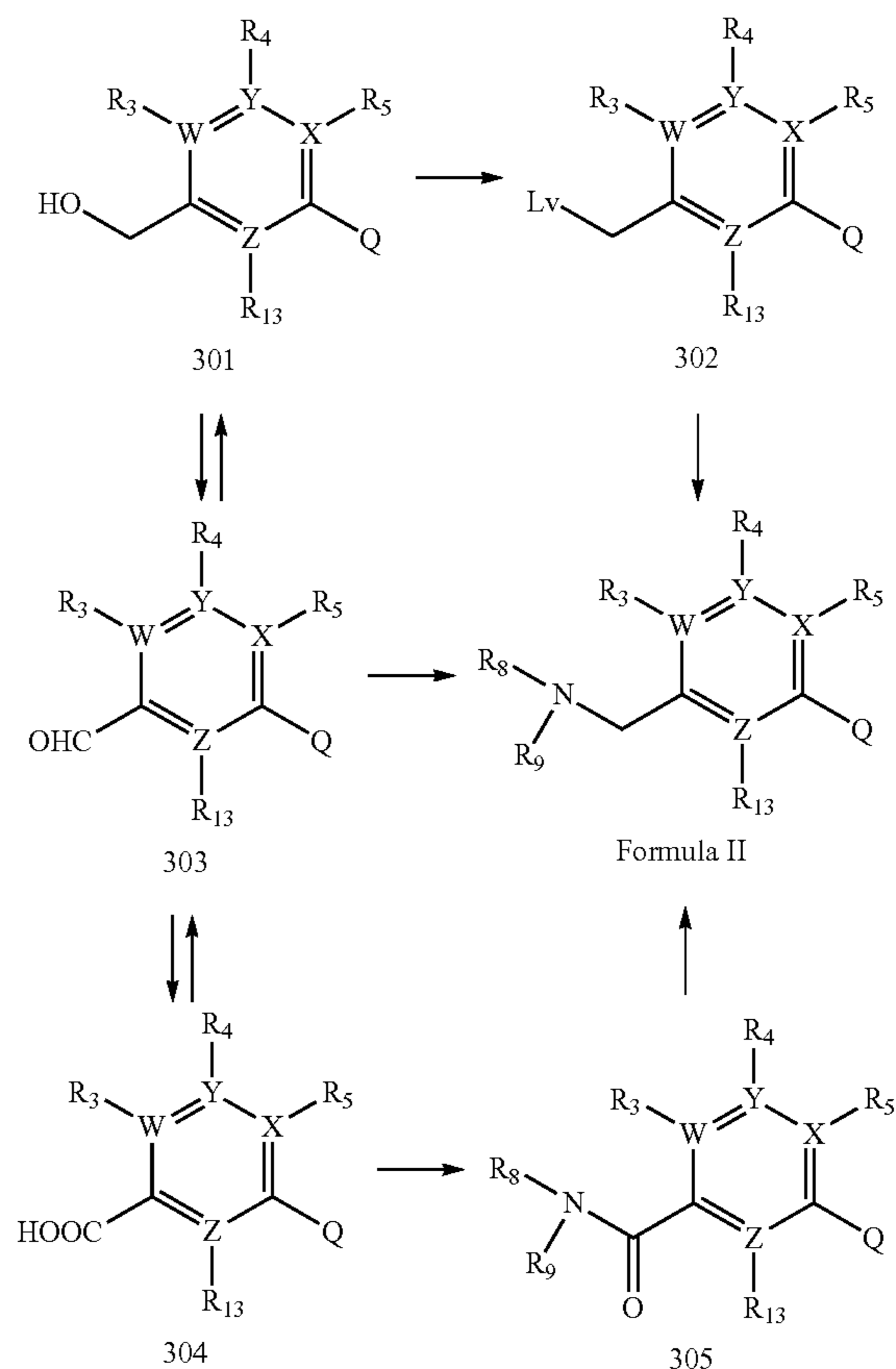
REACTION SCHEME 3
