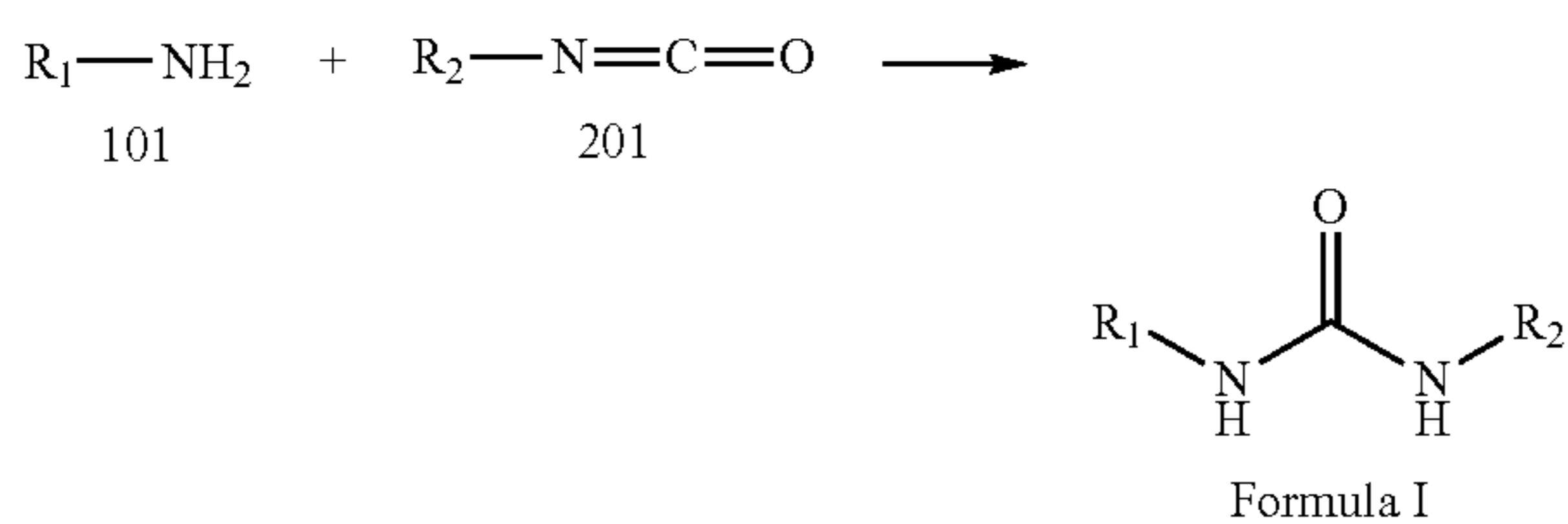
REACTION SCHEME 2
