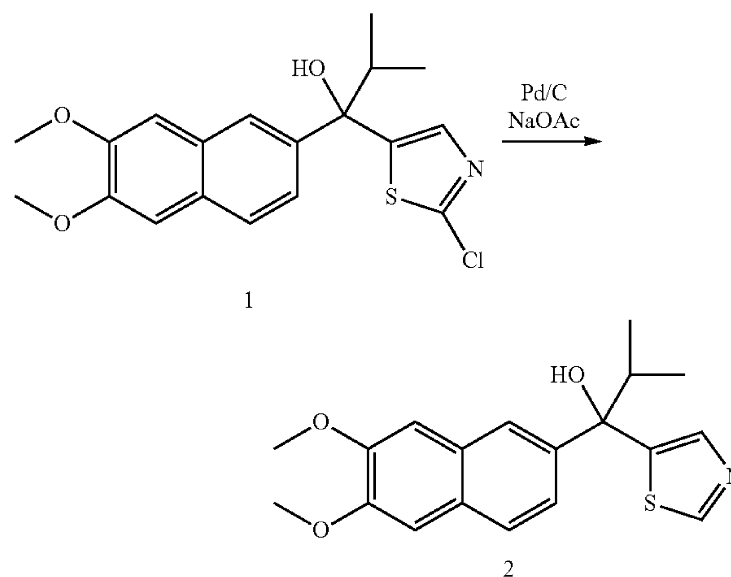
1-(6,7-dimethoxynaphthalen-2-yl)-2-methyl-1-(thiazol-5-yl)propan-1-ol (2)
