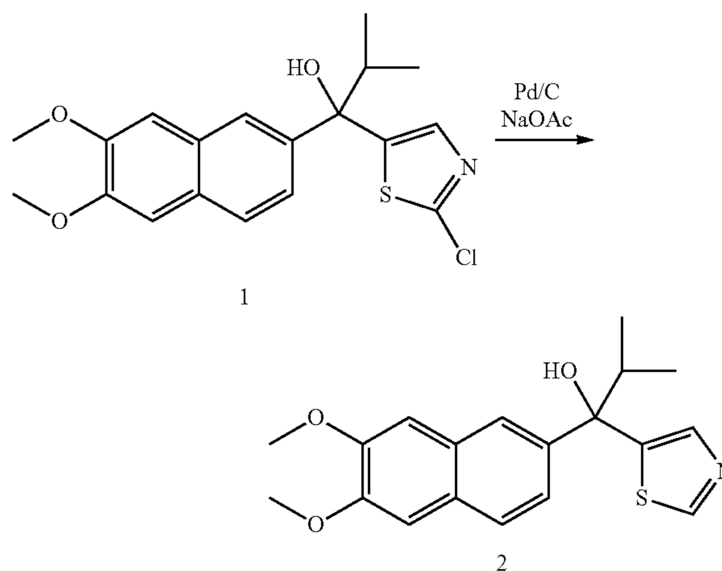
1-(6,7-dimethoxynaphthalen-2-yl)-2-methyl-1-(thiazol-5-yl)propan-1-ol (2)
