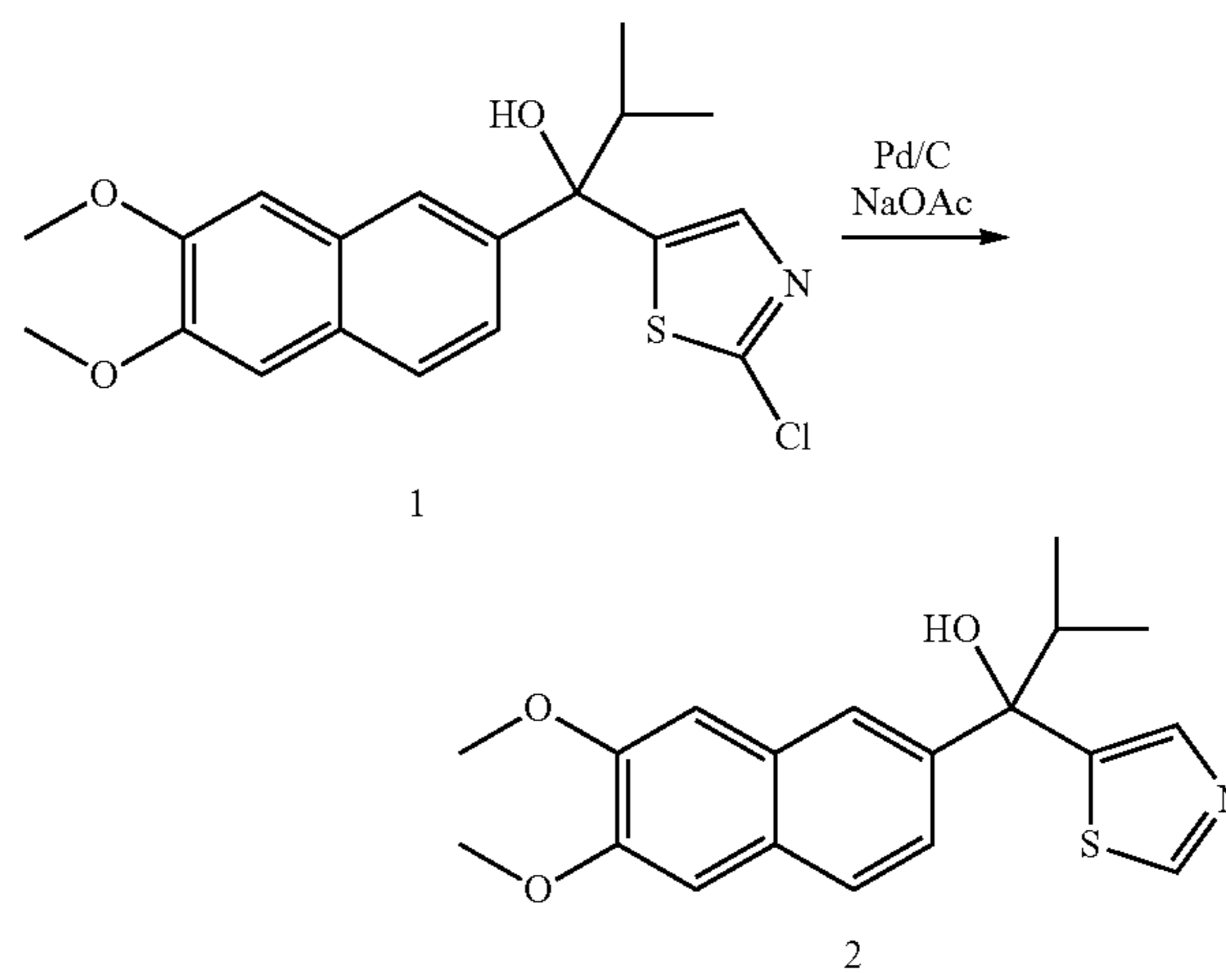
1-(6,7-dimethoxynaphthalen-2-yl)-2-methyl-1-(thiazol-5-yl)propan-1-ol (2)
