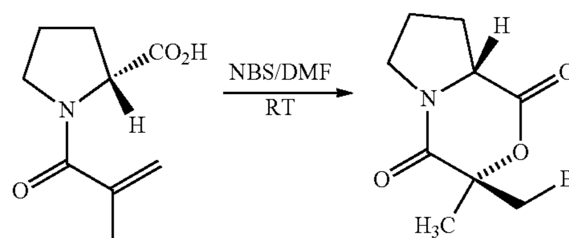
(3R,8aR)-3-Bromomethyl-3-methyl-tetrahydro-pyrrolo[2,1-c][1,4]oxazine-1,4-dione
