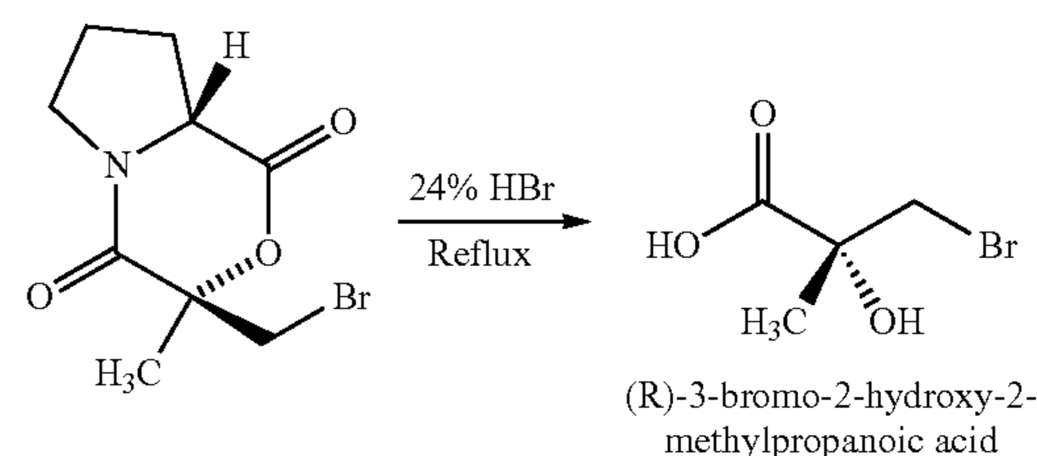
(2R)-3-Bromo-2-hydroxy-2-methylpropanoic Acid
