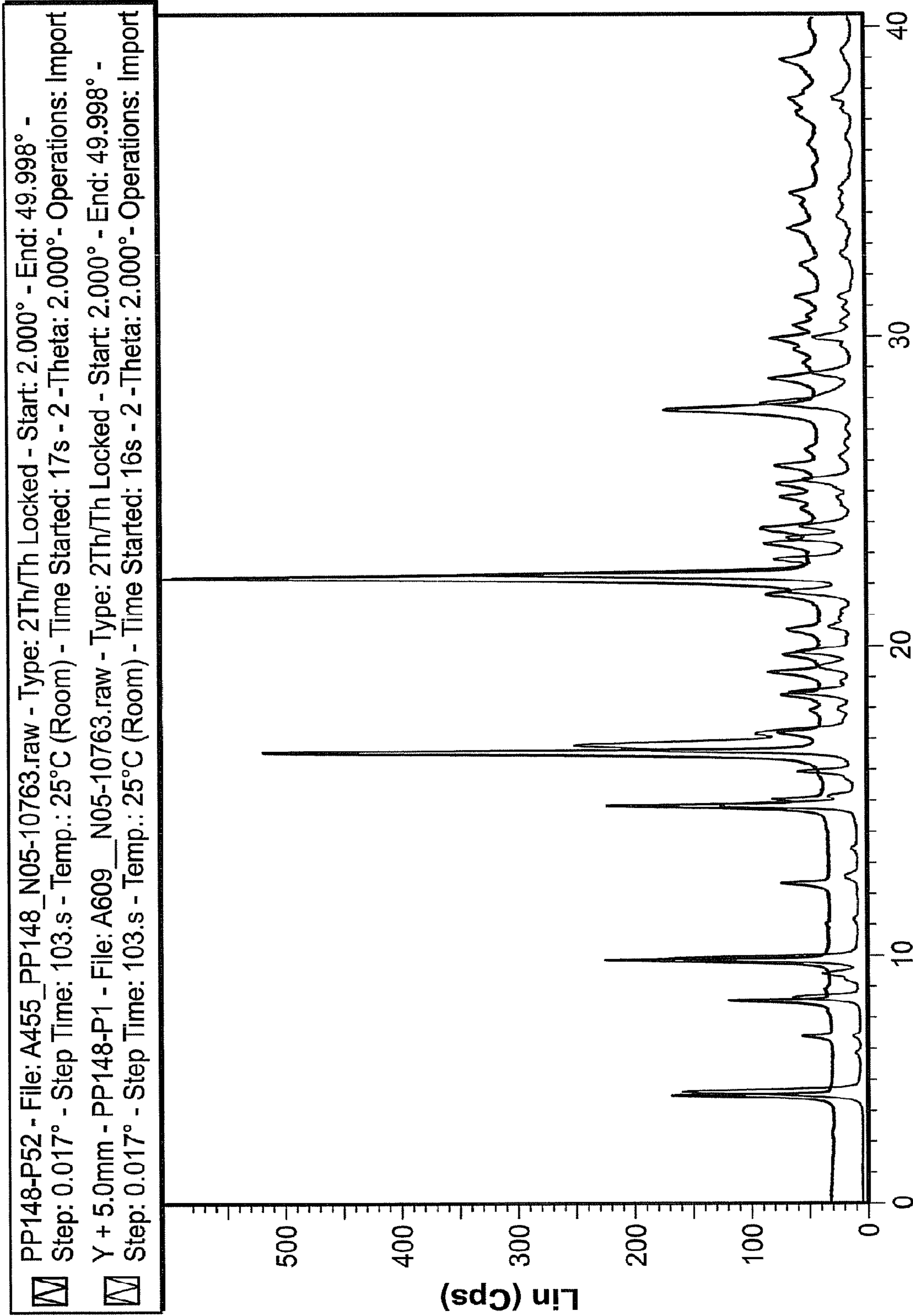
2-Theta - Scale, (Cu Kalpha Radiation) FIG. 12D
