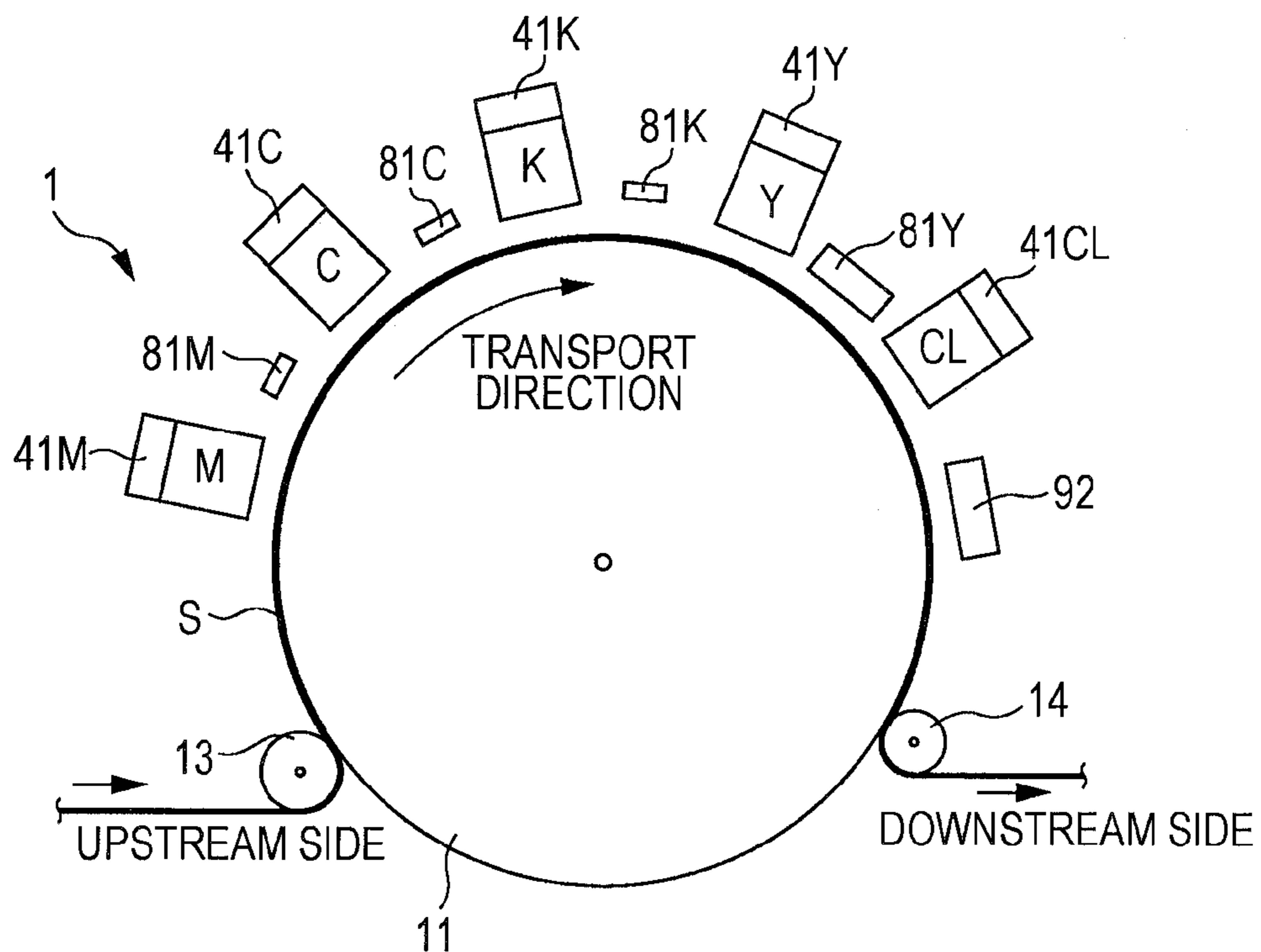
FIG. 10A FIFTH EMBODIMENT
