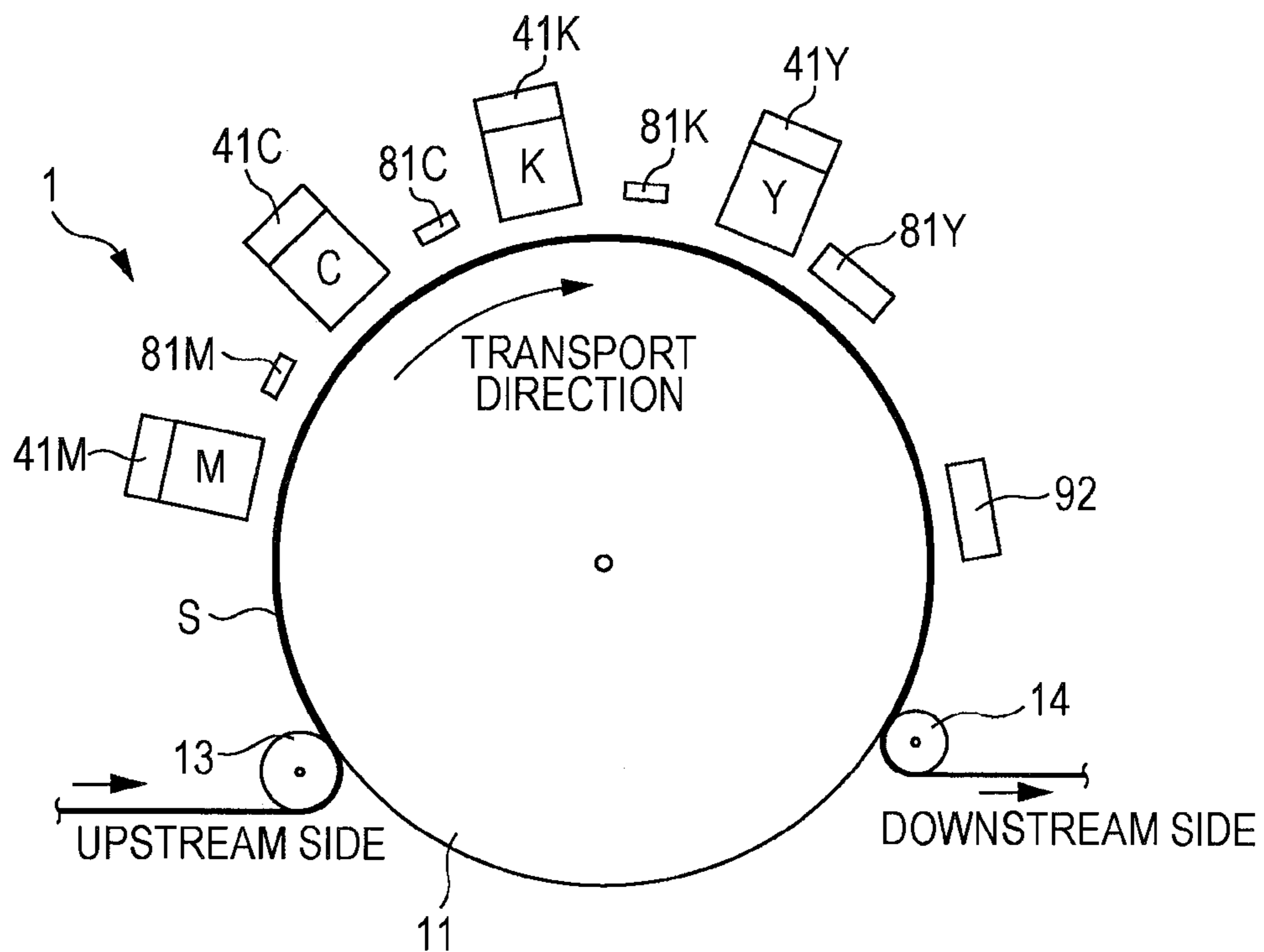
FIG. 10B FIFTH EMBODIMENT
