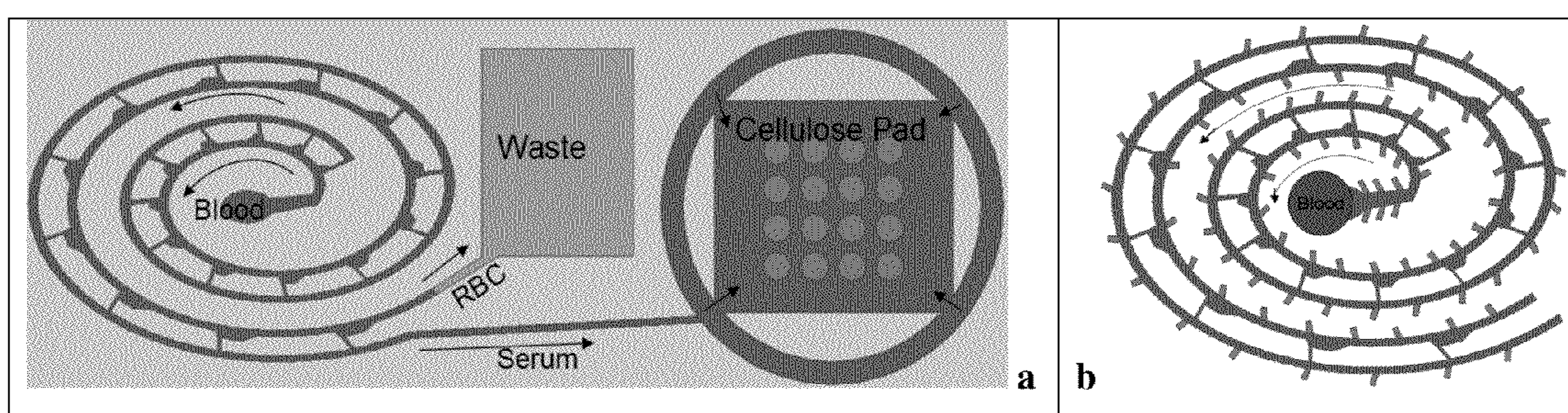
Fig. 15.a. The diagram shows the concept of the SMART chip for serum separation from whole blood and colorimetric assay. b. Serum separation spiral microfluidic channel is actuated by acoustic cavitations streaming pump.
