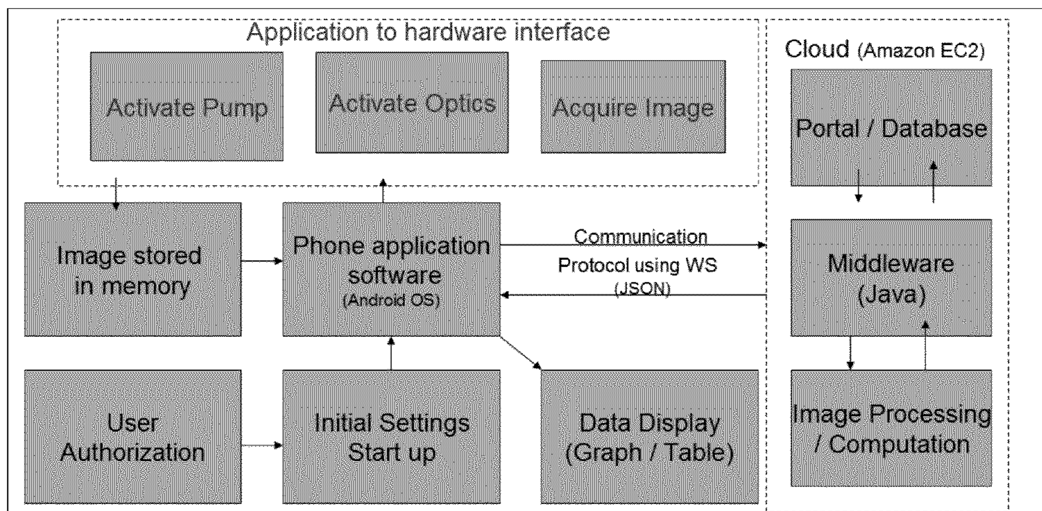
Fig. 19 Design of Smart phone for Software Control, Communication, Computation and Display
