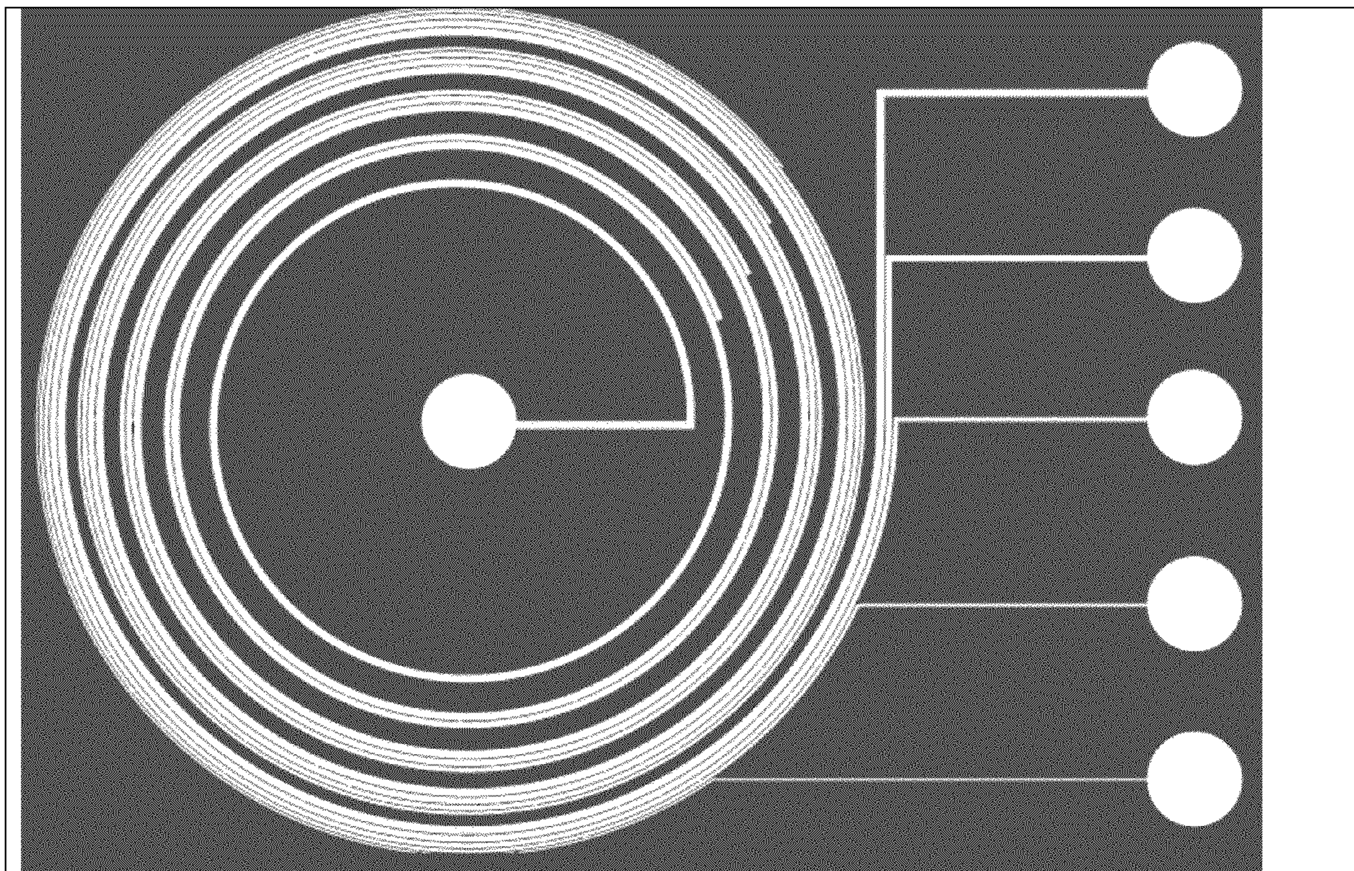
Fig. 13. Digital Centrifuge: Multiple size particulate sorting with 5 spirals.
