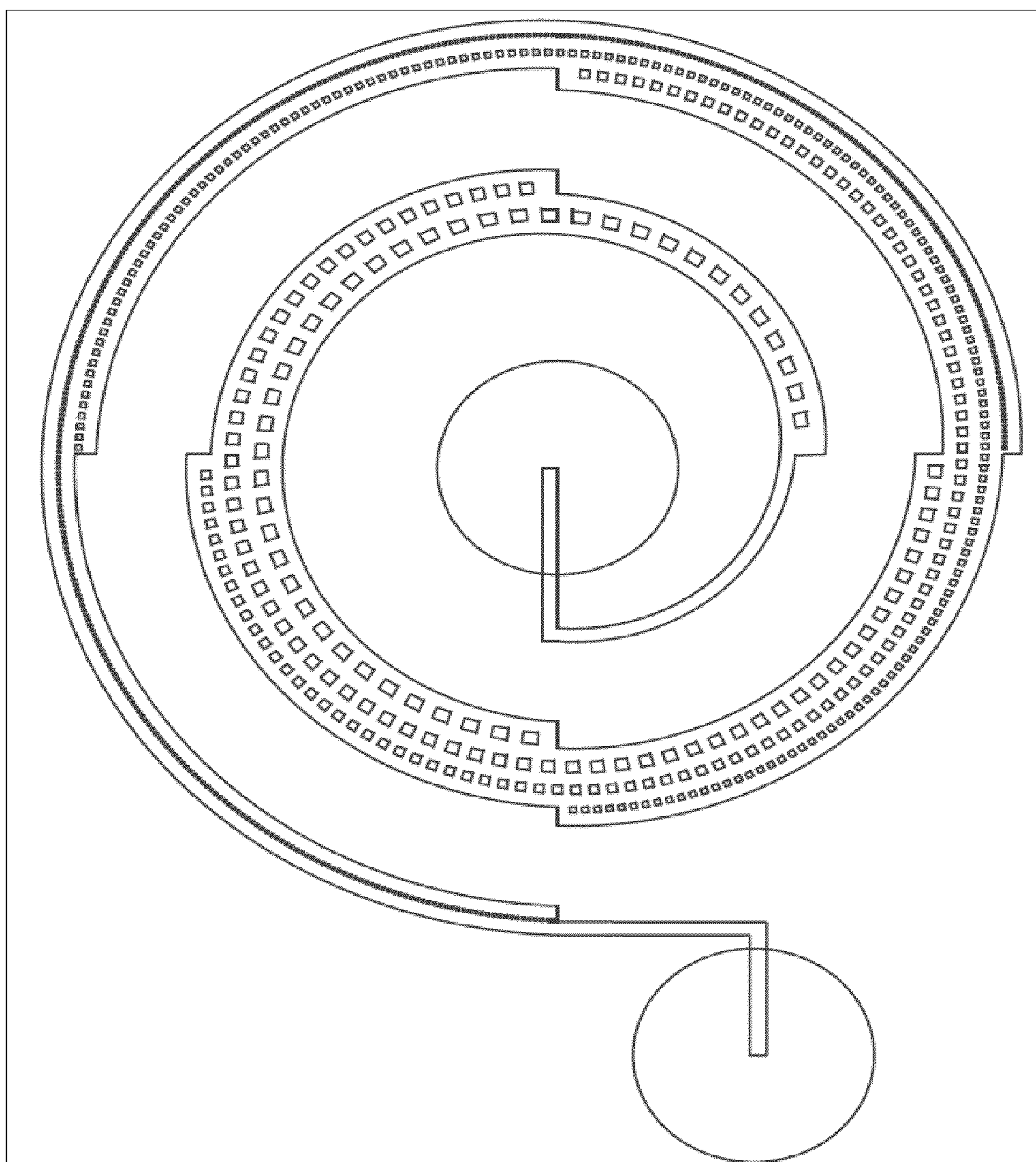
Fig.17. Design of Serum separation from whole blood using filters in spiral microfluidic channel
