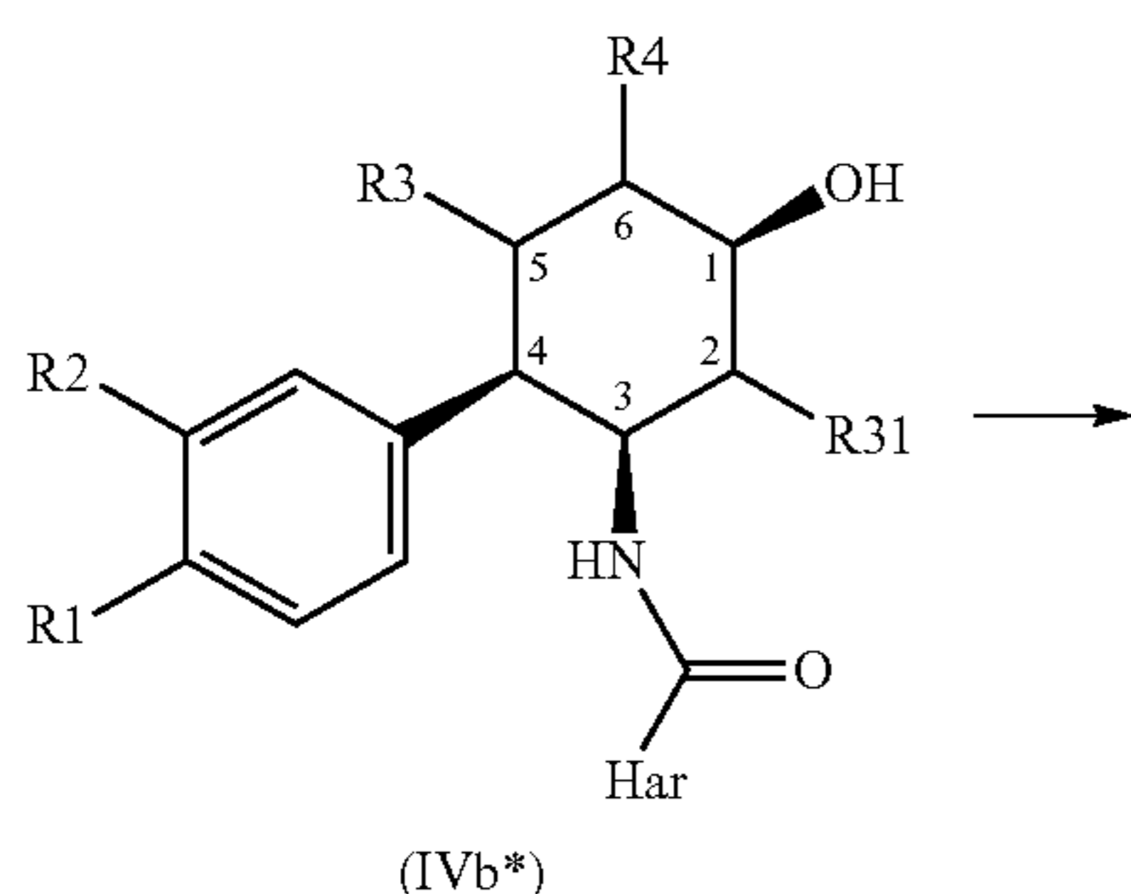
Reaction scheme 4:
