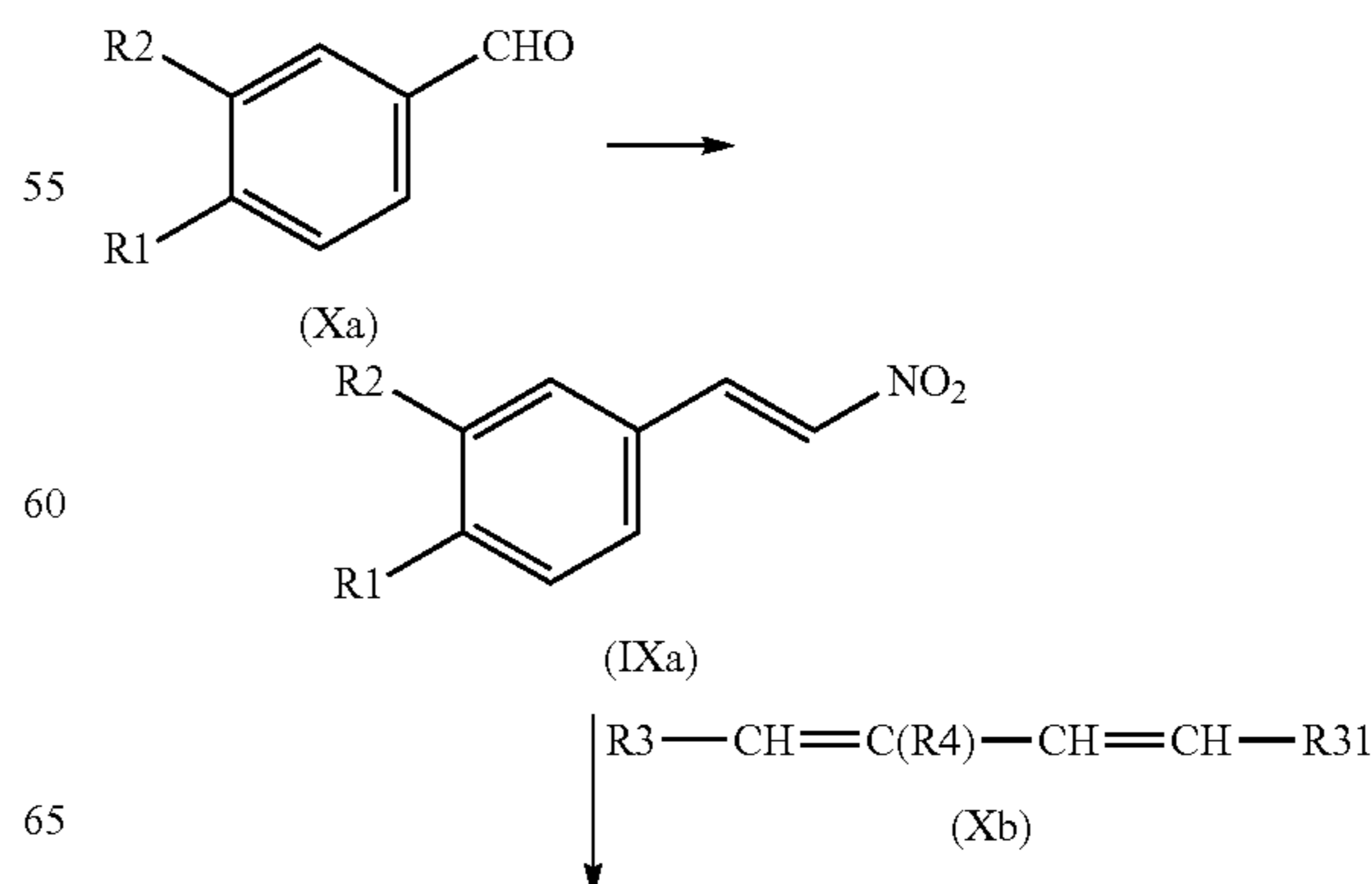
Reaction scheme 5:
