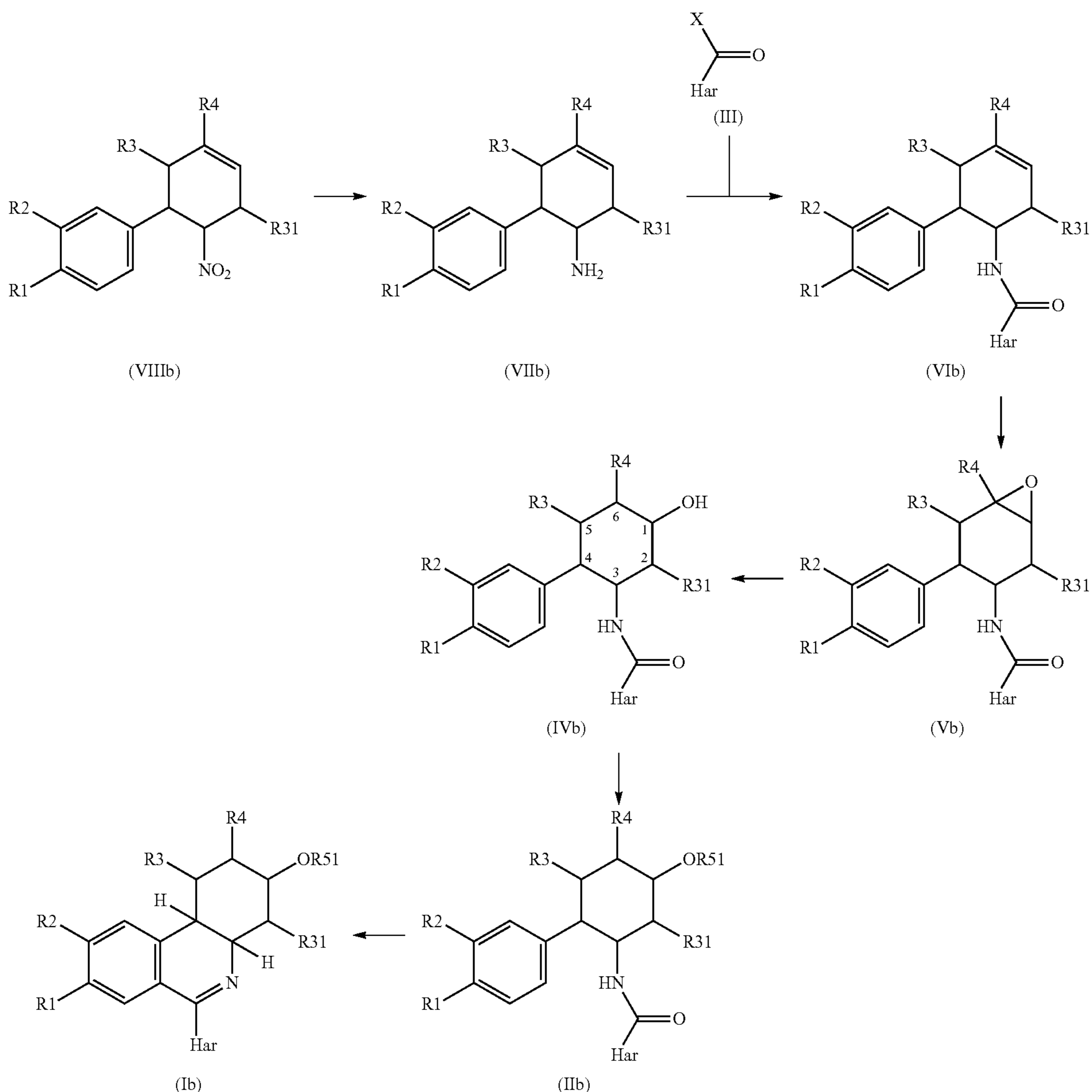
Reaction scheme 3:
