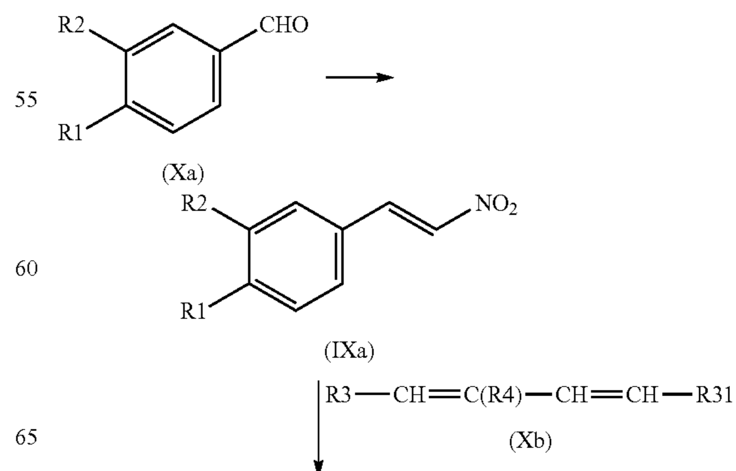
Reaction scheme 5:
