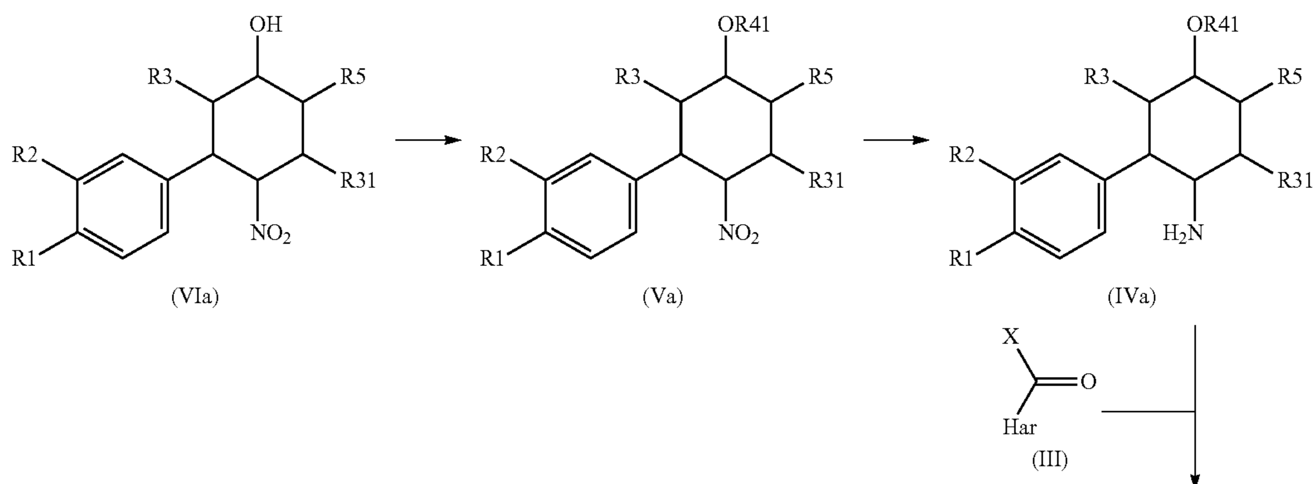
Reaction scheme 1:
