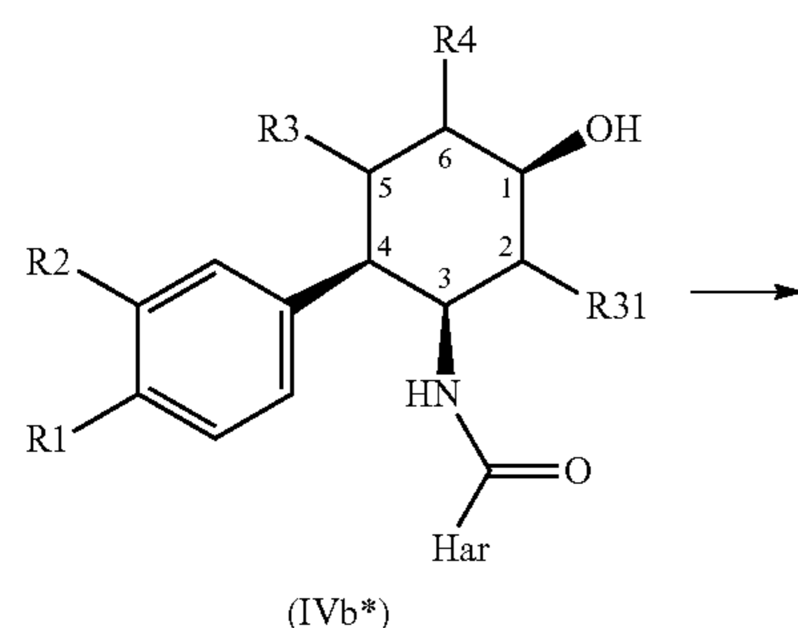
Reaction scheme 4:
