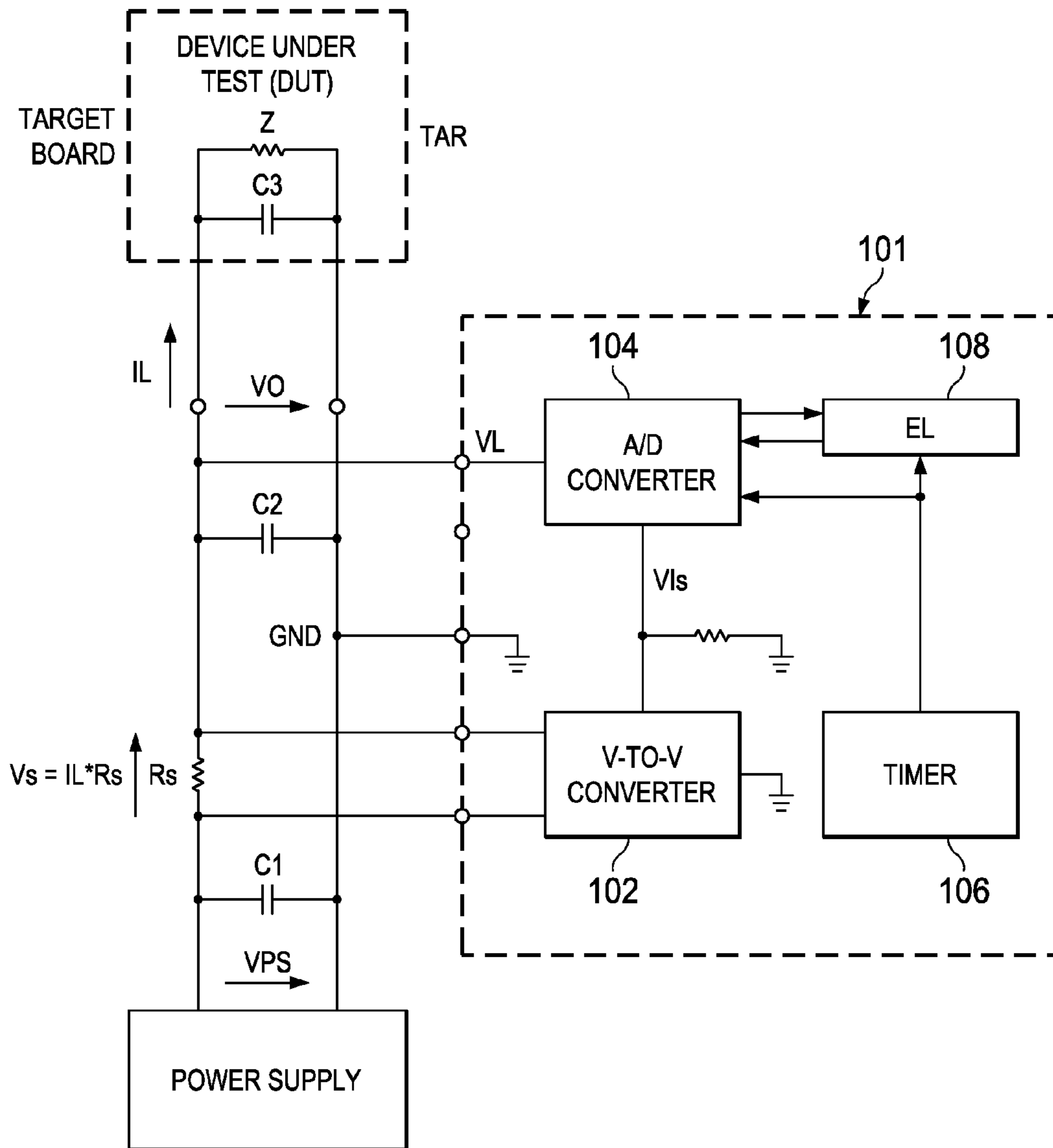
FIG. 1 (PRIOR ART)
