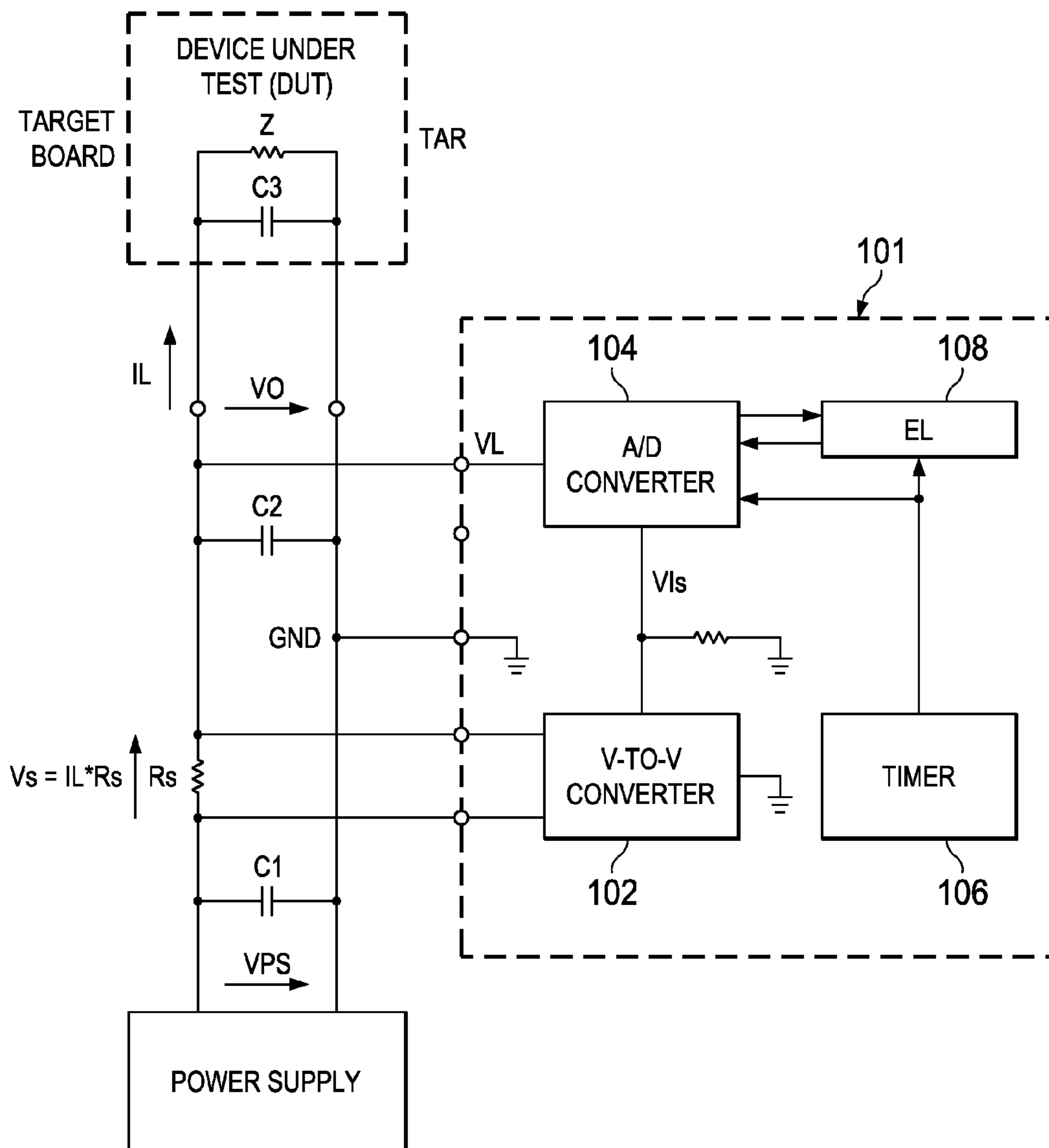
FIG. 1 (PRIOR ART)
