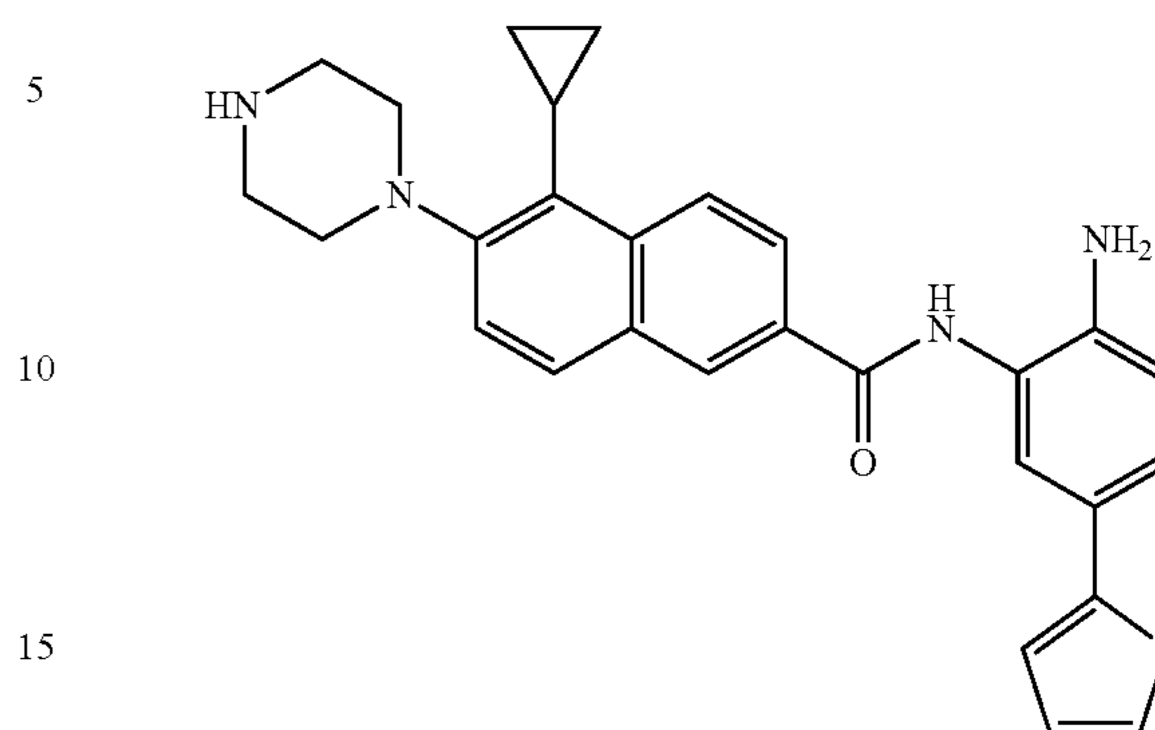
N-(2-amino-5-(thiophen-2-yl)phenyl)-5-cyclopropyl-6-(piperazin-1-yl)-2-naphthamide
