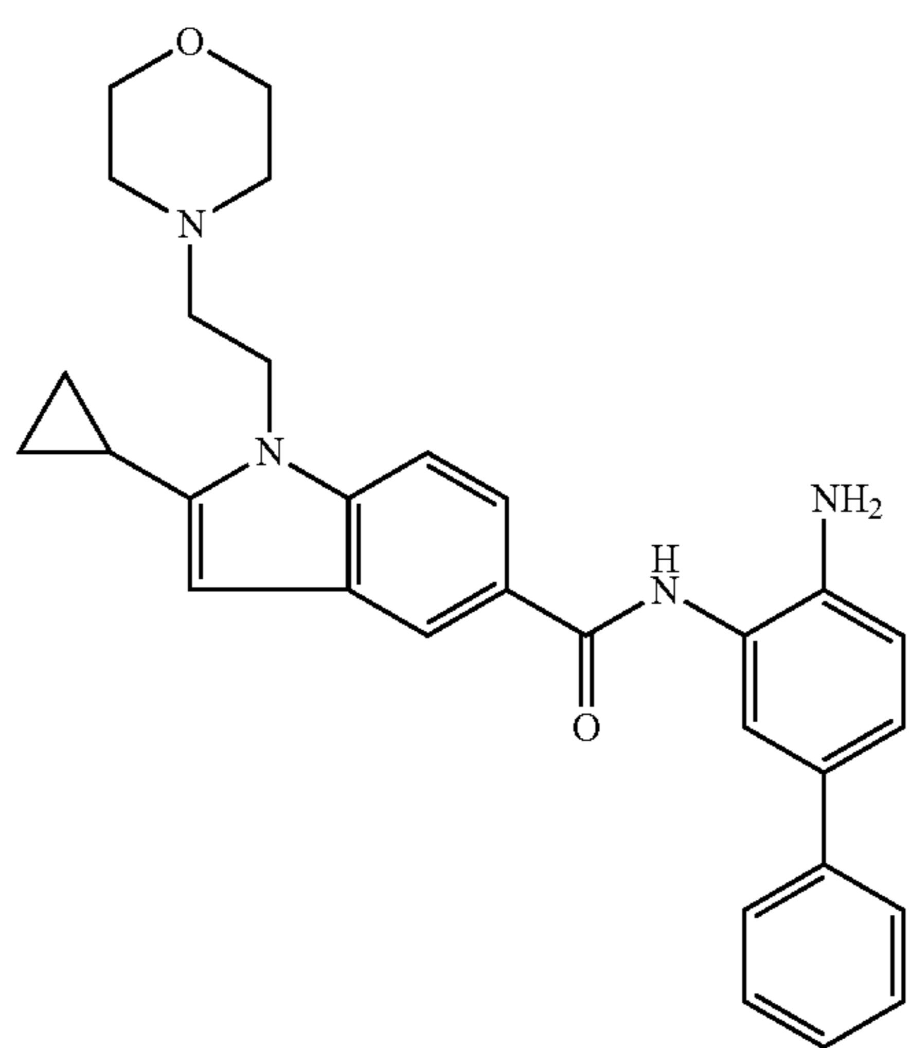
N-(4-amino-[1,1'-biphenyl]-3-yl)-2-cyclopropyl-1-(2-morpholinoethyl)-1H-indole-5-carboxamide
