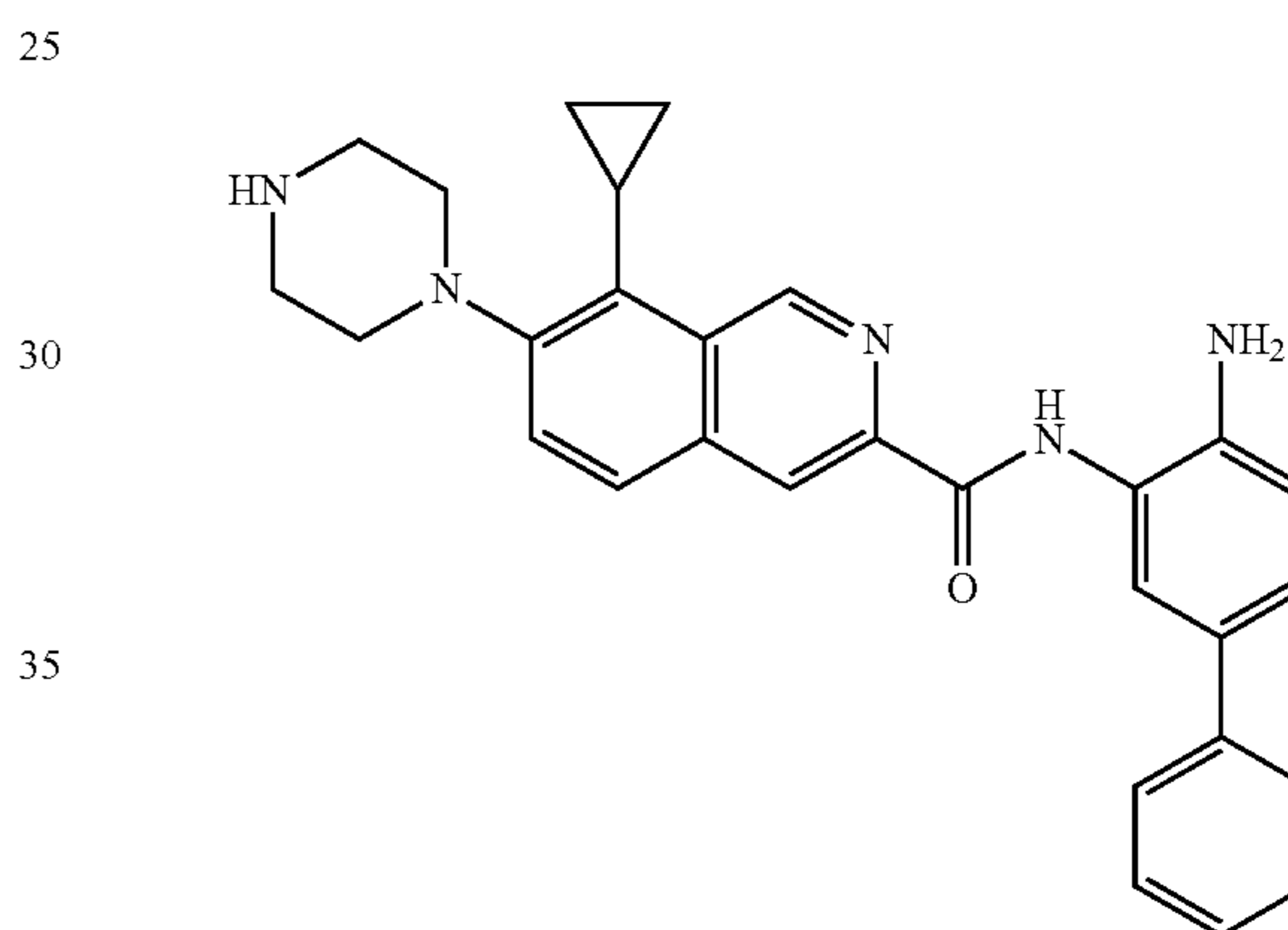
N-(4-amino-[1,1'-biphenyl]-3-yl)-8-cyclopropyl-7-(piperazin-1-yl)isoquinoline-3-carboxamide
