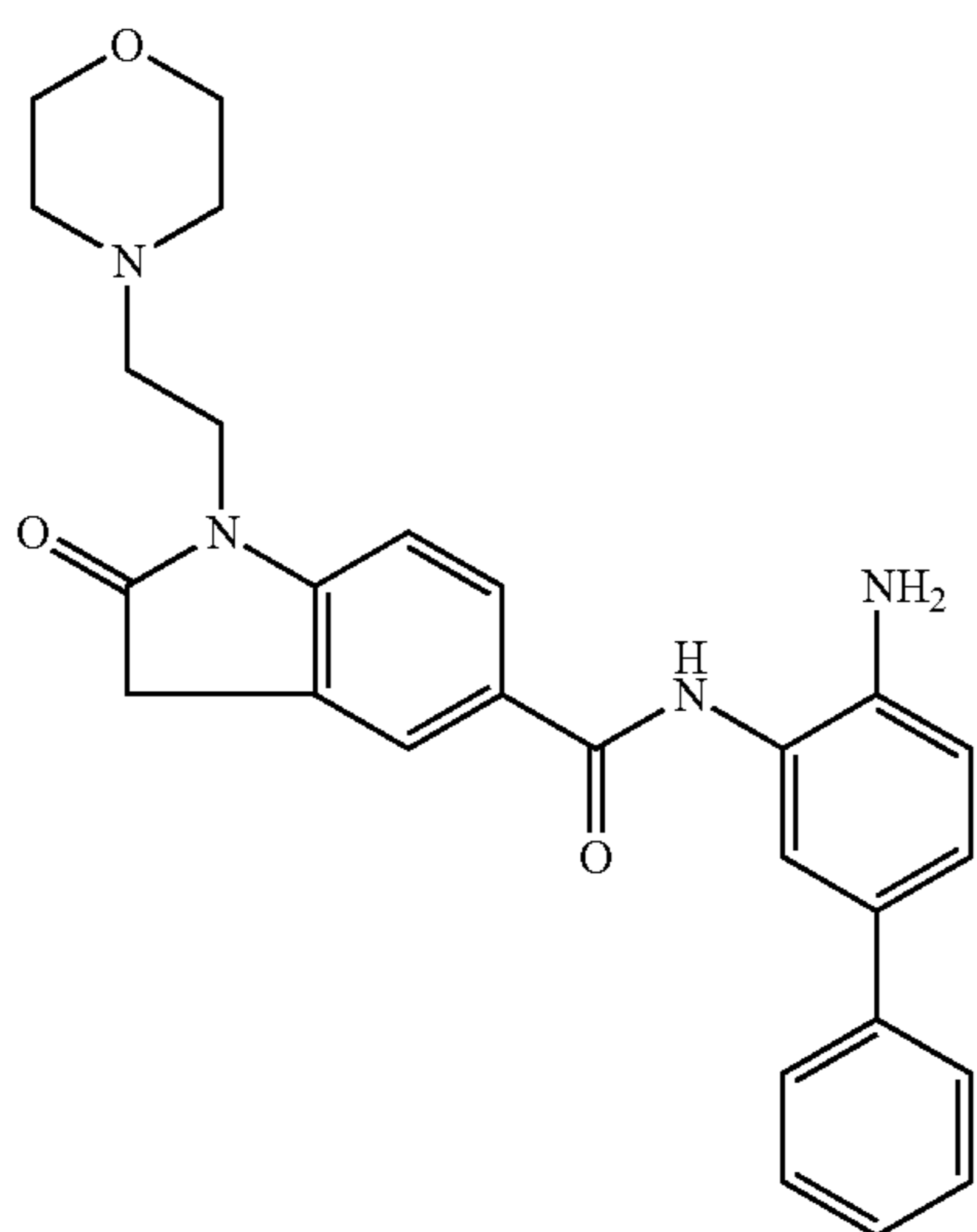
N-(4-amino-[1,1'-biphenyl]-3-yl)-1-(2-morpholinoethyl)-2-oxindoline-5-carboxamide
