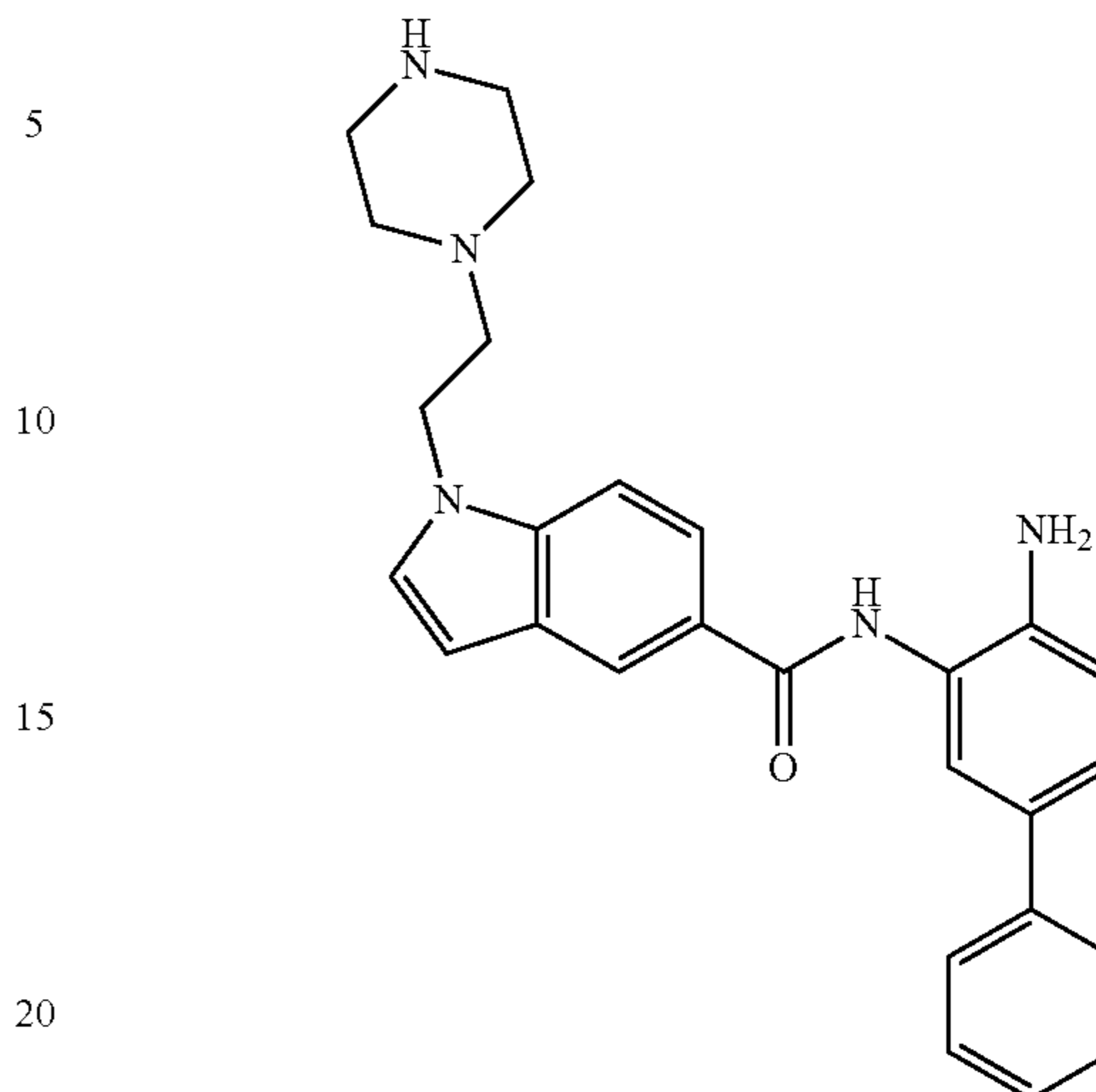
N-(4-amino-[1,1'-biphenyl]-3-yl)-1-(2-(piperazin-1-yl)ethyl)-1H-indole-5-carboxamide
