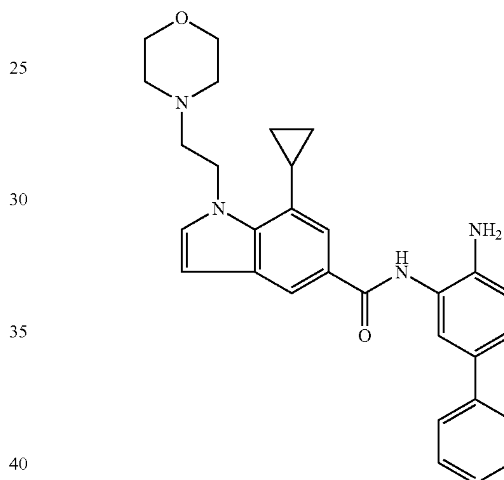
N-(4-amino-[1,1'-biphenyl]-3-yl)-7-cyclopropyl-1-(2-morpholinoethyl)-1H-indole-5-carboxamide
