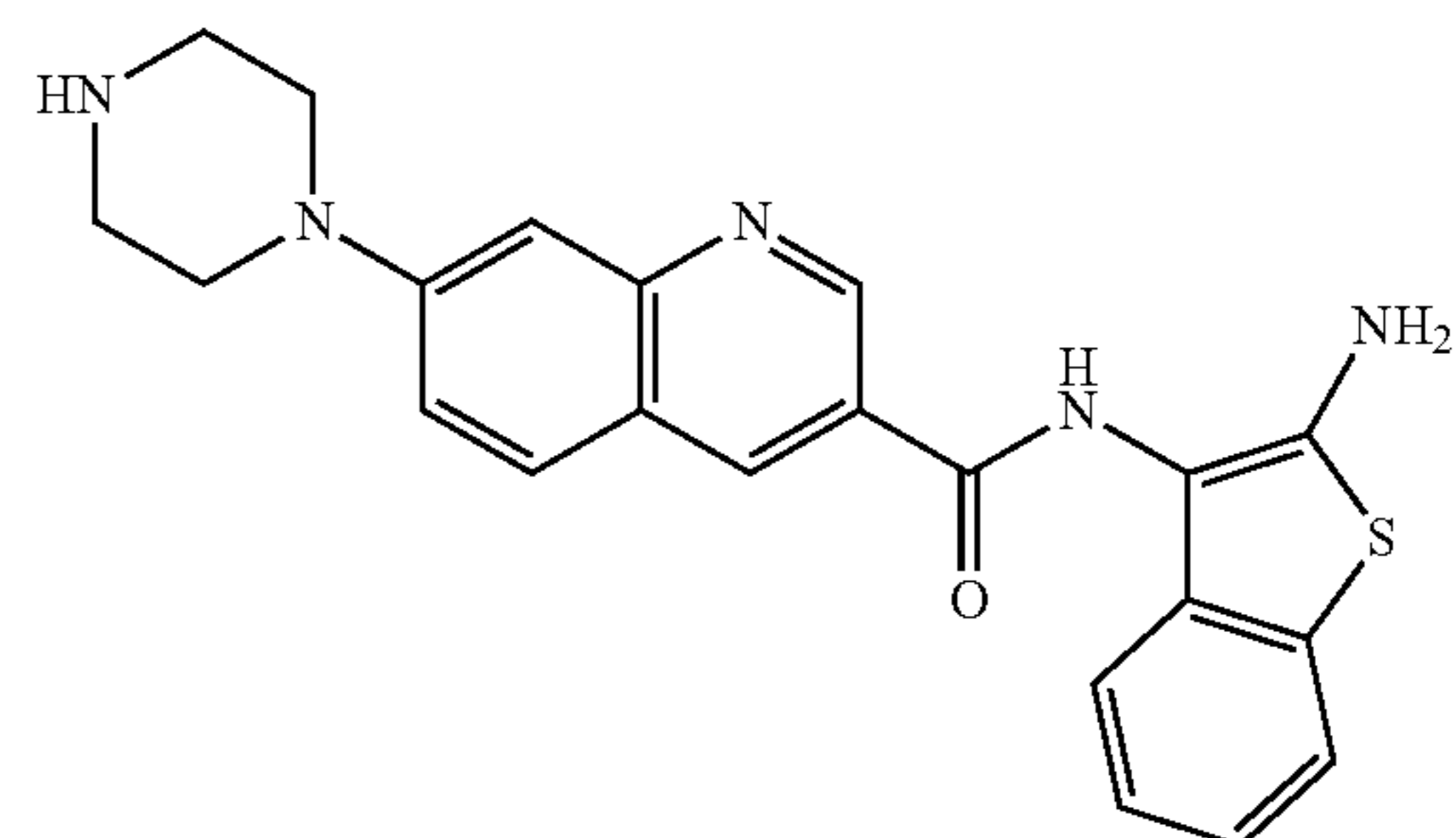
N-(2-aminobenzo[b]thiophen-3-yl)-7-(piperazin-1-yl)quinoline-3-carboxamide
