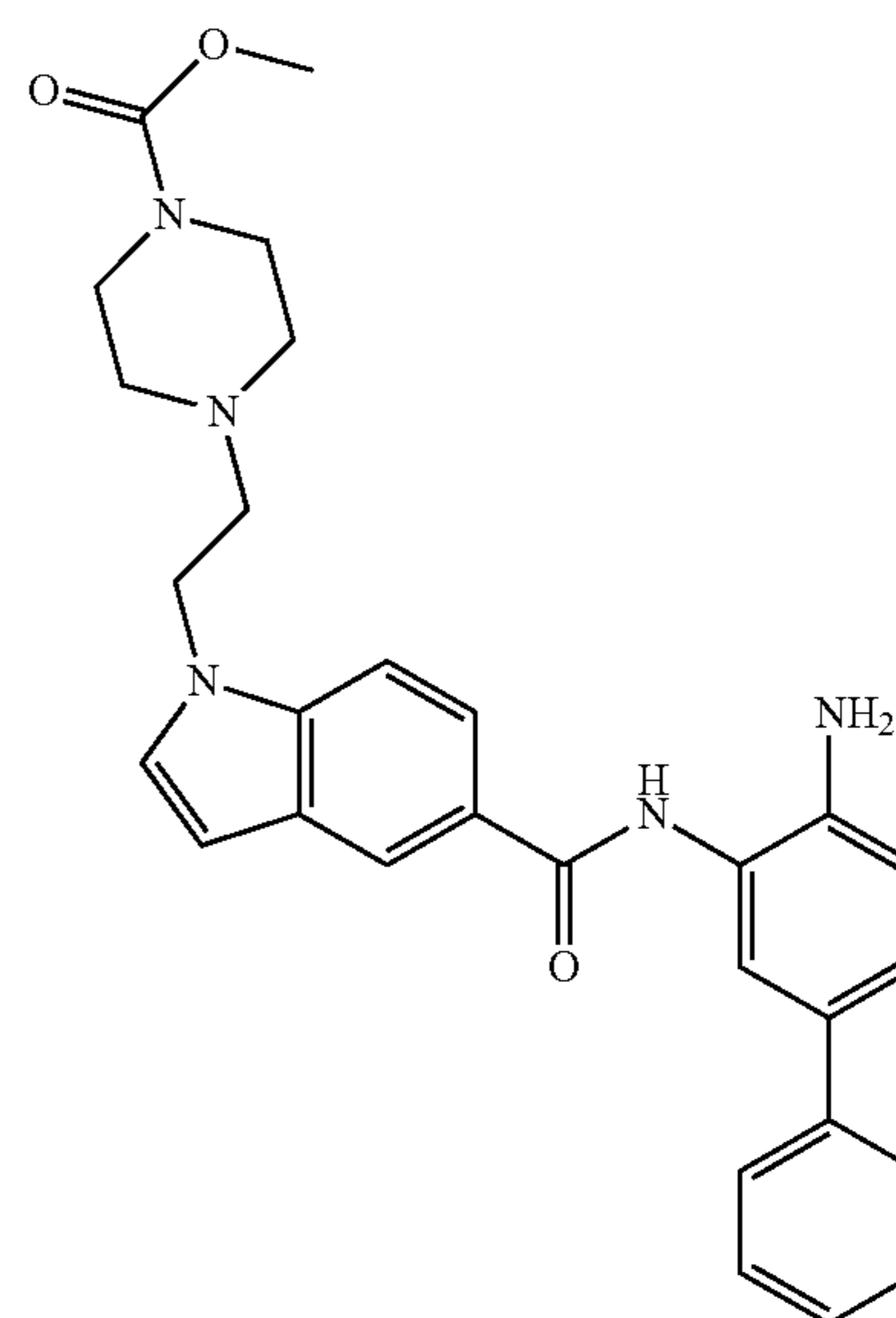
methyl 4-(2-(5-((4-amino-[1,1'-biphenyl]-3-yl)carbamoyl)-1H-indol-1-yl)ethyl)piperazine-1-carboxylate
