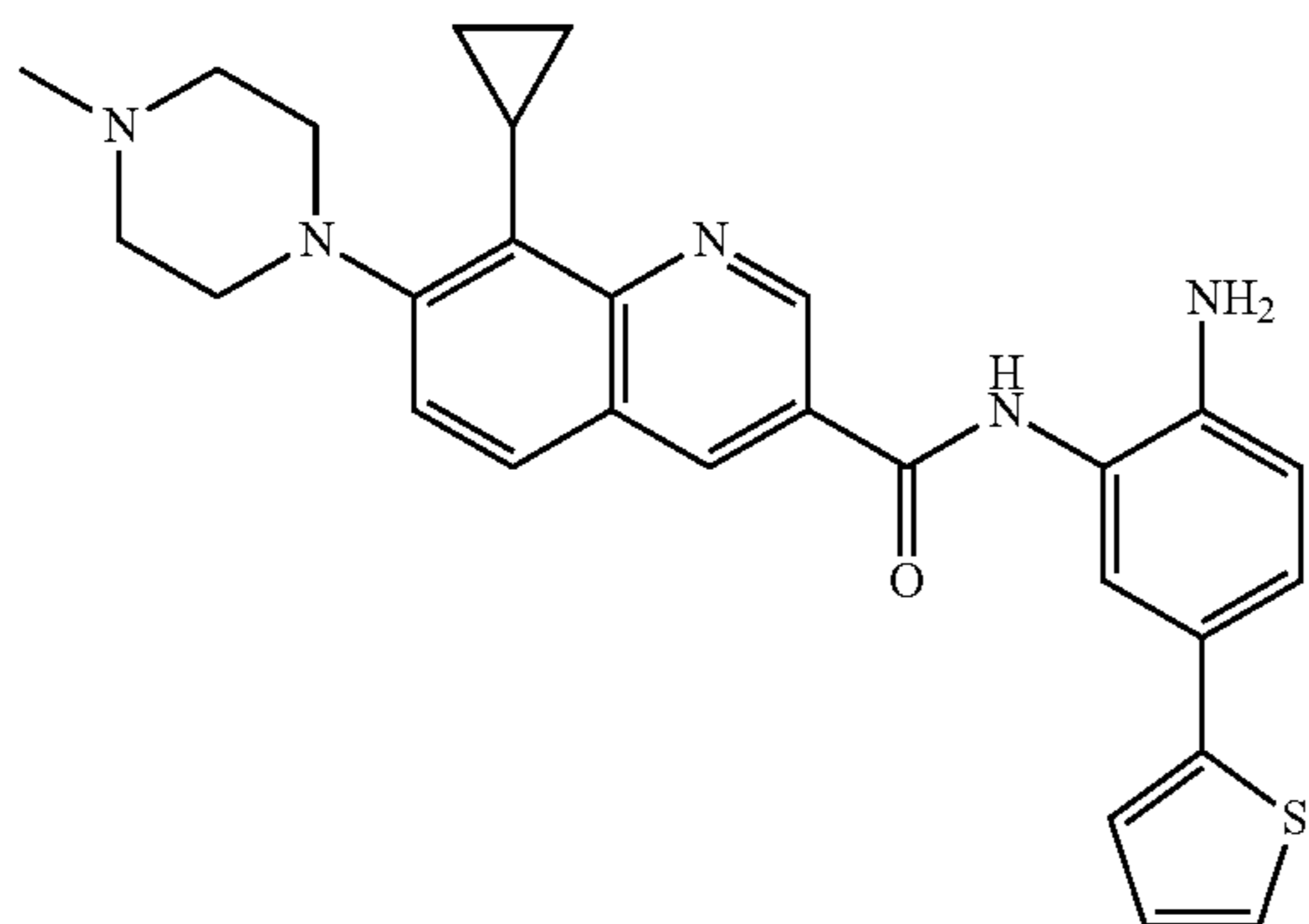
N-(2-amino-5-(thiophen-2-yl)phenyl)-8-cyclopropyl-7-(4-methylpiperazin-1-yl)quinoline-3-carboxamide
