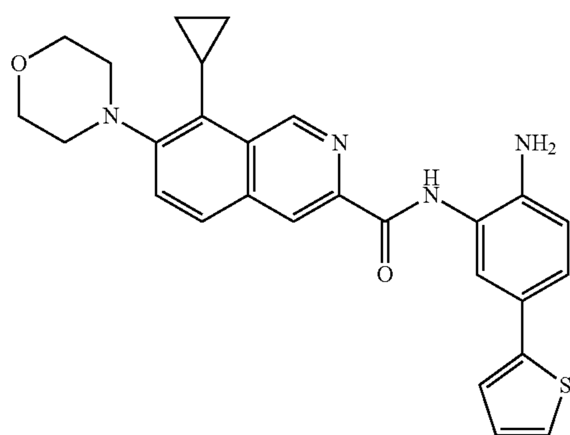
N-(2-amino-5-(thiophen-2-yl)phenyl)-8-cyclopropyl-7-morpholinoisoquinoline-3-carboxamide
