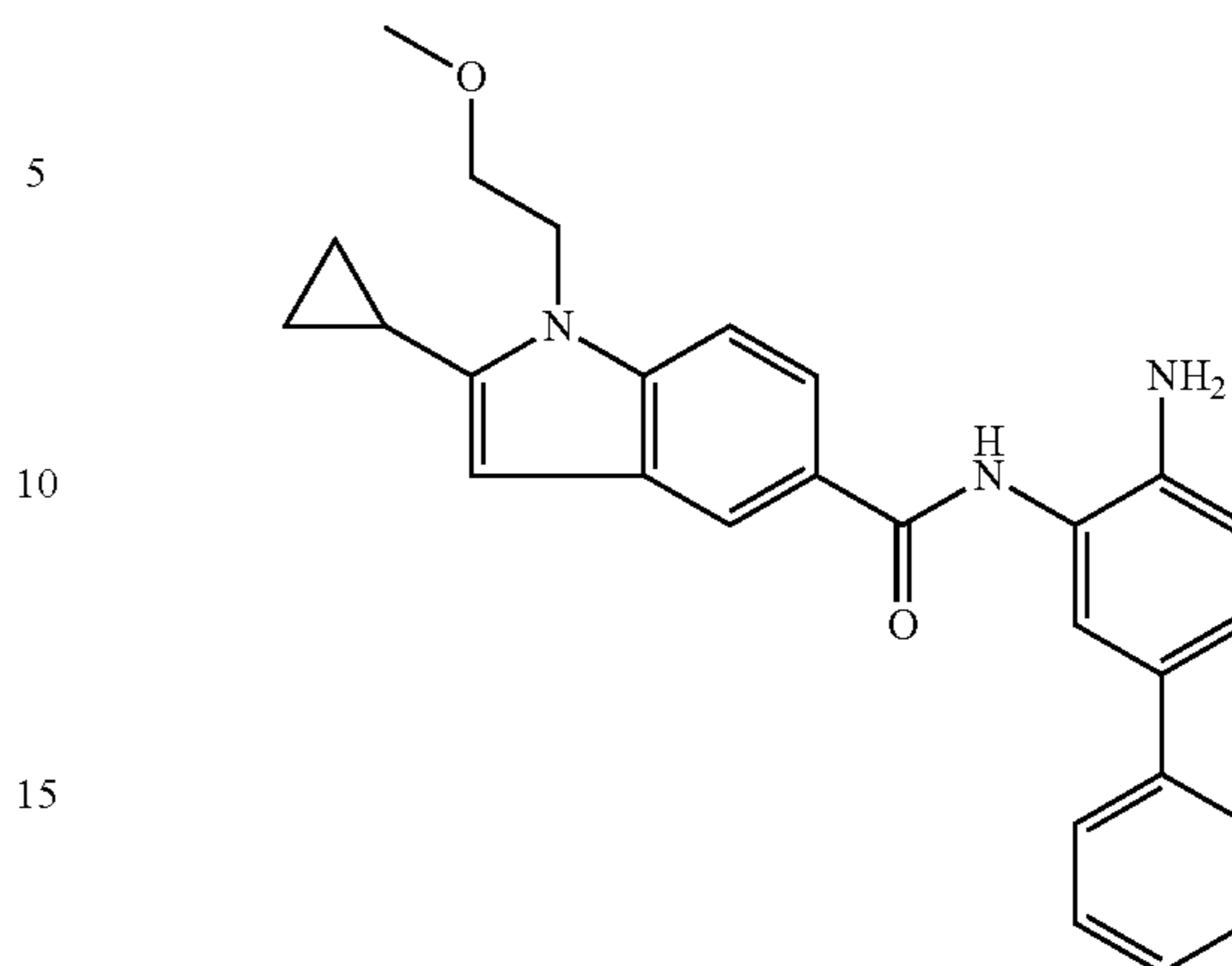
N-(4-amino-[1,1'-biphenyl]-3-yl)-2-cyclopropyl-1-(2-methoxyethyl)-1H-indole-5-carboxamide
