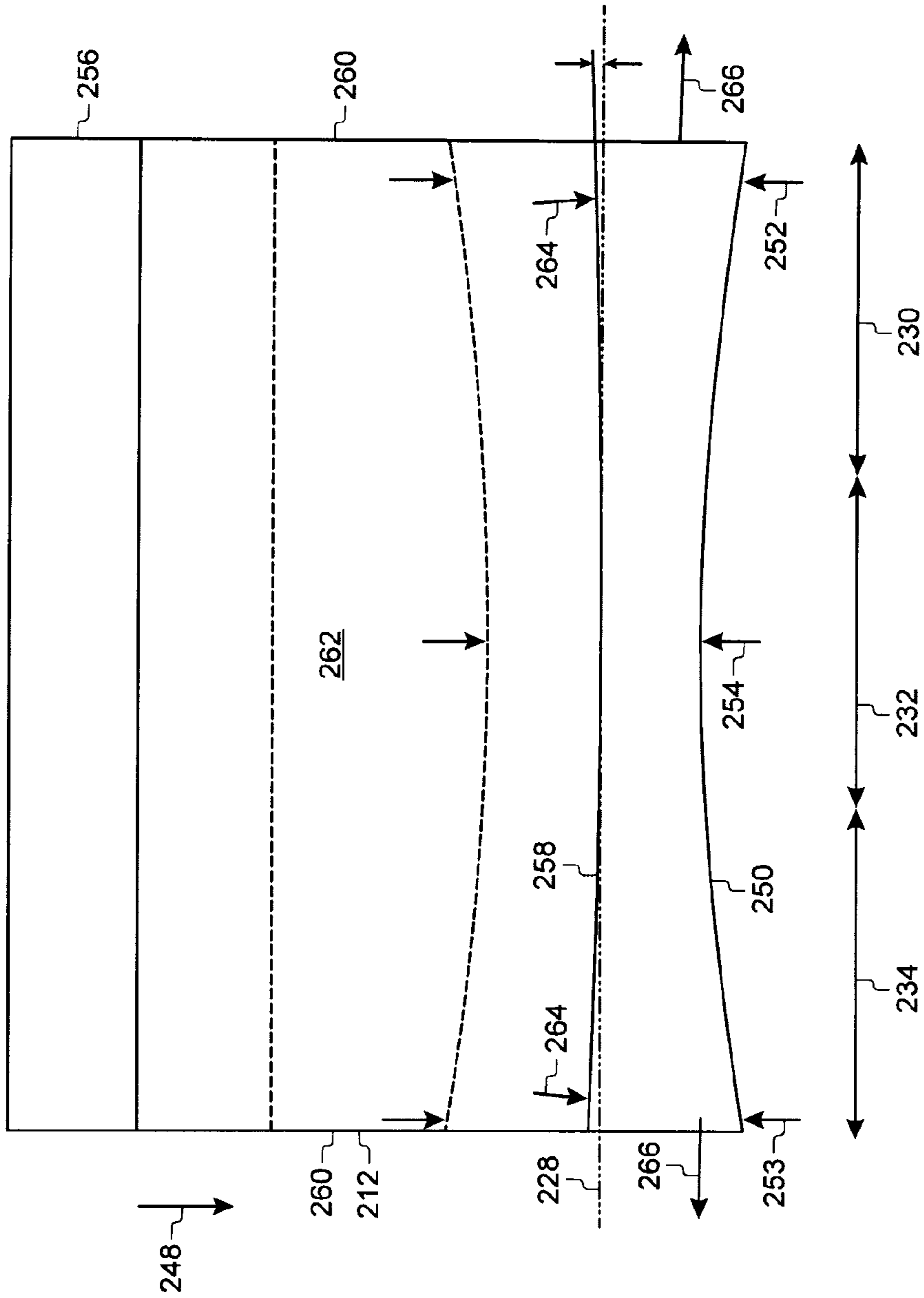
FIG. 4 (PRIOR ART)
