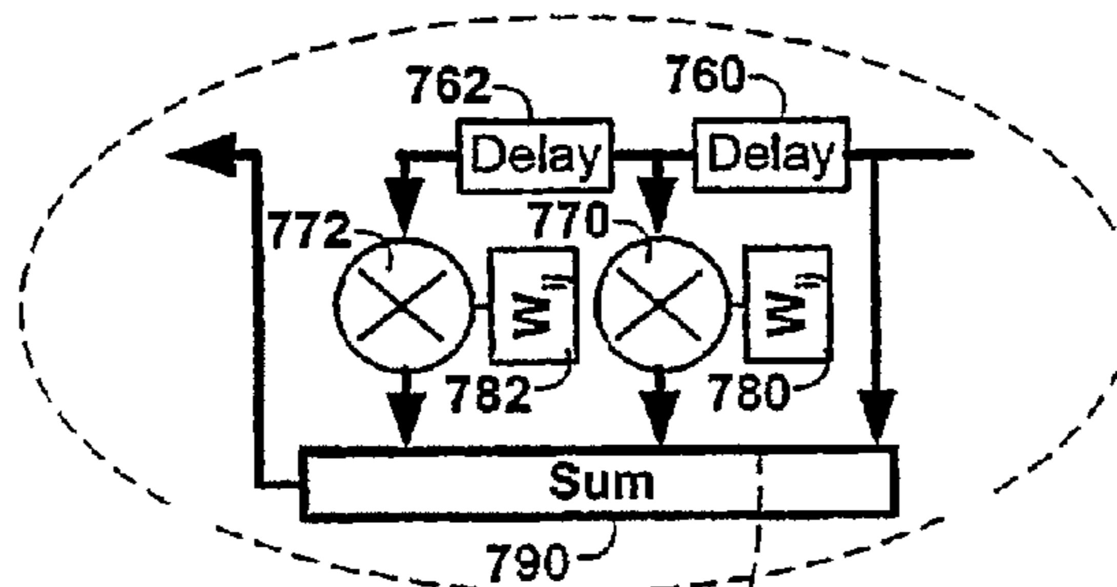
Space-Time Processor FIG. 7C
