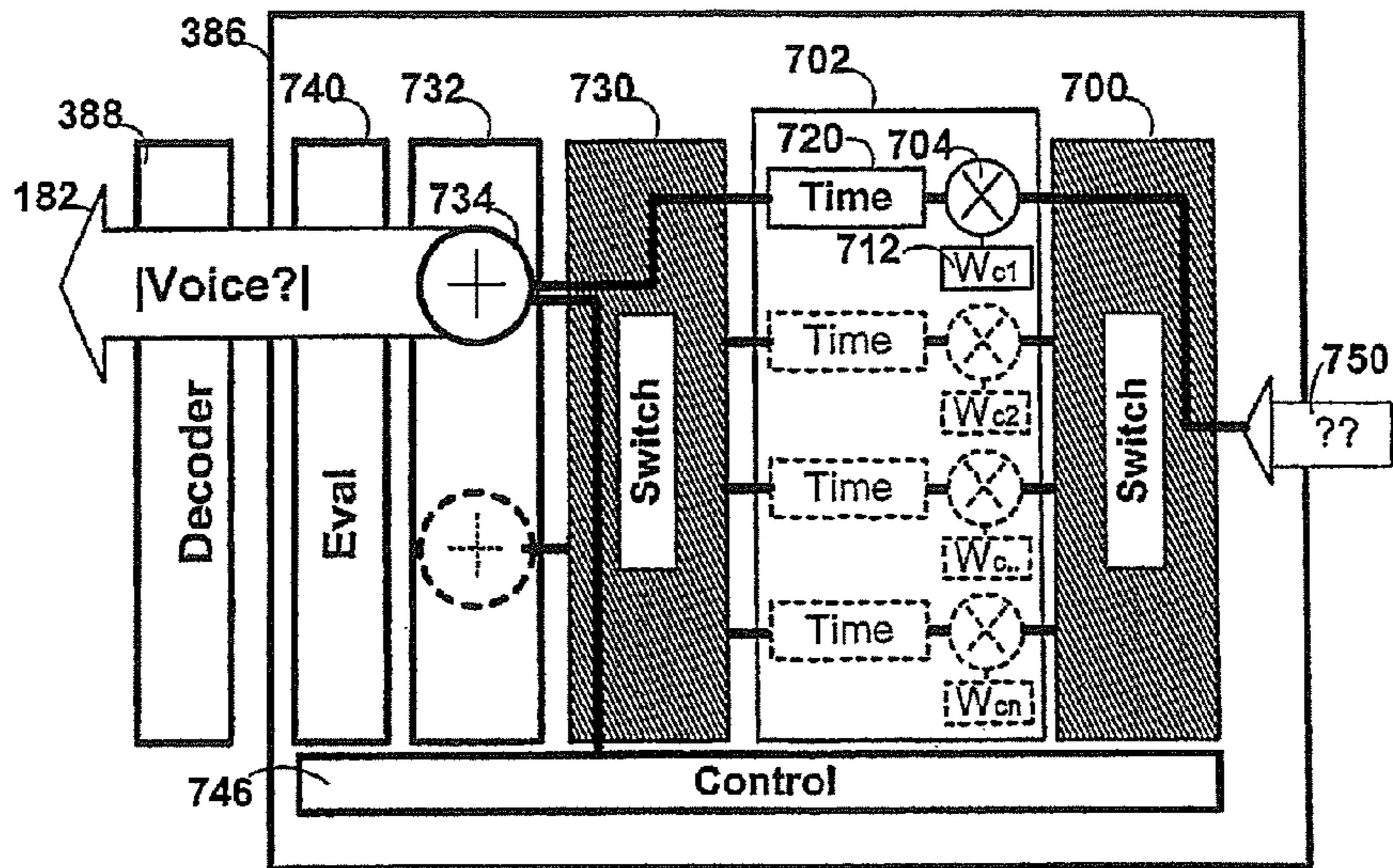
Space-Time Processor FIG. 7C
