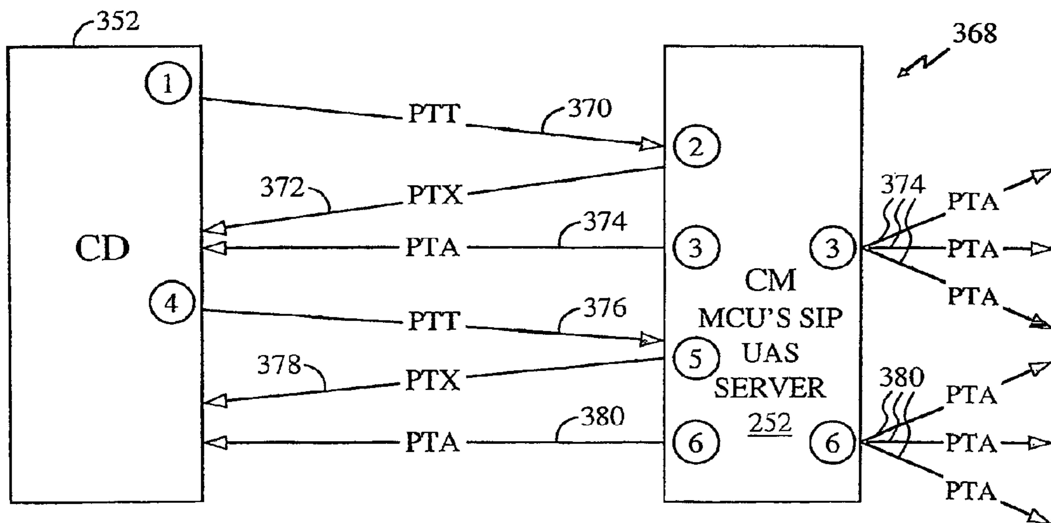
FIG. 12 MEDIA SIGNALING MESSAGE SEQUENCE (PTT)
