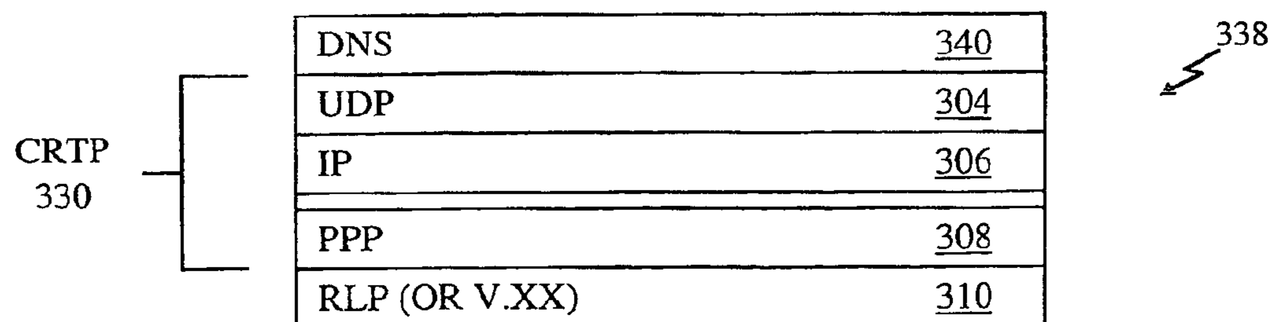
DNS CLIENT PROTOCOL STACK
