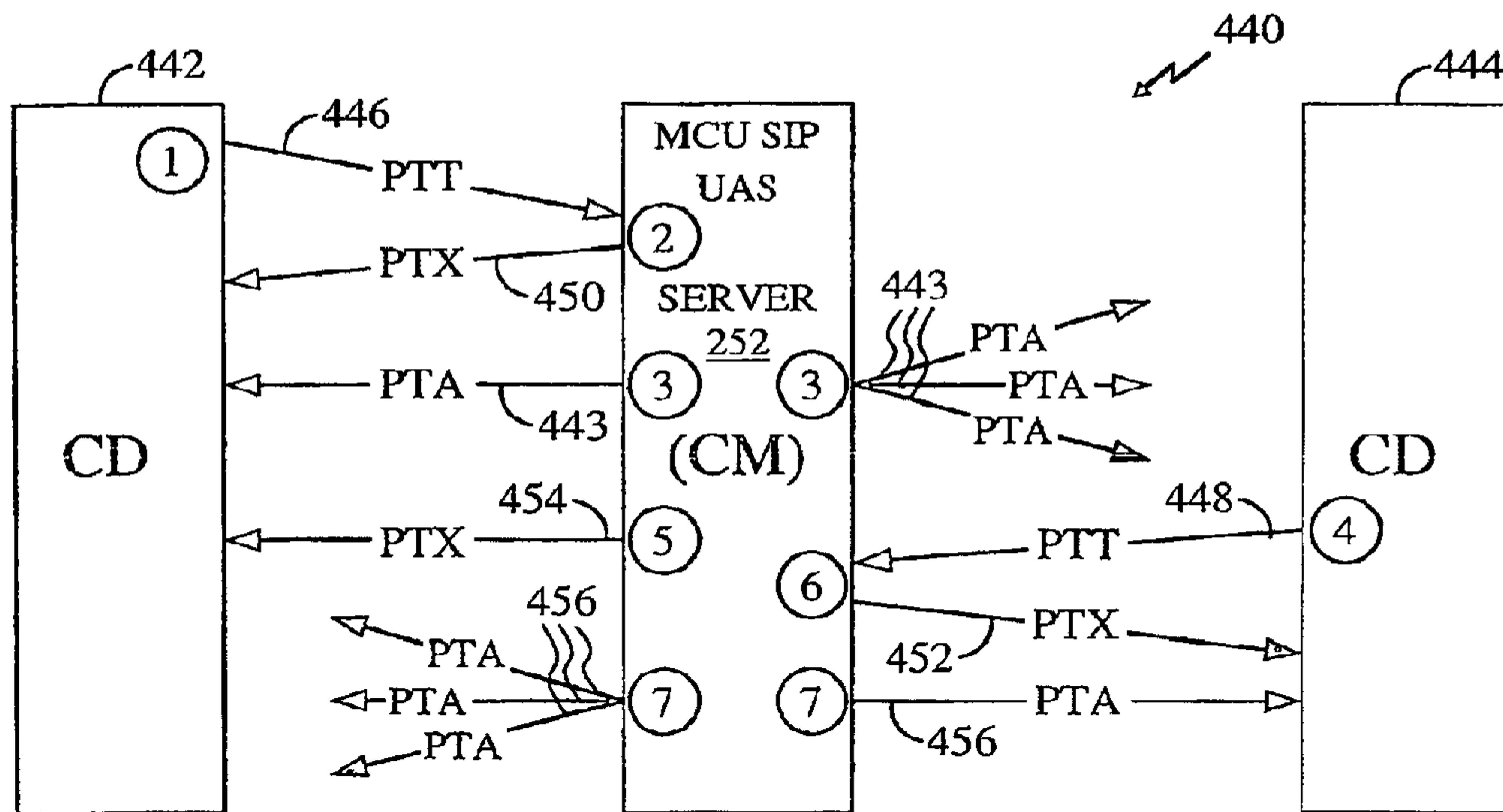
MEDIA SIGNALING MESSAGE SEQUENCE (PRIORITY ARBITRATION)
