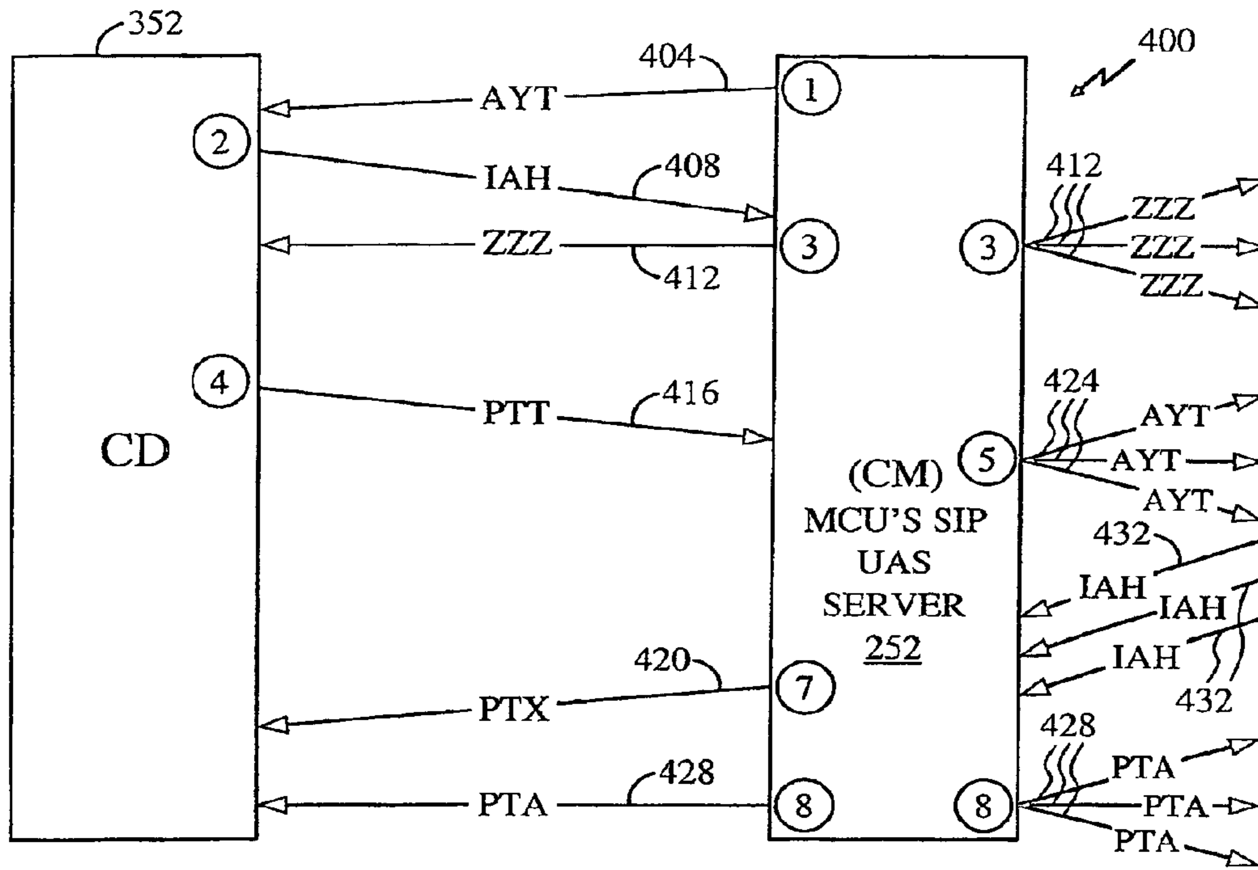
MEDIA SIGNALING MESSAGE SEQUENCE (DORMANCY)
