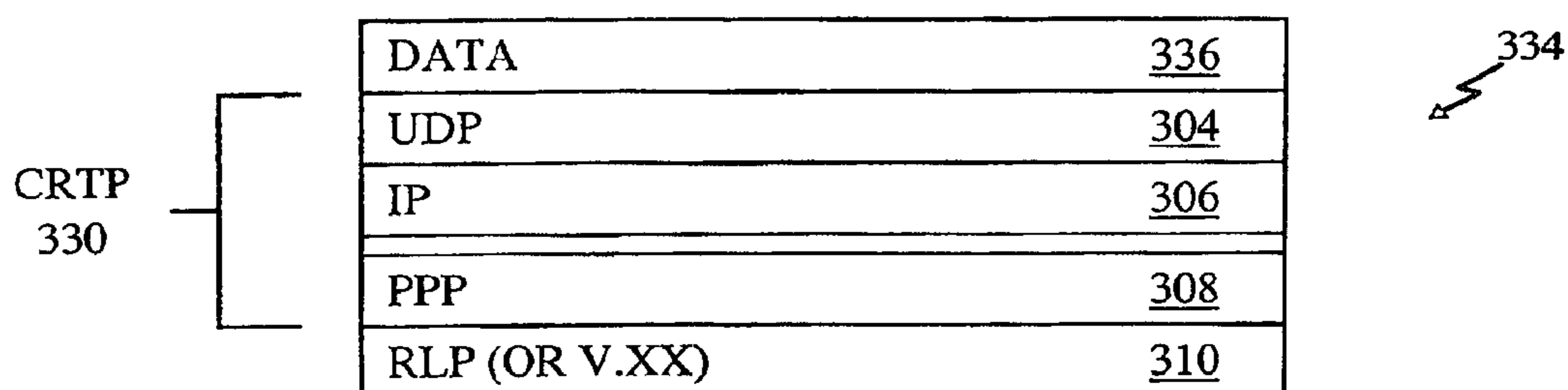
MEDIA TRAFFIC (DATA) PROTOCOL STACK
