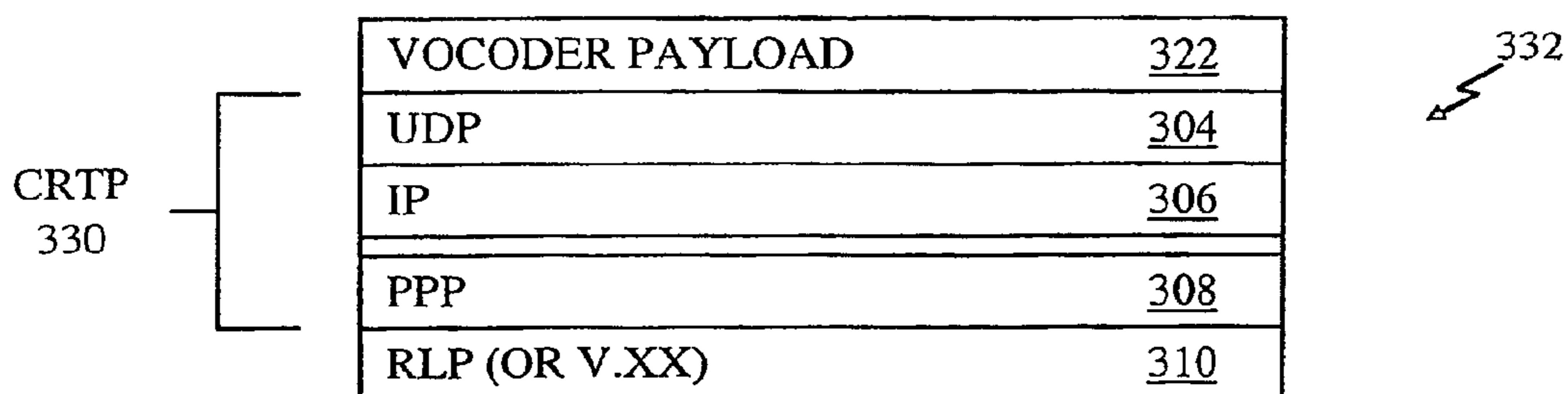
UDP VOICE MEDIA PROTOCOL STACK
