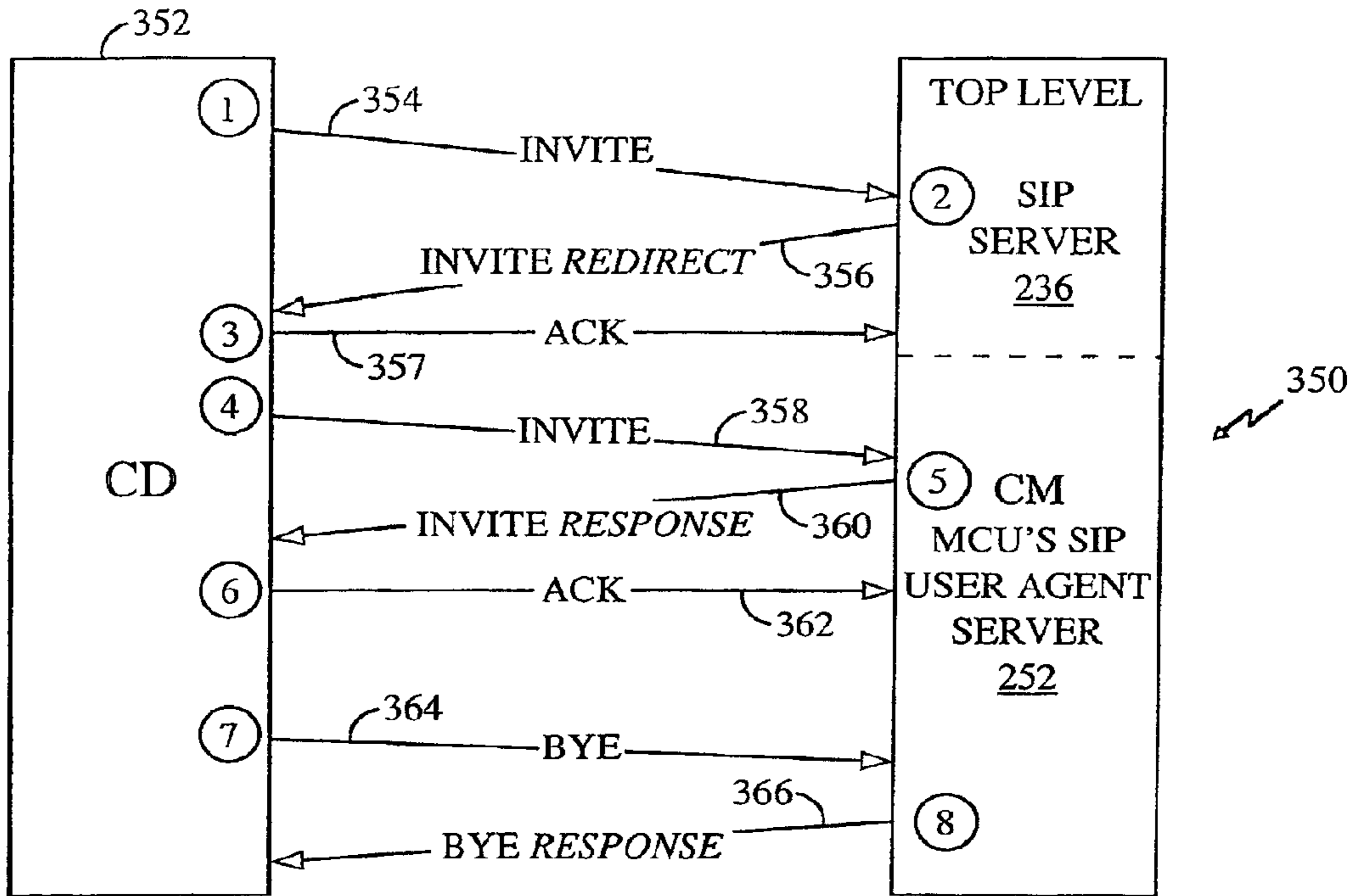
FIG. 11 SIP CALL SIGNALING
