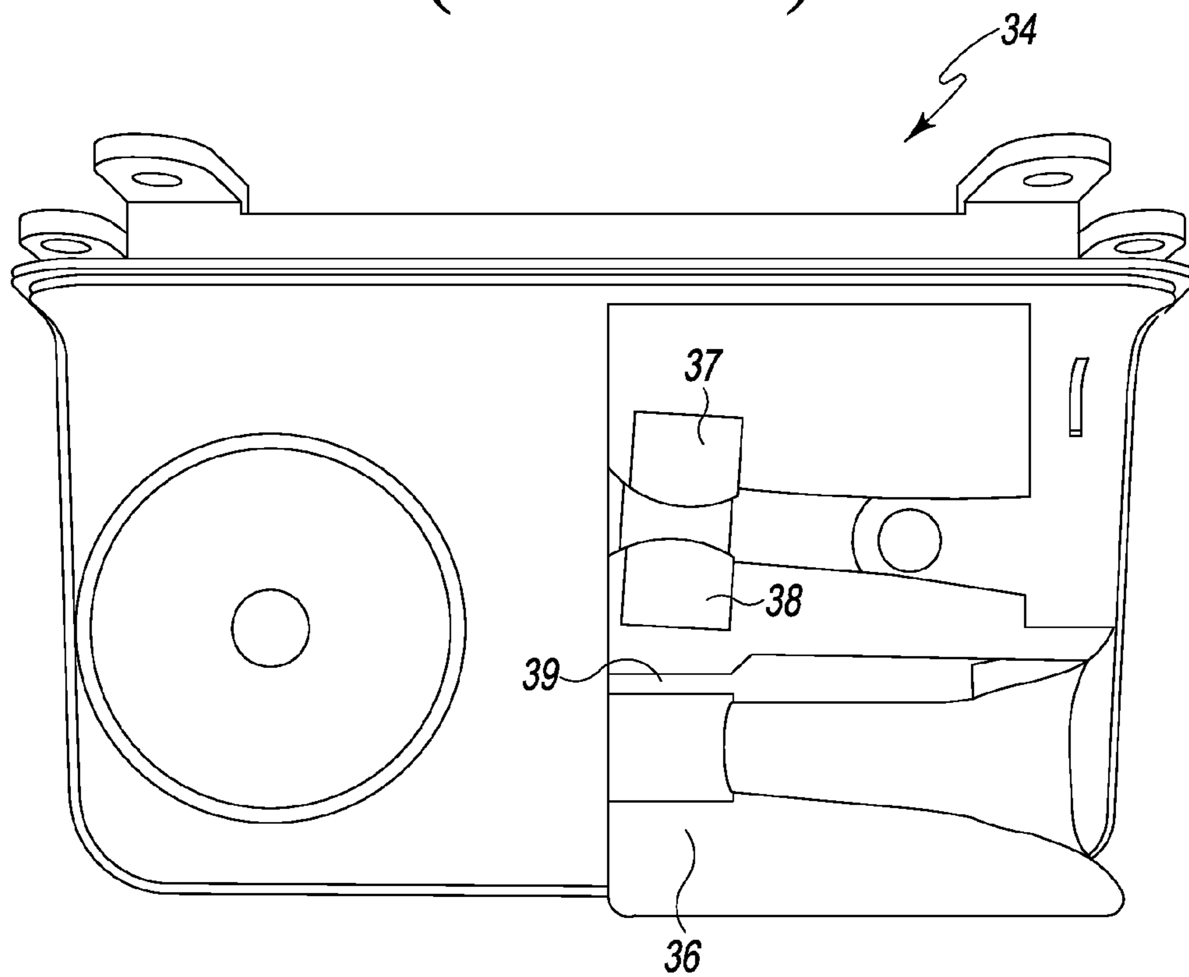
Fig. 3 (Prior Art)
