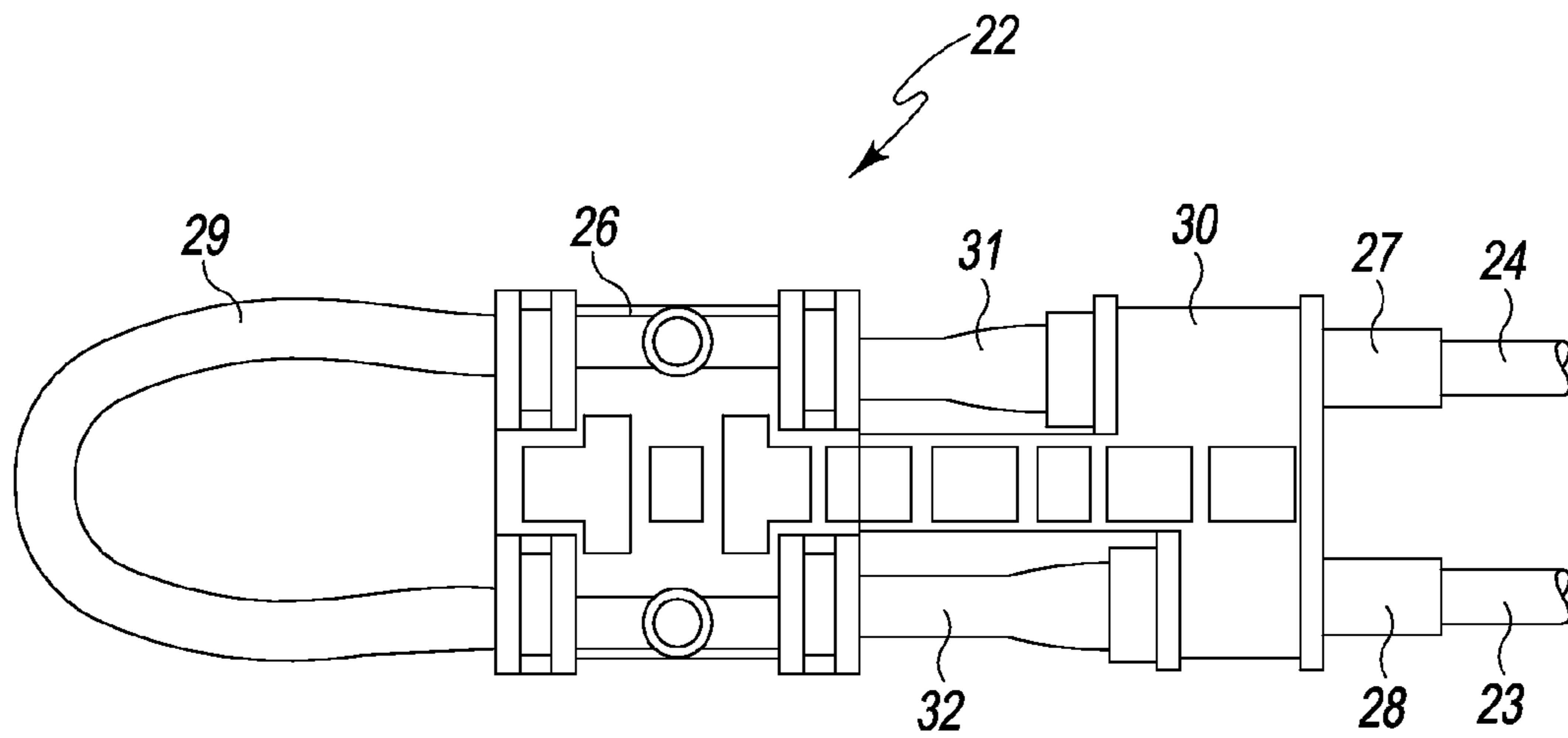
Fig. 2 (Prior Art)
