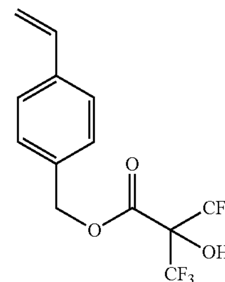
Monomer 1
