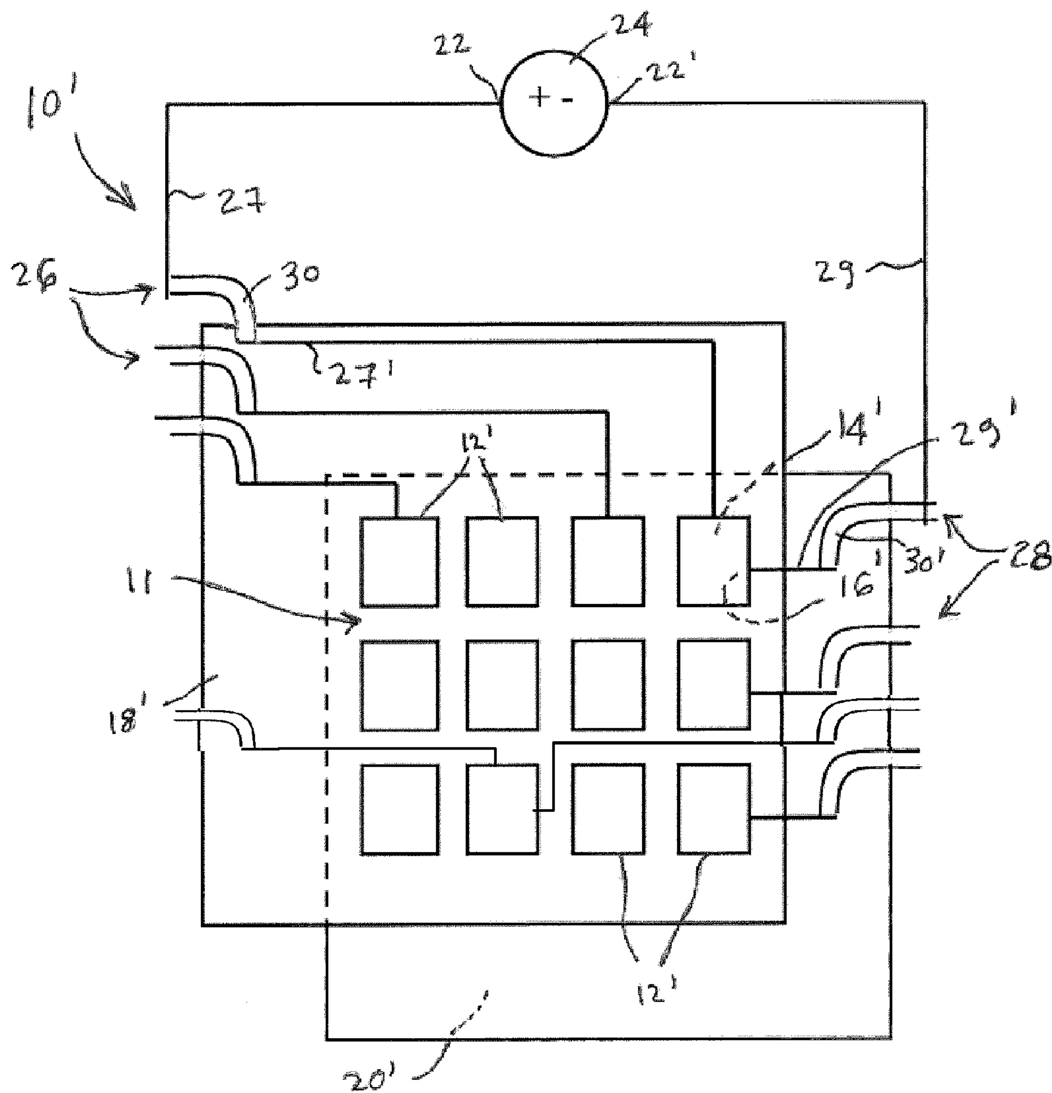
Fig. 4 (Prior Art)
