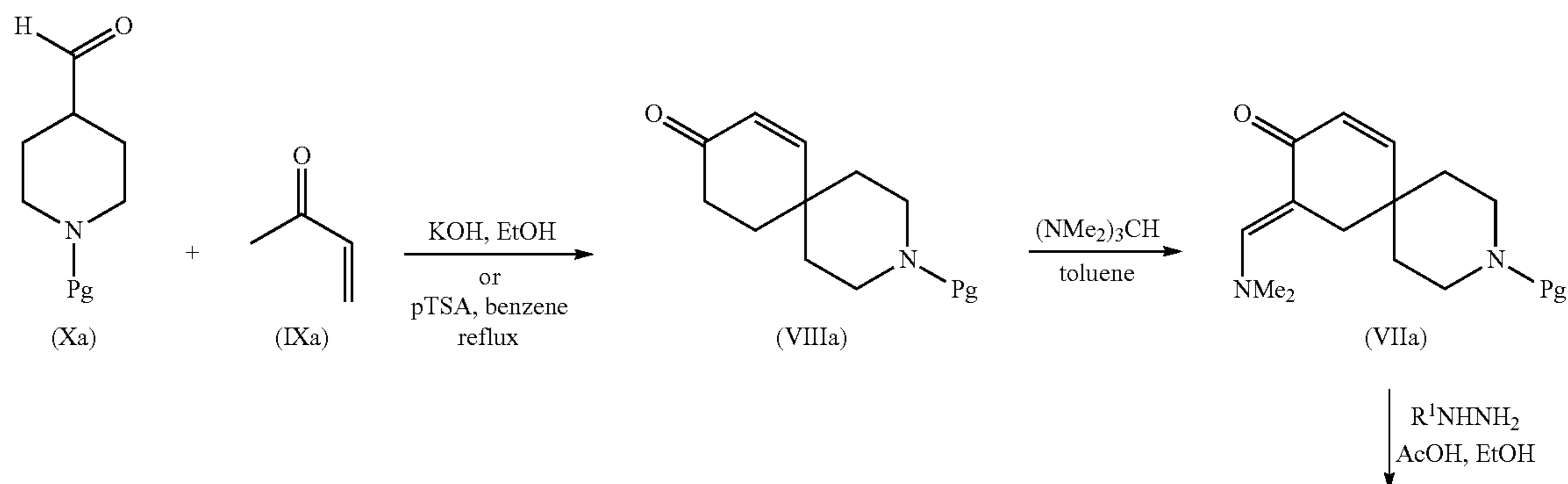
Reaction Scheme I
