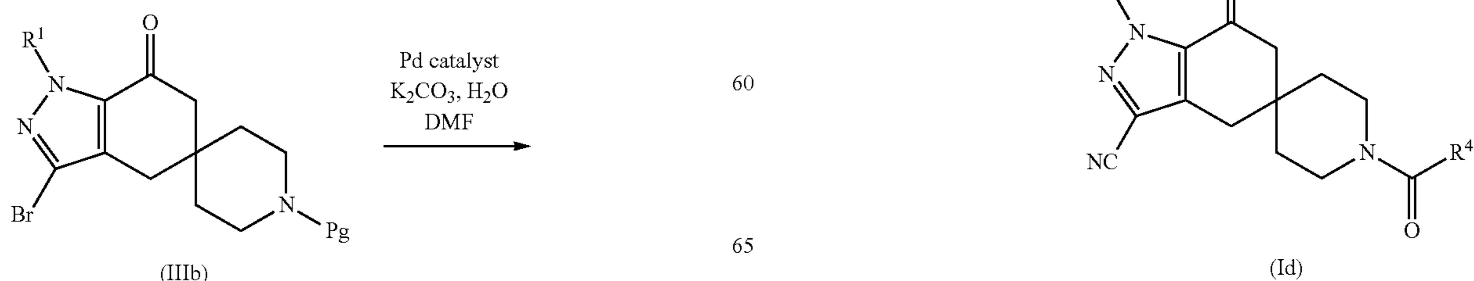
Reaction Scheme IV
