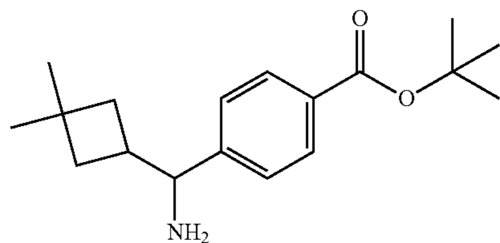
tert-butyl 4-(amino(3,3-dimethylcyclobutyl)methyl)benzoate
