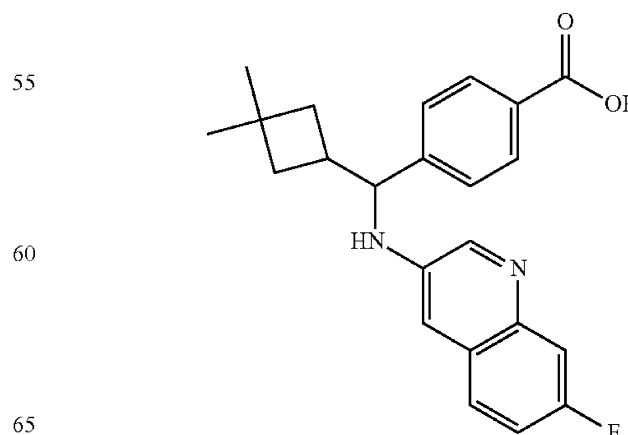
4-((3,3-dimethylcyclobutyl)(7-fluoroquinolin-3-ylamino)methyl)benzoic acid
