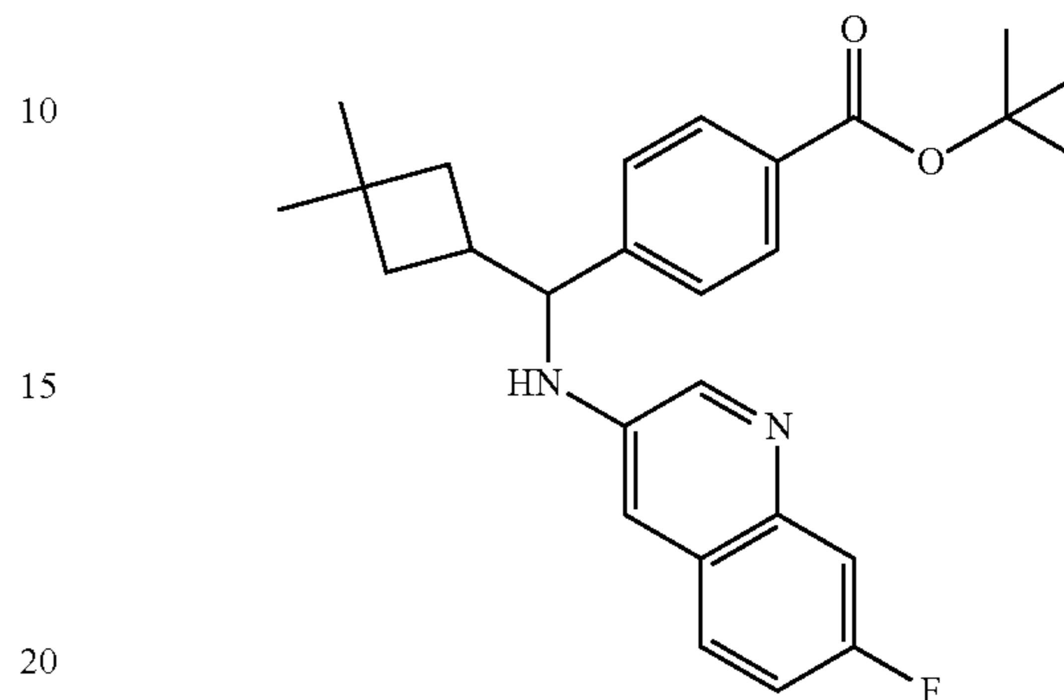
tert-butyl 4-((3,3-dimethylcyclobutyl)(7-fluoroquinolin-3-ylamino)methyl)benzoate
