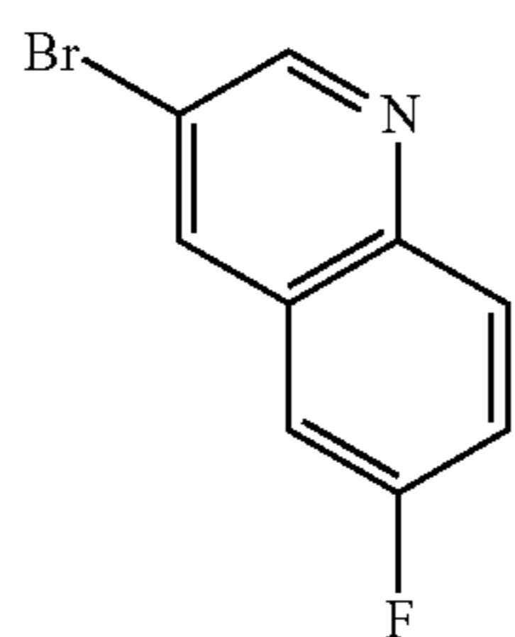
3-bromo-6-fluoroquinoline
