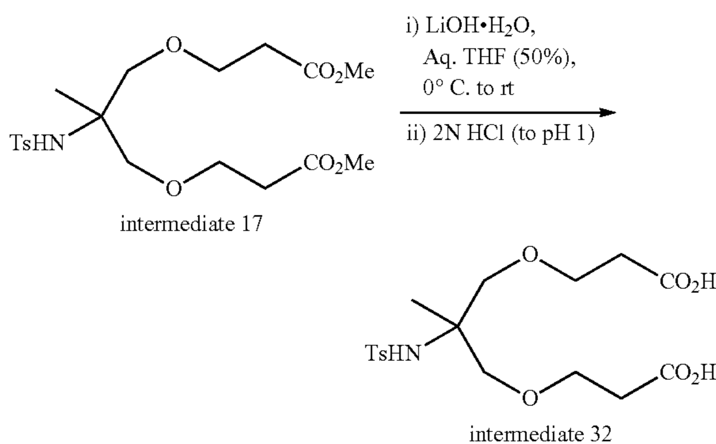
Scheme 35
