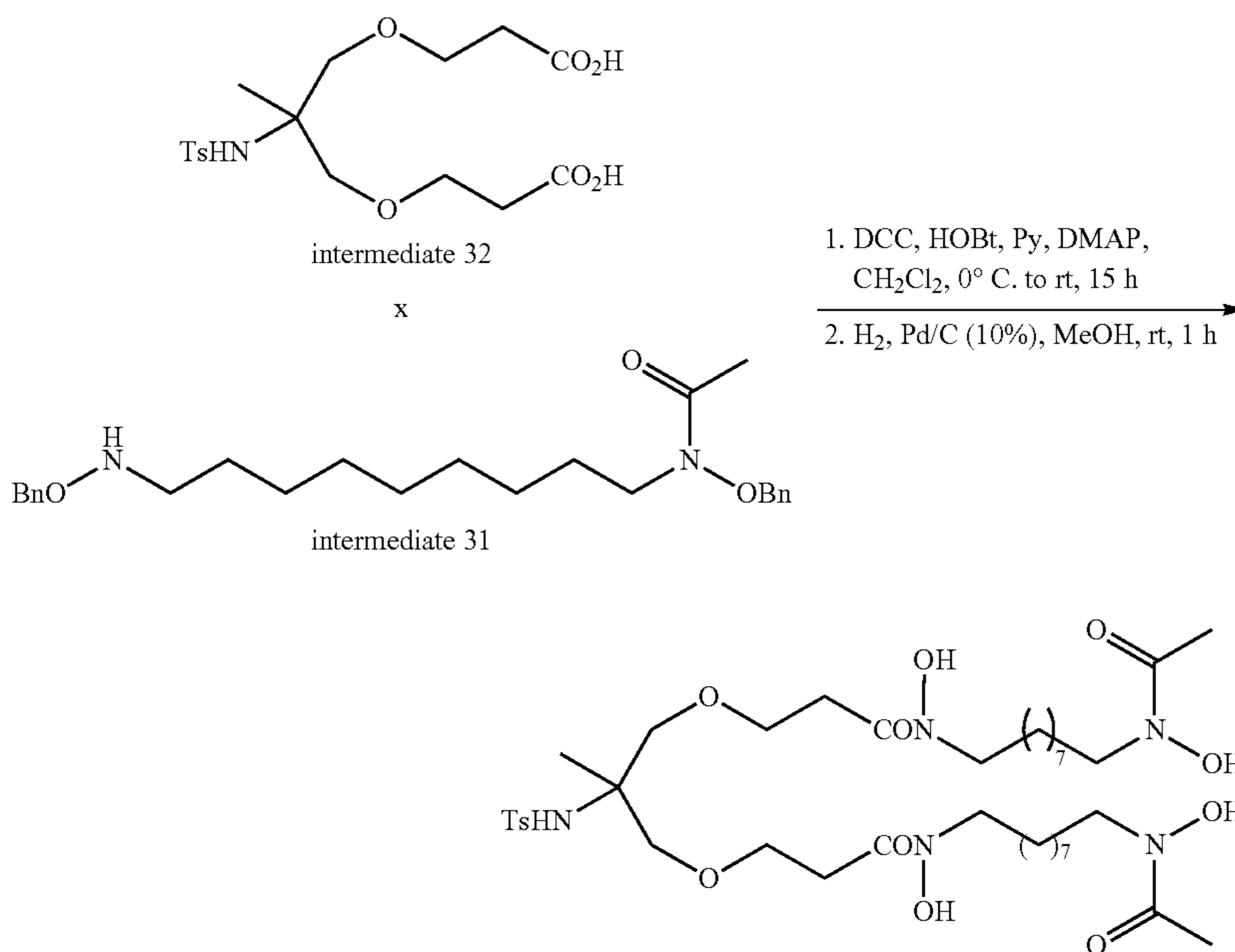
Scheme 36
