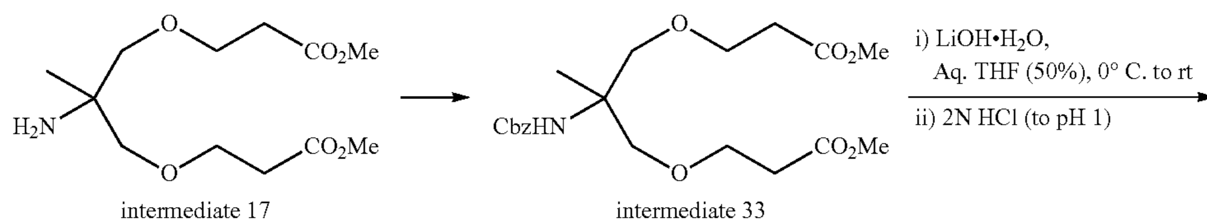
Scheme 37
