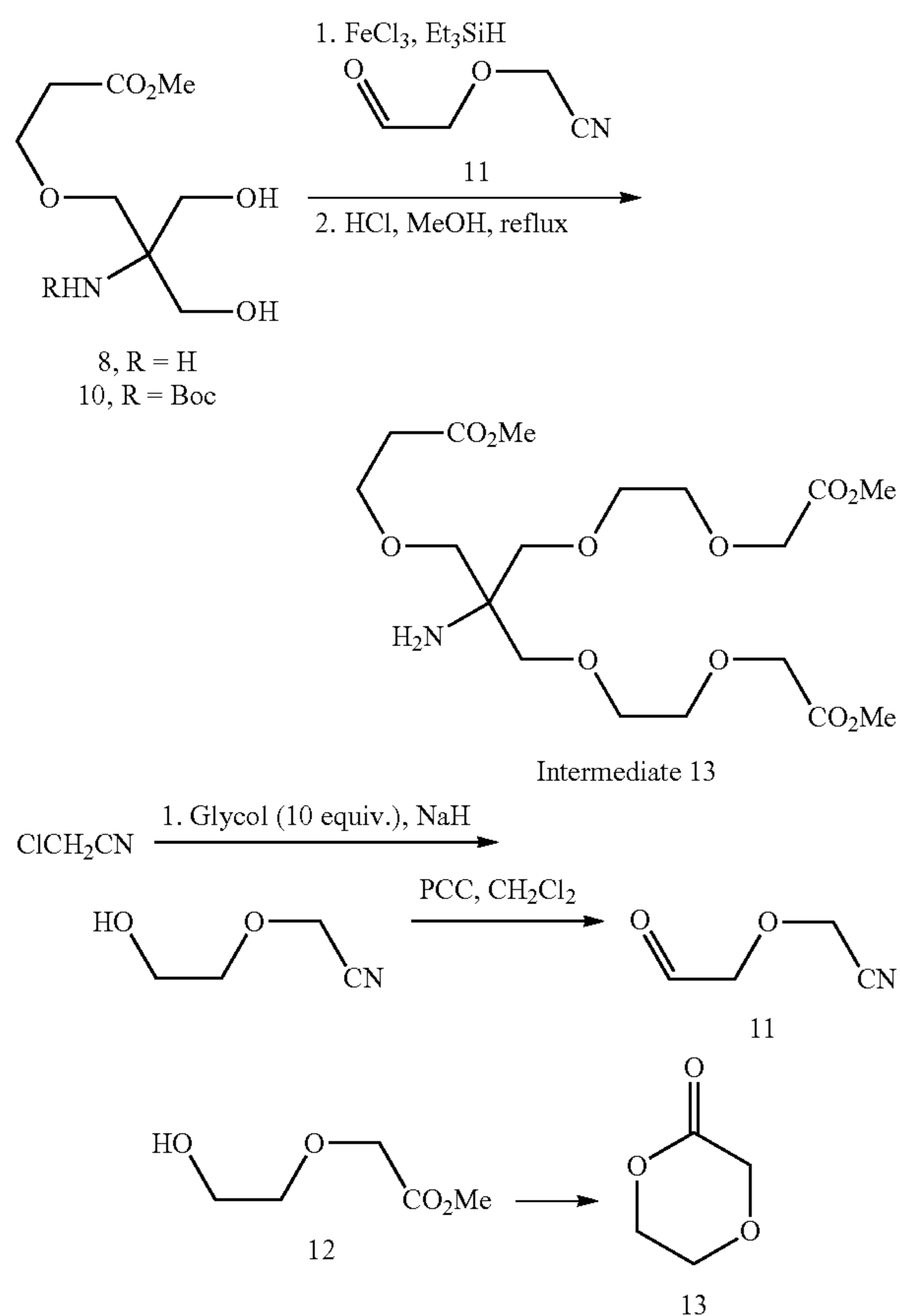
Scheme 10
