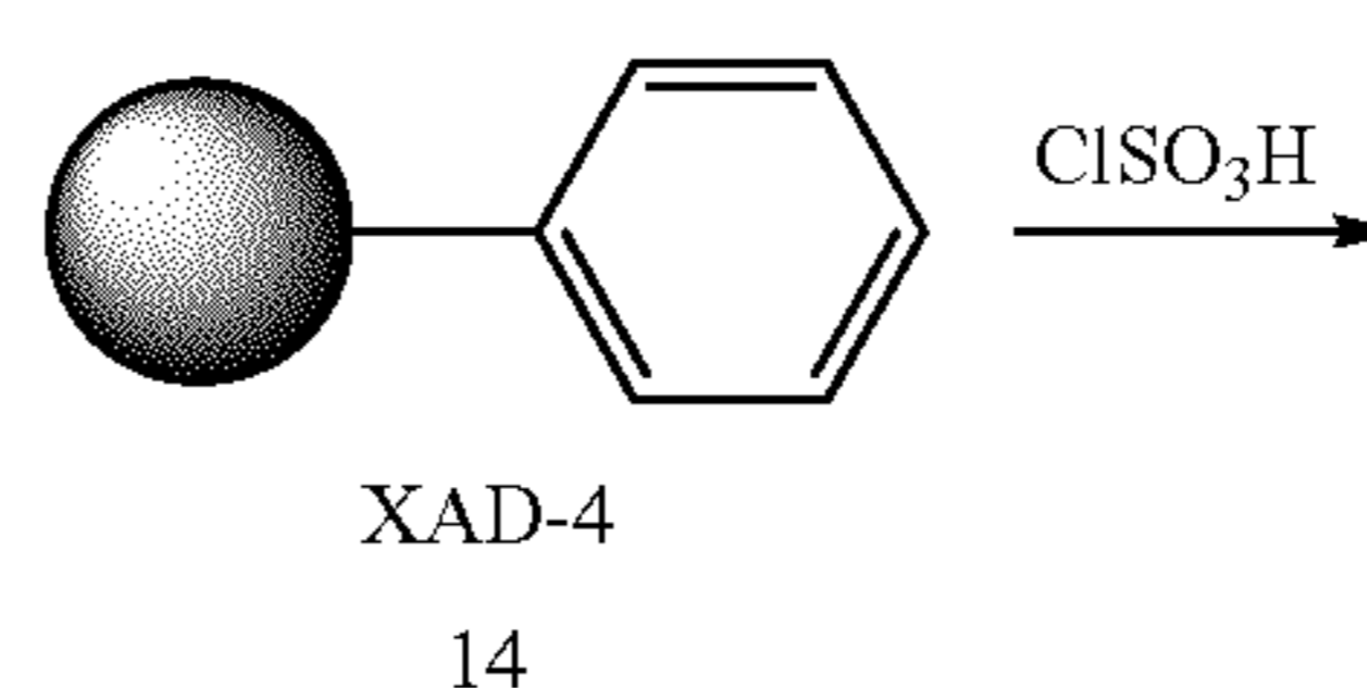
Scheme 12
