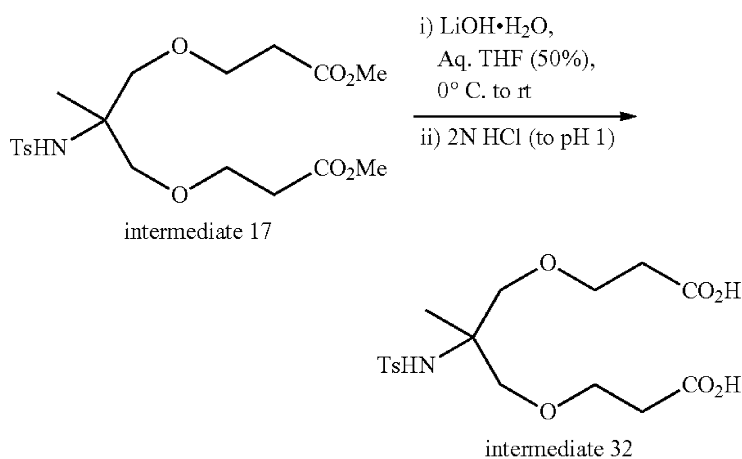
Scheme 35
