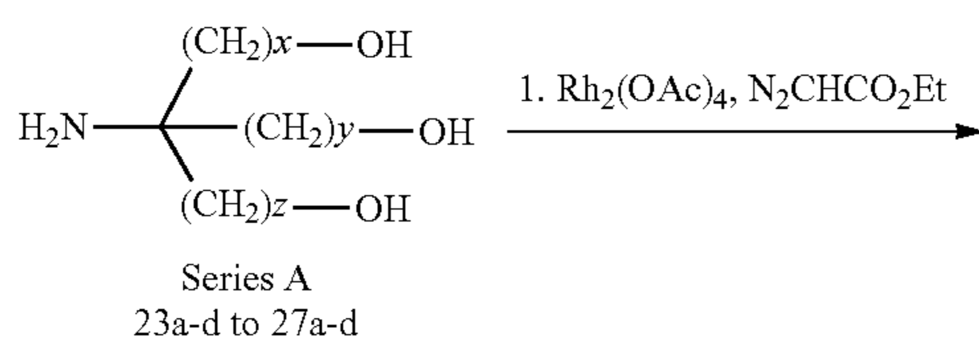
Scheme 26
