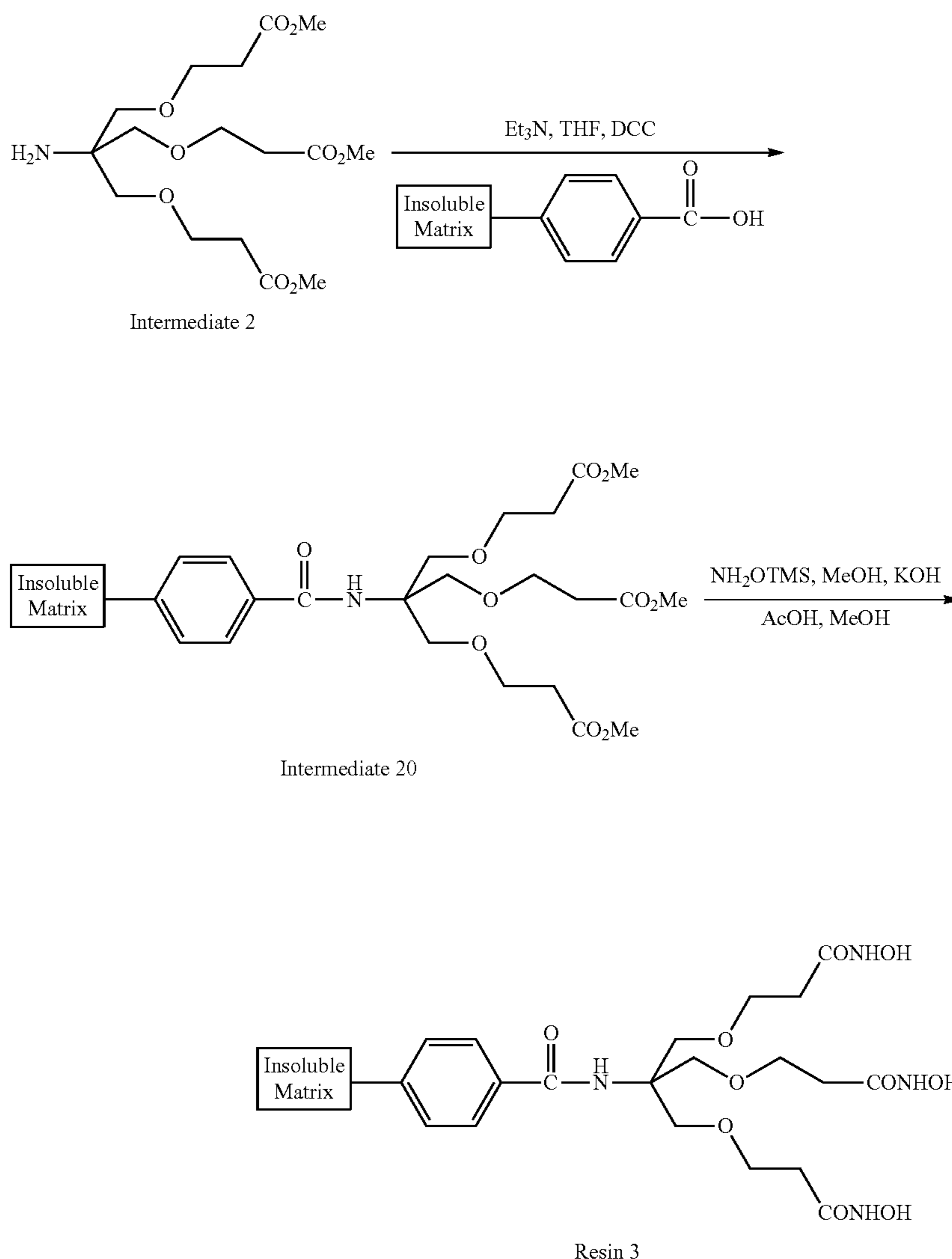
Scheme 14
