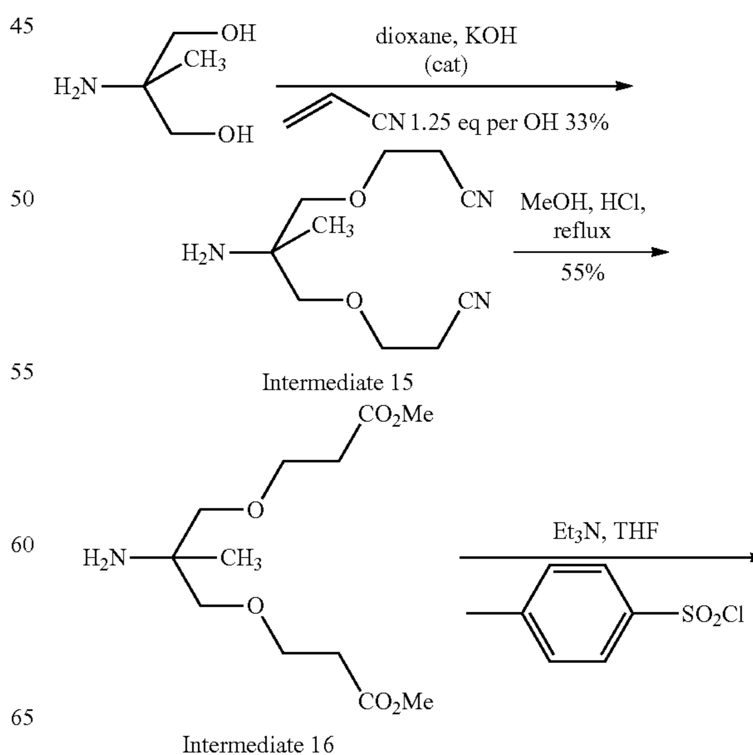
Scheme 11
