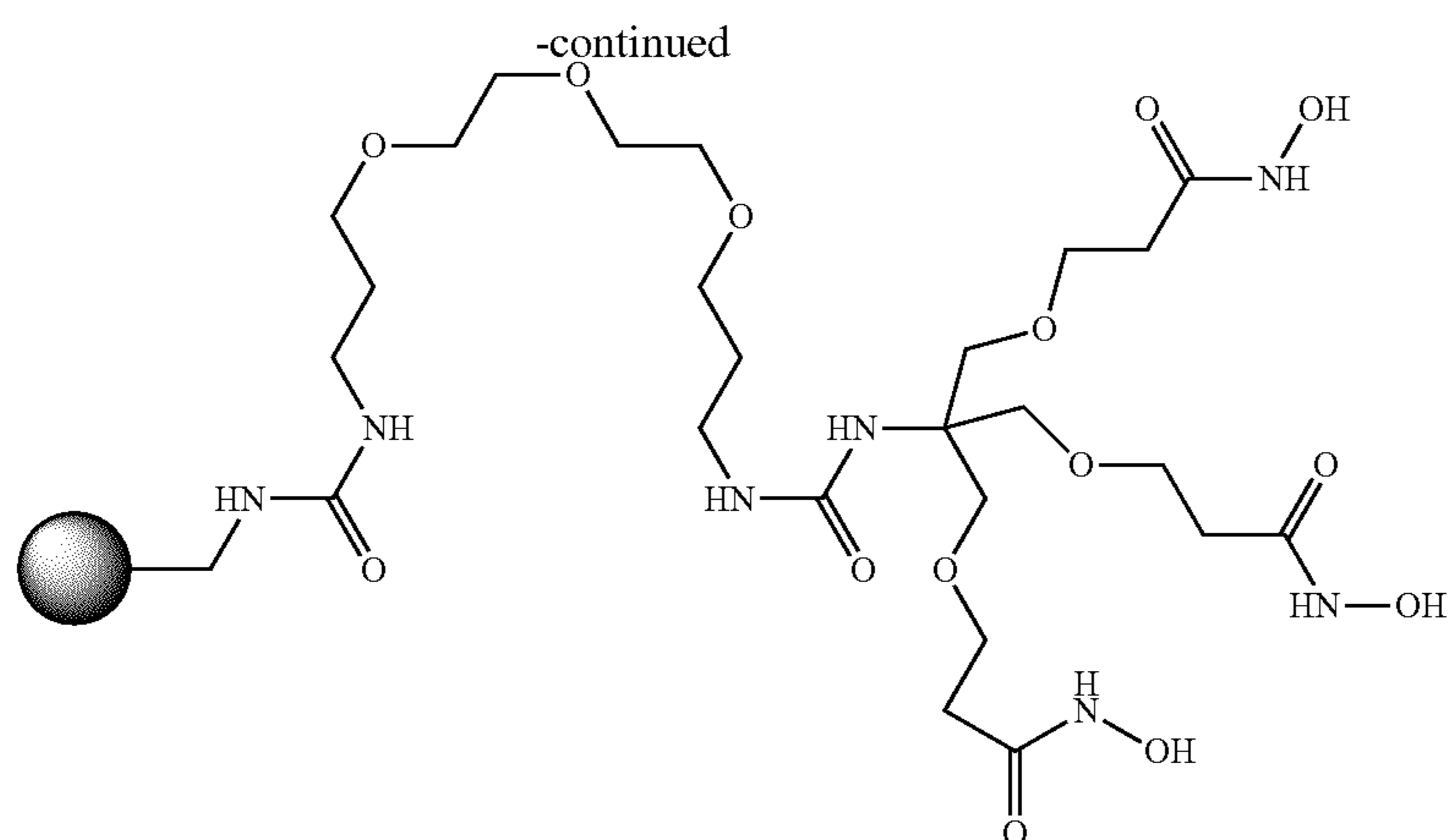
Resin 7 (0.70 meq/g)
