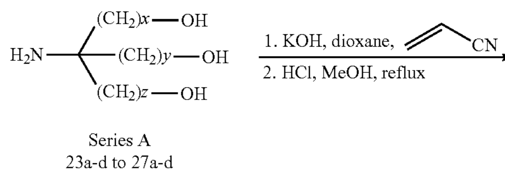
Scheme 25
