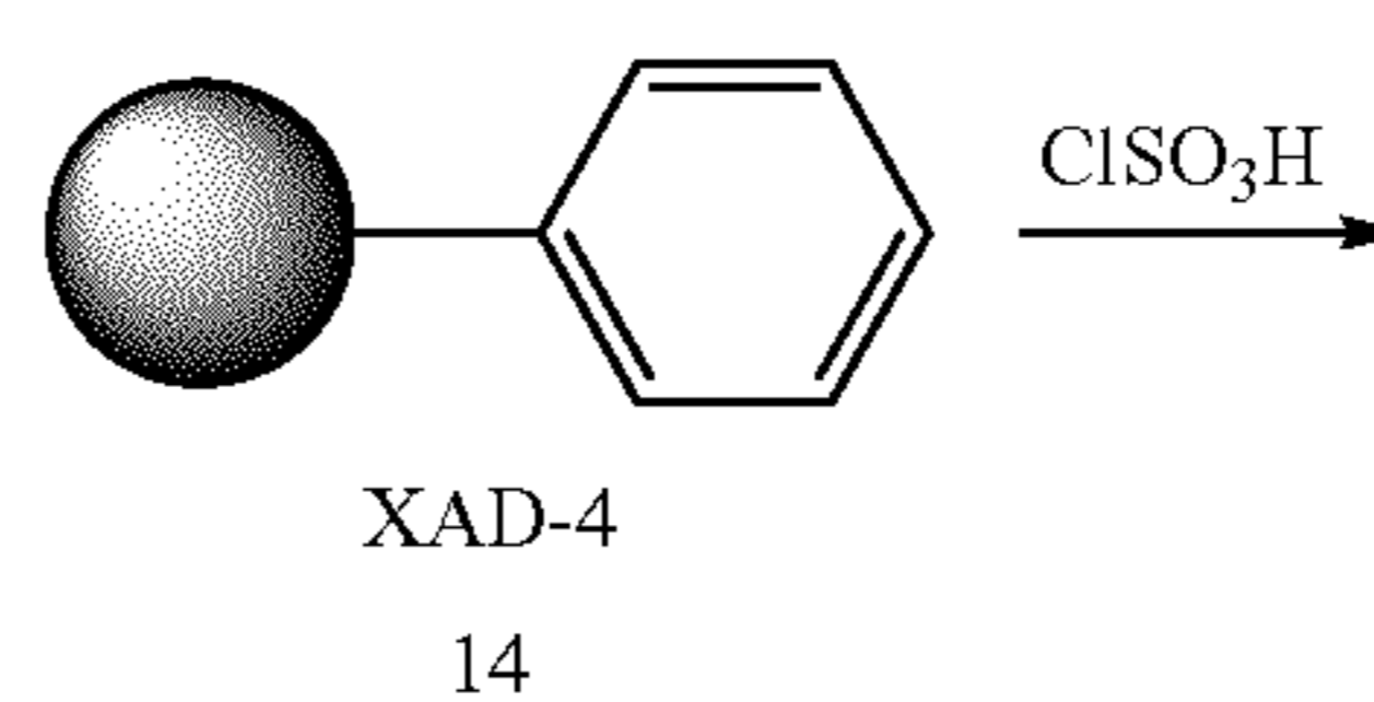
Scheme 12
