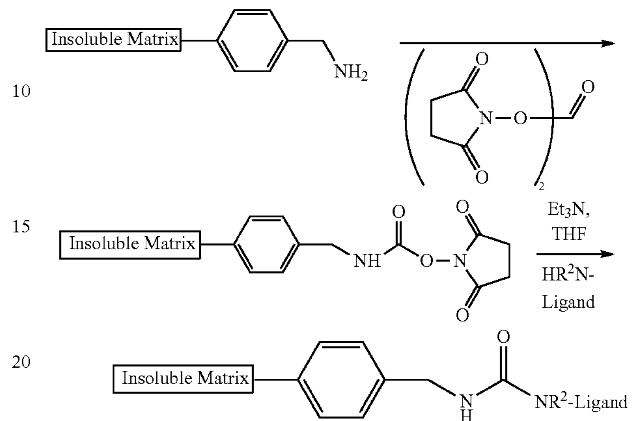
Scheme 3
