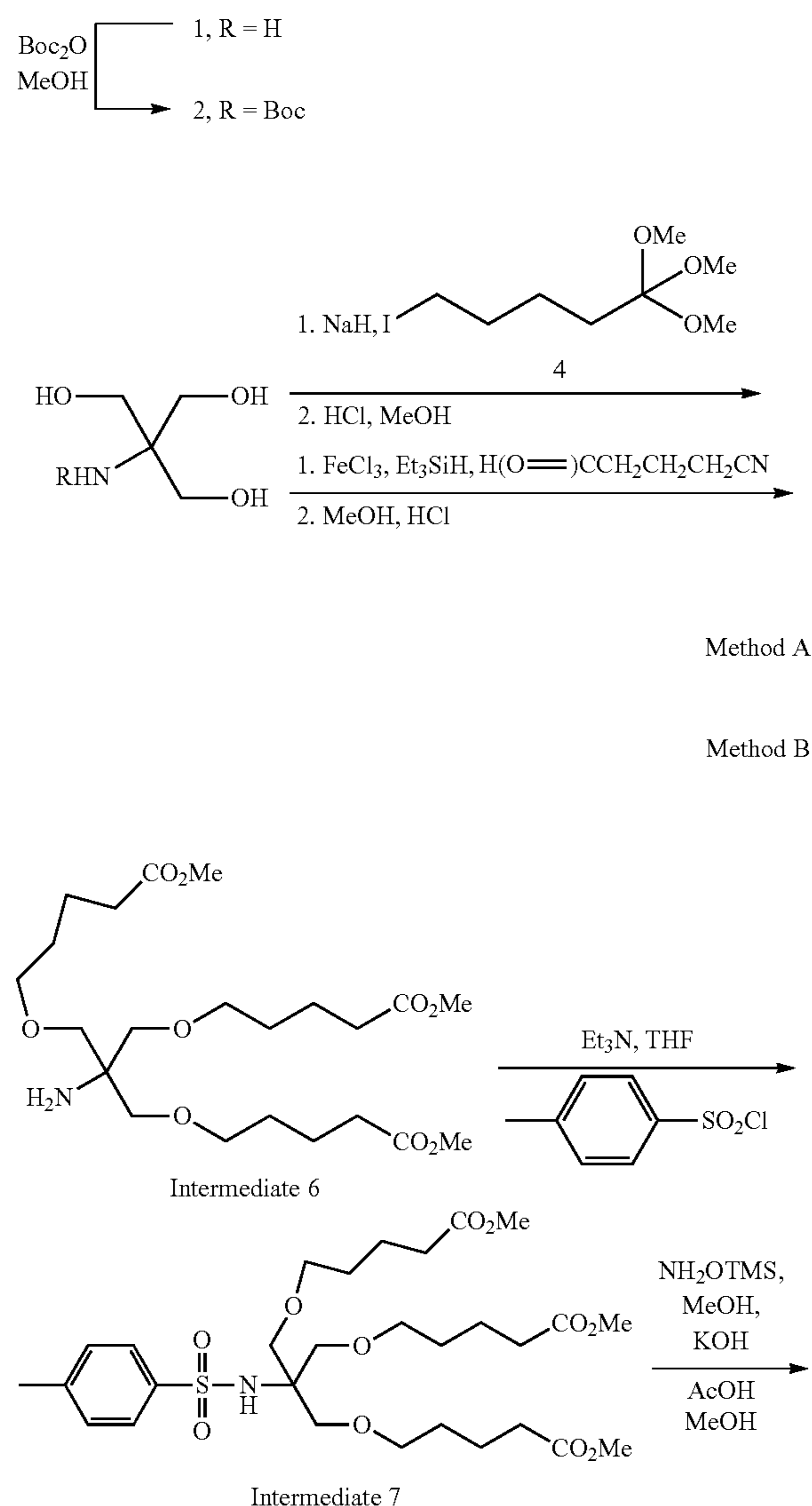
Scheme 7
