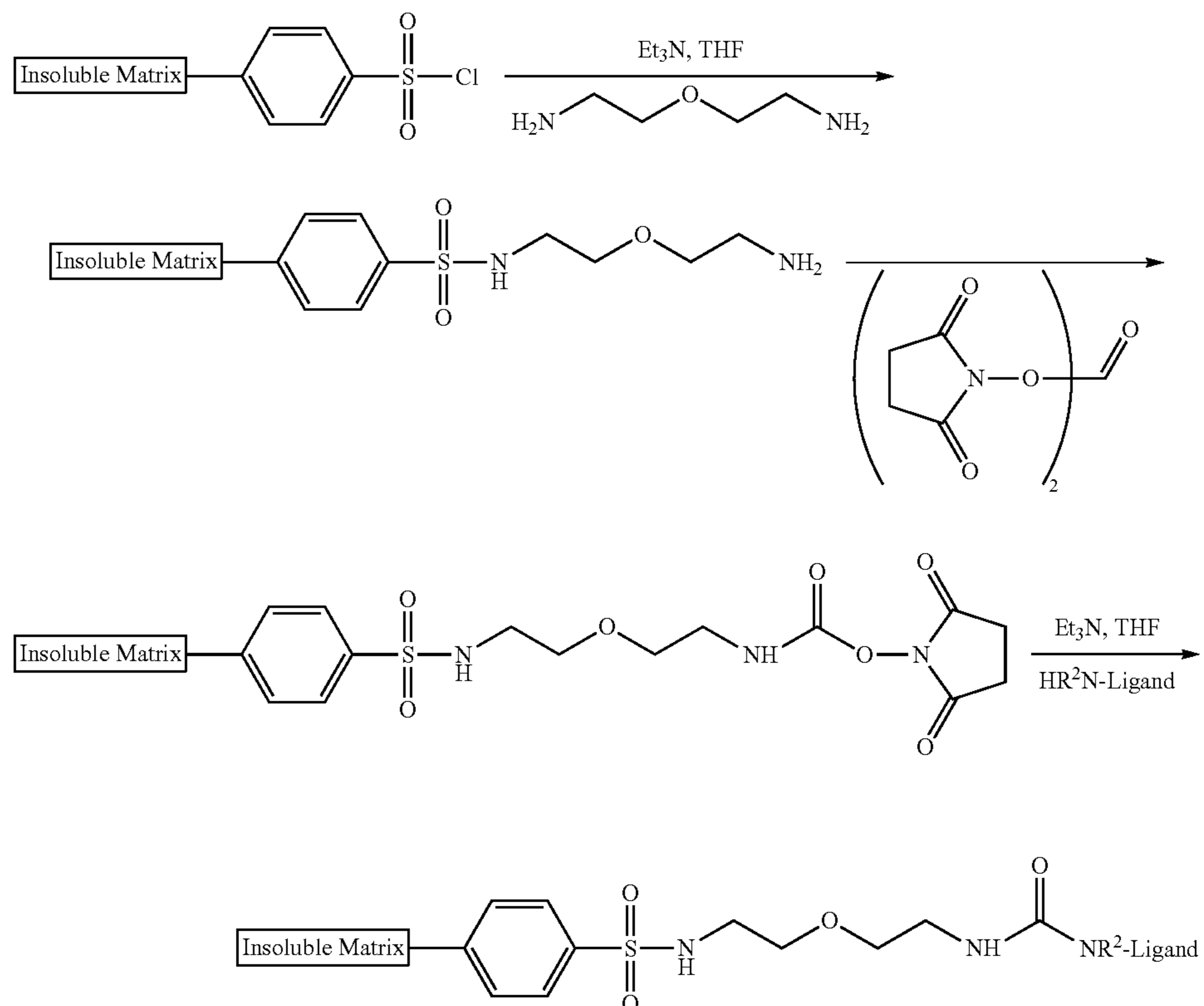
Scheme 4
