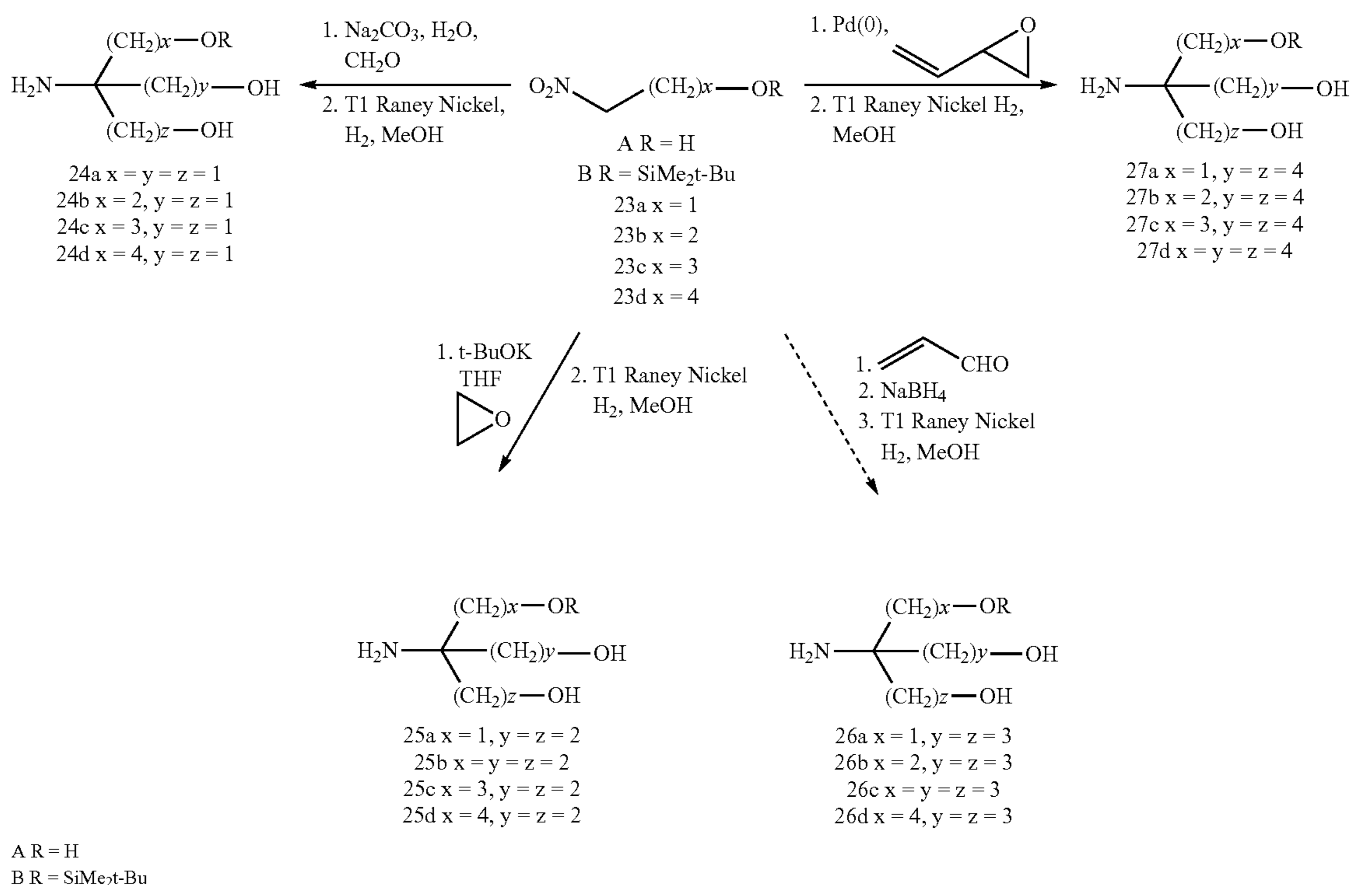
Scheme 24
