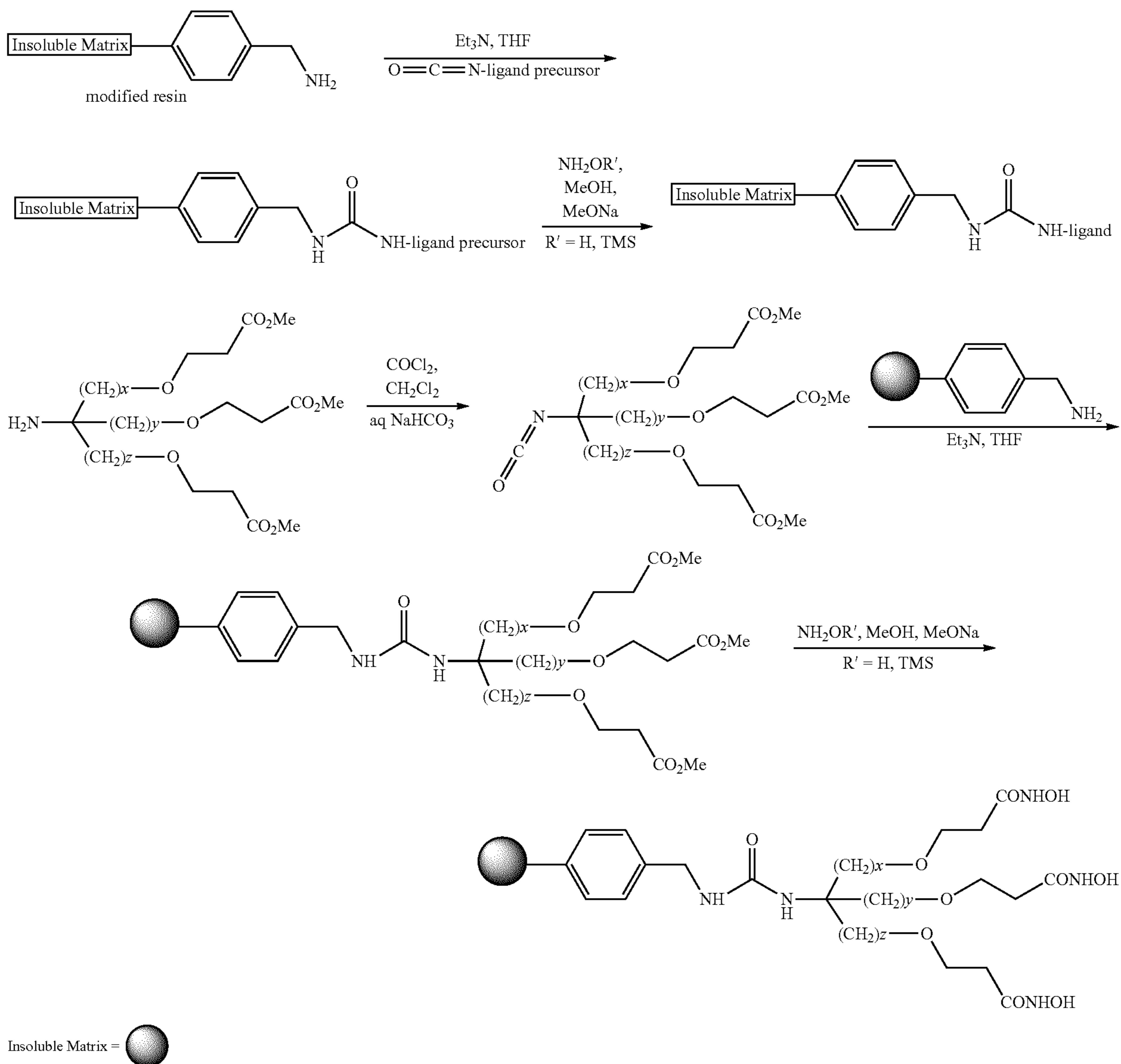
Scheme 19
