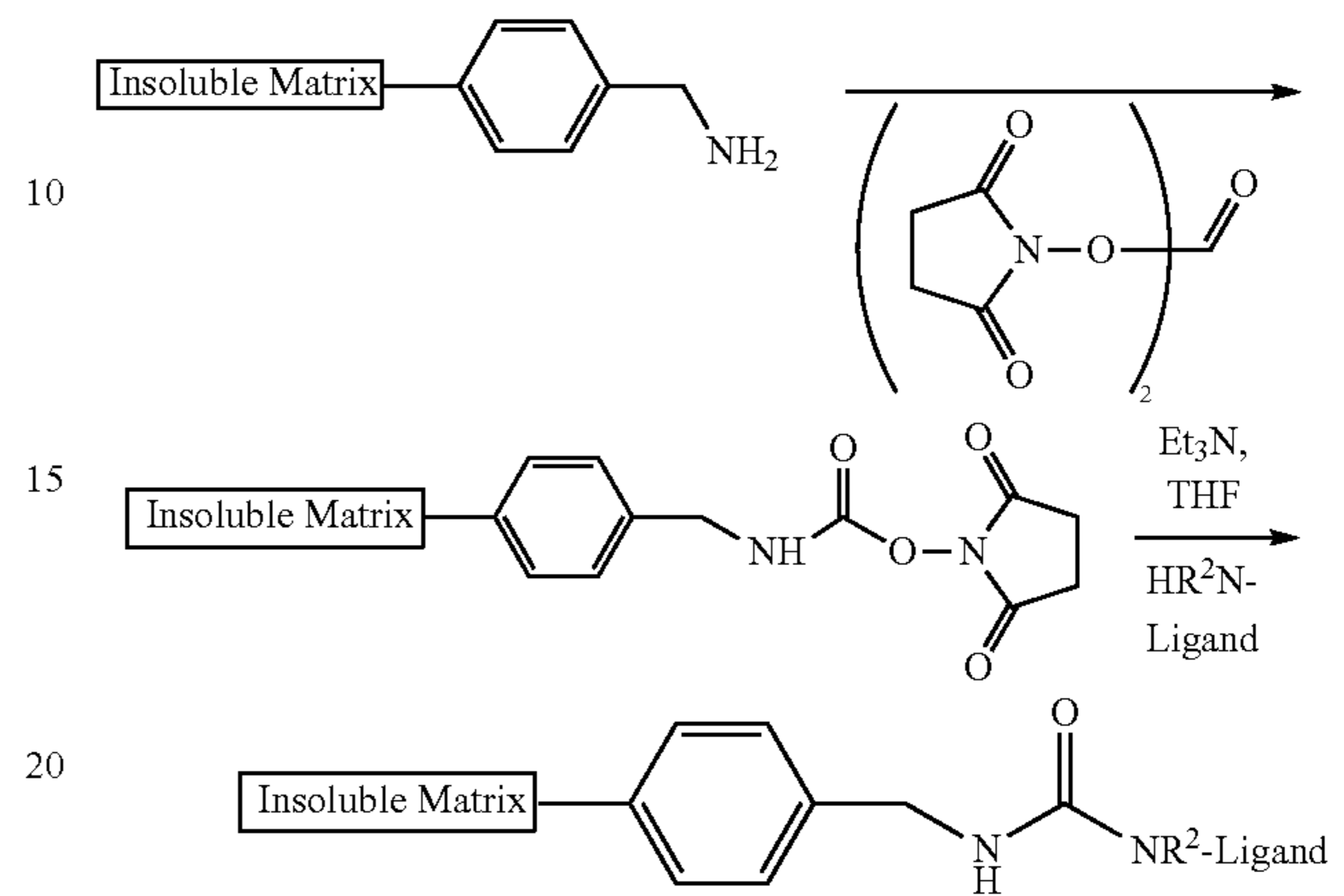
Scheme 3
