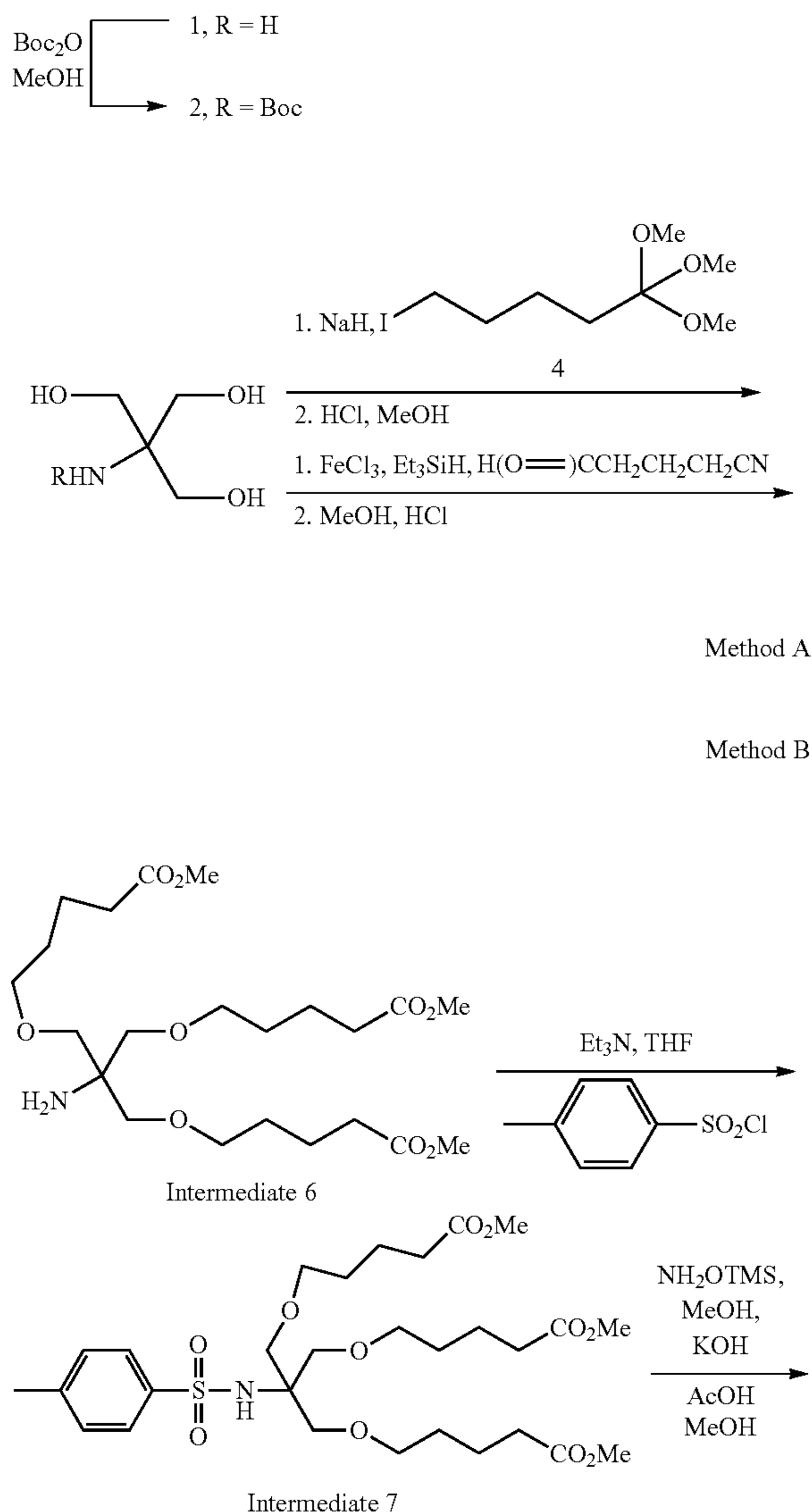
Scheme 7
