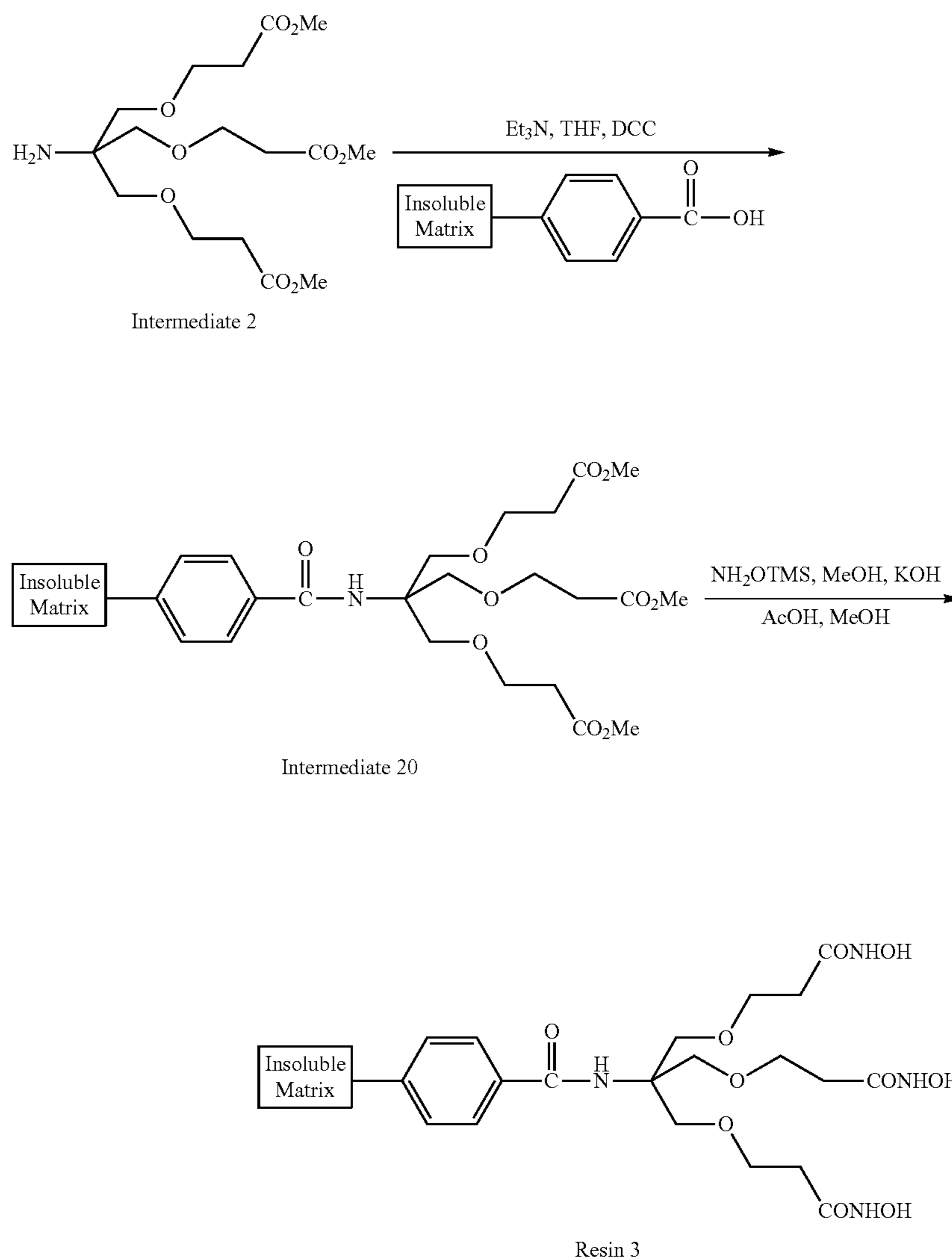
Scheme 14
