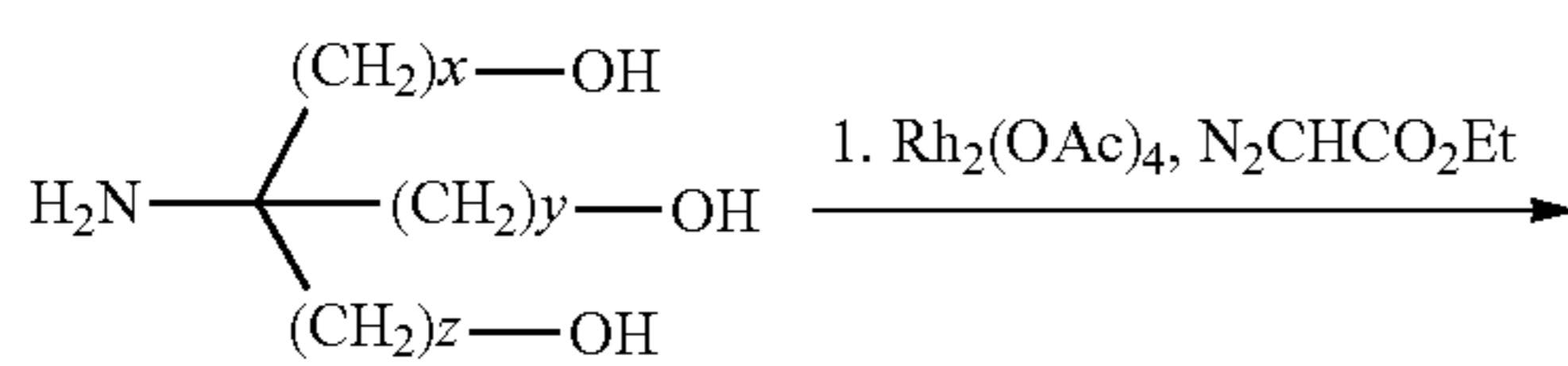
Scheme 26
