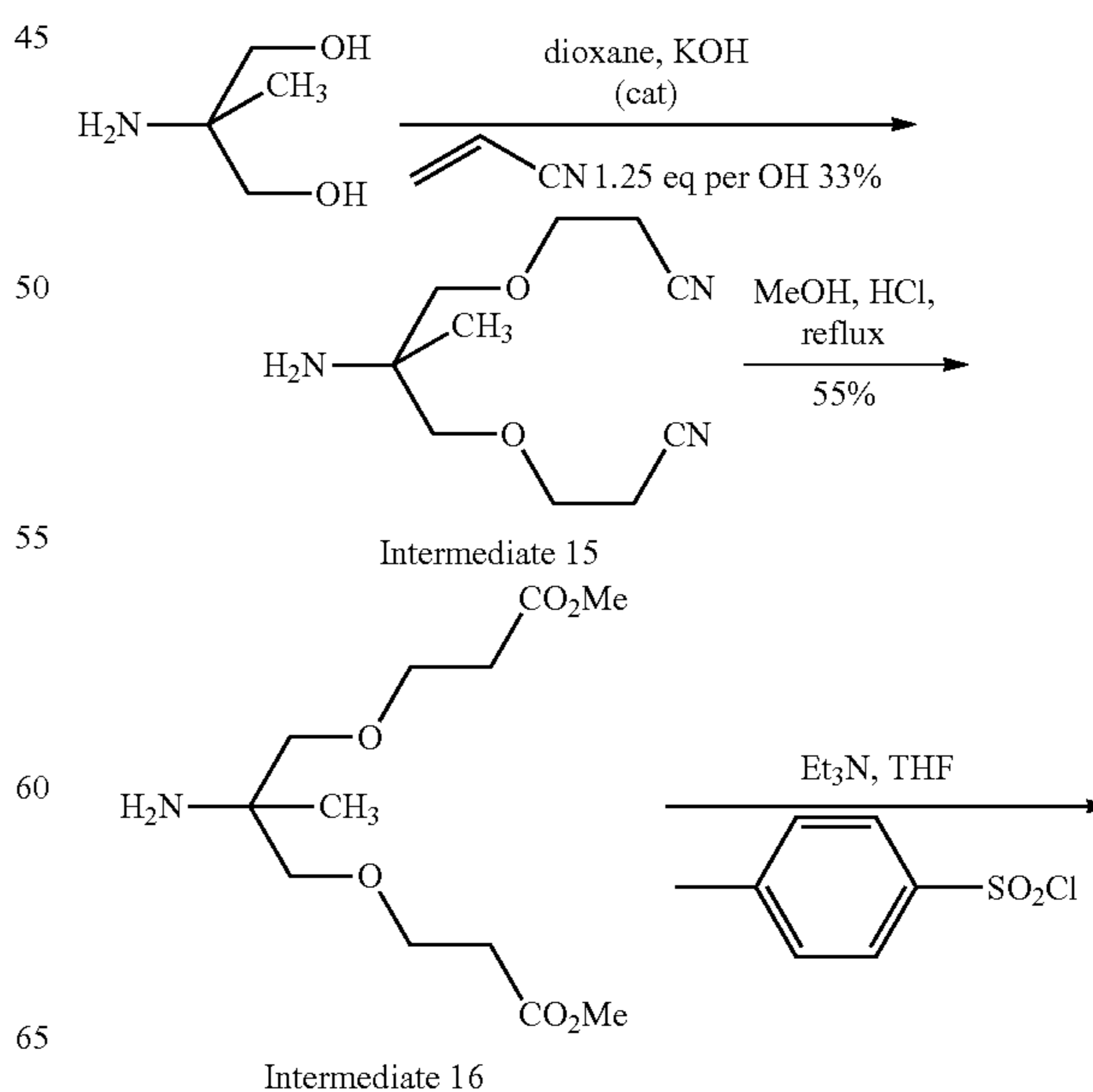
Scheme 11
