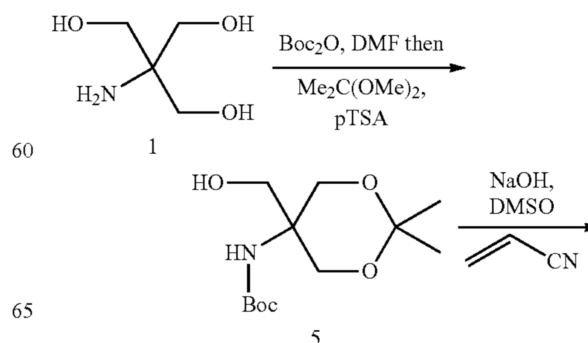
Scheme 8
