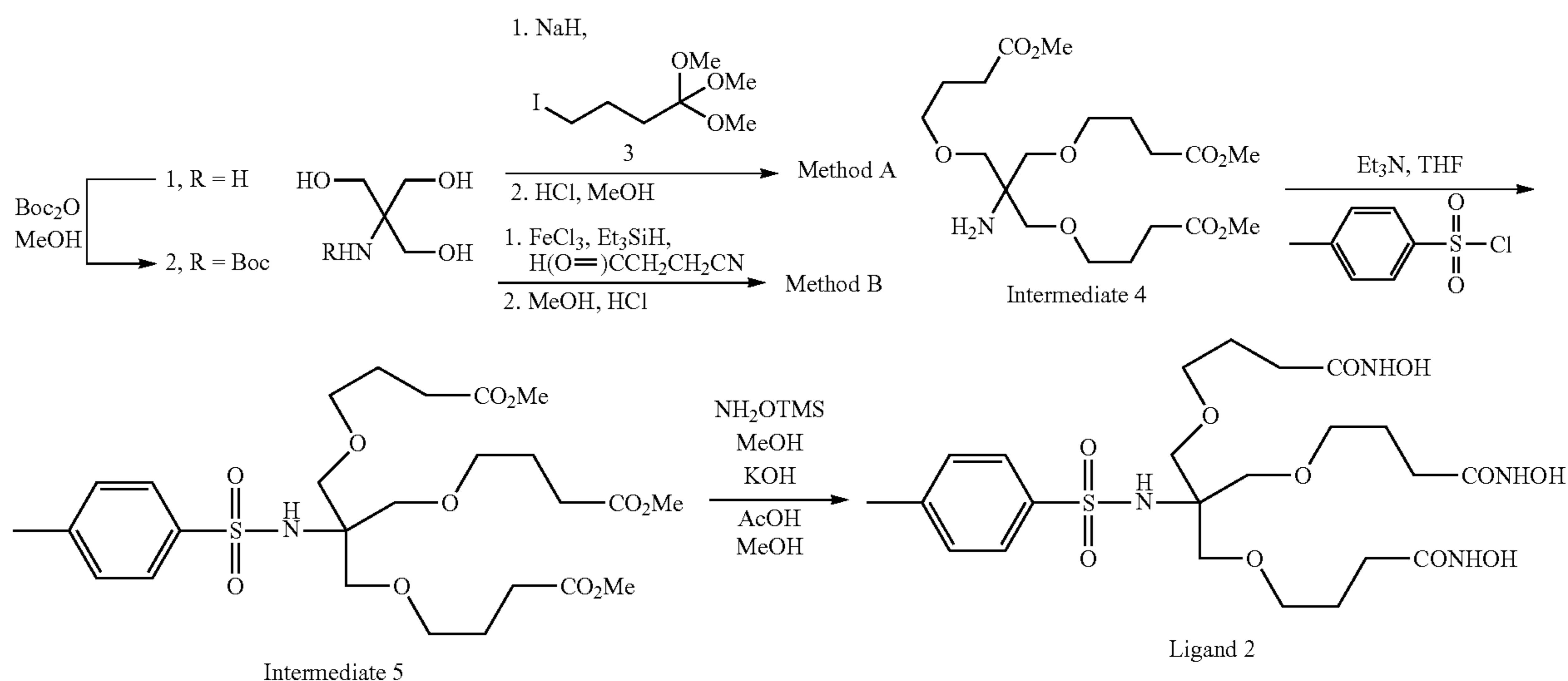
Scheme 6
