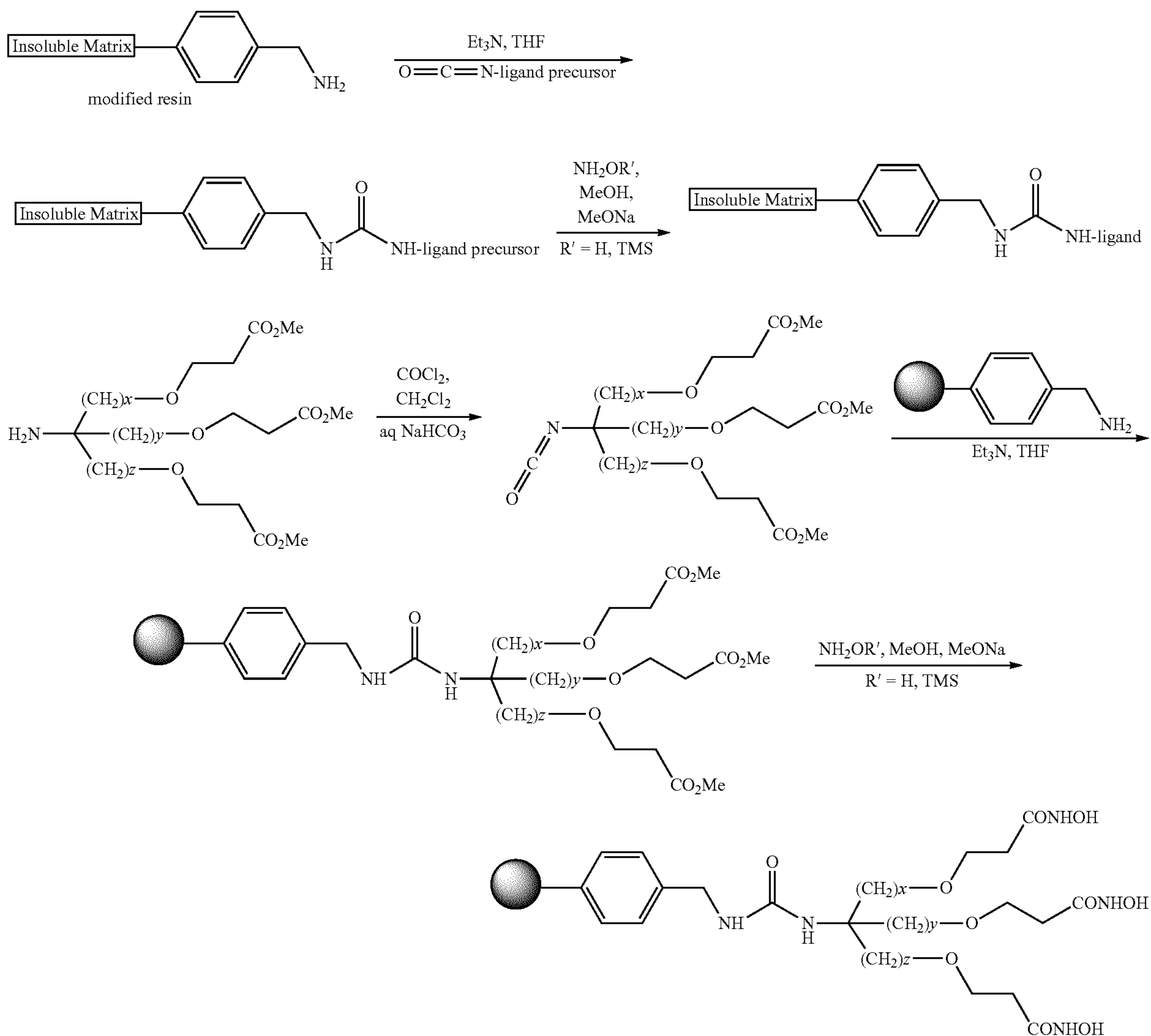
Scheme 19
