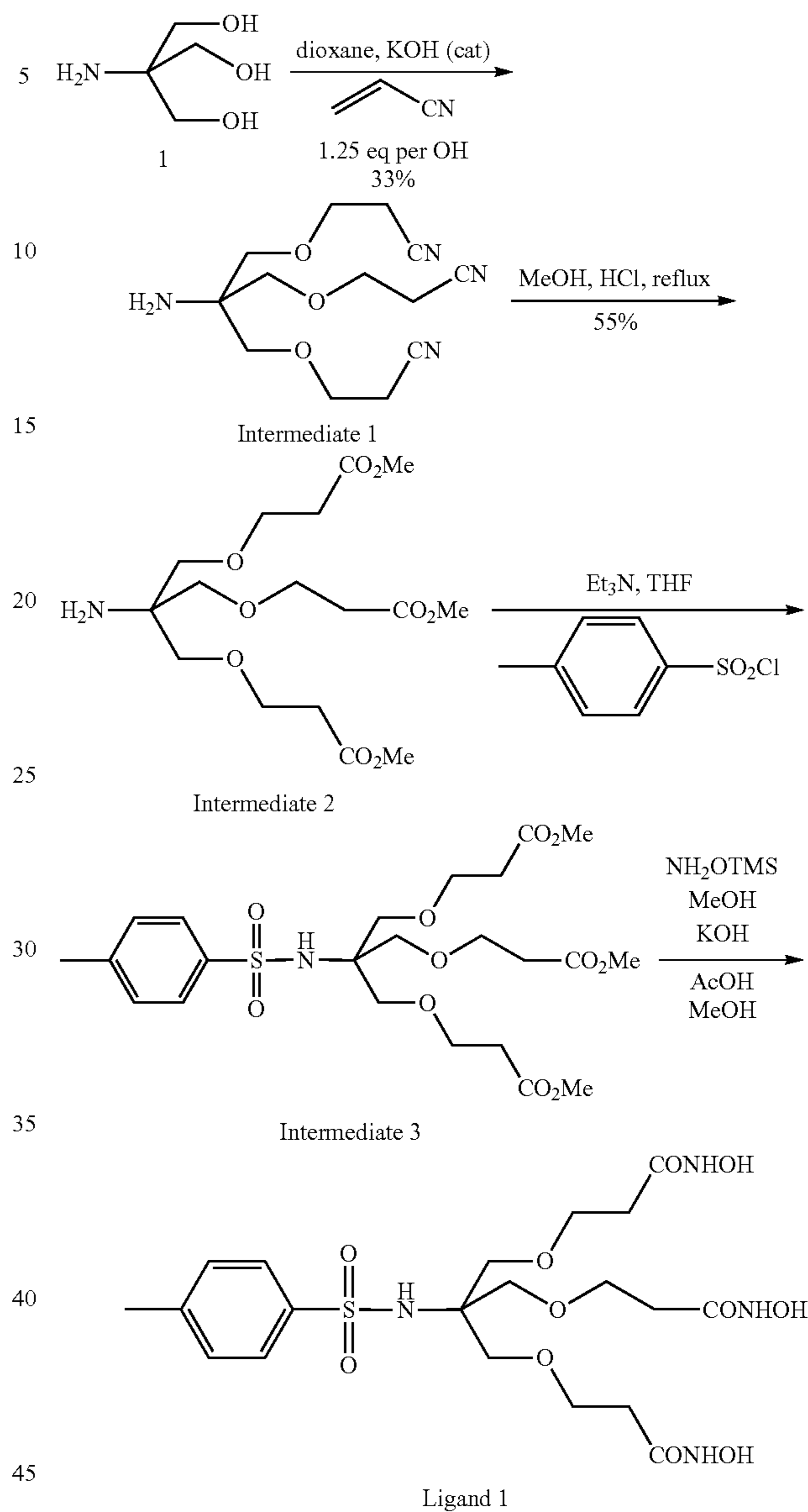
Scheme 5
