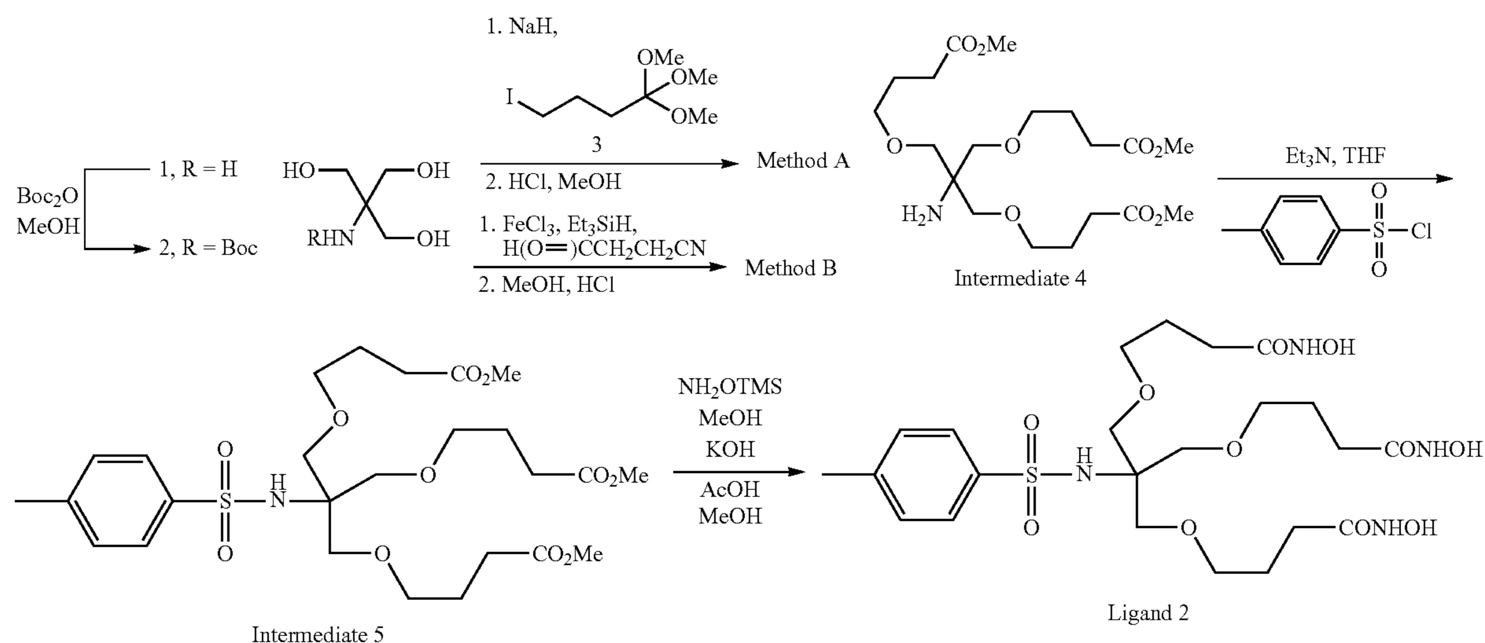
Scheme 6
