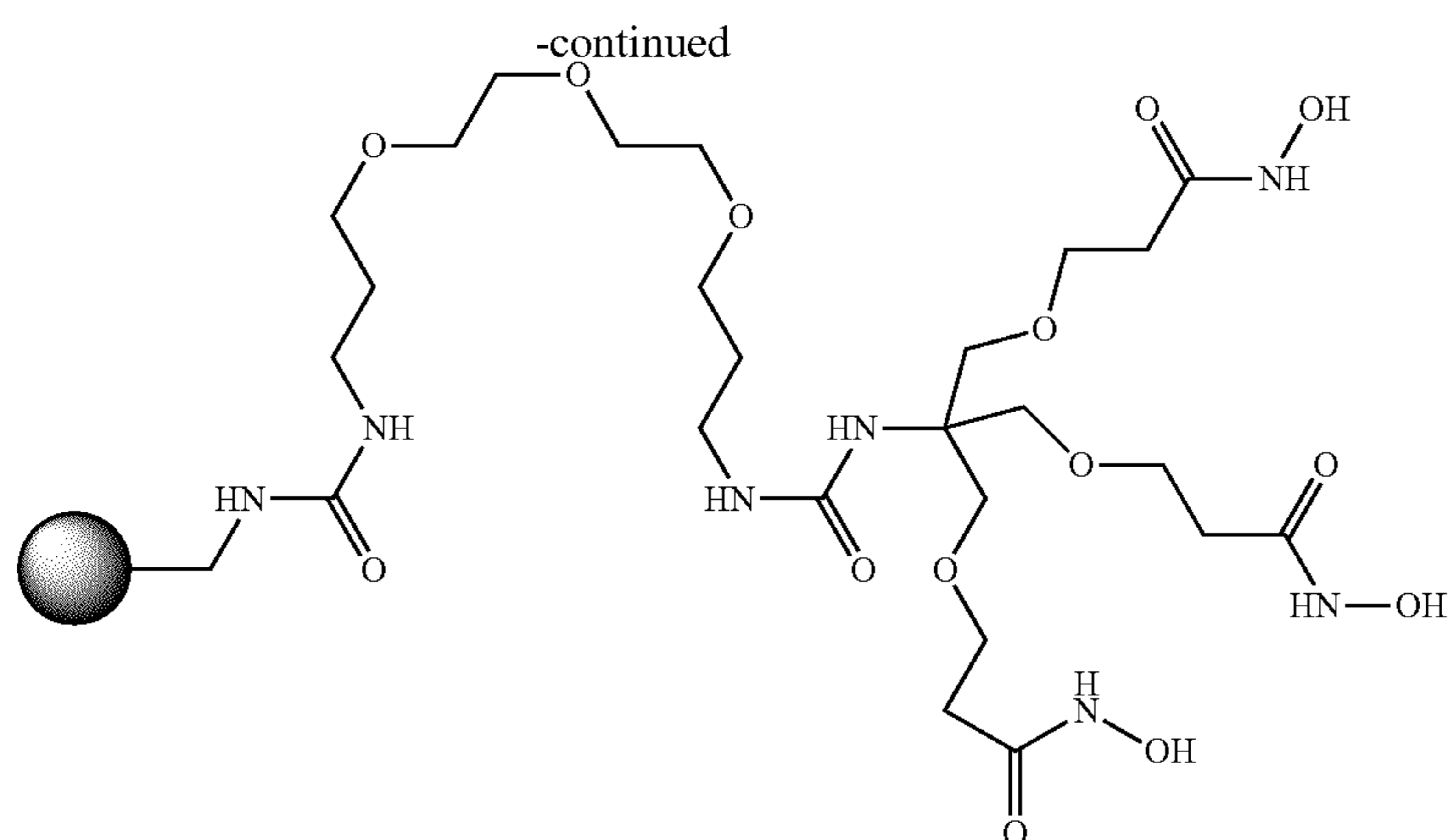
Resin 7 (0.70 meq/g)
