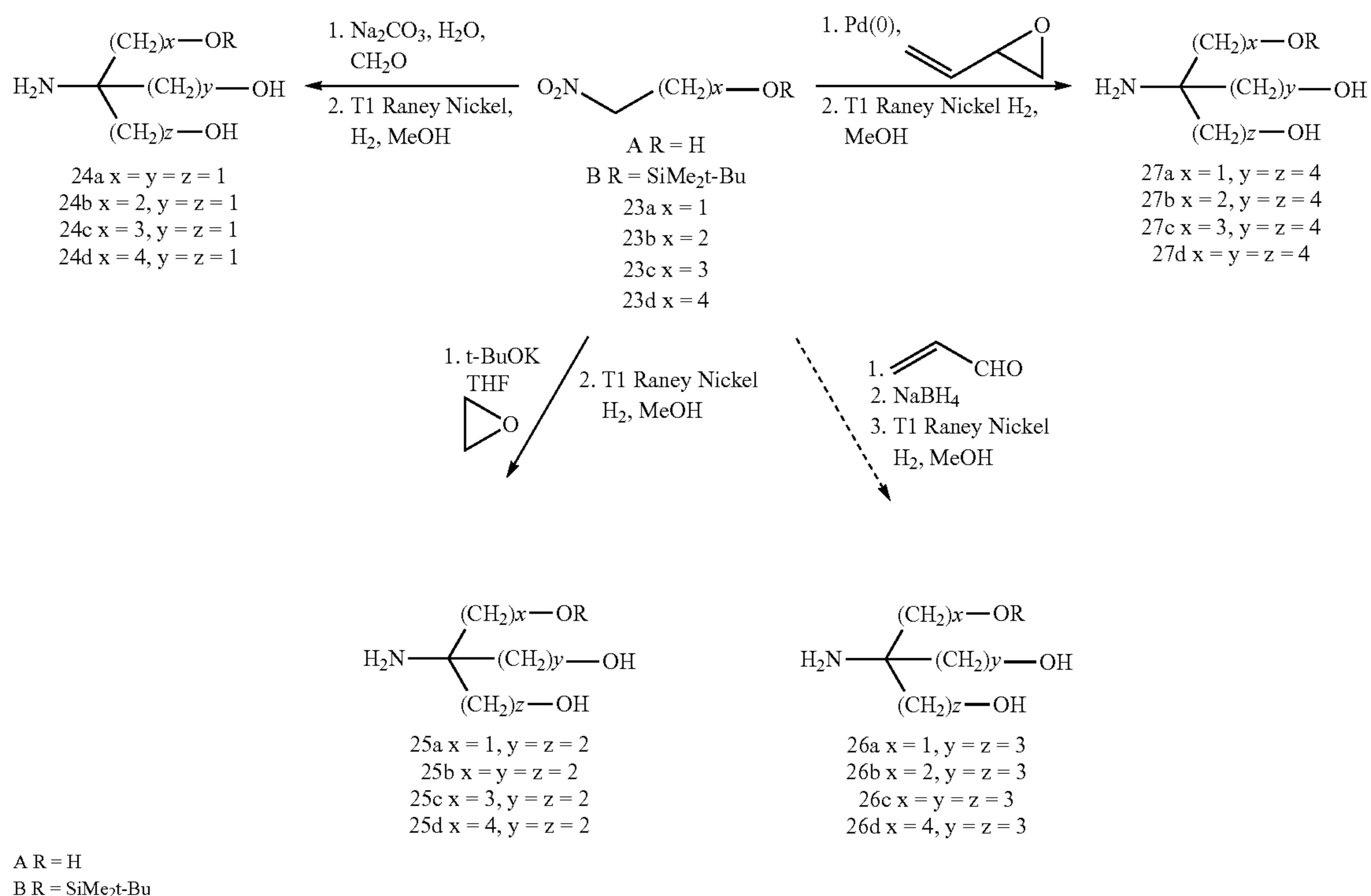
Scheme 24
