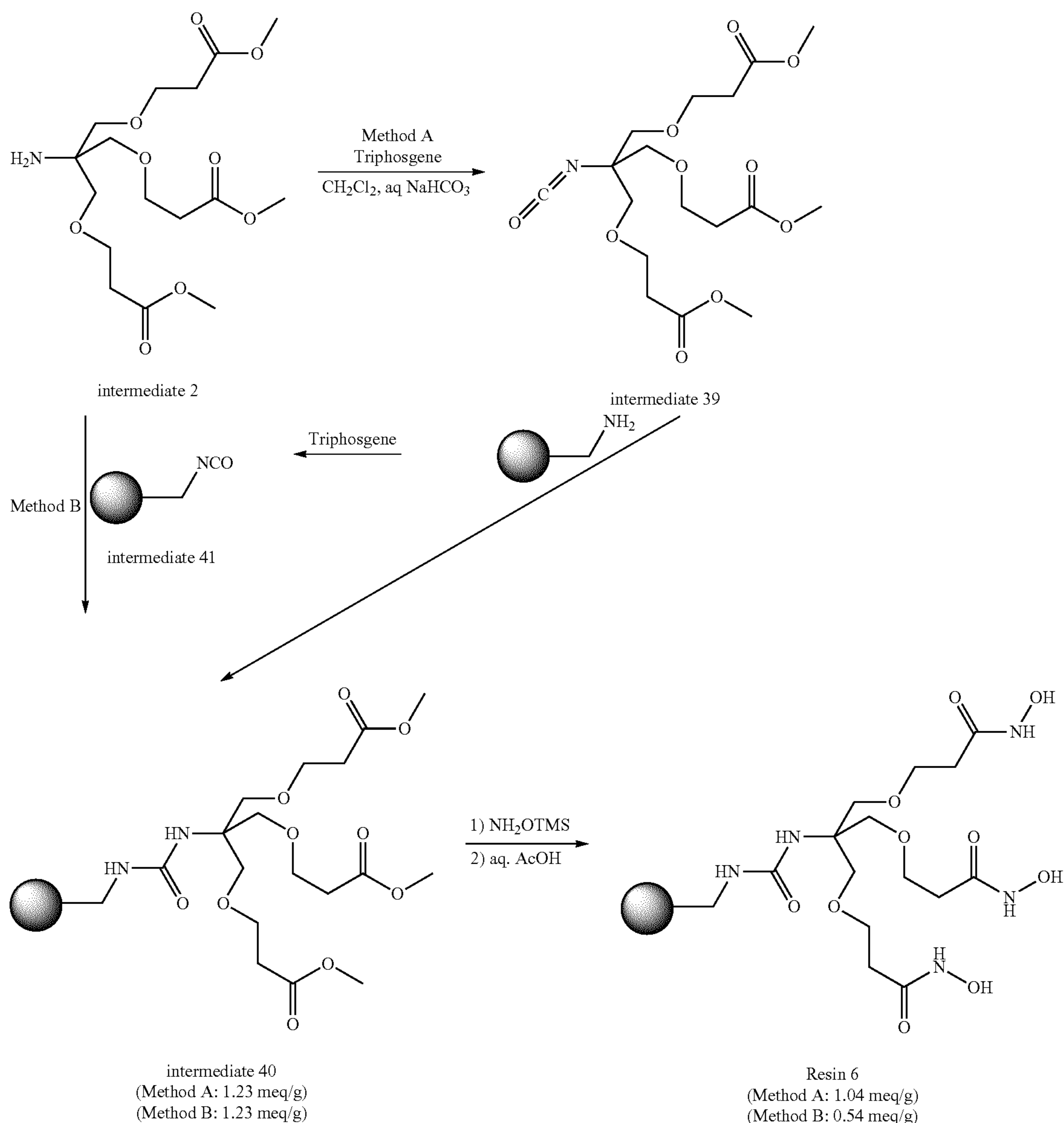
Scheme 42
