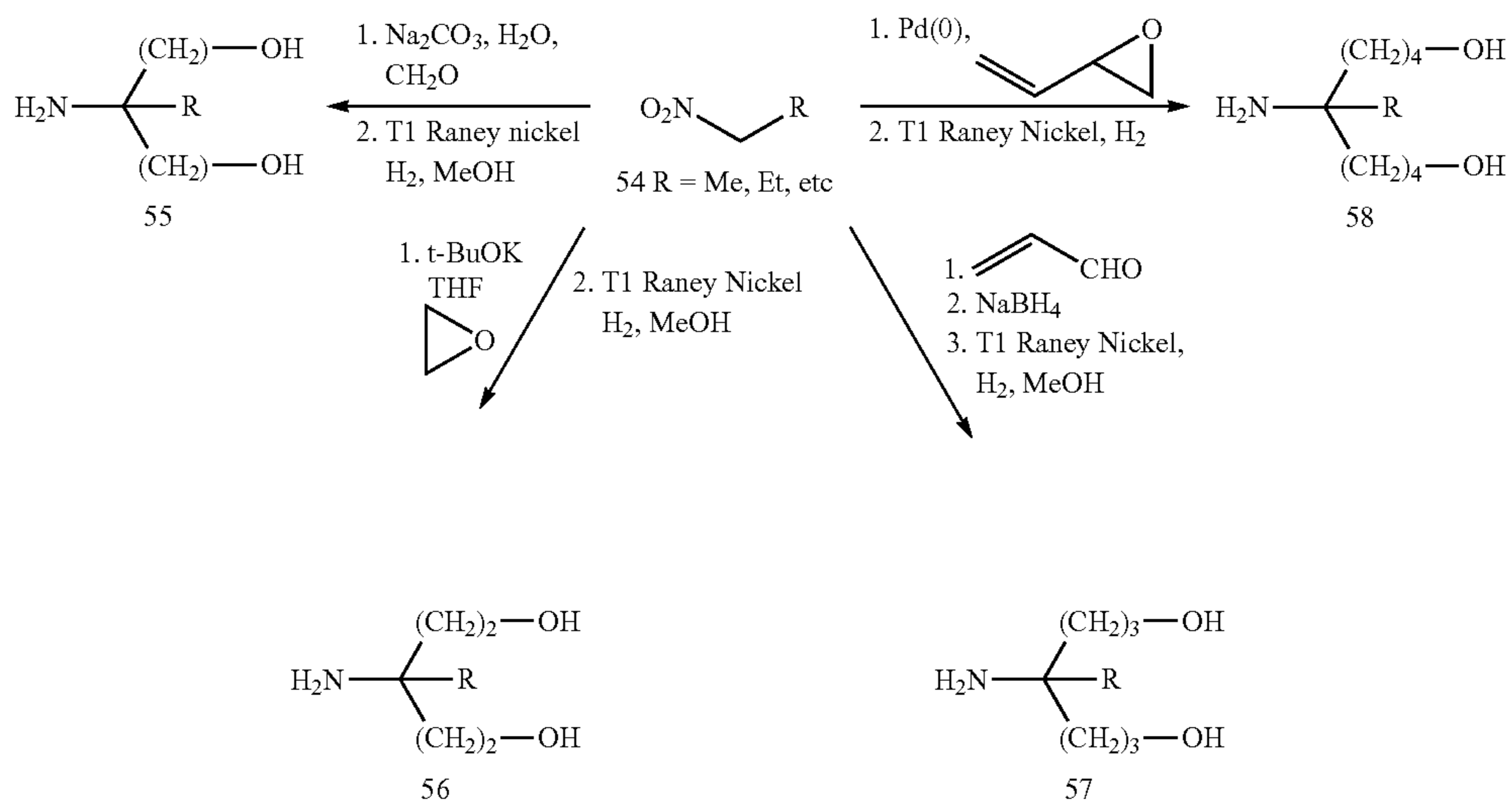
Scheme 30
