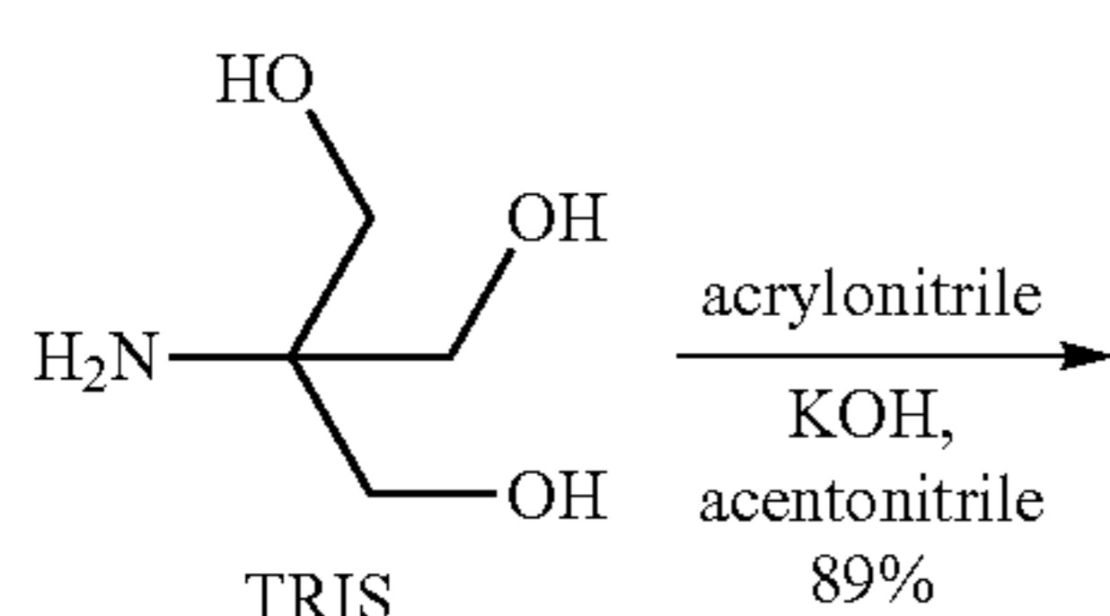
Scheme 45
