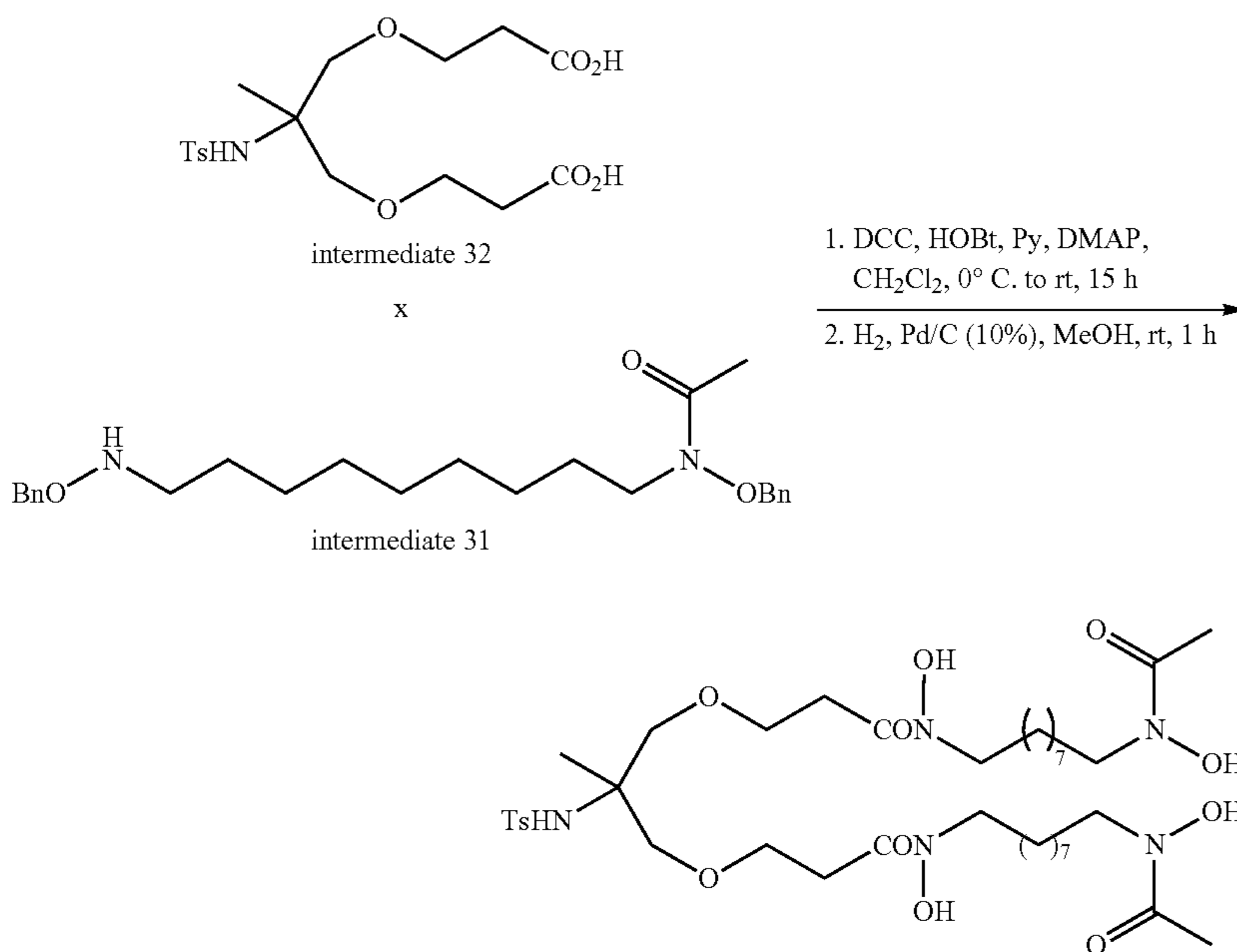
Scheme 36
