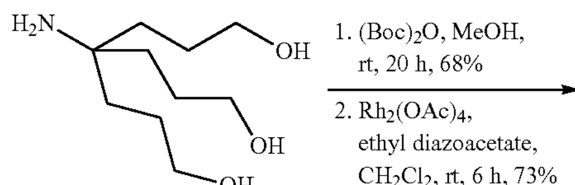
Scheme 27
