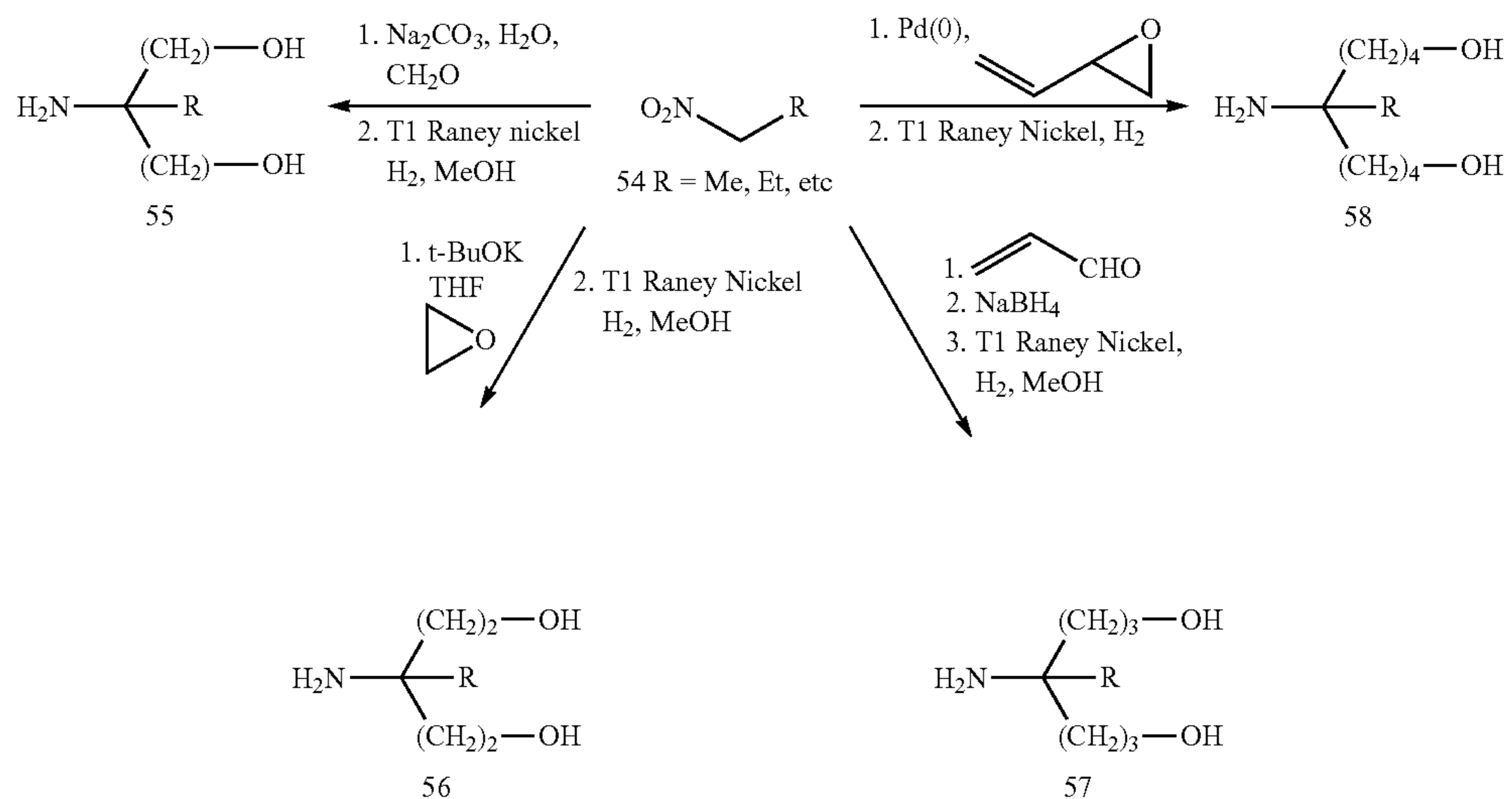
Scheme 30
