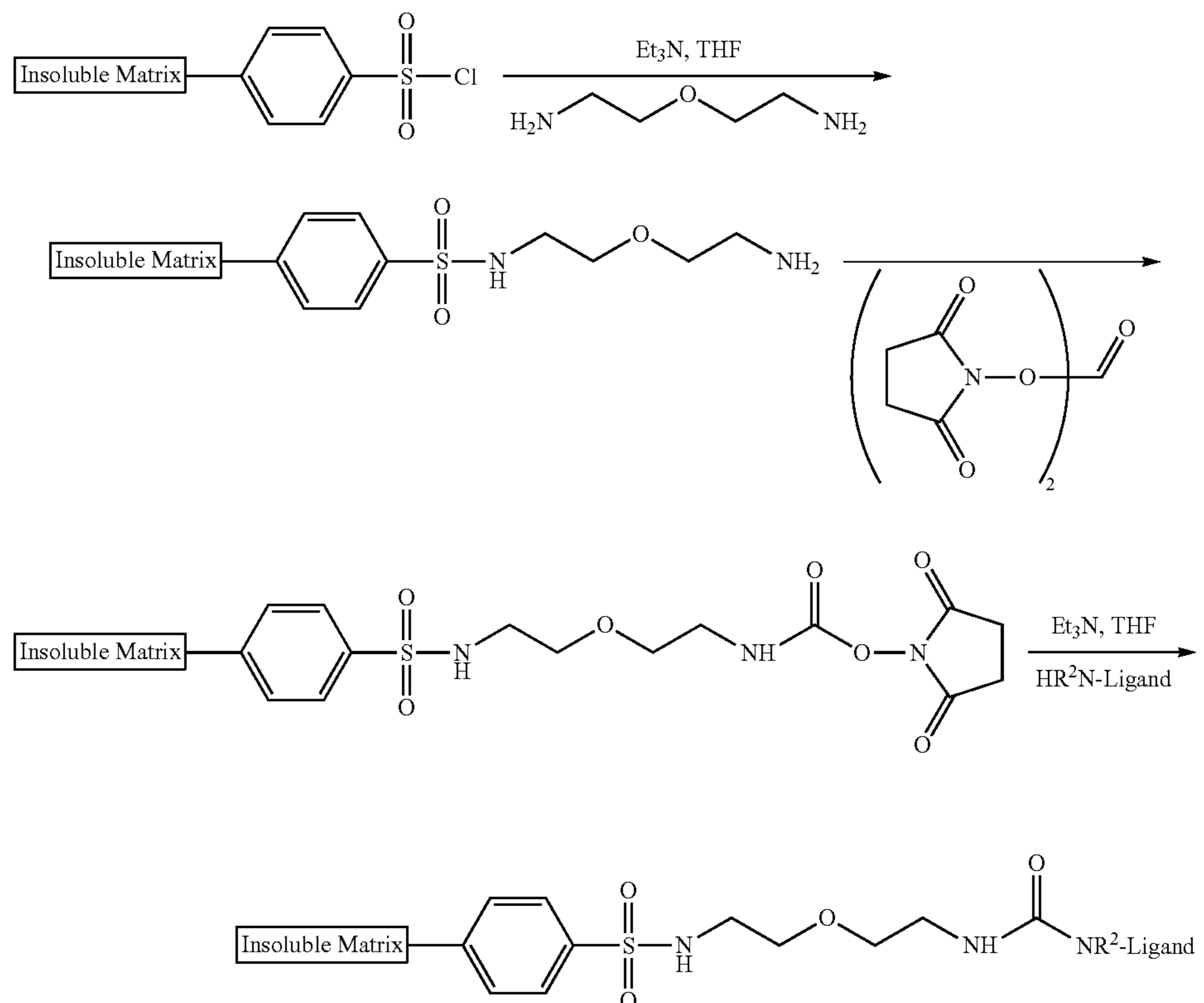
Scheme 4
