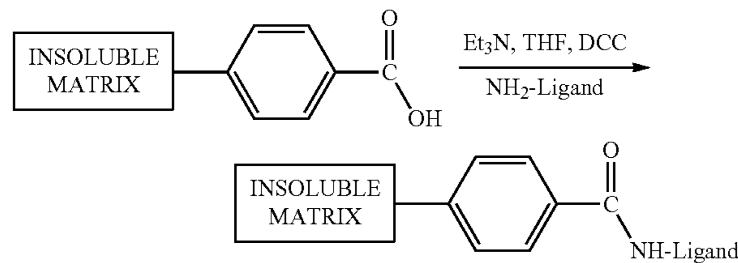
Scheme 2
