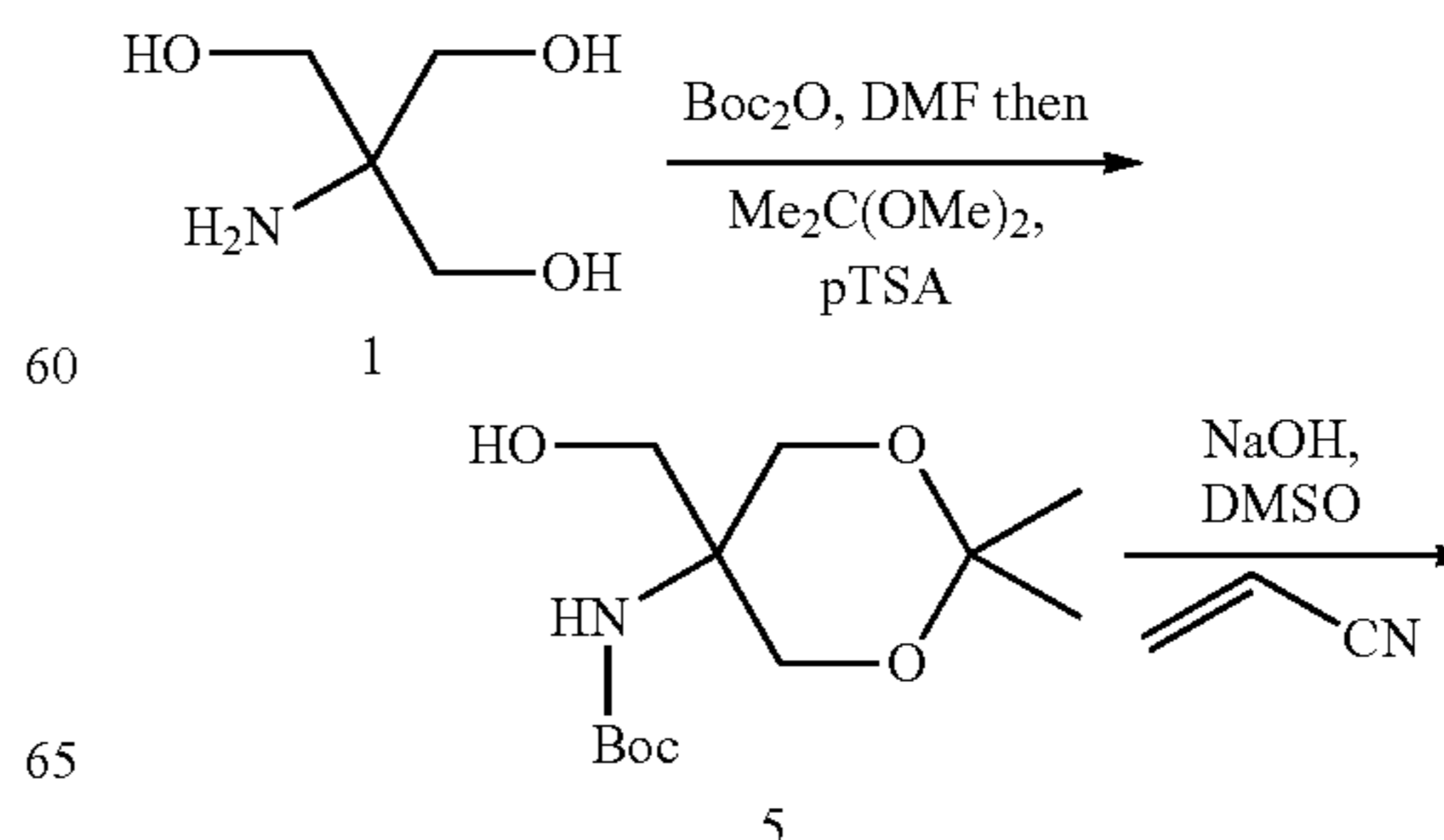
Scheme 8
