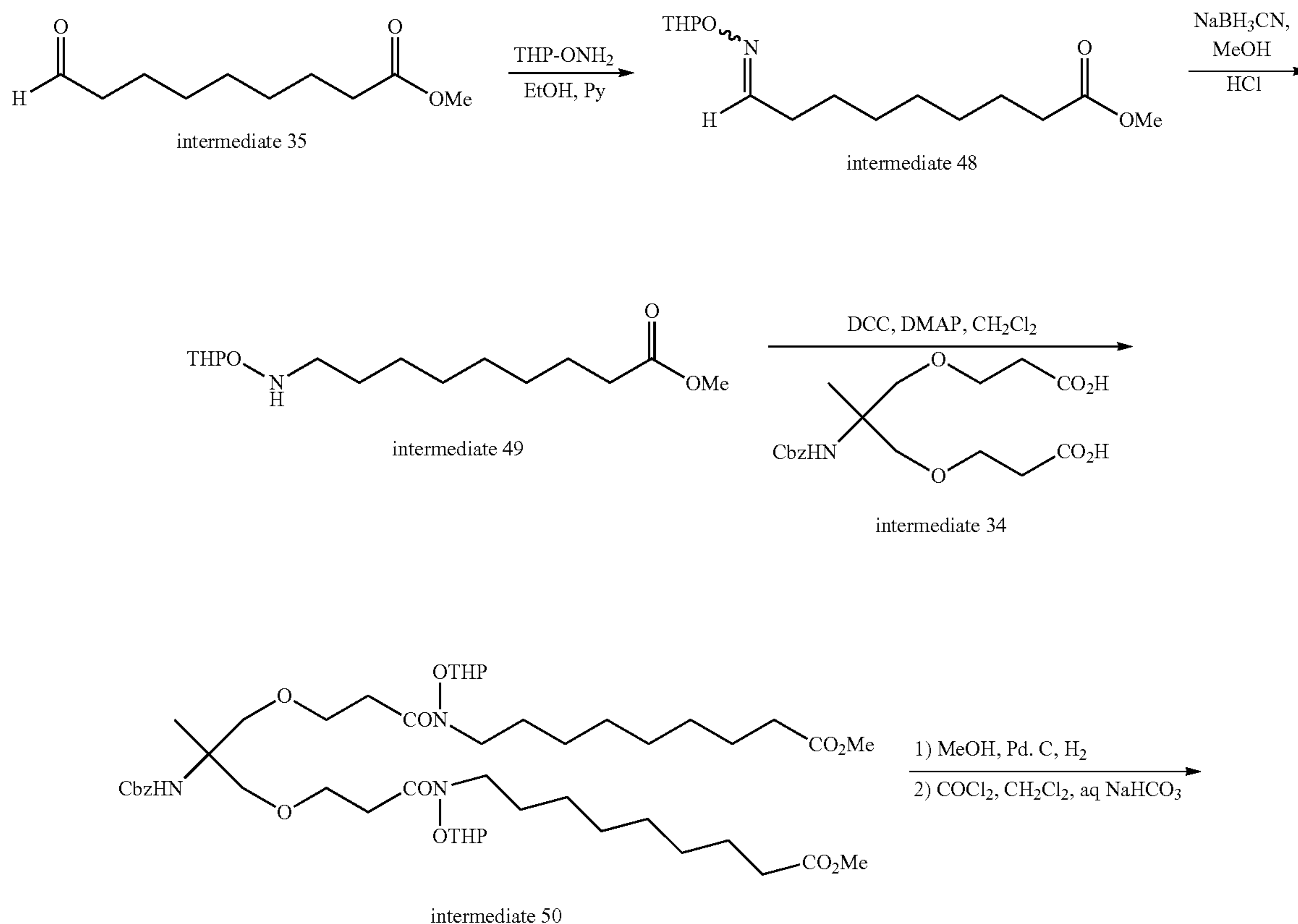
Scheme 46
