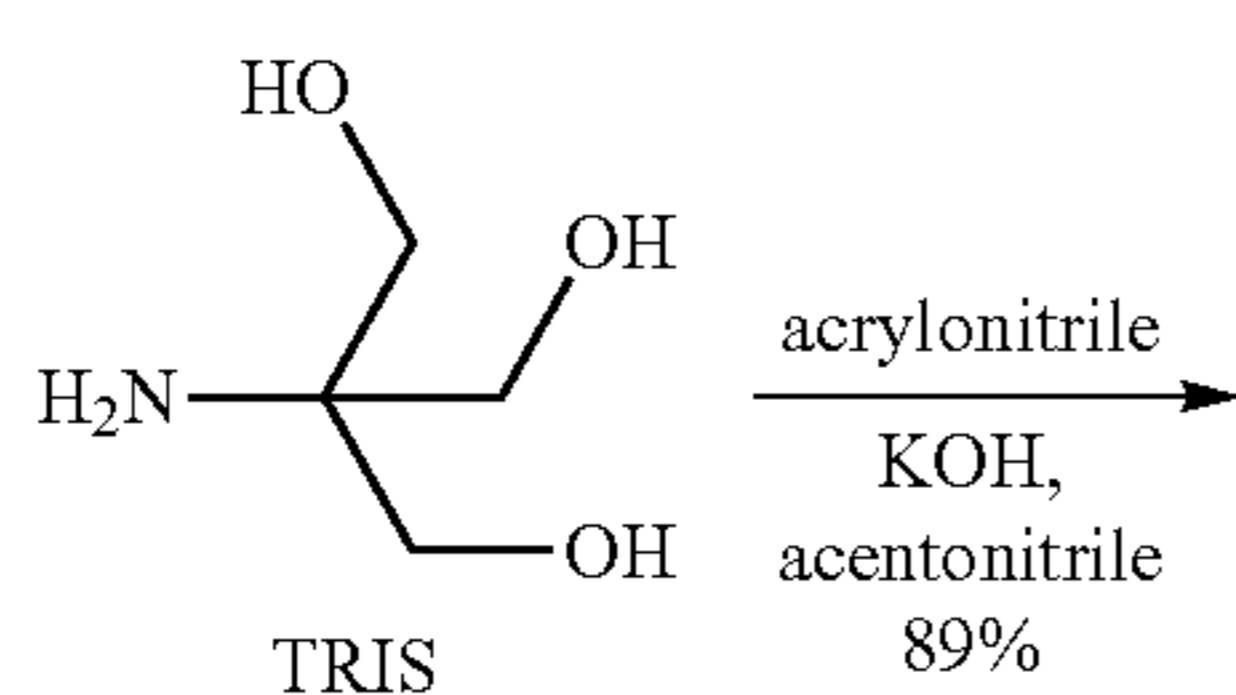
Scheme 45
