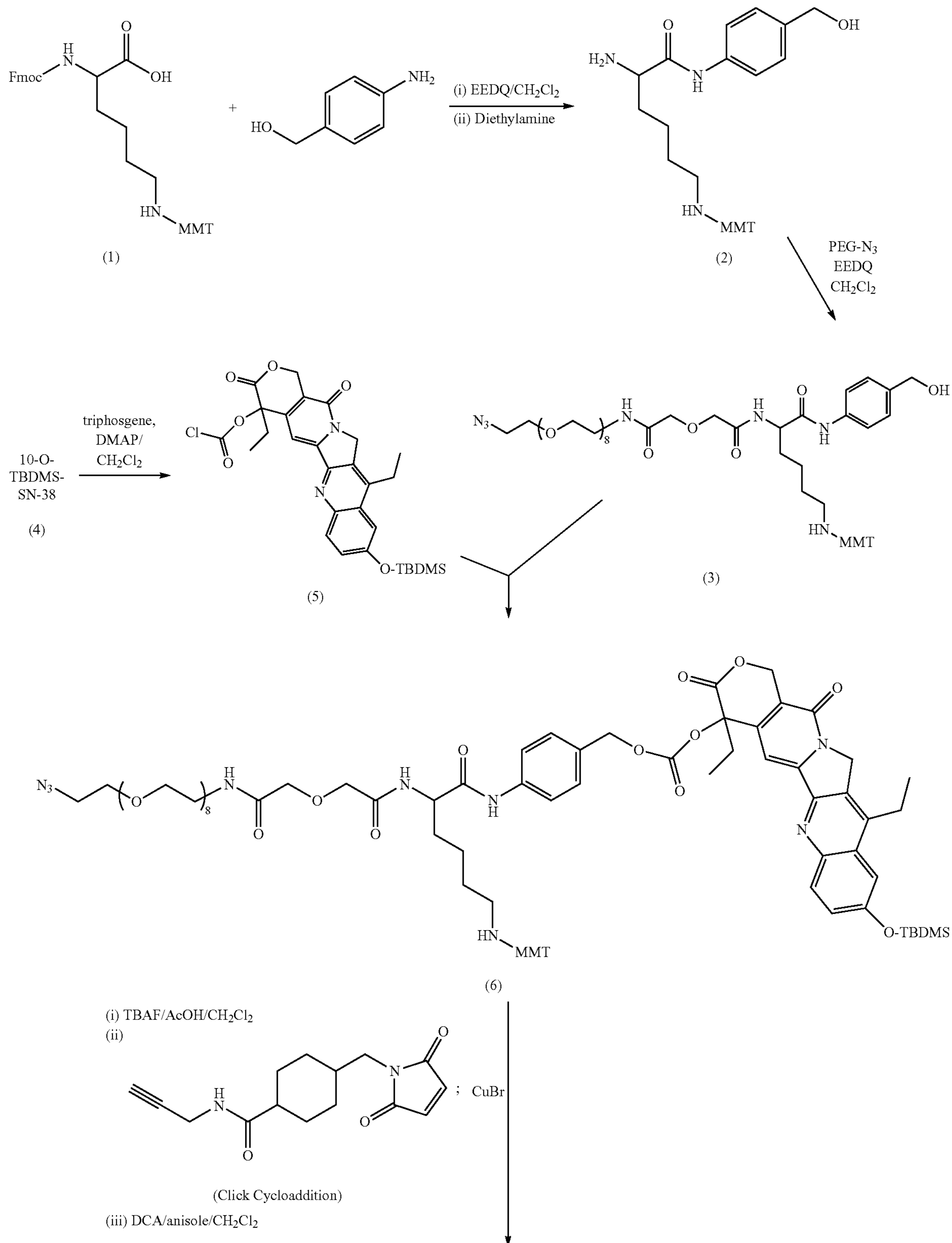
Scheme-3: Preparation of CL2A-SN-38
