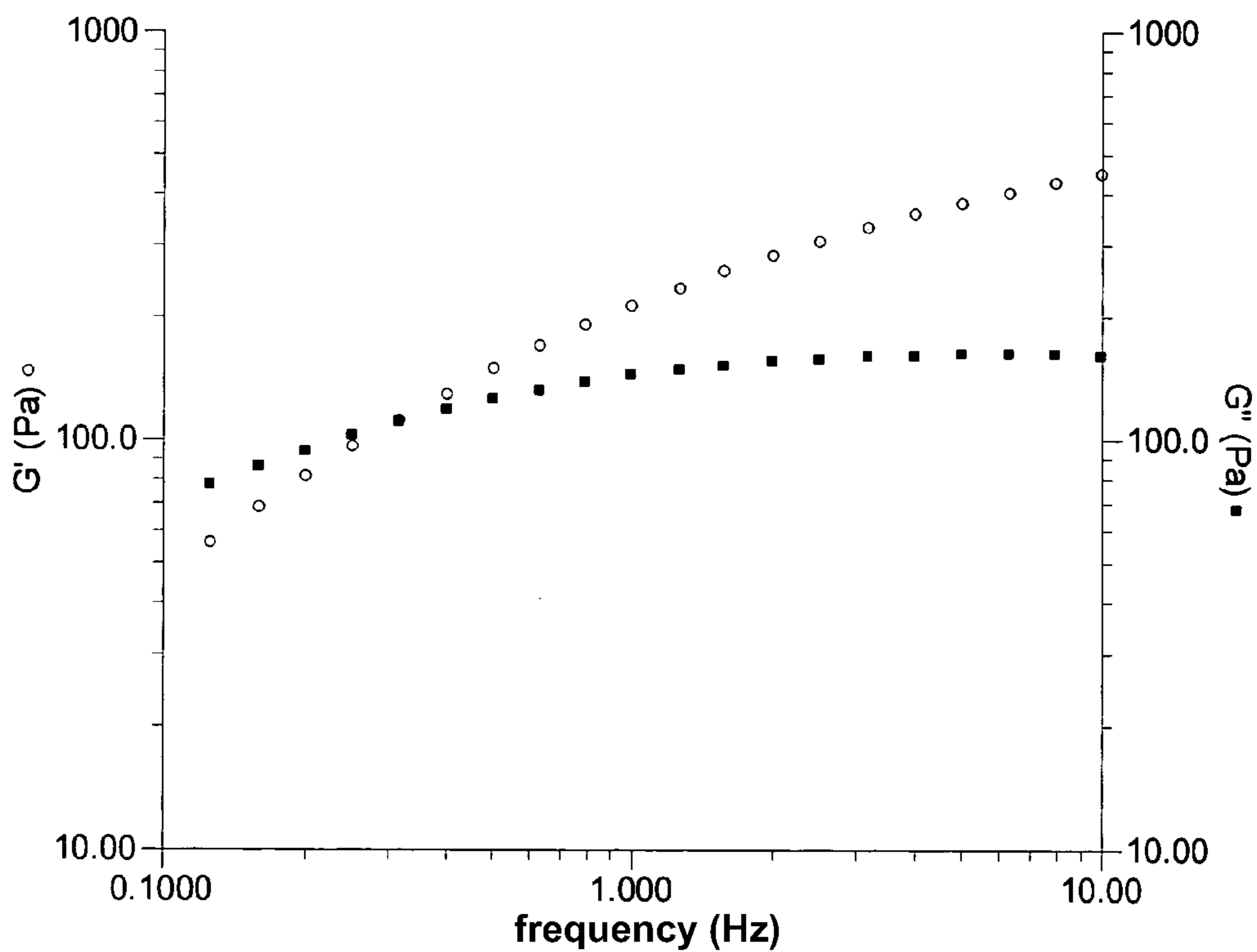
Figure 2. Frequency scanning, formulation B
