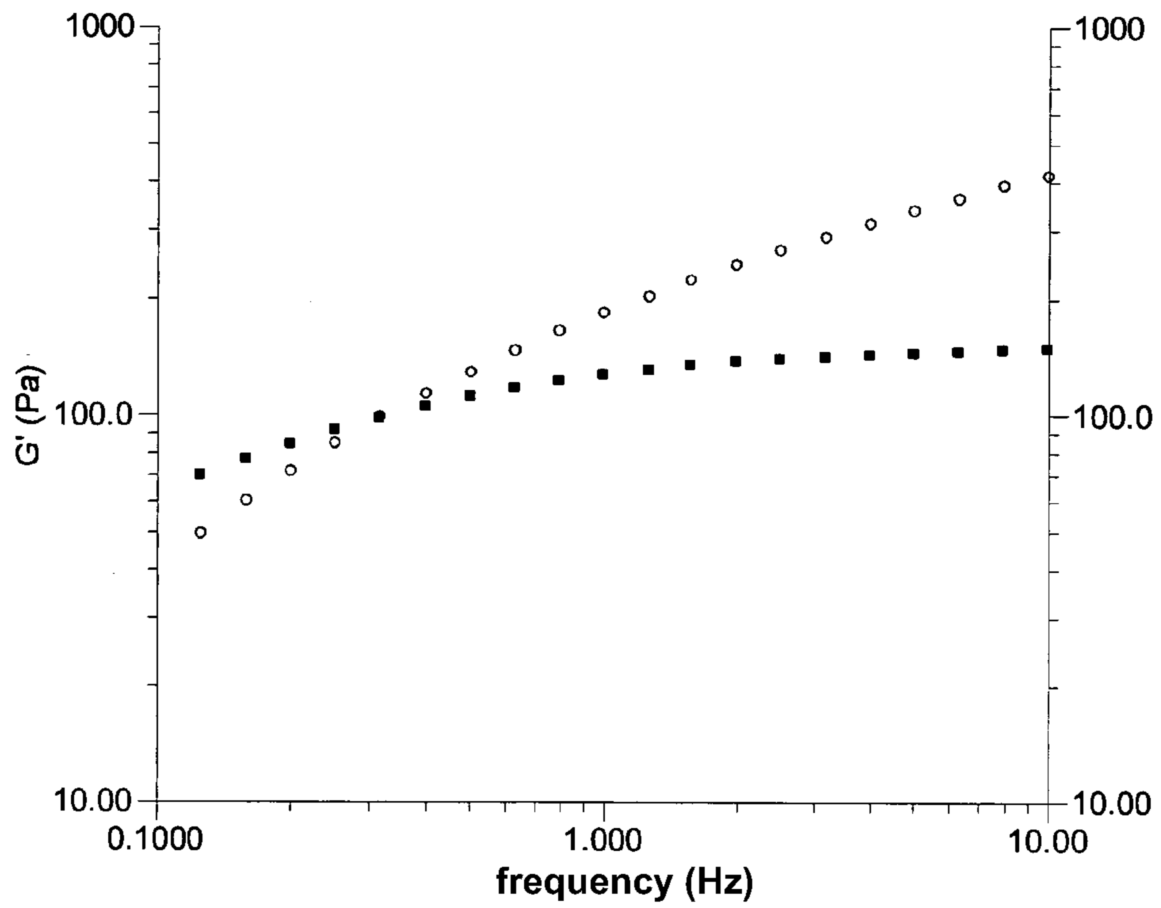
Figure 4. Frequency scanning, formulation D
