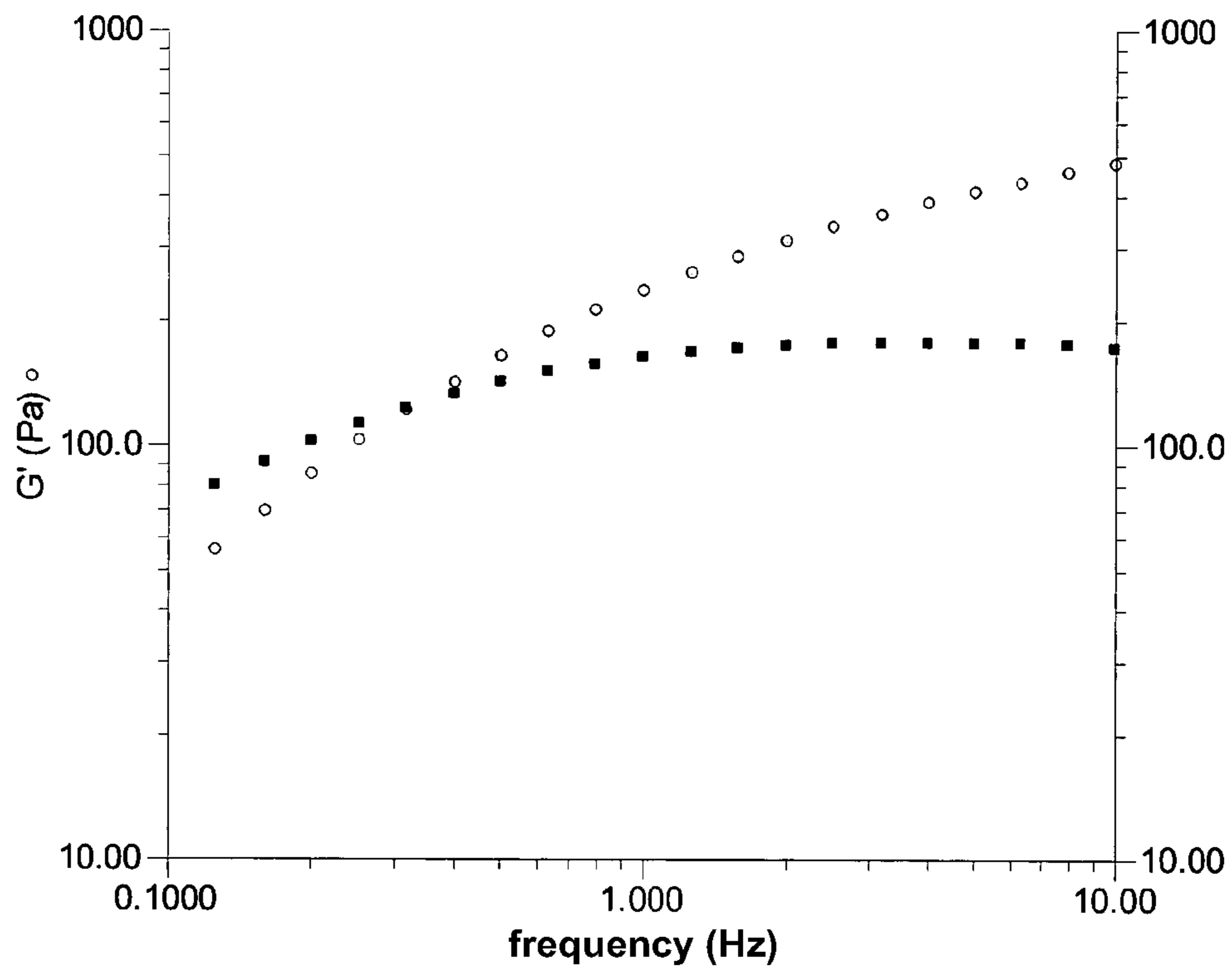
Figure 5. Frequency scanning, formulation E
