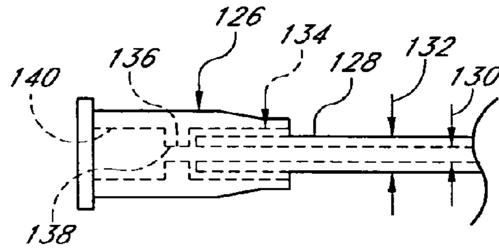
FIG. 15 (PRIOR ART)
