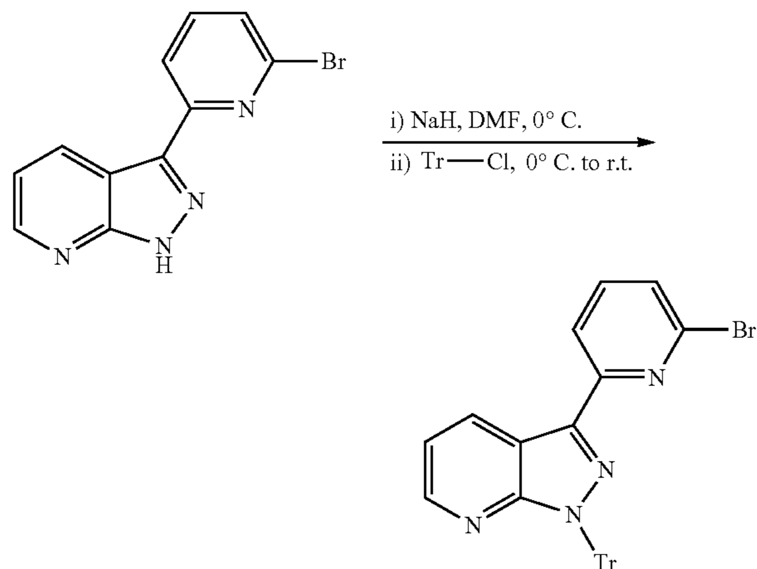
3-(6-bromopyridin-2-yl)-1-trityl-1H-pyrazolo[3,4-b]pyridine
