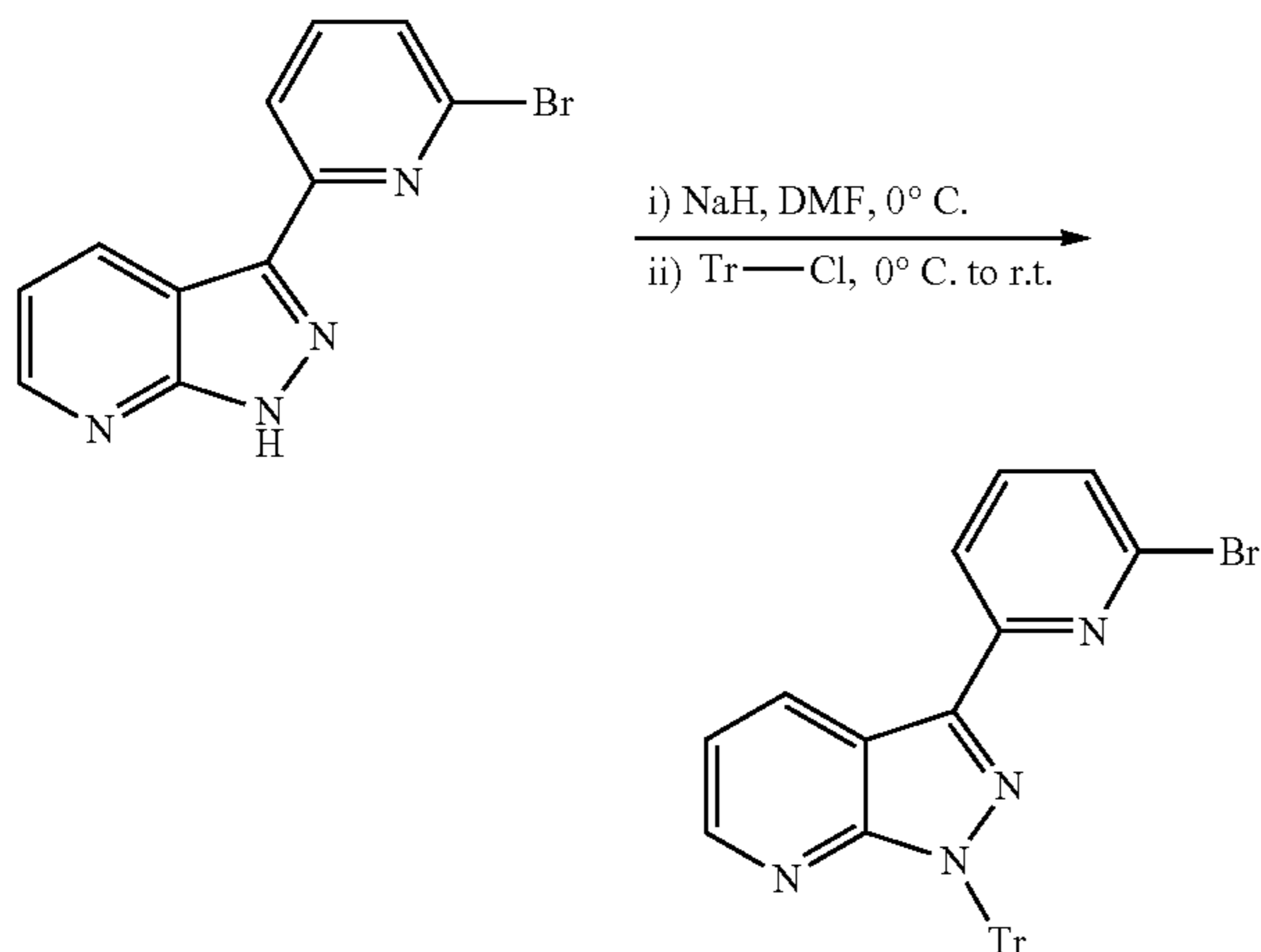
3-(6-bromopyridin-2-yl)-1-trityl-1H-pyrazolo[3,4-b]pyridine
