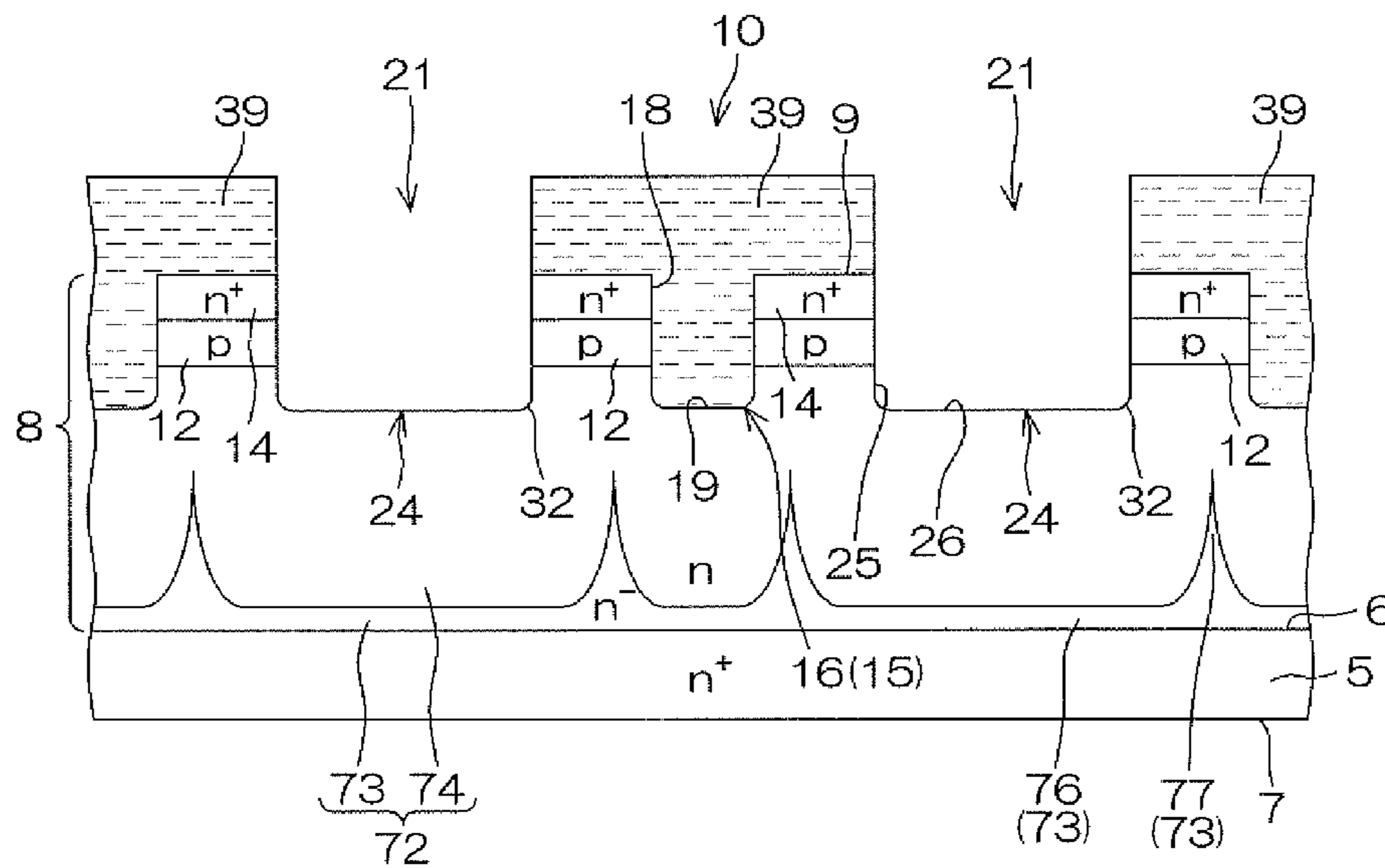
B-B SECTION
