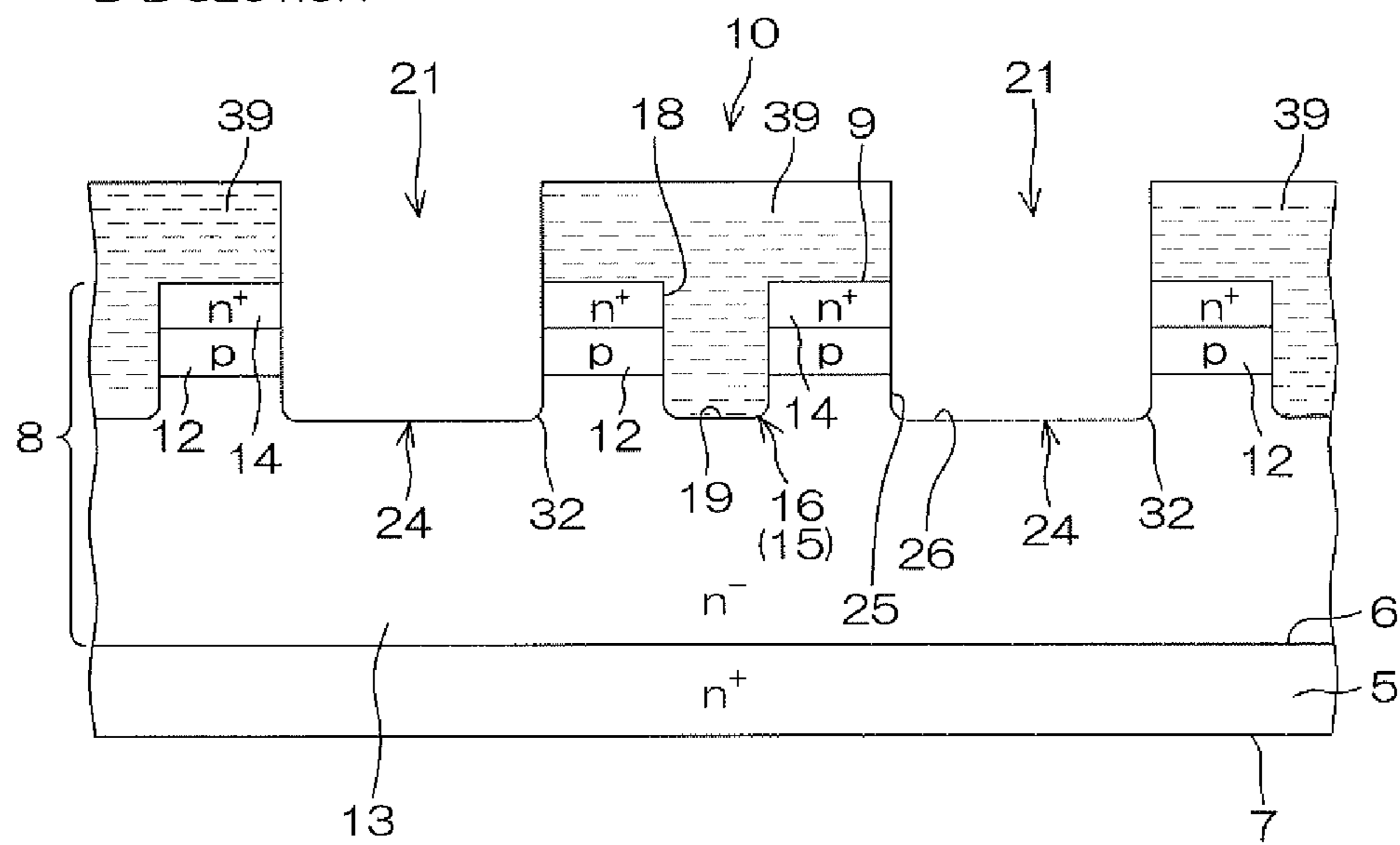
B-B SECTION
