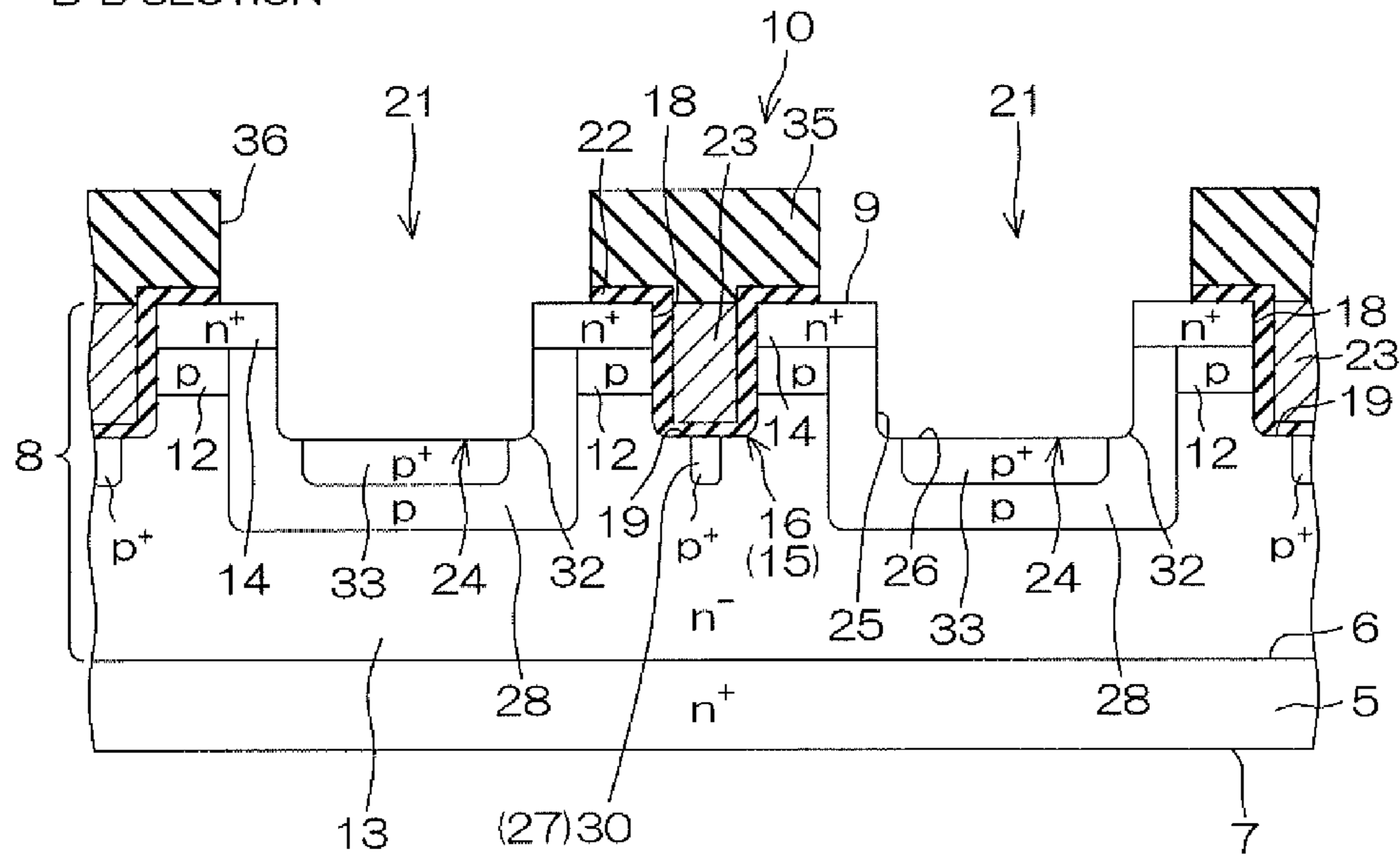
B-B SECTION
