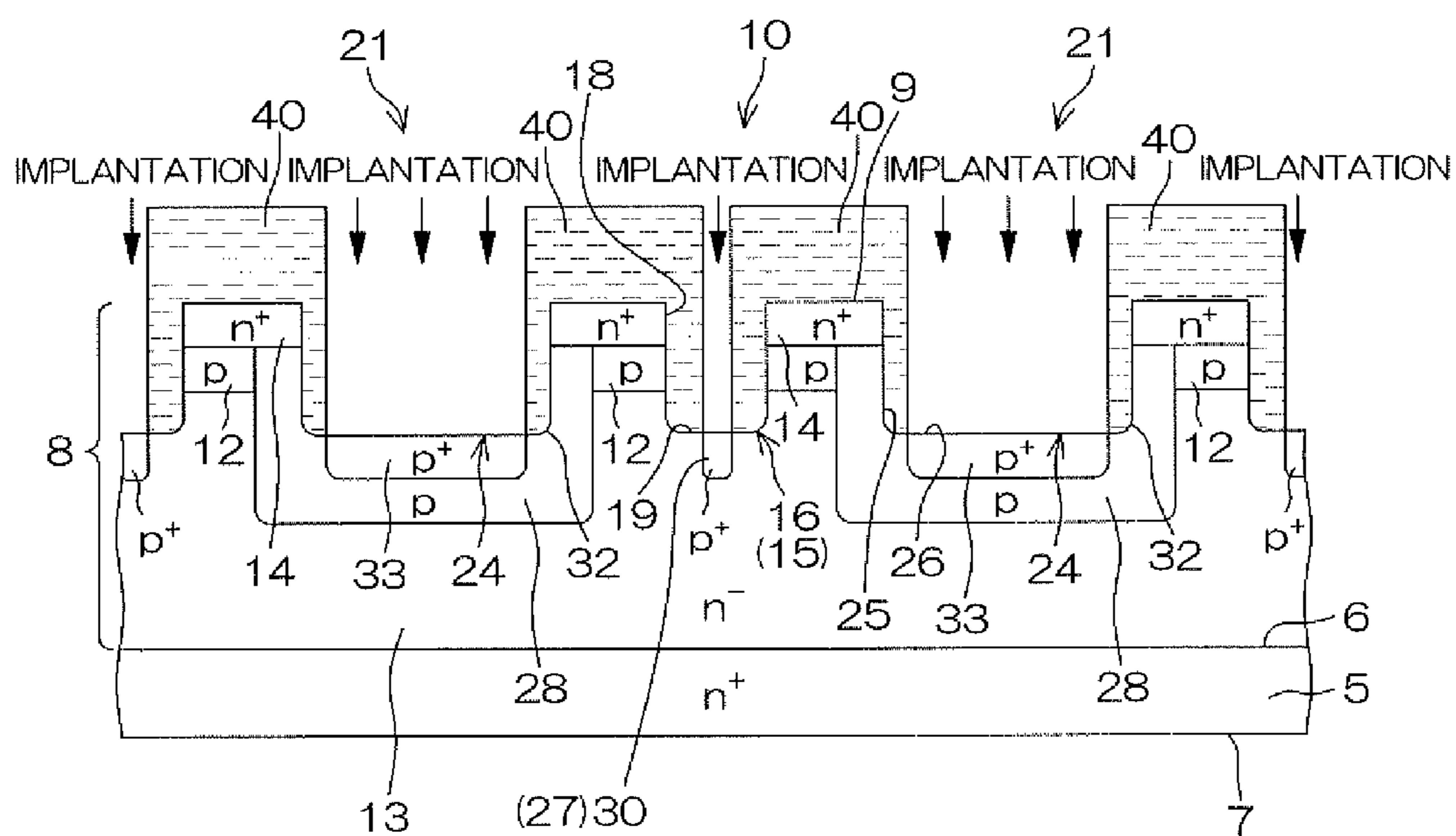
B-B SECTION
