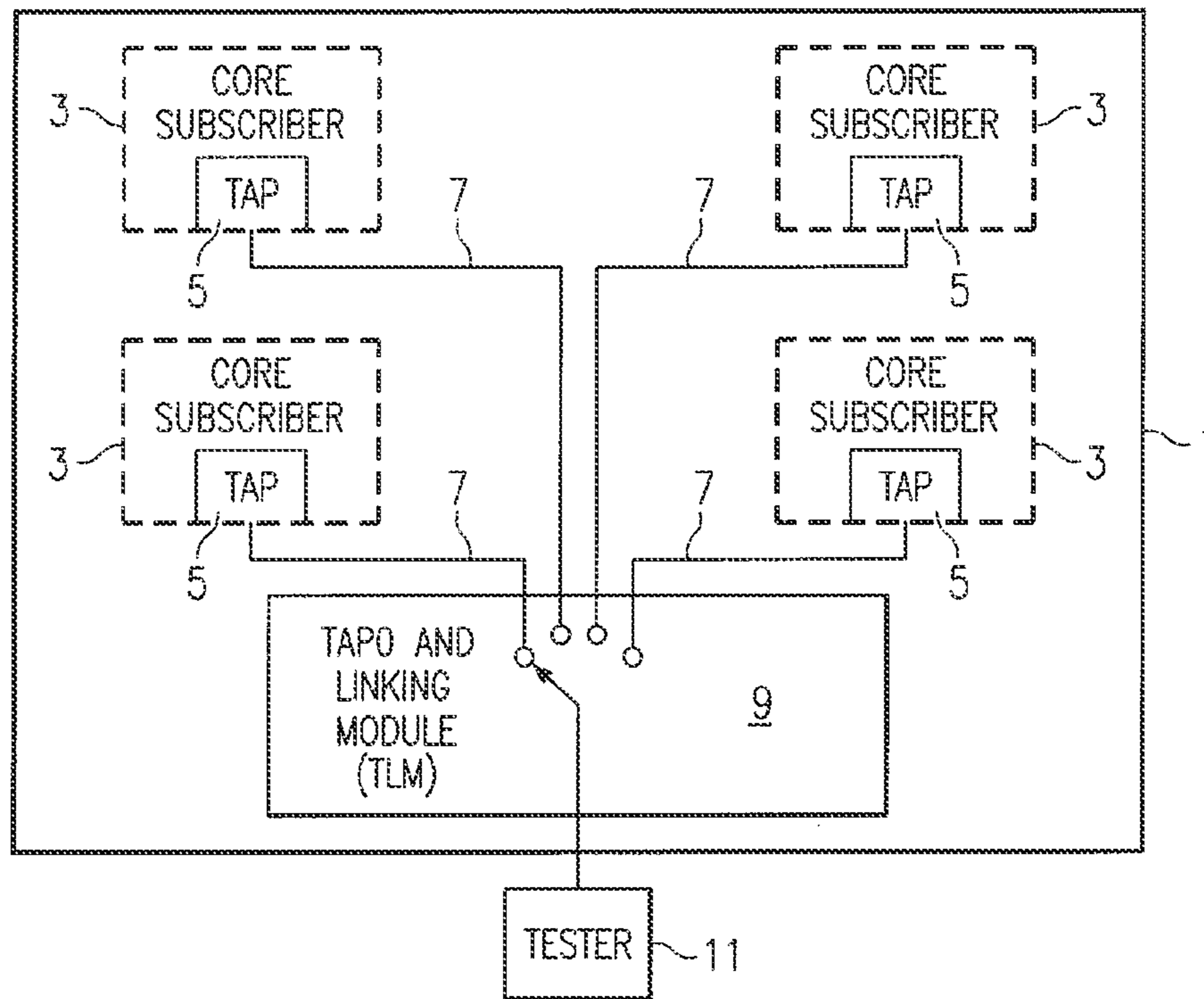
FIG. 1 (PRIOR ART)
