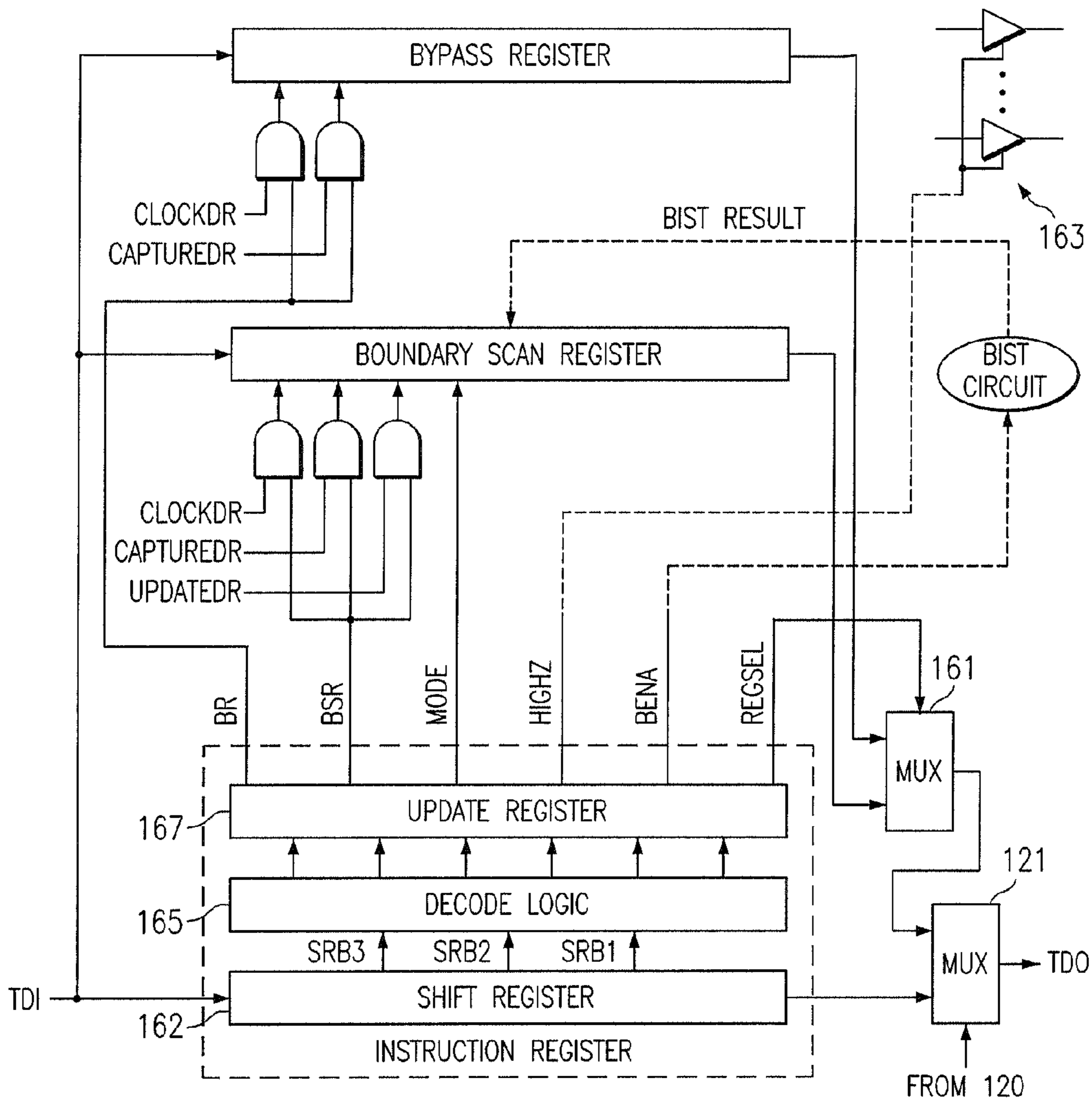
FIG. 16 (PRIOR ART)
