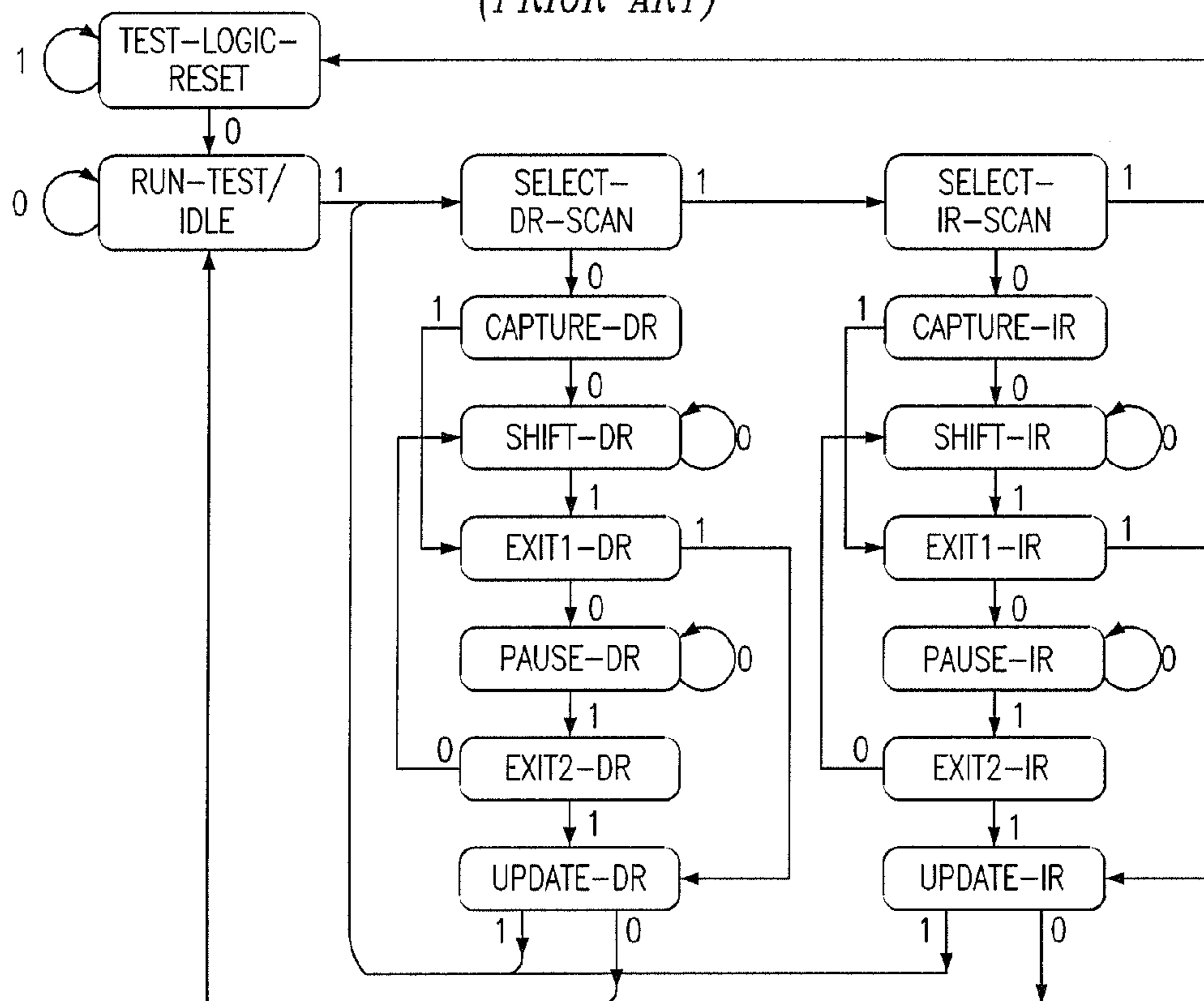
FIG. 14 (PRIOR ART)
