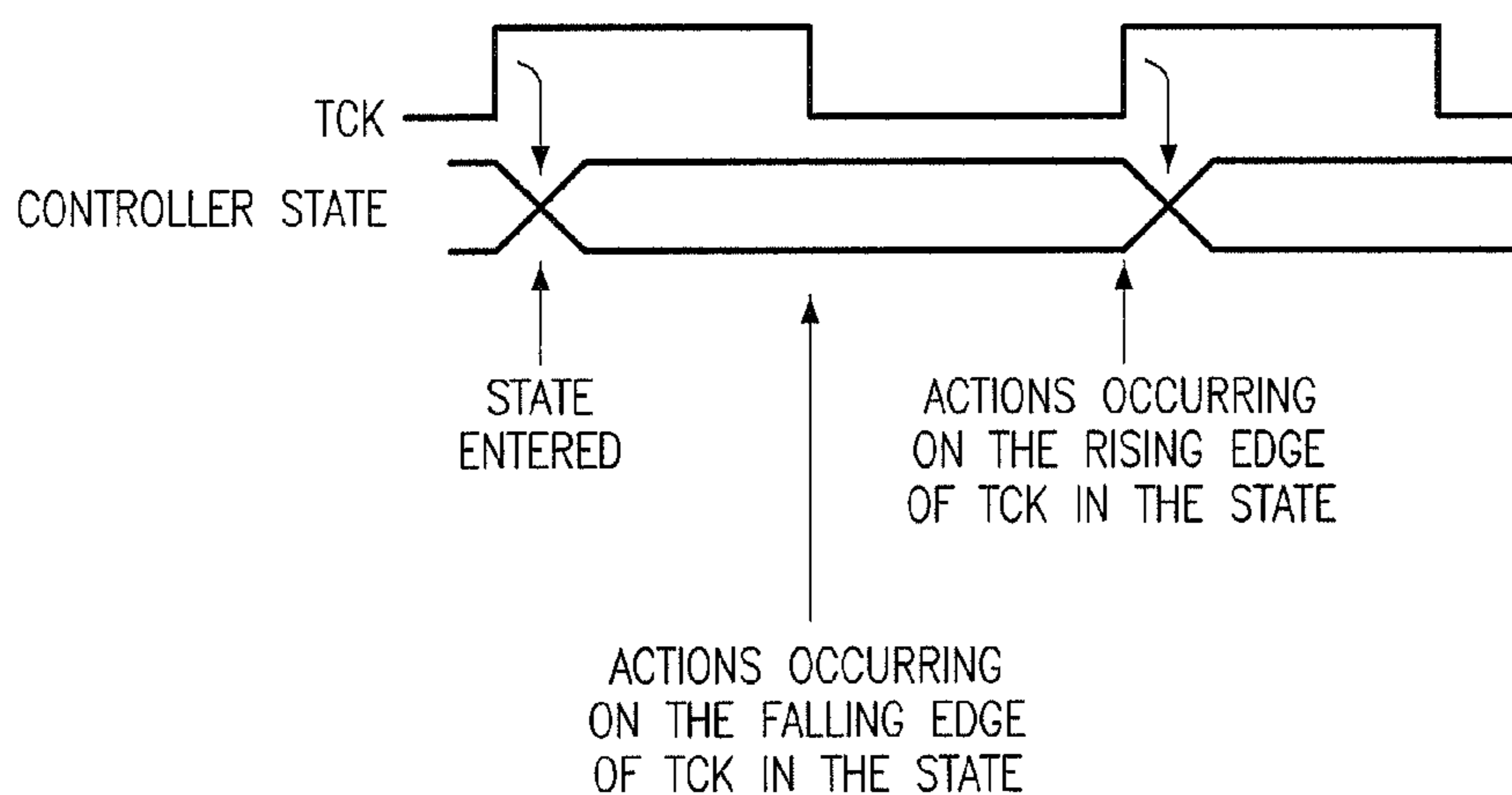
FIG. 15 (PRIOR ART)
