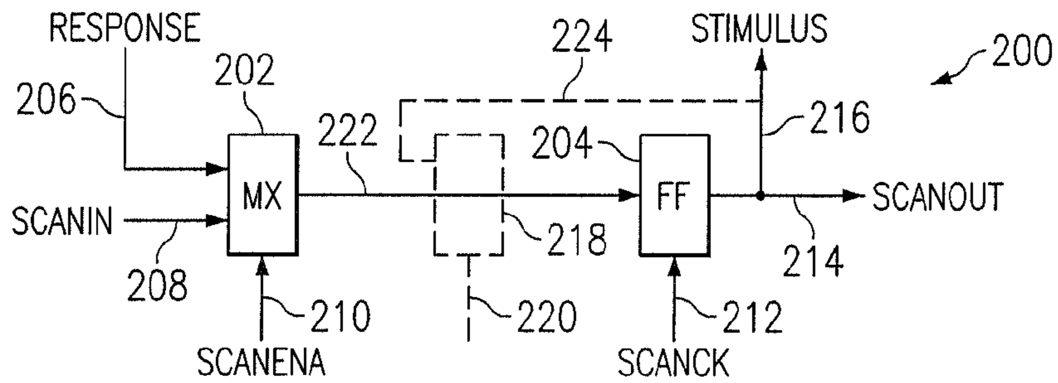
FIG. 2 (PRIOR ART)
