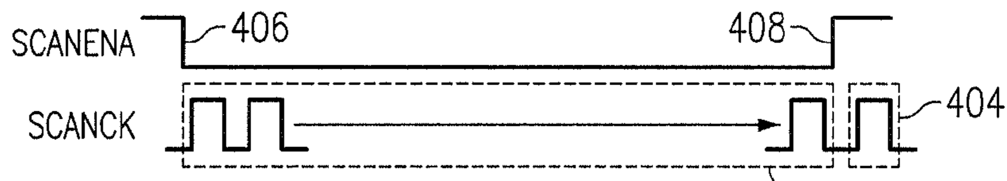
FIG. 4 (PRIOR ART)
