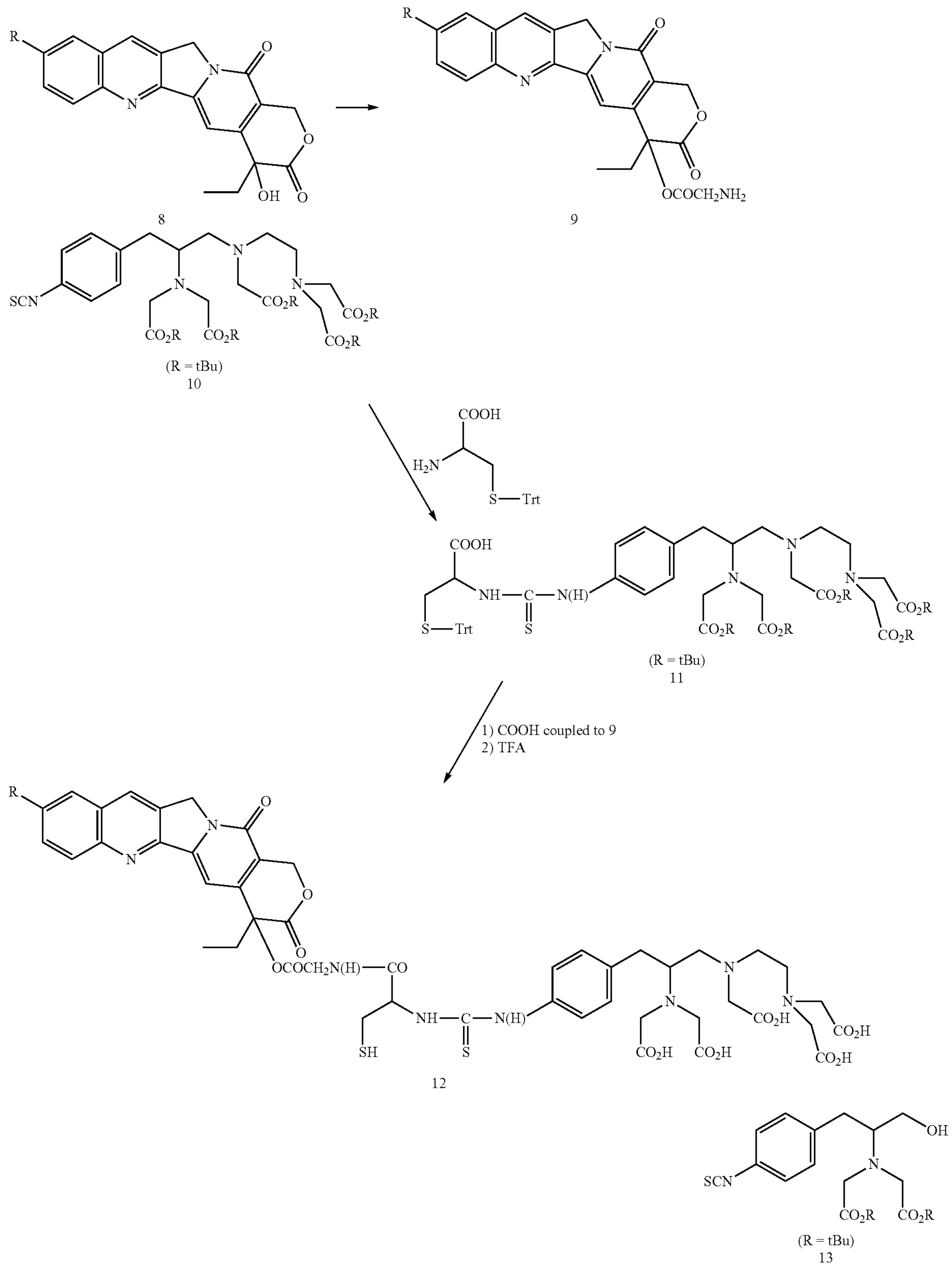
Scheme-4 (R = H for CPT or OH for 10-OH-CPT)
