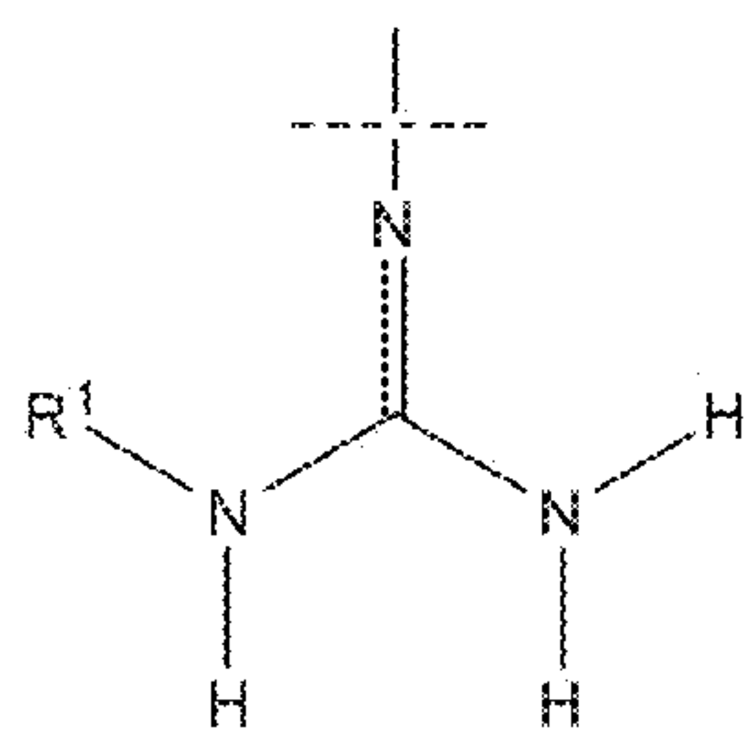
R^1 = \text{alkyl, aryl, aralkyl} R^{2-4} = H
