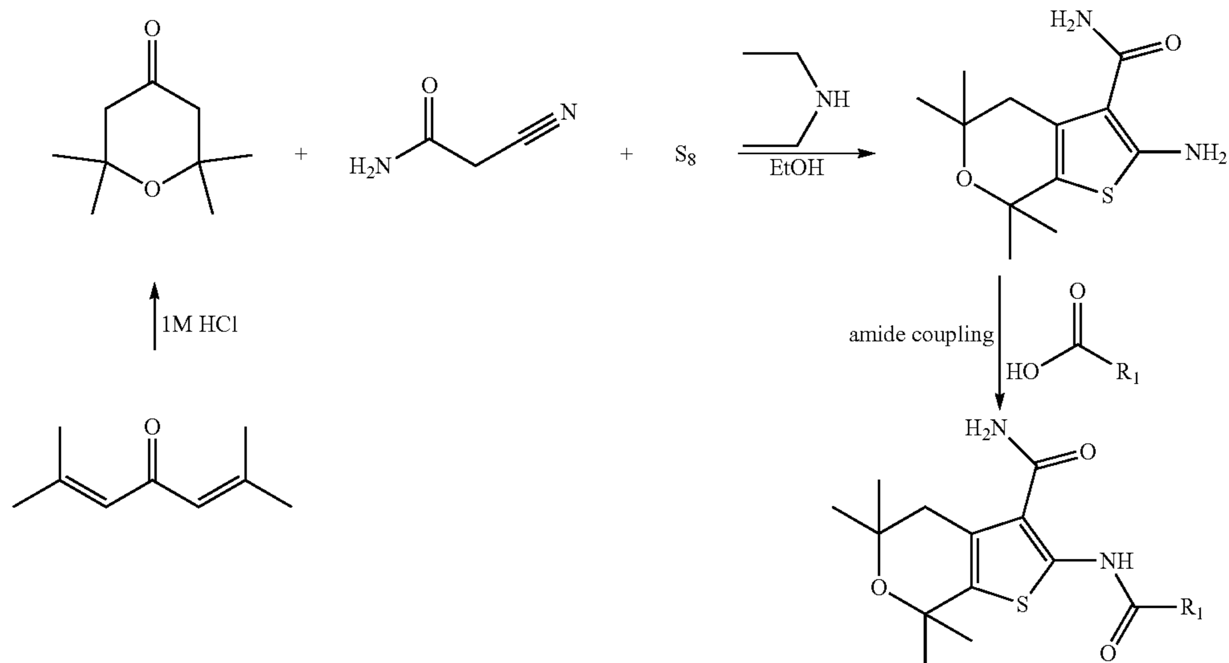
Scheme 1: synthesis of the core and subsequent amide coupling
