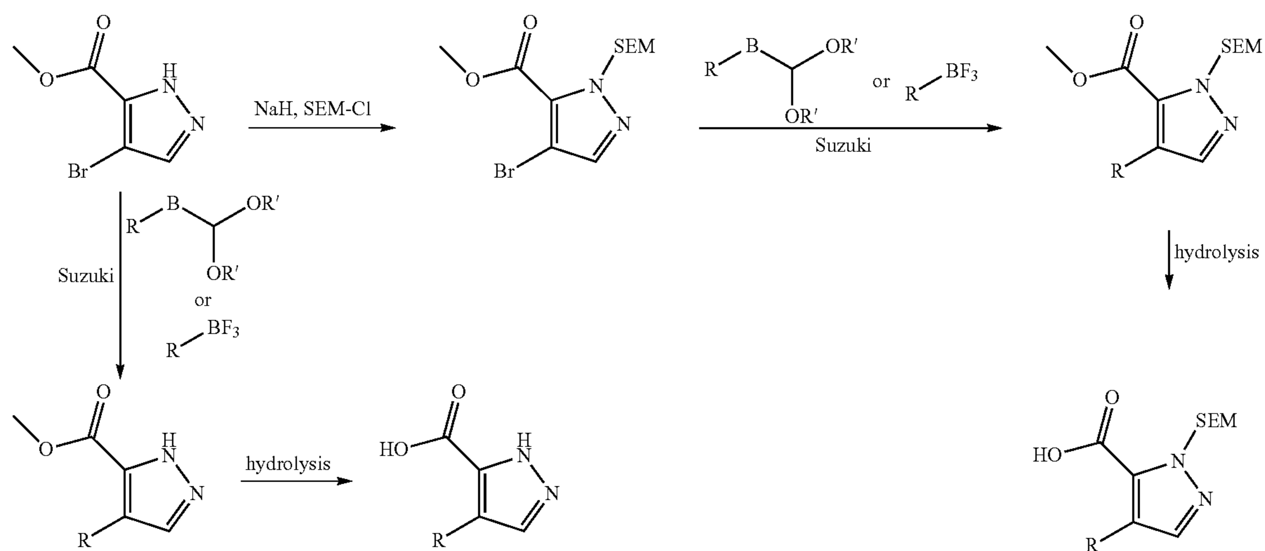
Scheme 2: synthesis of 4-substituted pyrazole derivatives
