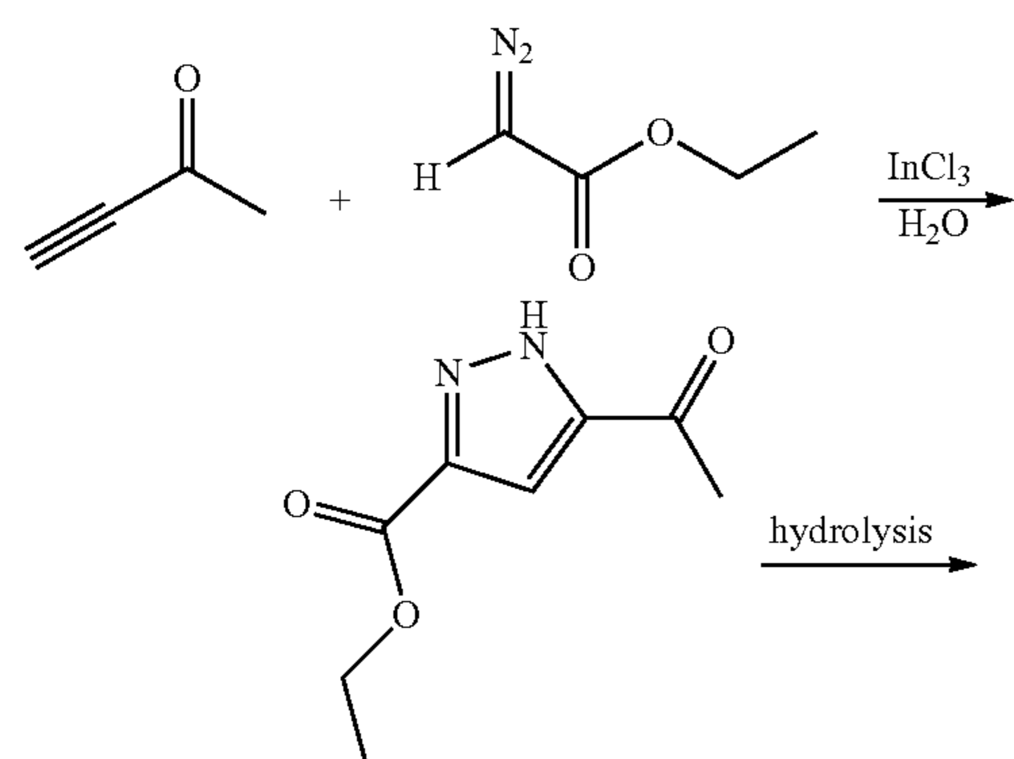
Scheme 3: synthesis of 3-substituted pyrazole derivatives
