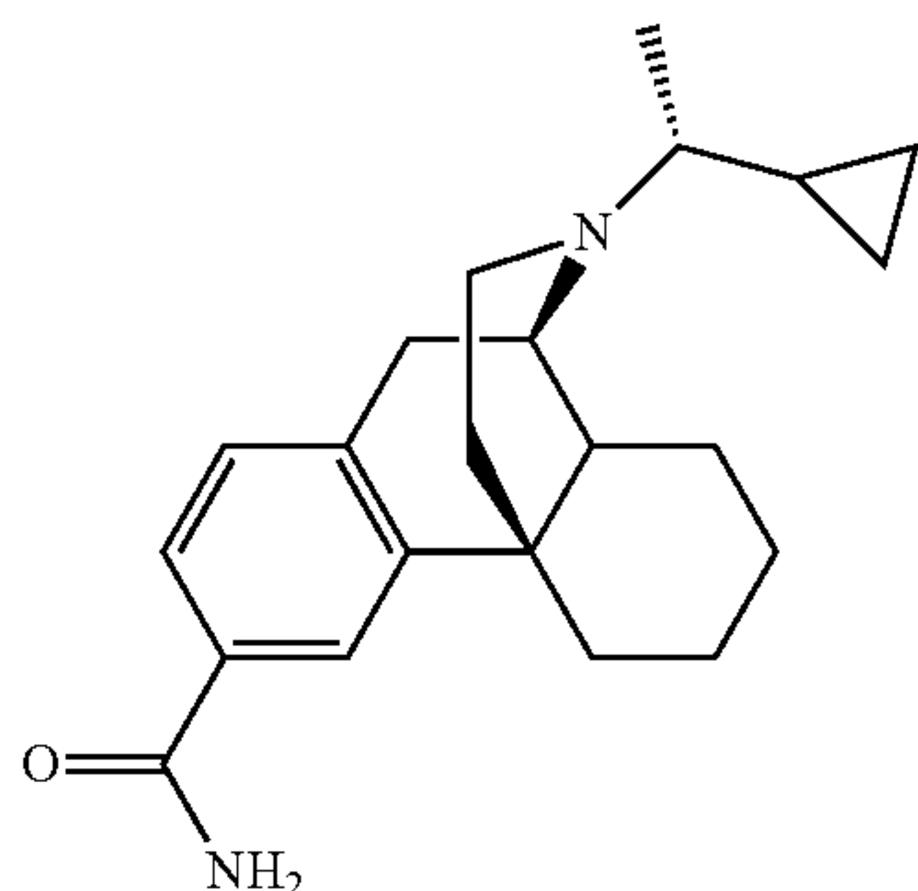
Chemical Formula: \text{C}_{22}\text{H}_{30}\text{N}_2\text{O} Exact Mass: 338.24 Molecular Weight: 338.49
