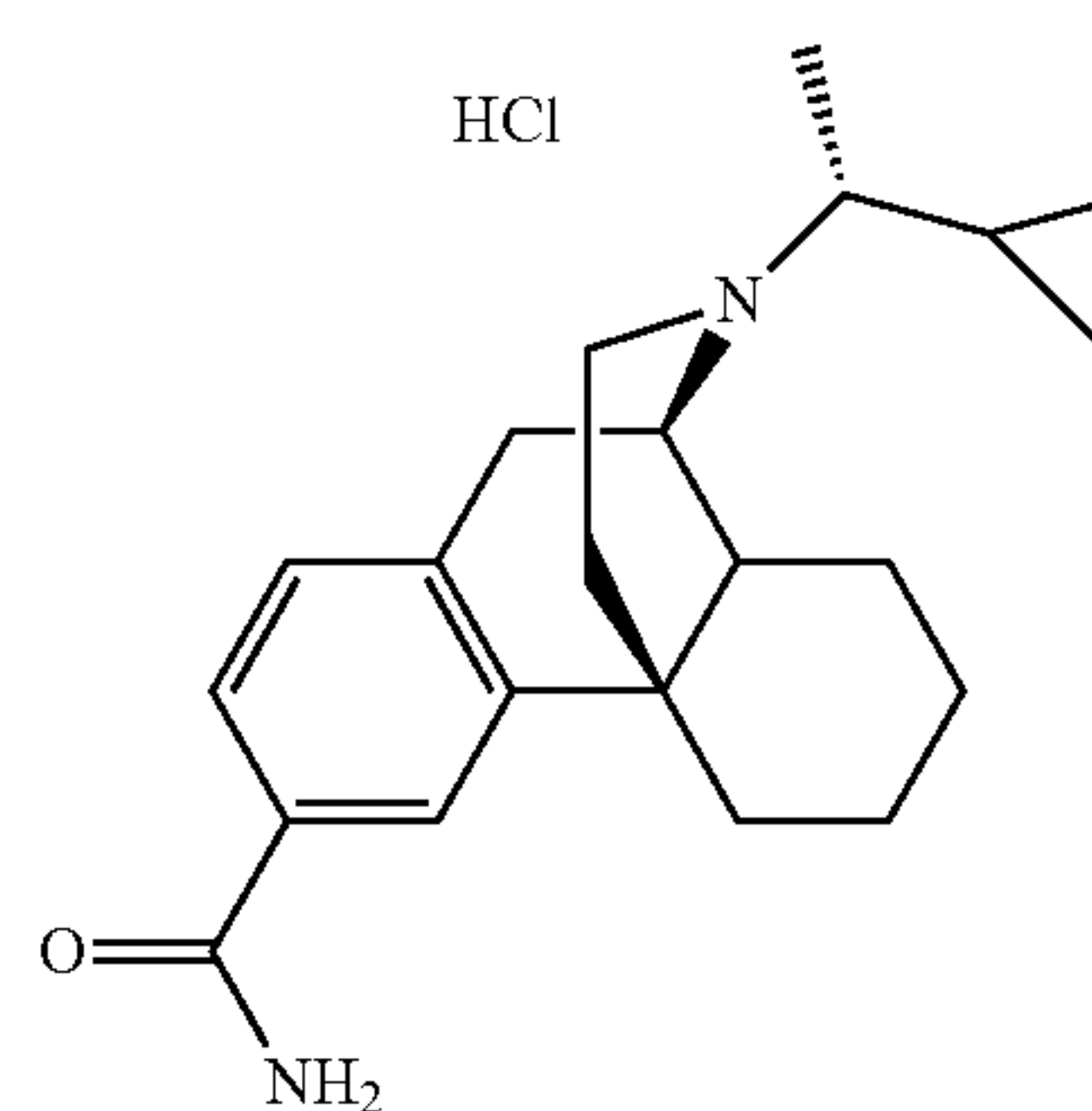
Chemical Formula: \text{C}_{22}\text{H}_{31}\text{ClN}_2\text{O} Exact Mass: 374.21 Molecular Weight: 374.95
