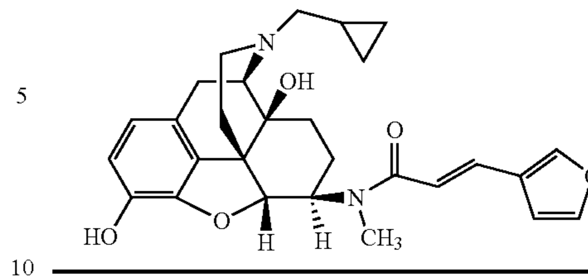
Compound 20
