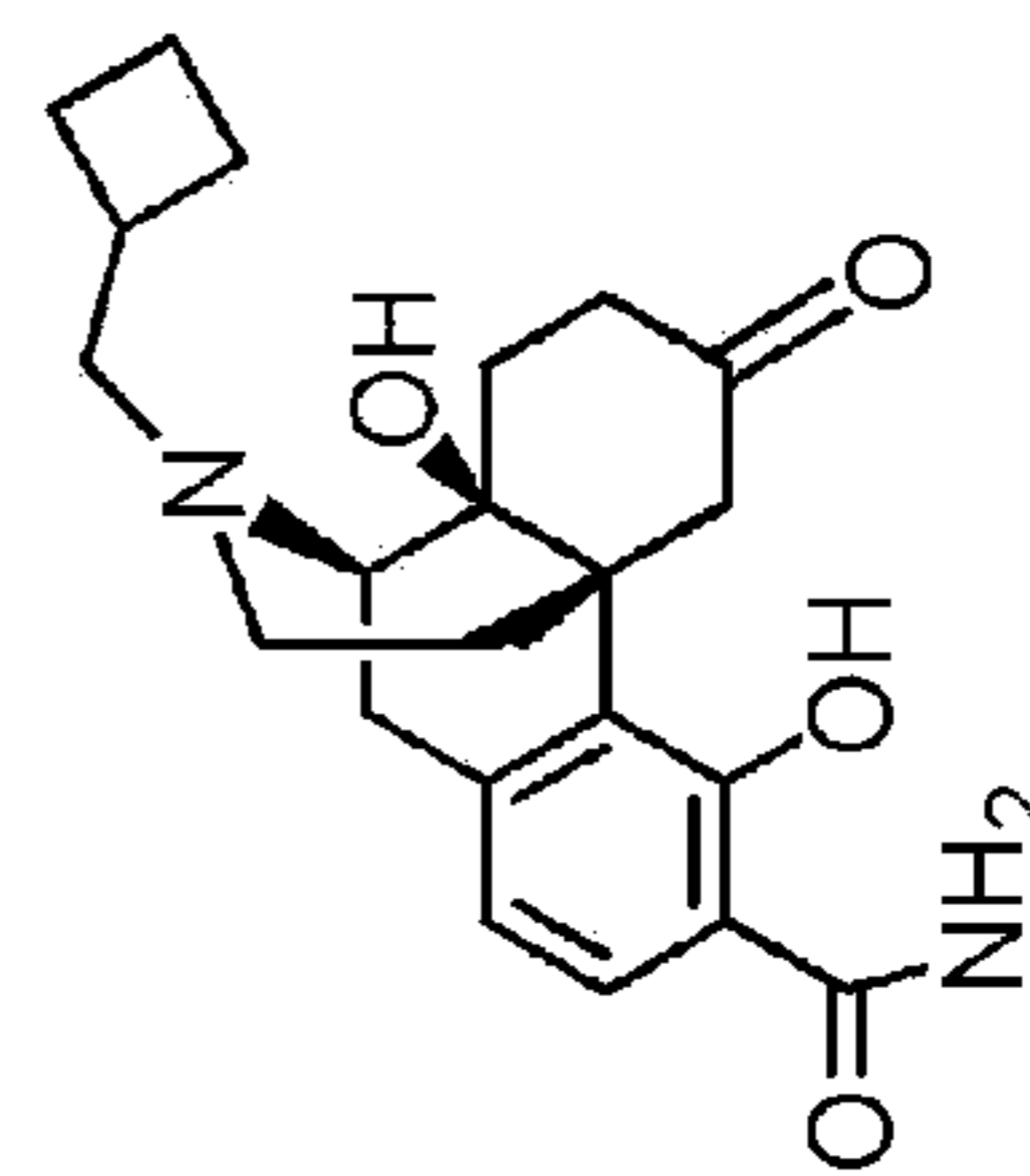
Compound A
