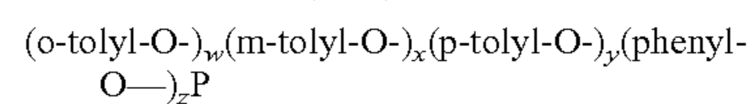
Formula (IVa)
