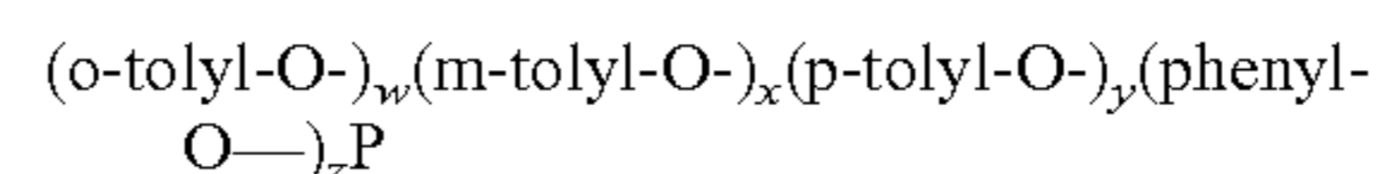
Formula (IVa)
