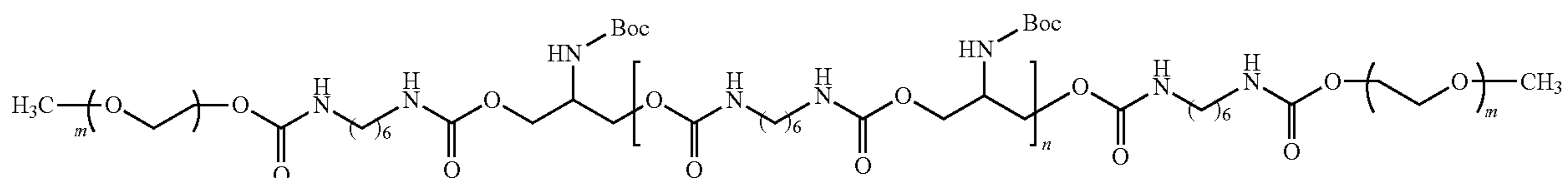
Scheme 1. Chemical structure of ESHU.
