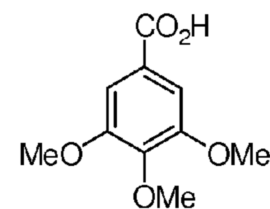
3,4,5-trimethoxybenzoic acid
