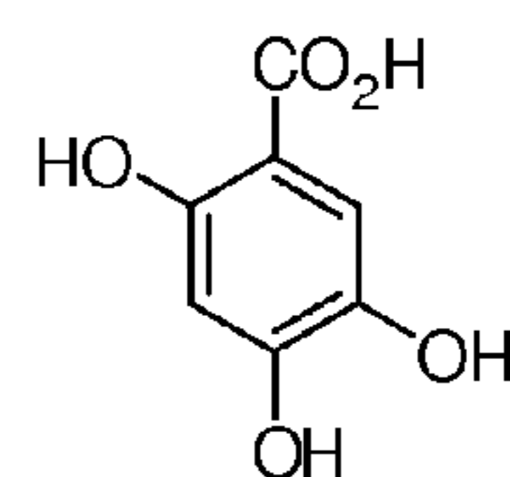
2,4,5-trihydroxybenzoic acid
