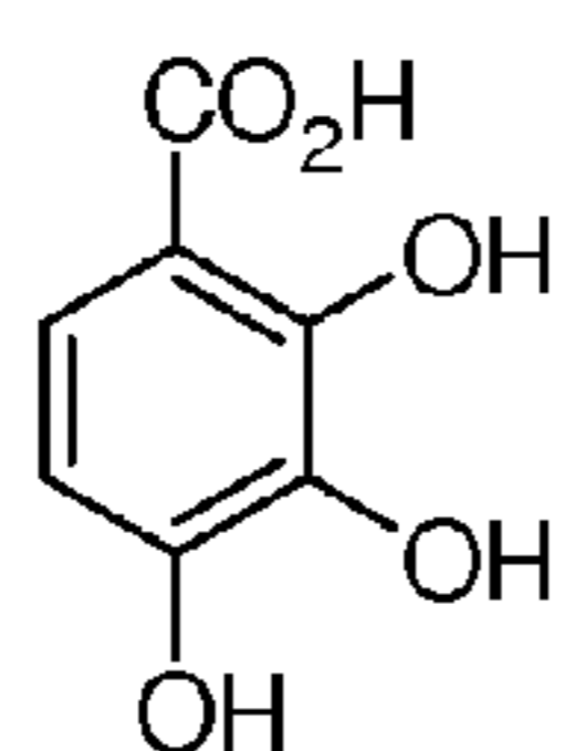
2,3,4-trihydroxybenzoic acid
