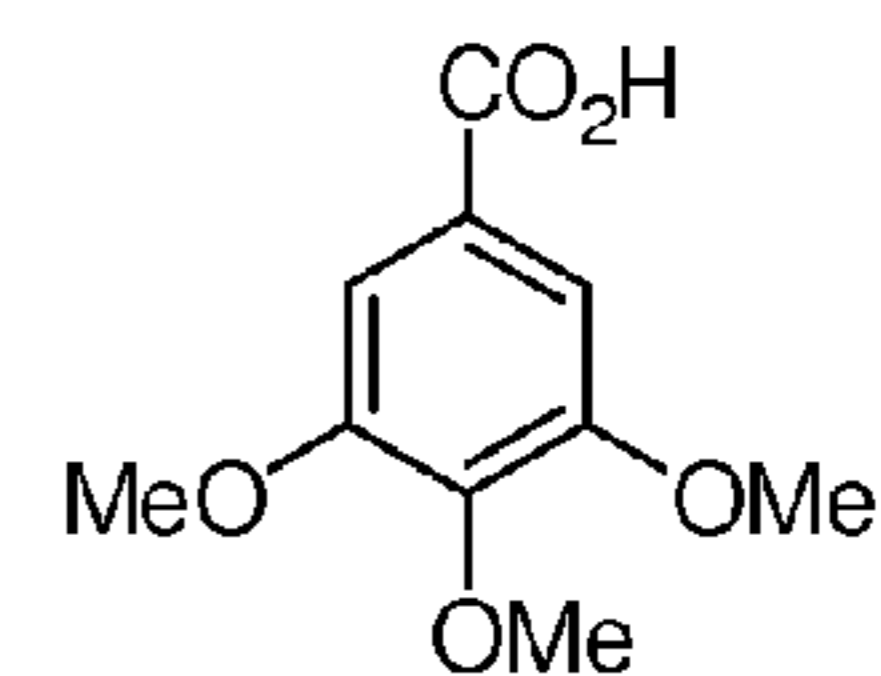
3,4,5-trimethoxybenzoic acid
