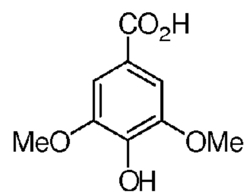
syringic acid
