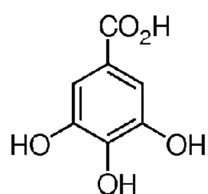
gallic acid
