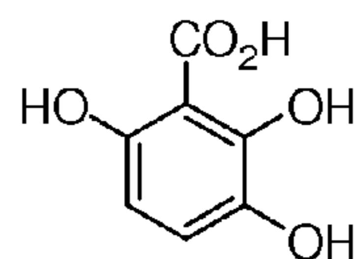
2,3,6-trihydroxybenzoic acid
