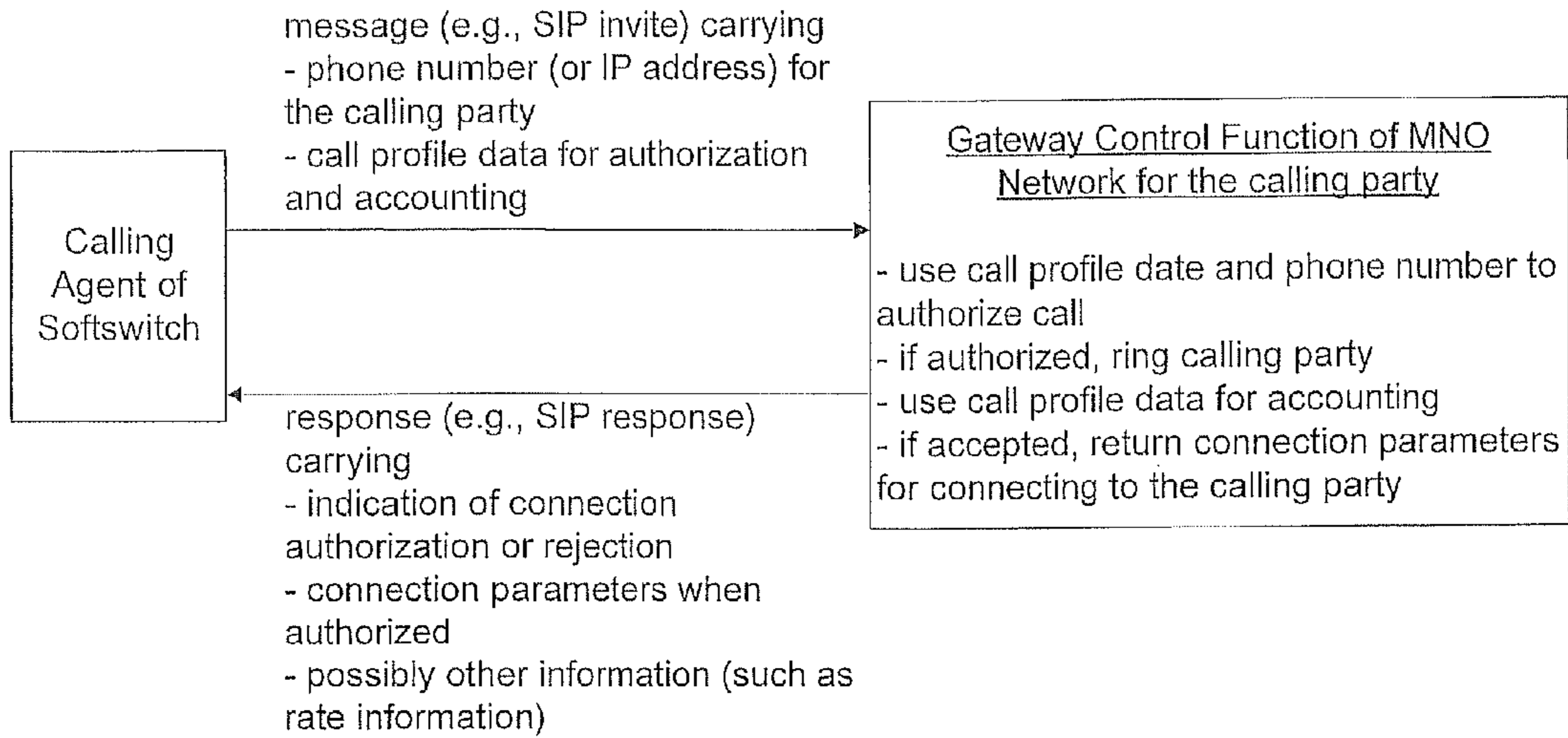
Calling Party Call-Setup Loop
