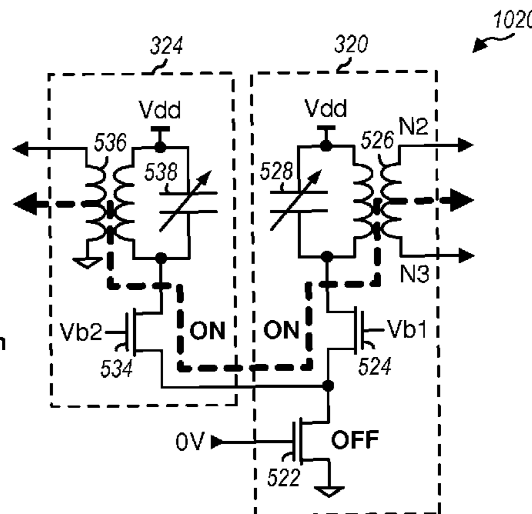
Programmable Attenuator
