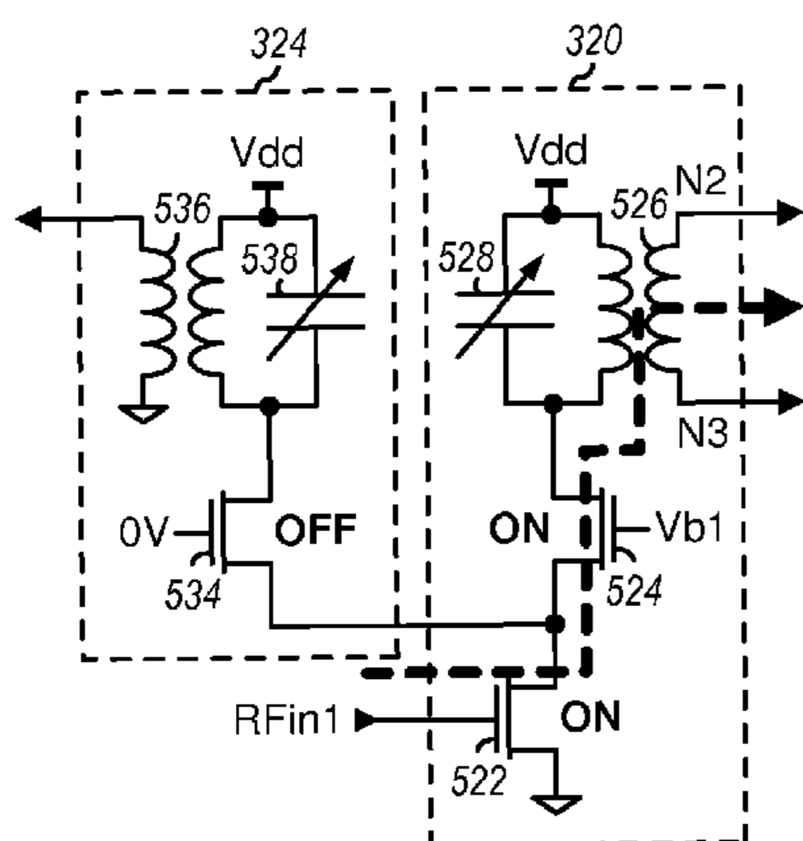
Common-Source LNA & Interface Circuit
