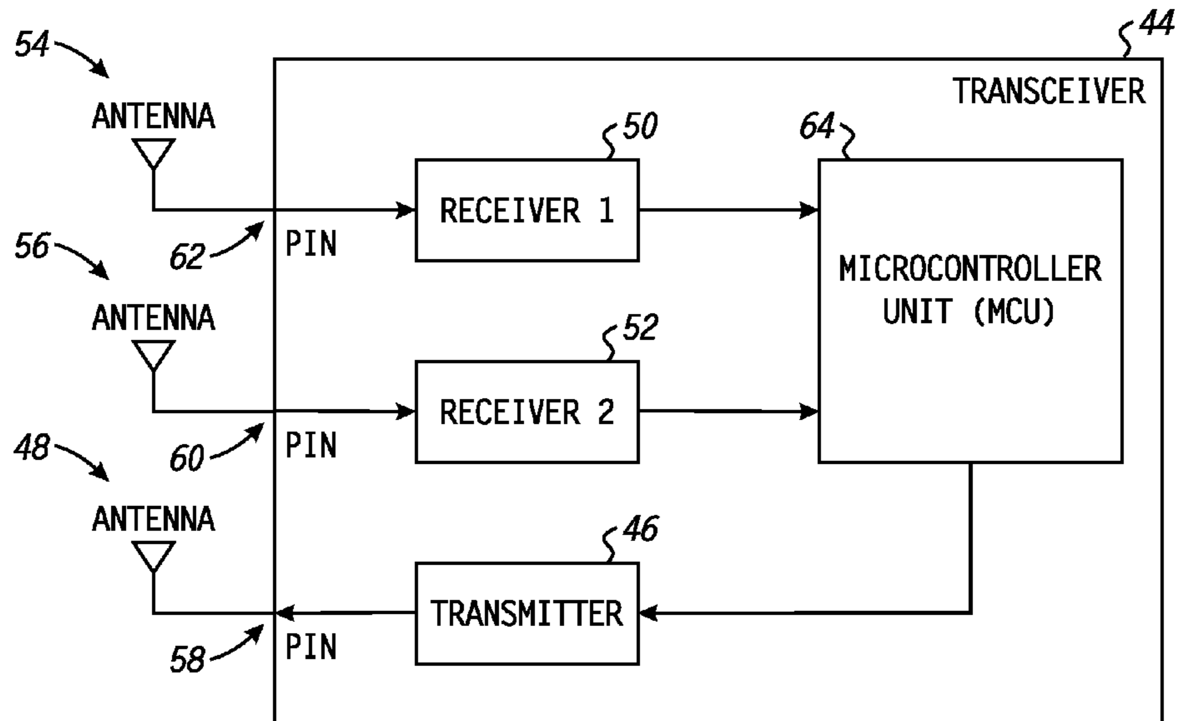
FIG. 3 (PRIOR ART)
