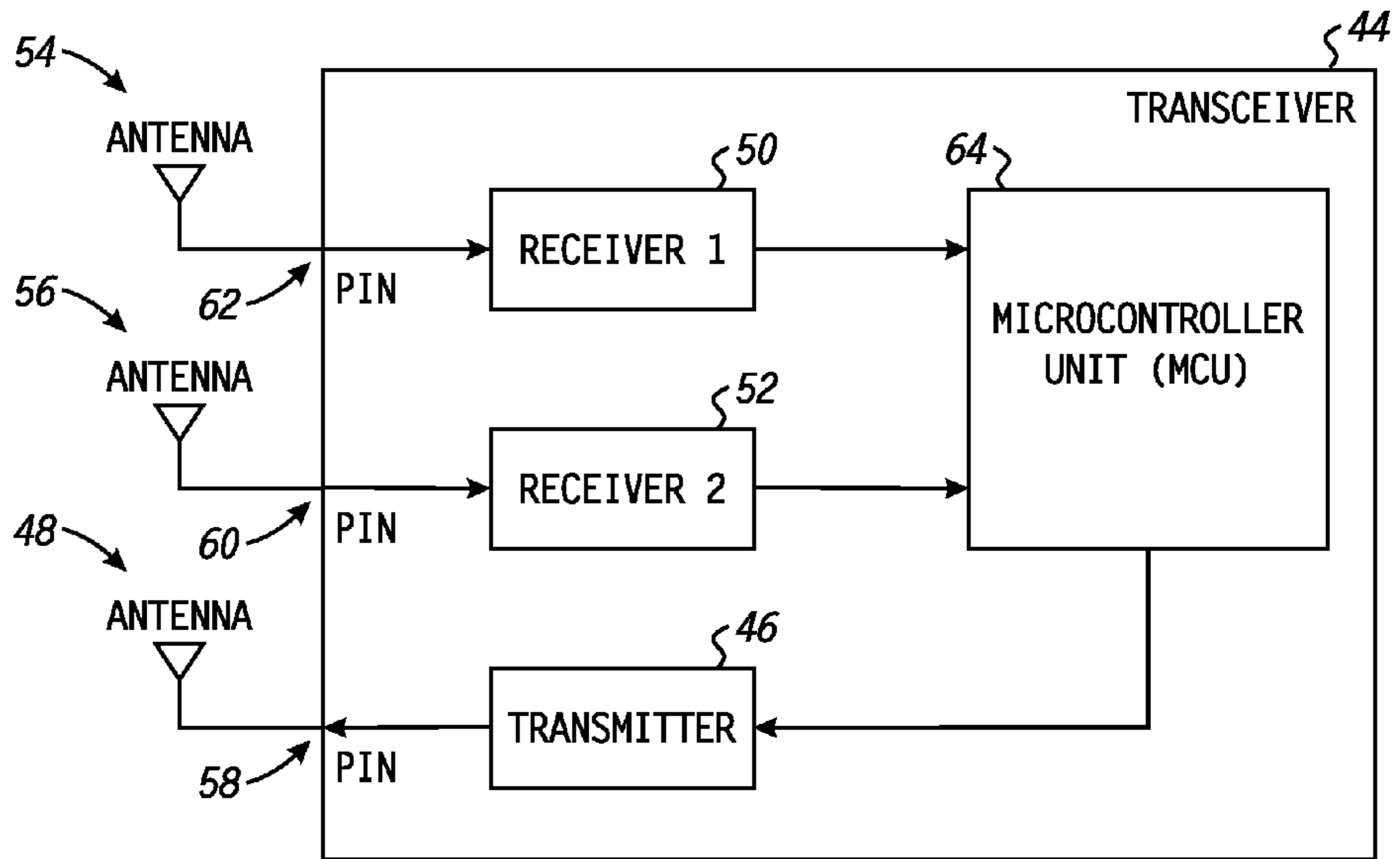
FIG. 3 (PRIOR ART)
