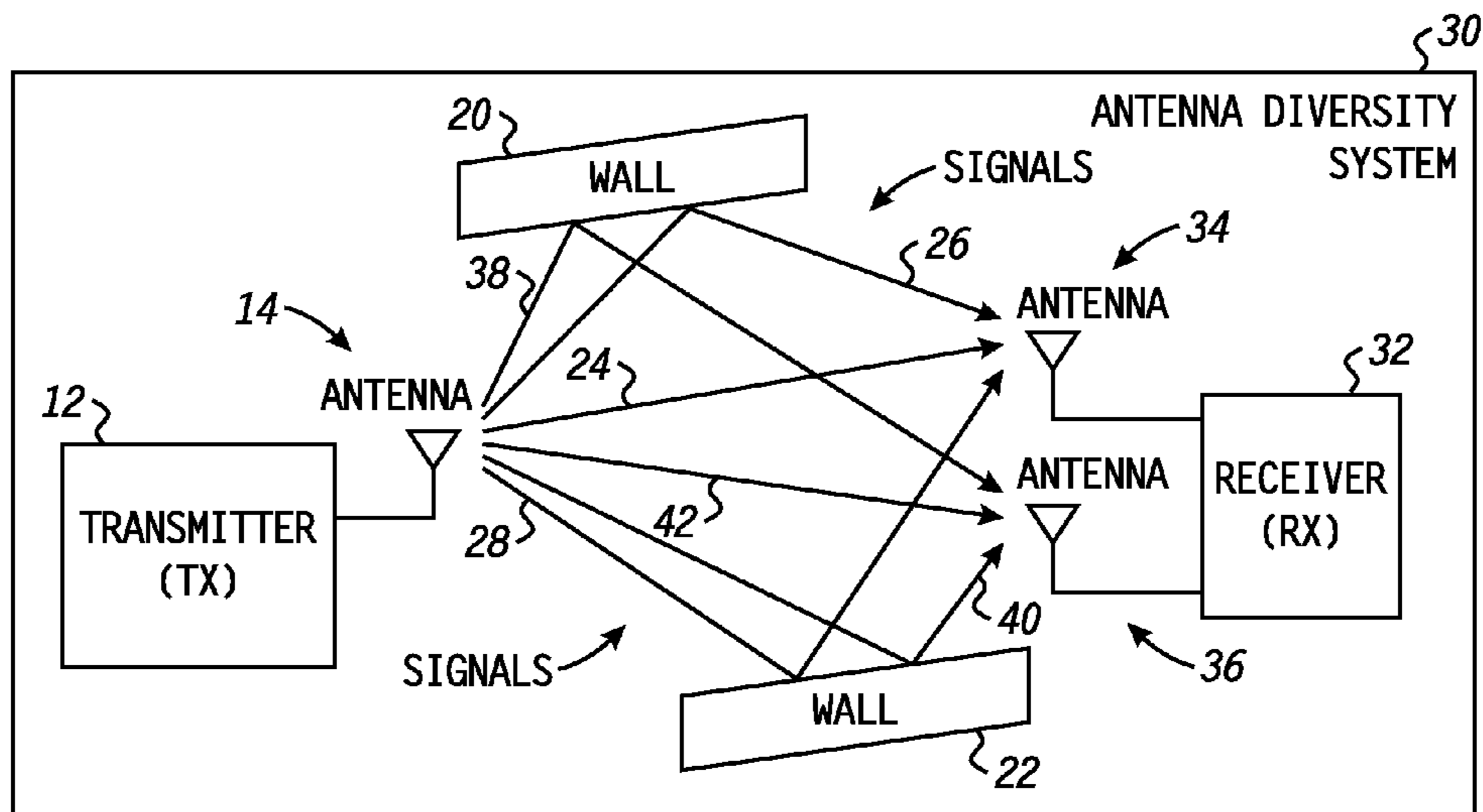
FIG. 2 (PRIOR ART)
