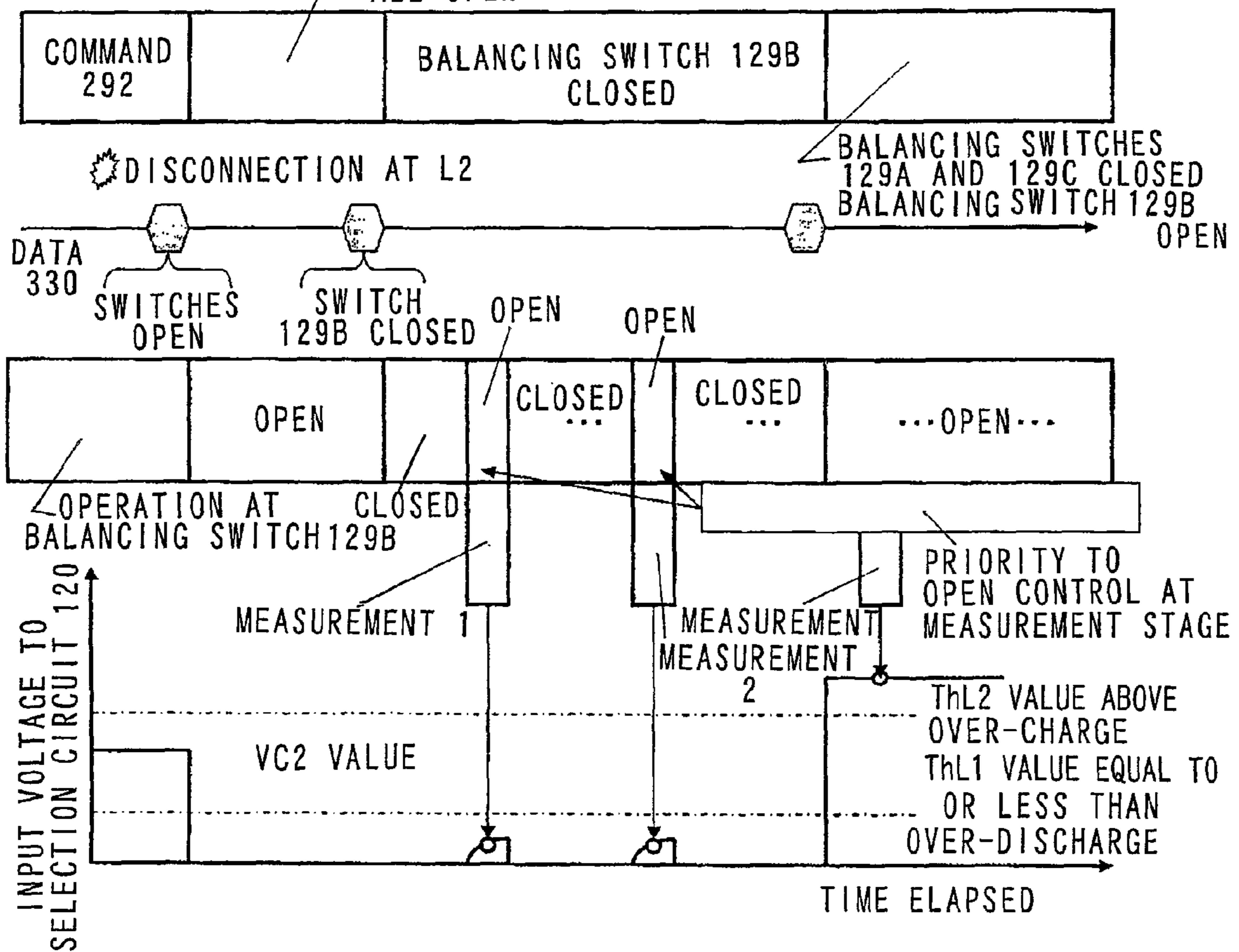
FIG.29 BALANCING SWITCHES 129 ALL OPEN
