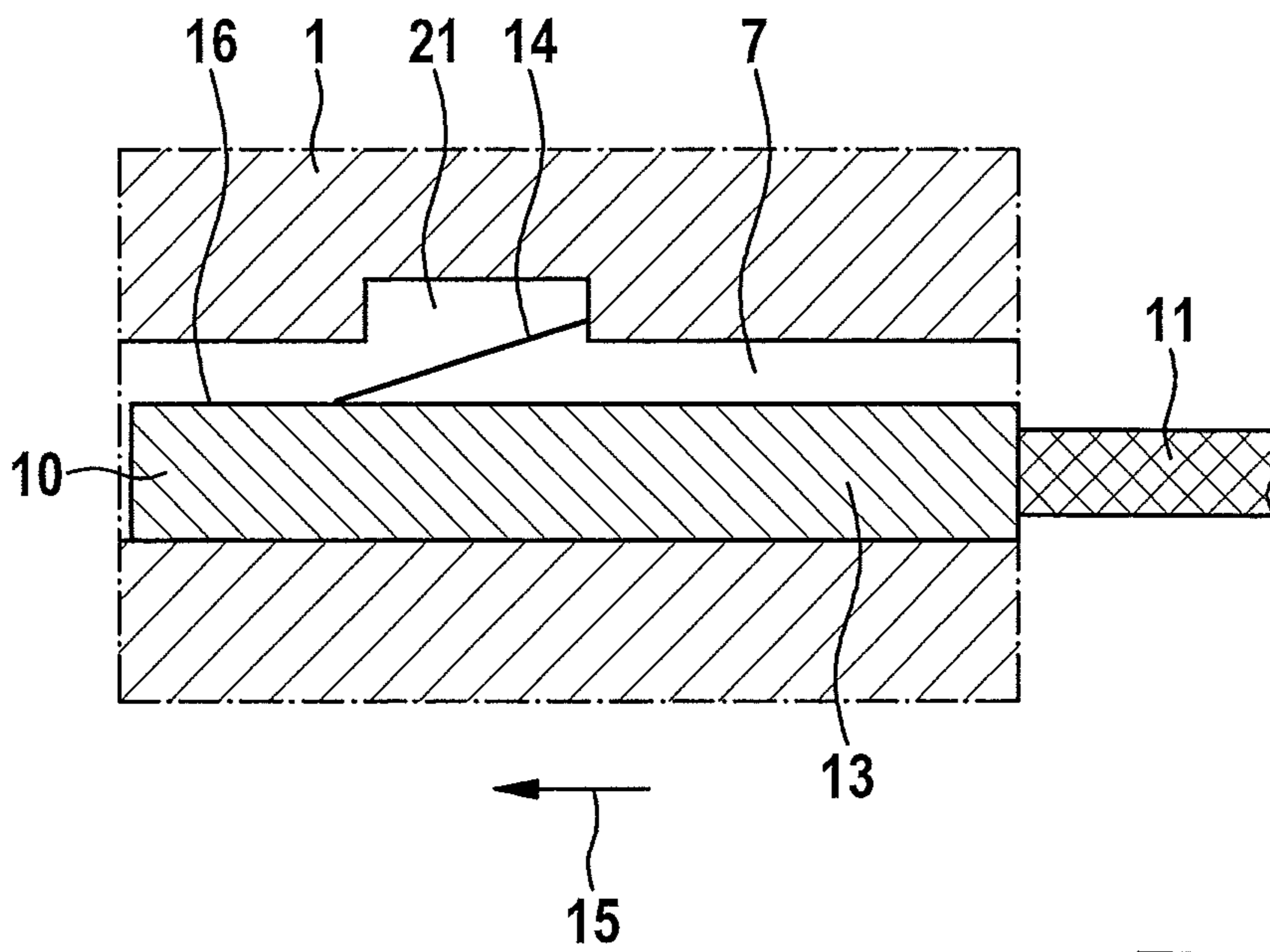
Fig. 3 Prior Art
