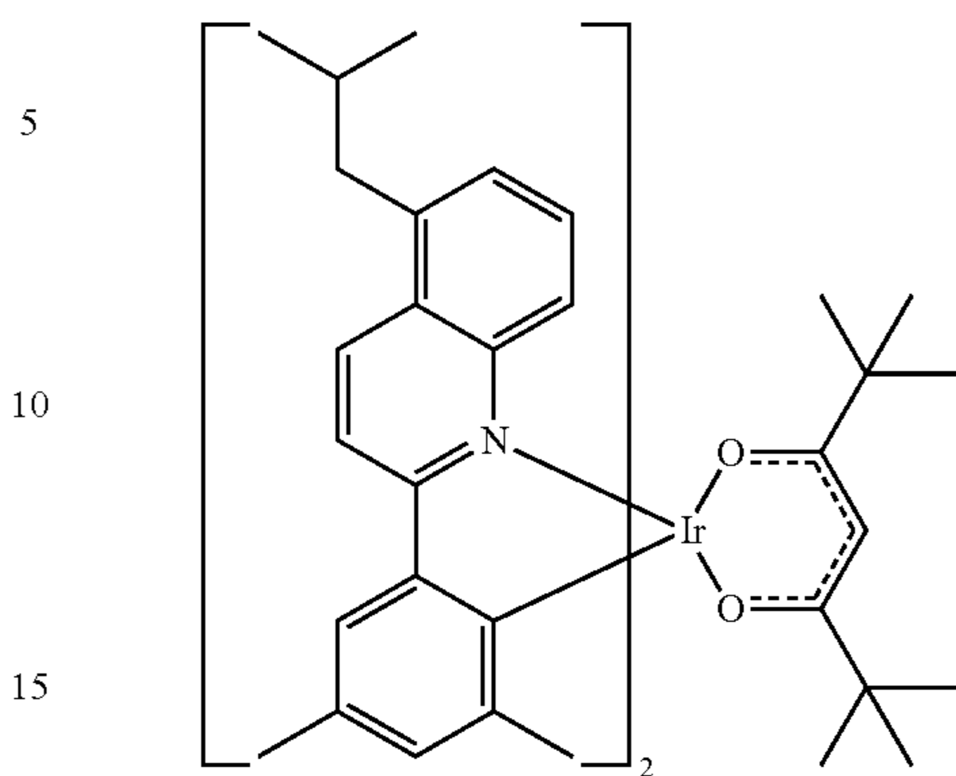
Compound 1
