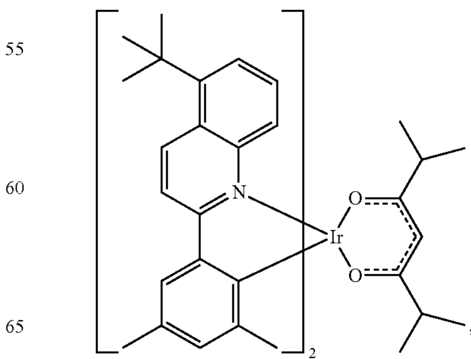
Compound 16
