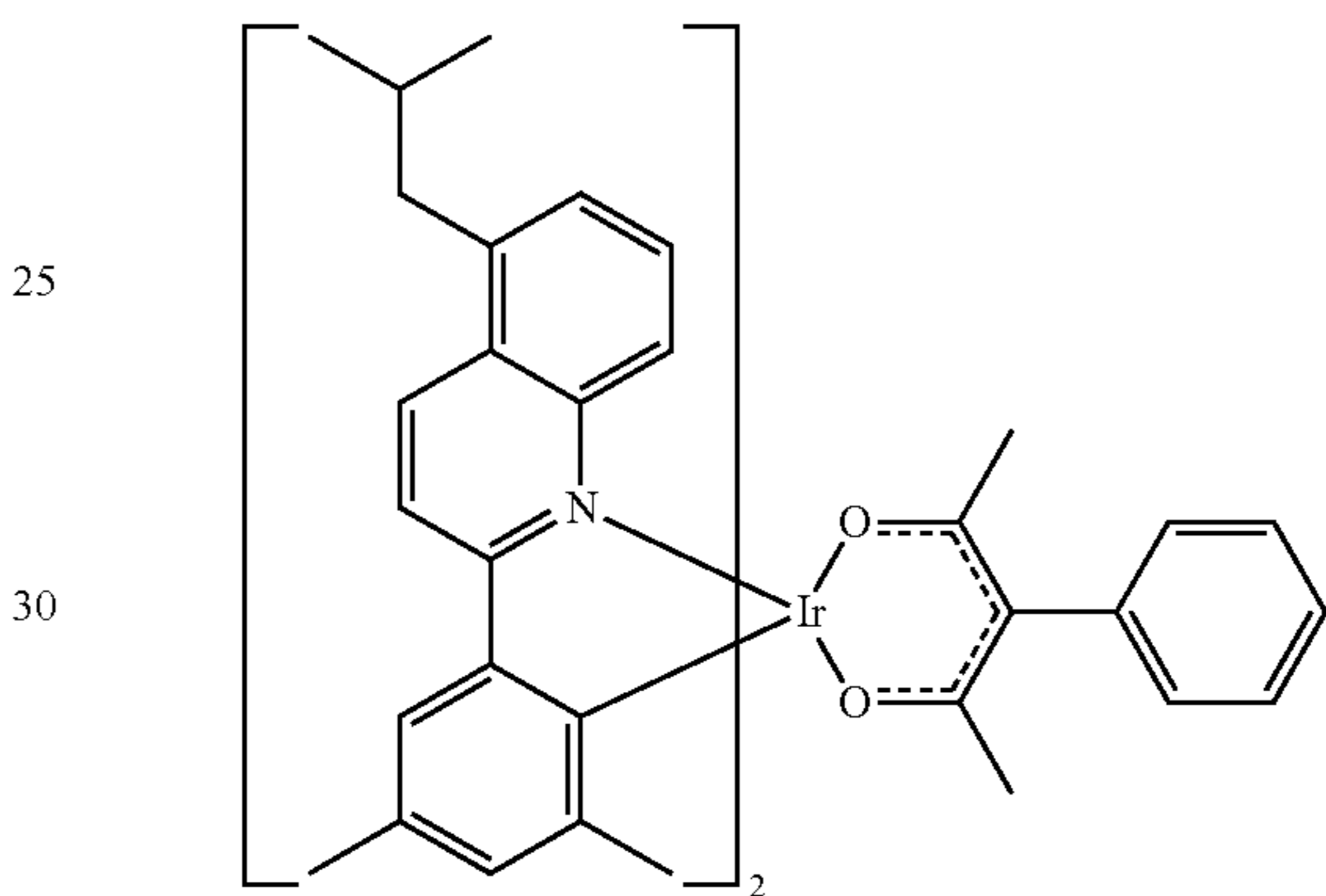
Compound 5
