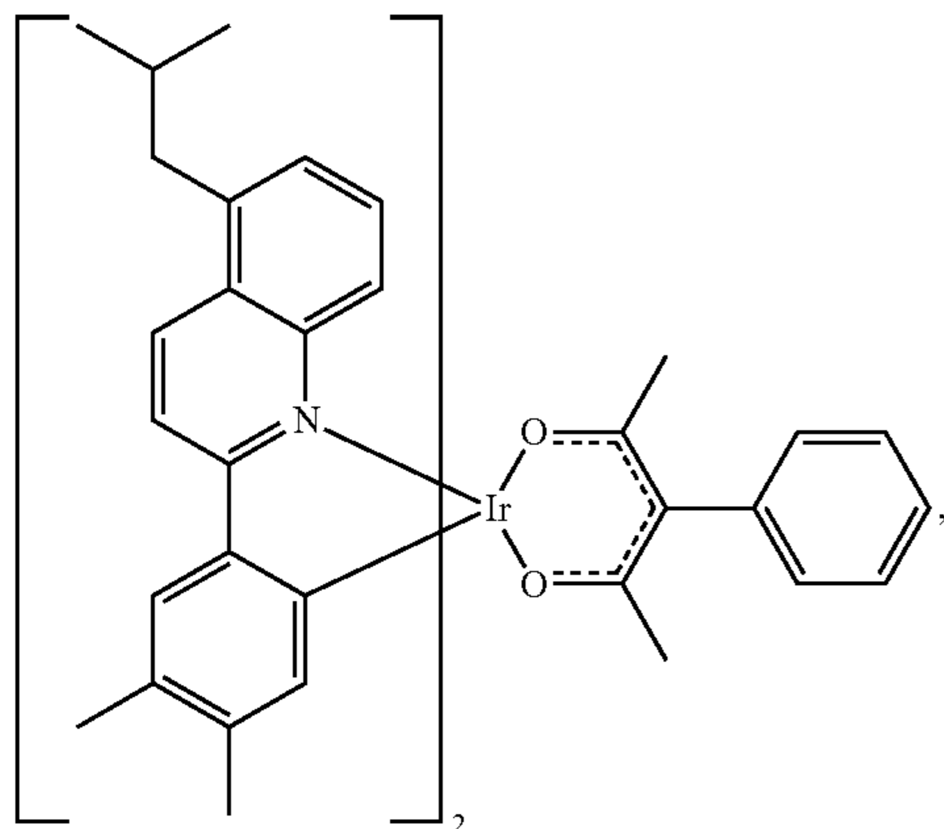
Compound 37
