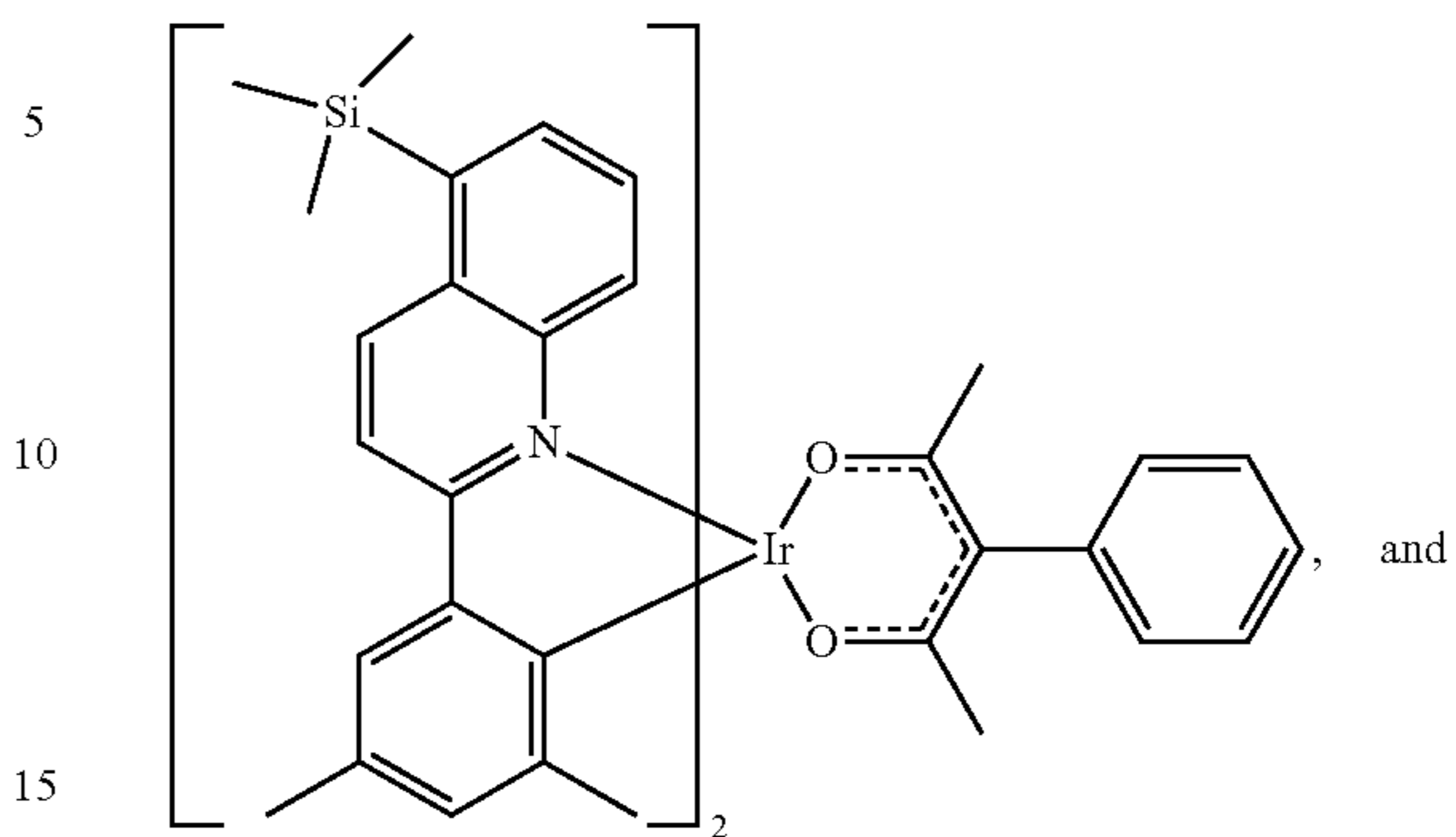
Compound 14
