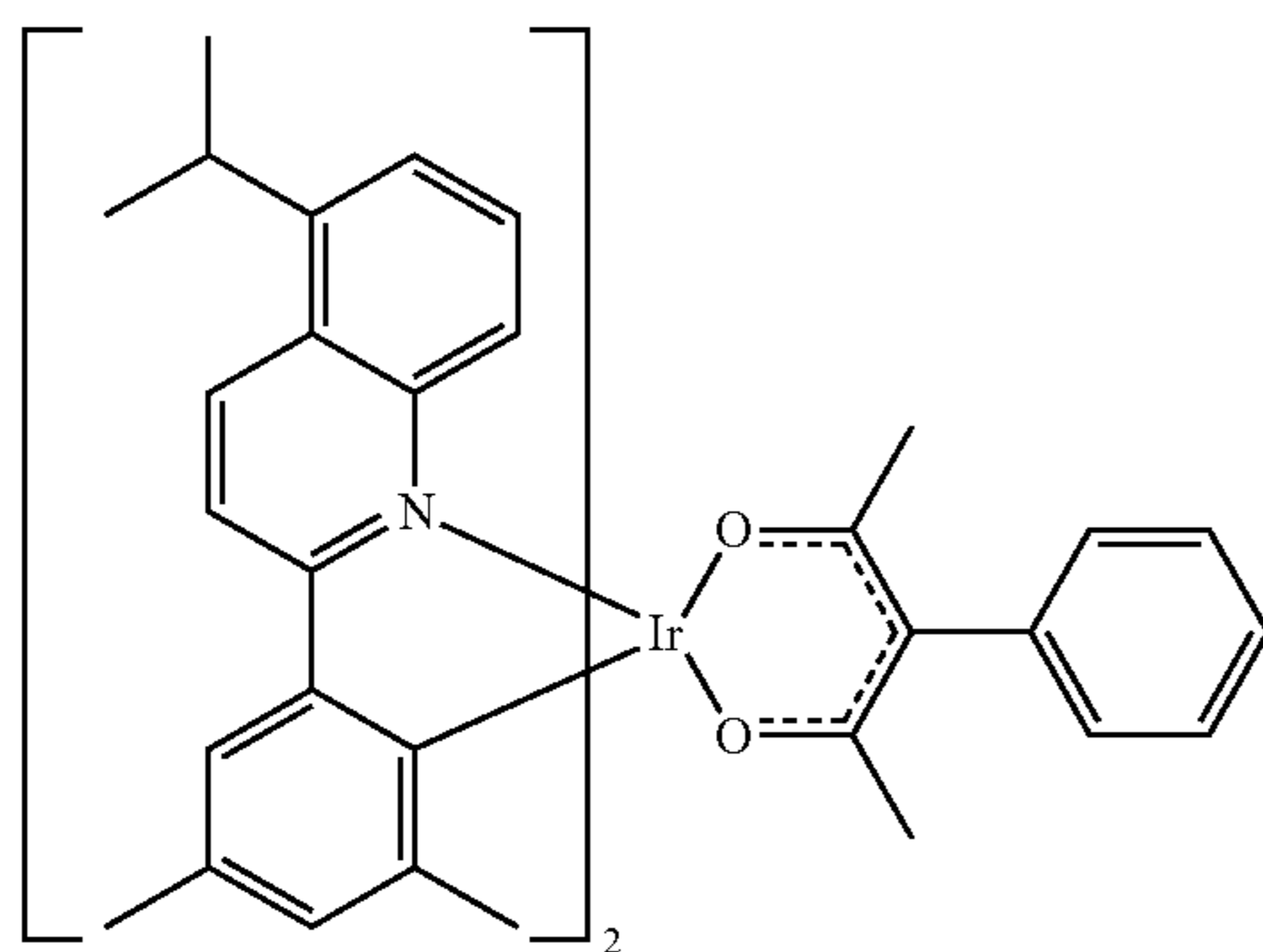
Compound 21
