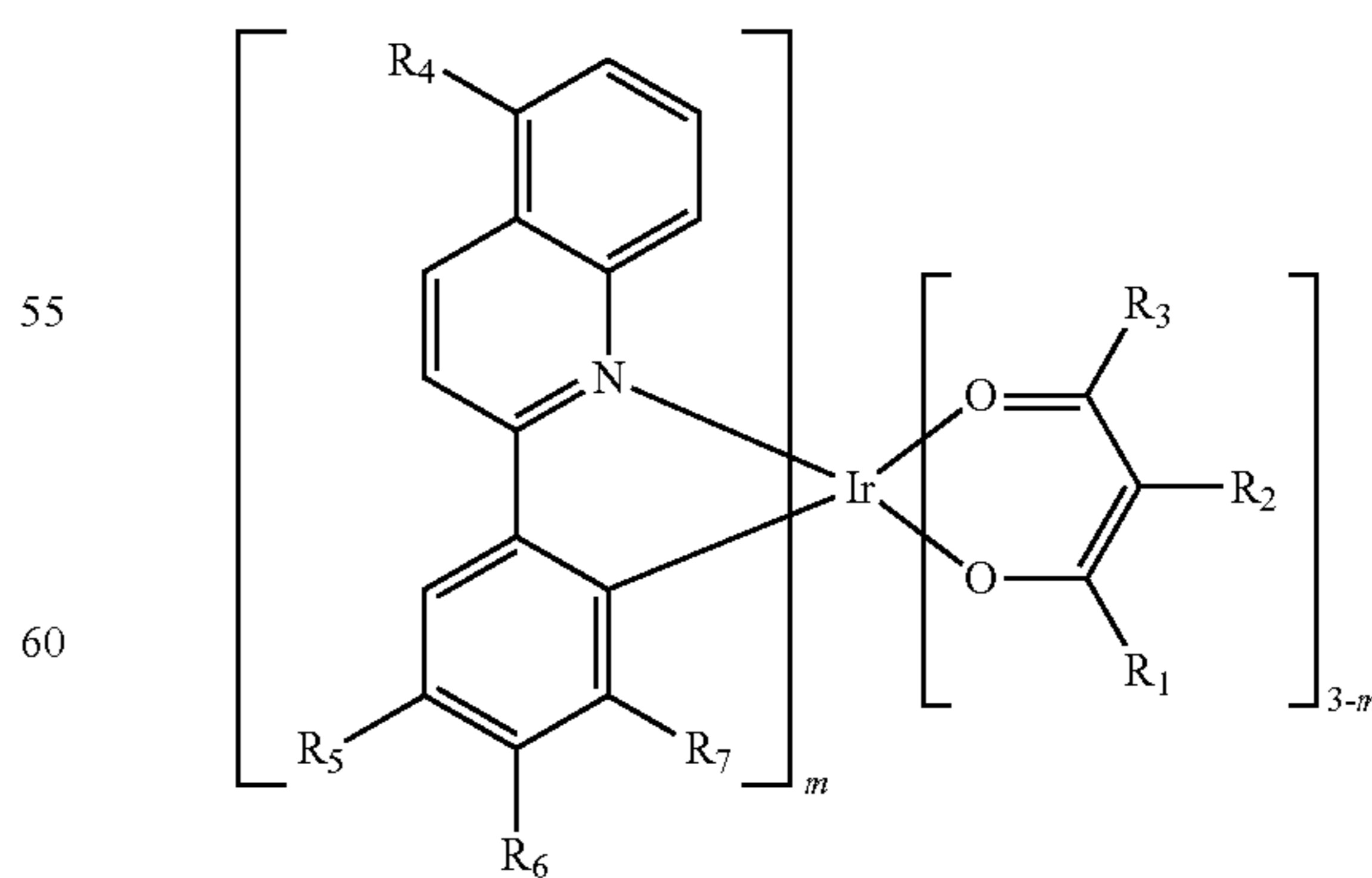
Formula III
