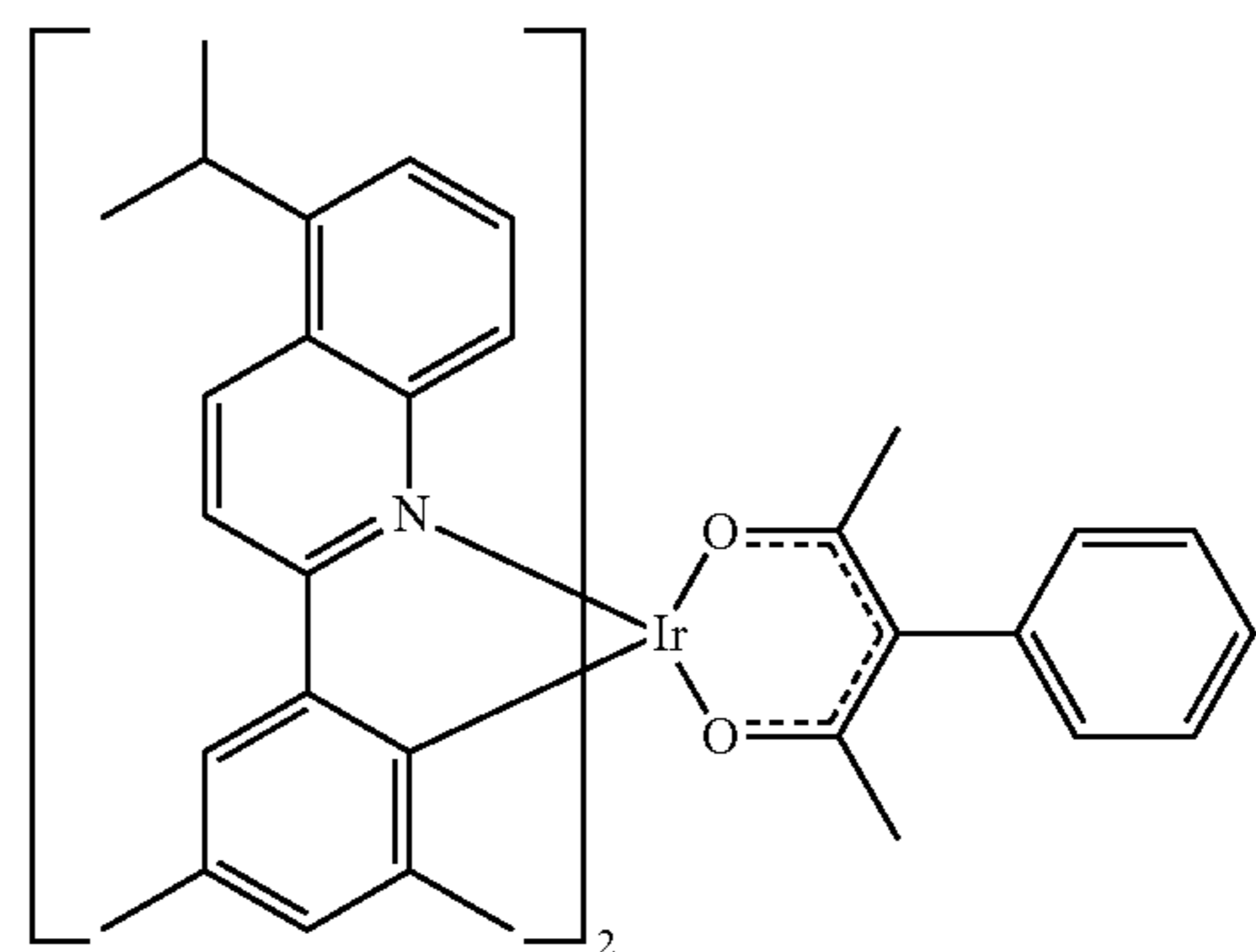
Compound 21
