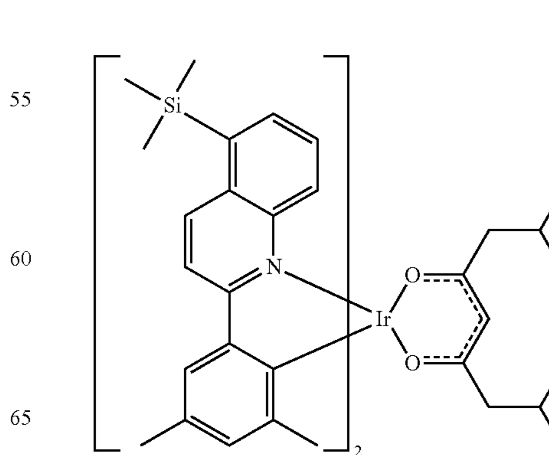
Compound 10
