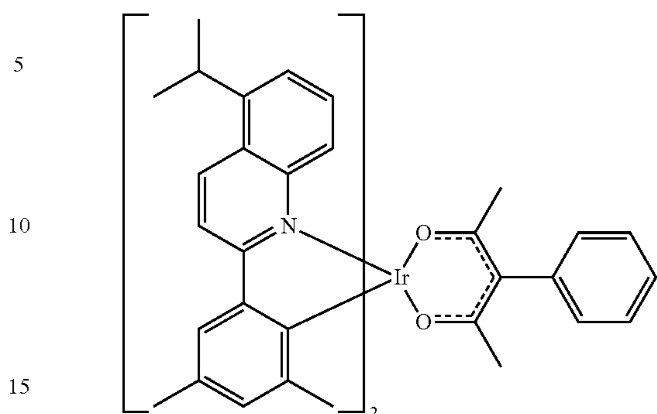
Compound 33
