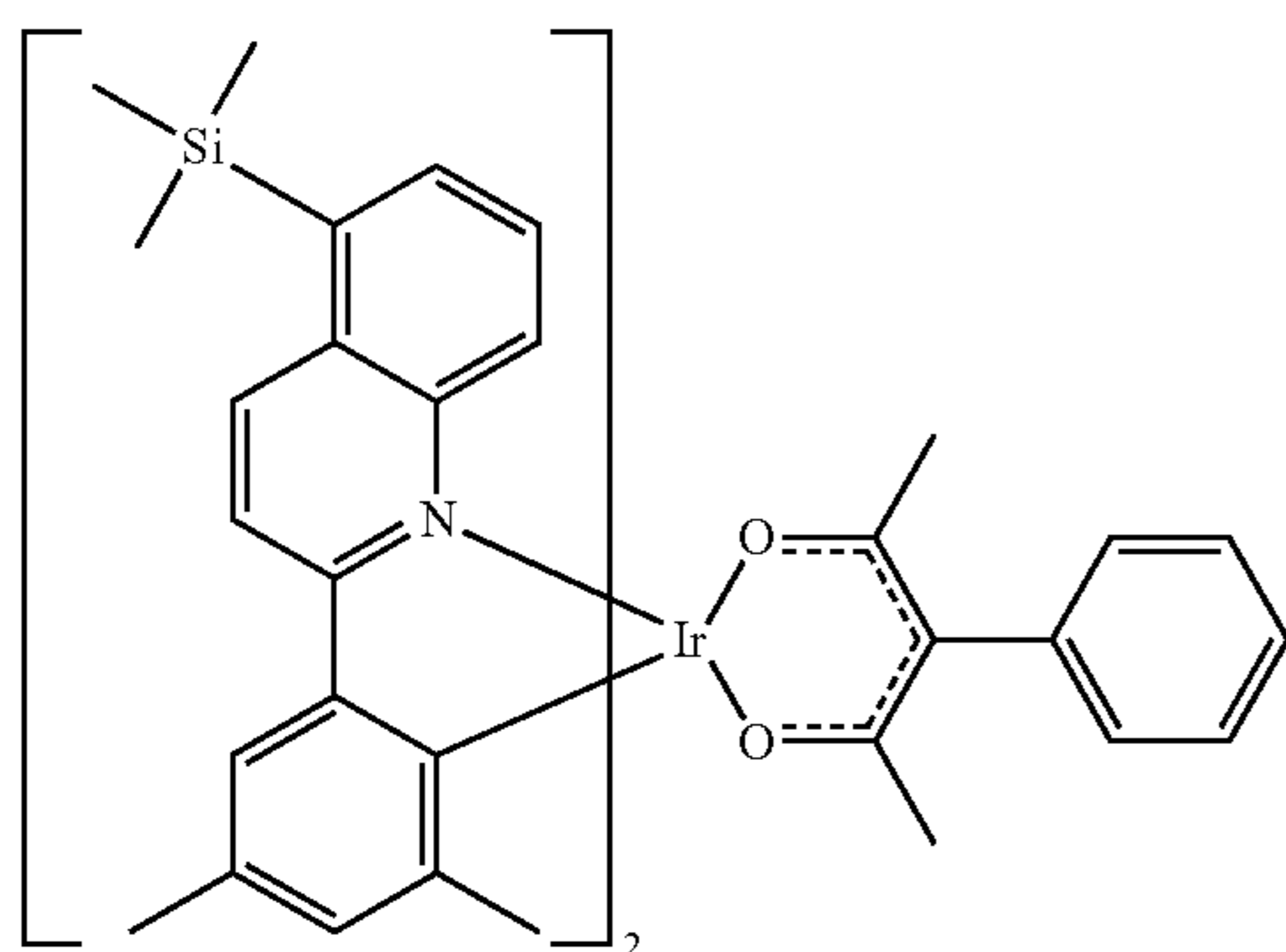
Compound 14
