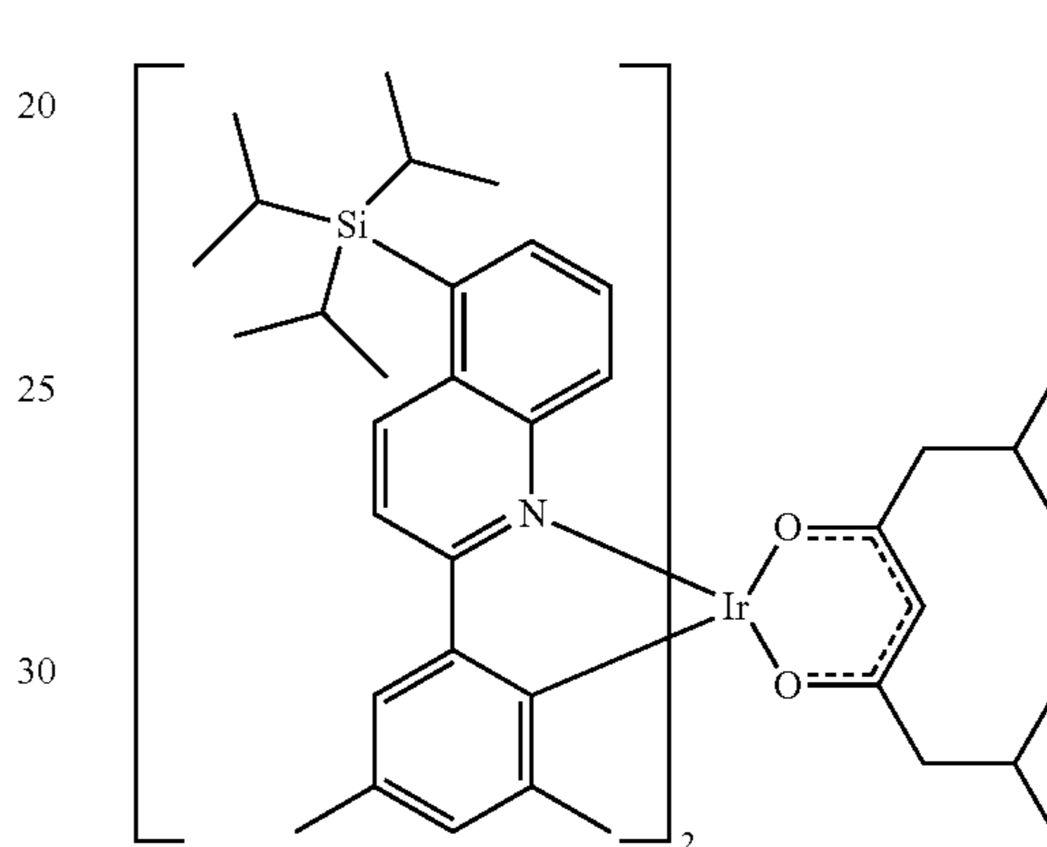
Compound 8
