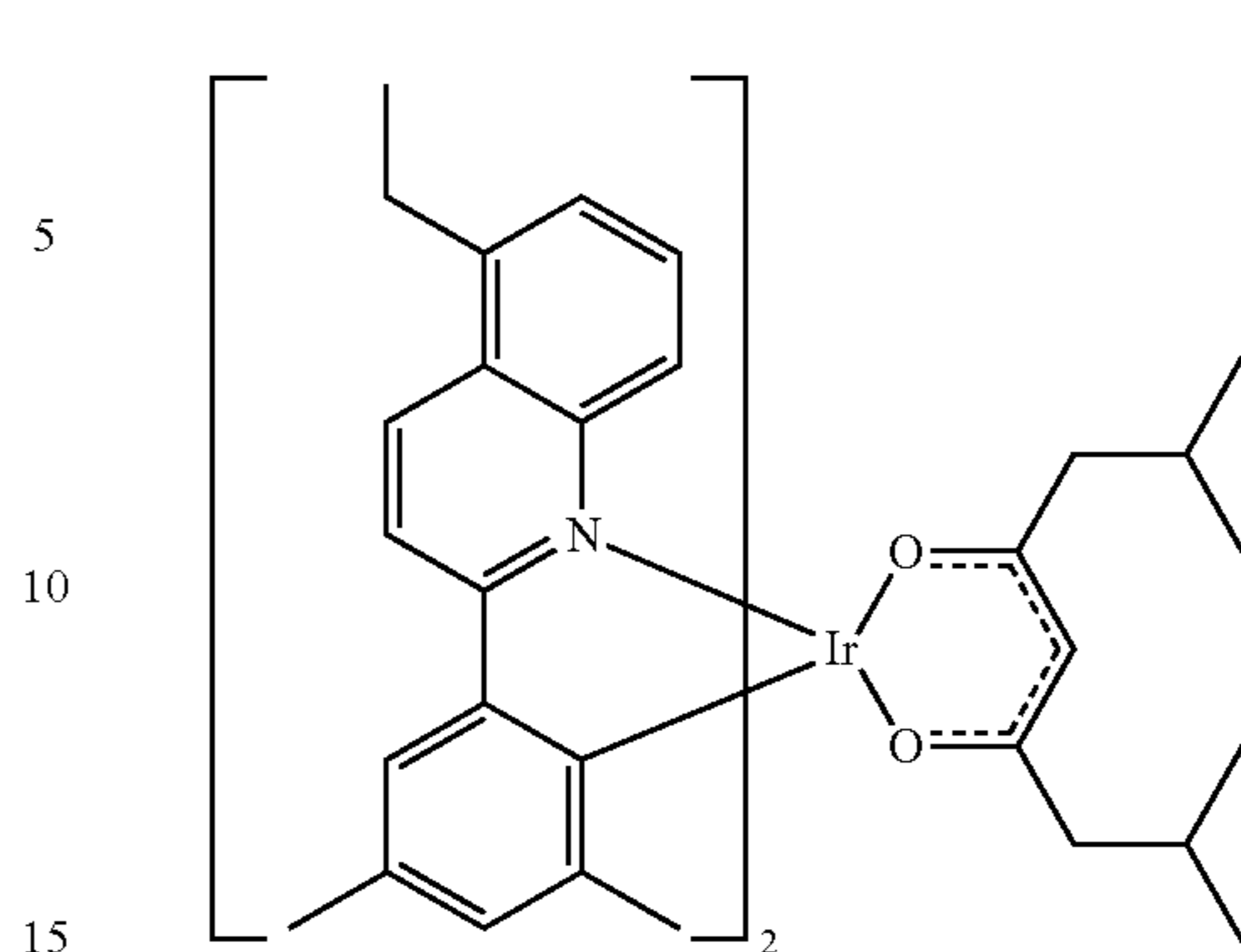
Compound 19
