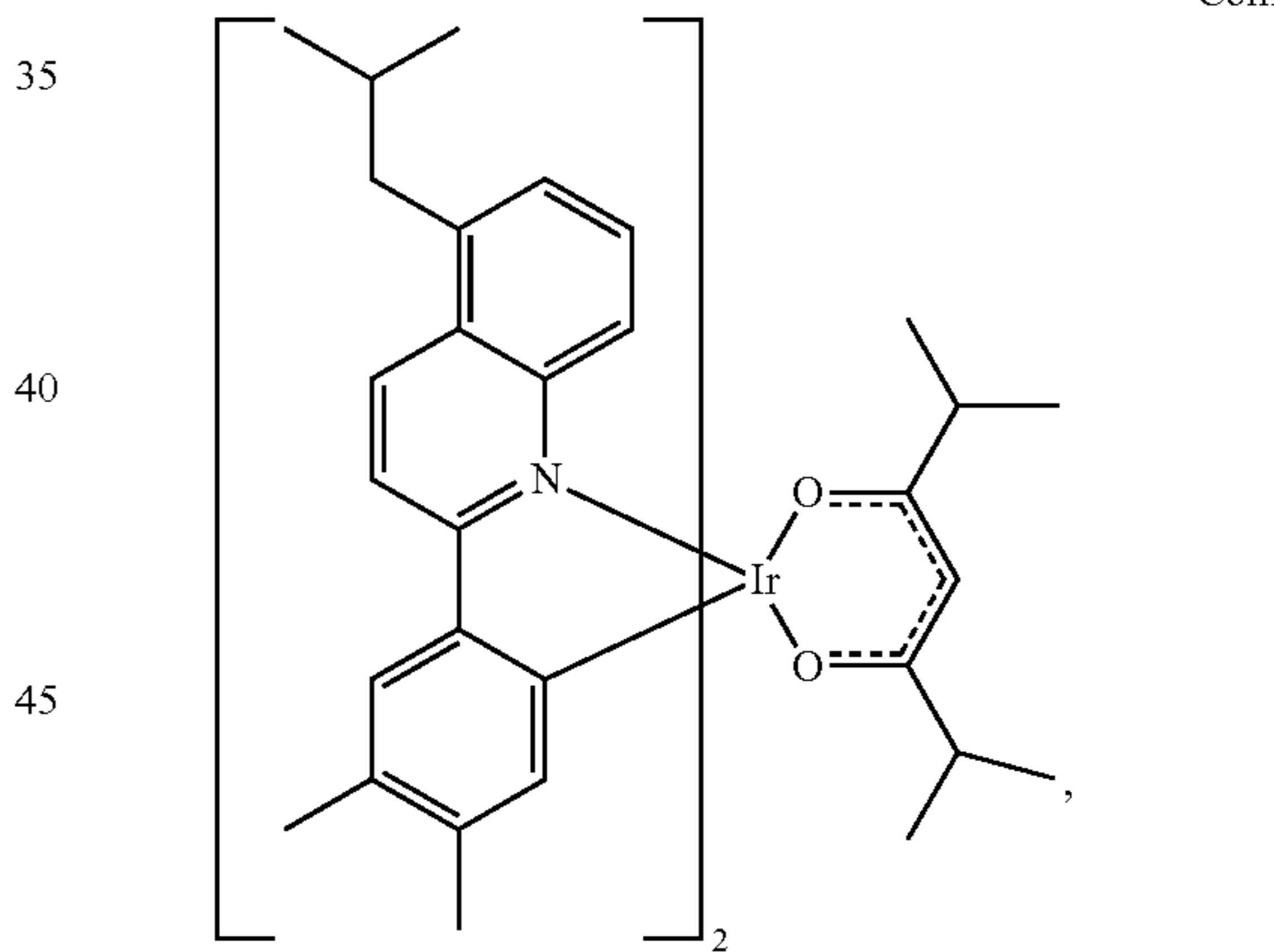
Compound 37
