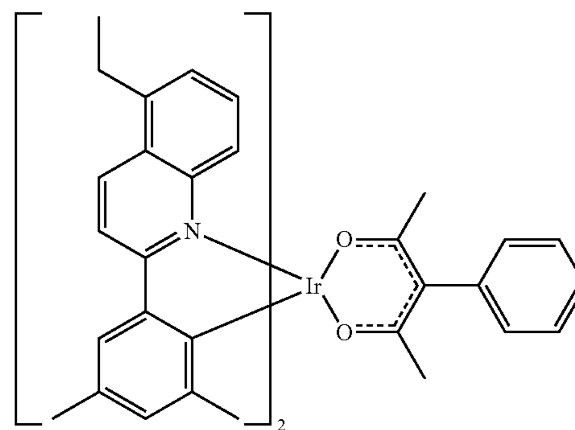
Compound 25
