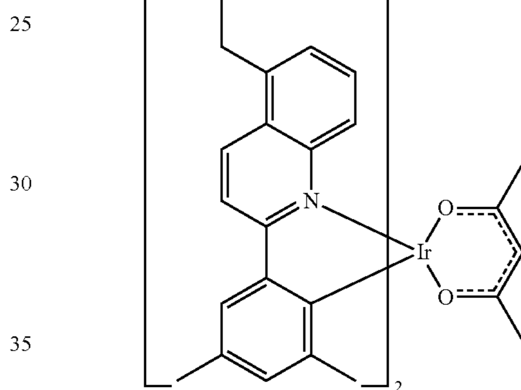
Compound 41
