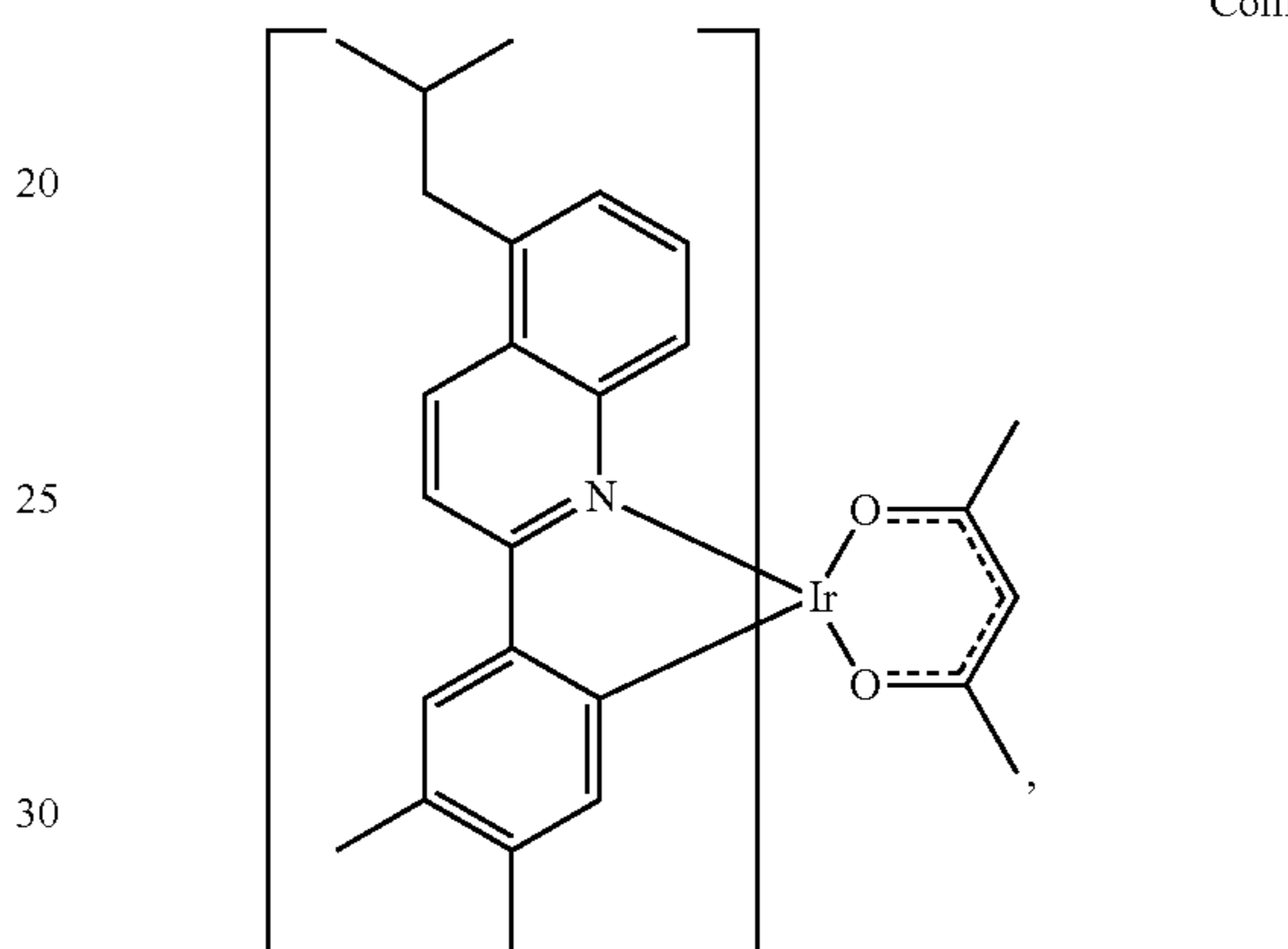
Compound 35
