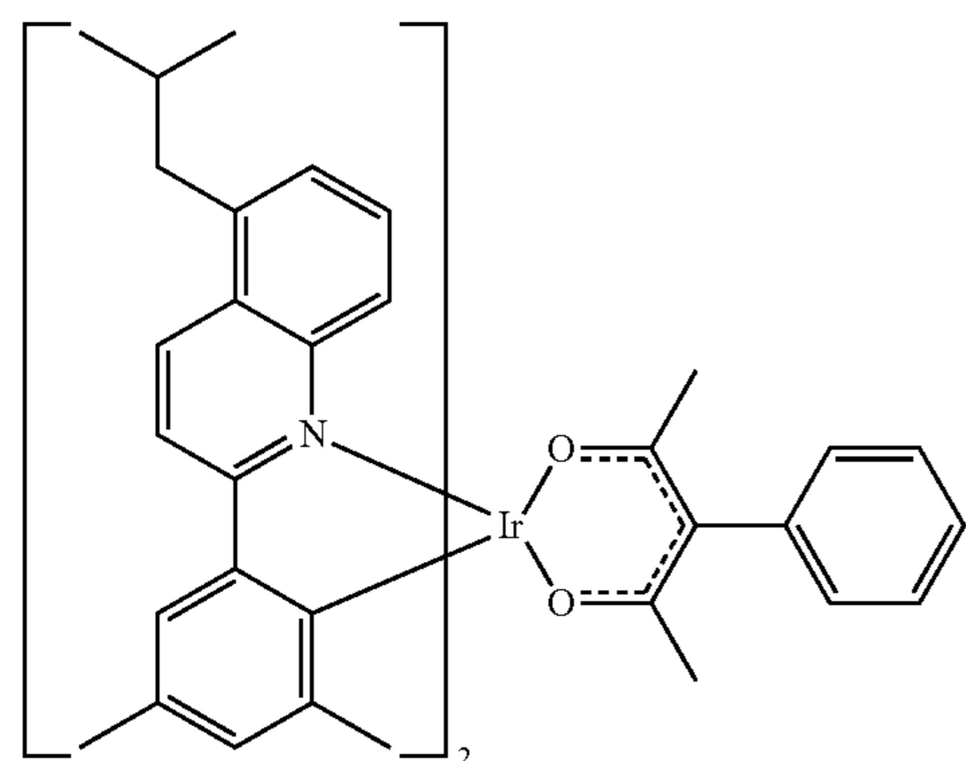
Compound 5
