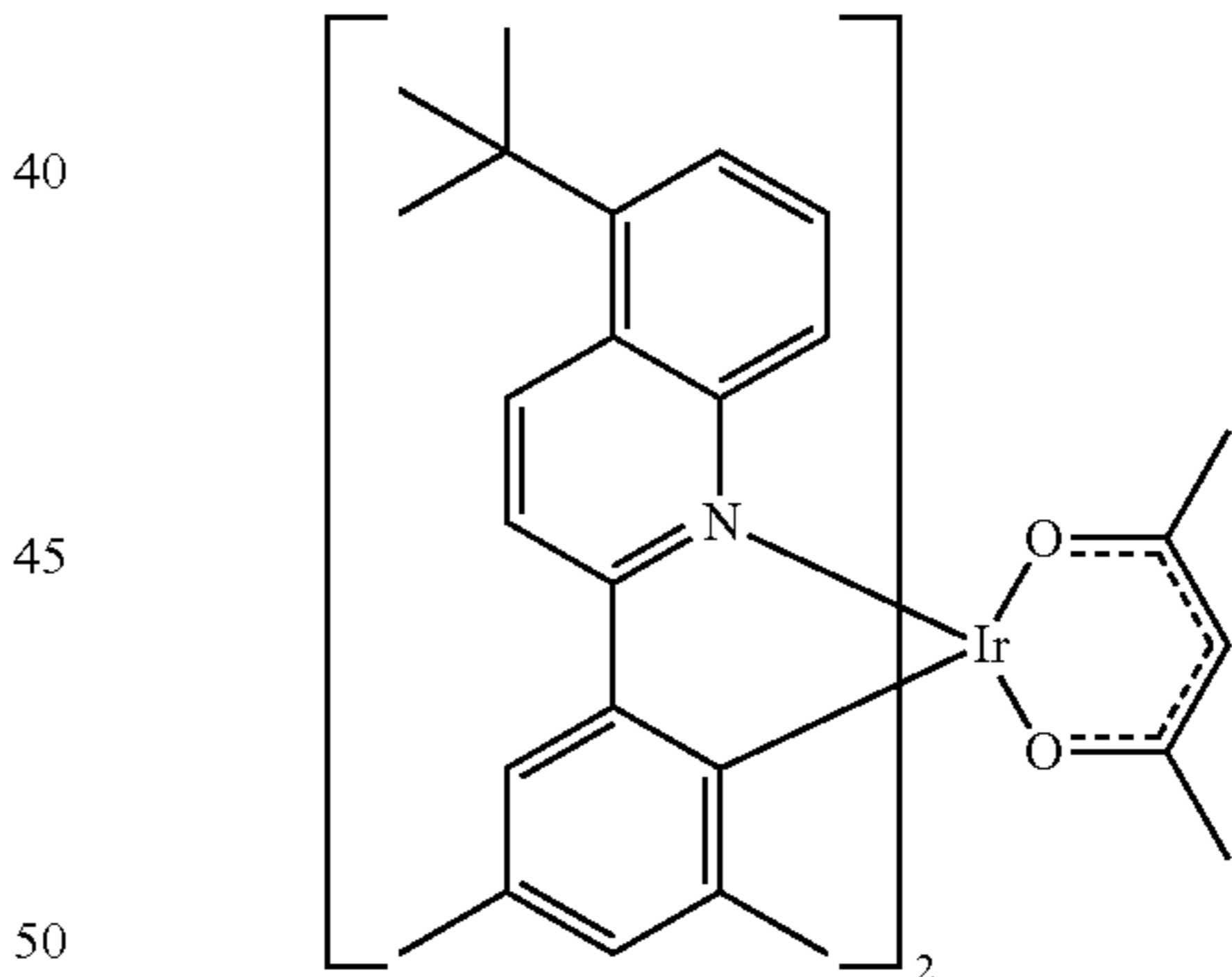
Compound 15
