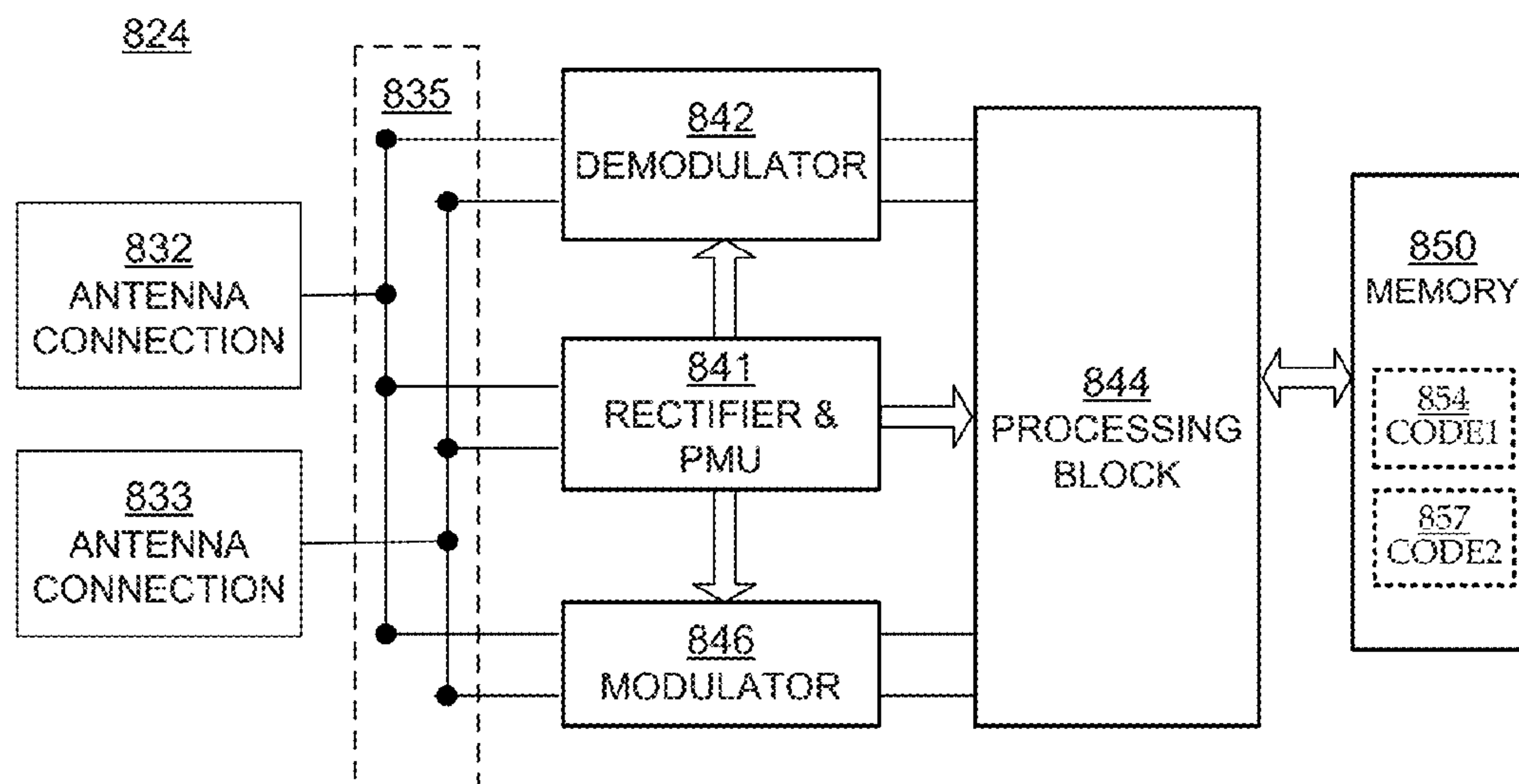
RFID TAG COMPONENTS
