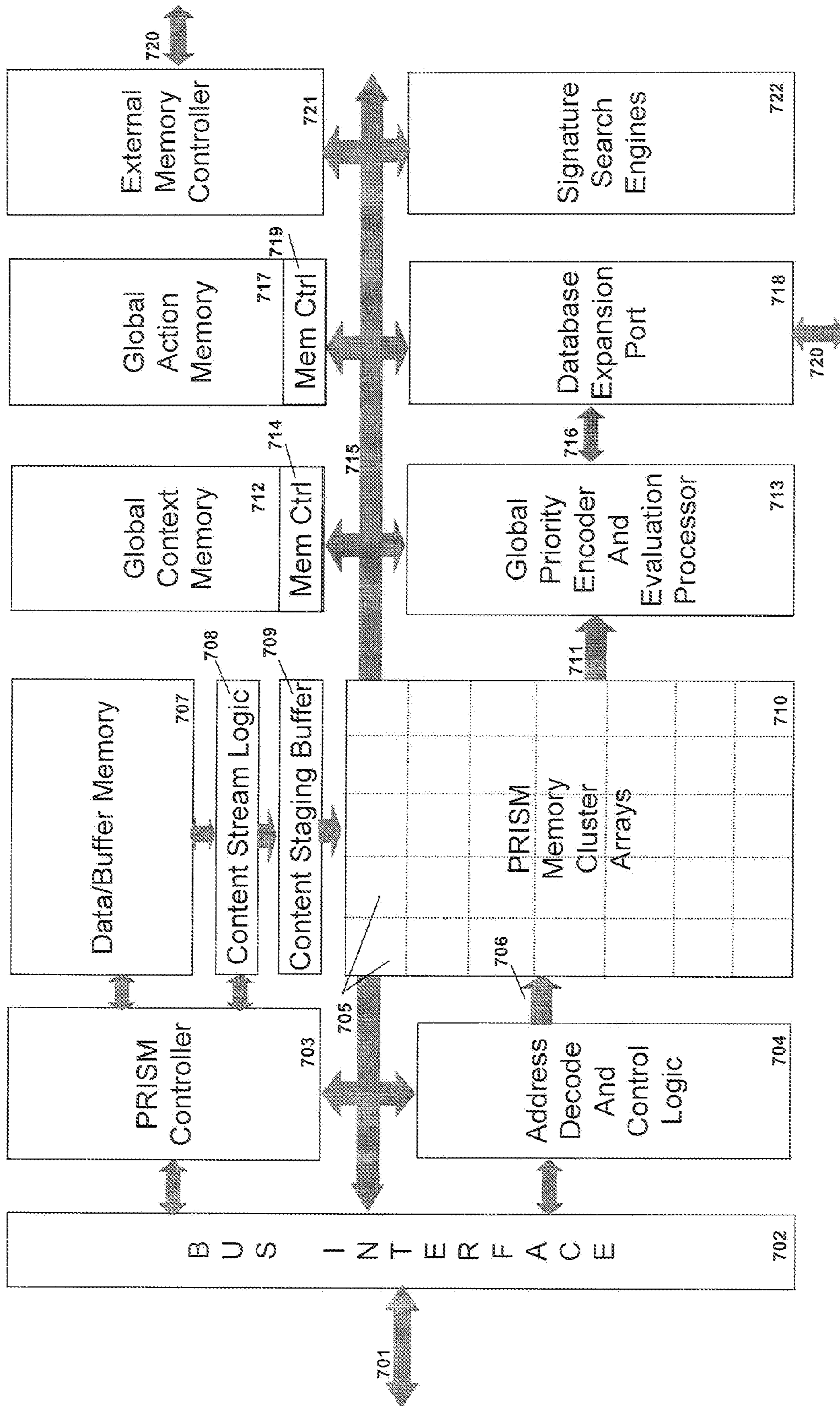
Fig. 7 PRISM Block Diagram
