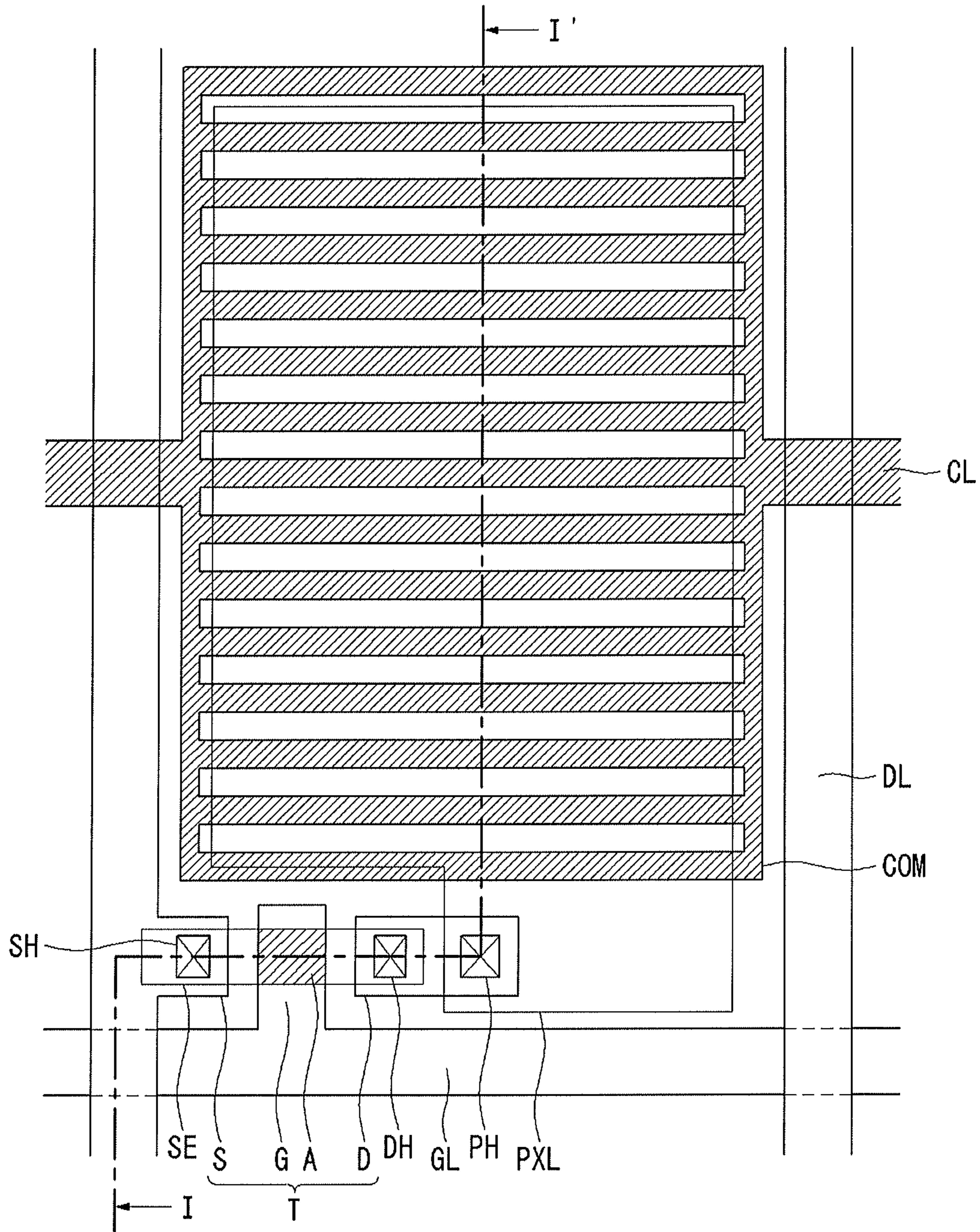
FIG. 1 Related Art
