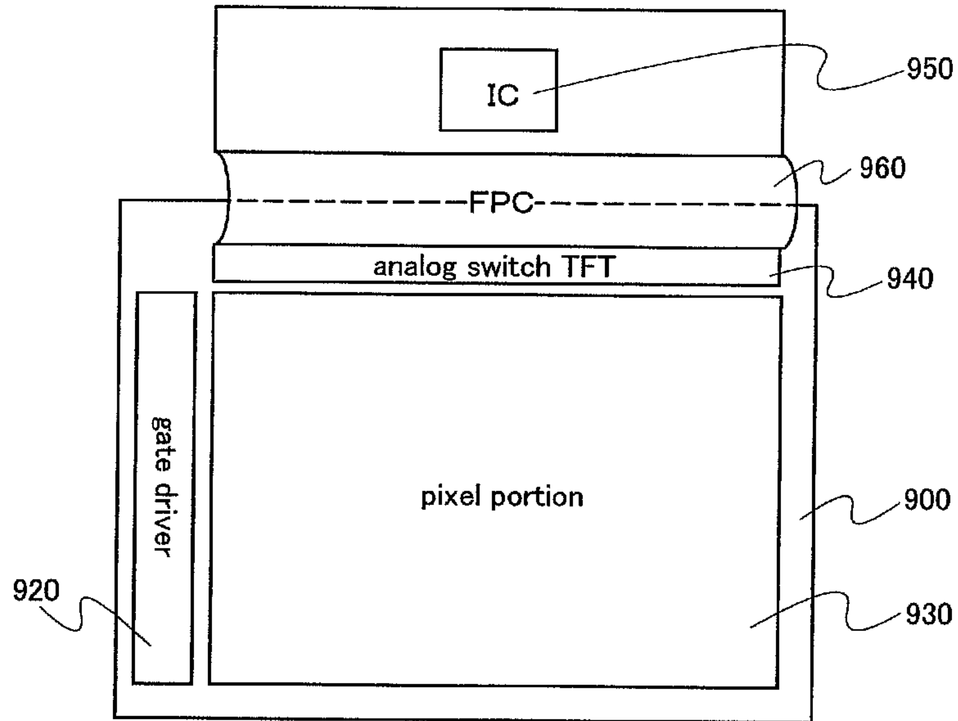
FIG. 17A IC connected by FPC
