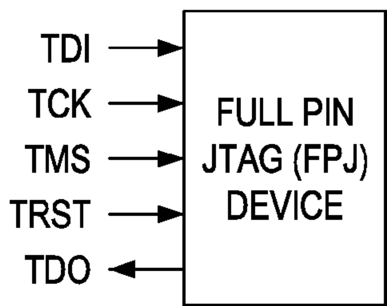
FIG. 1 (PRIOR ART)
