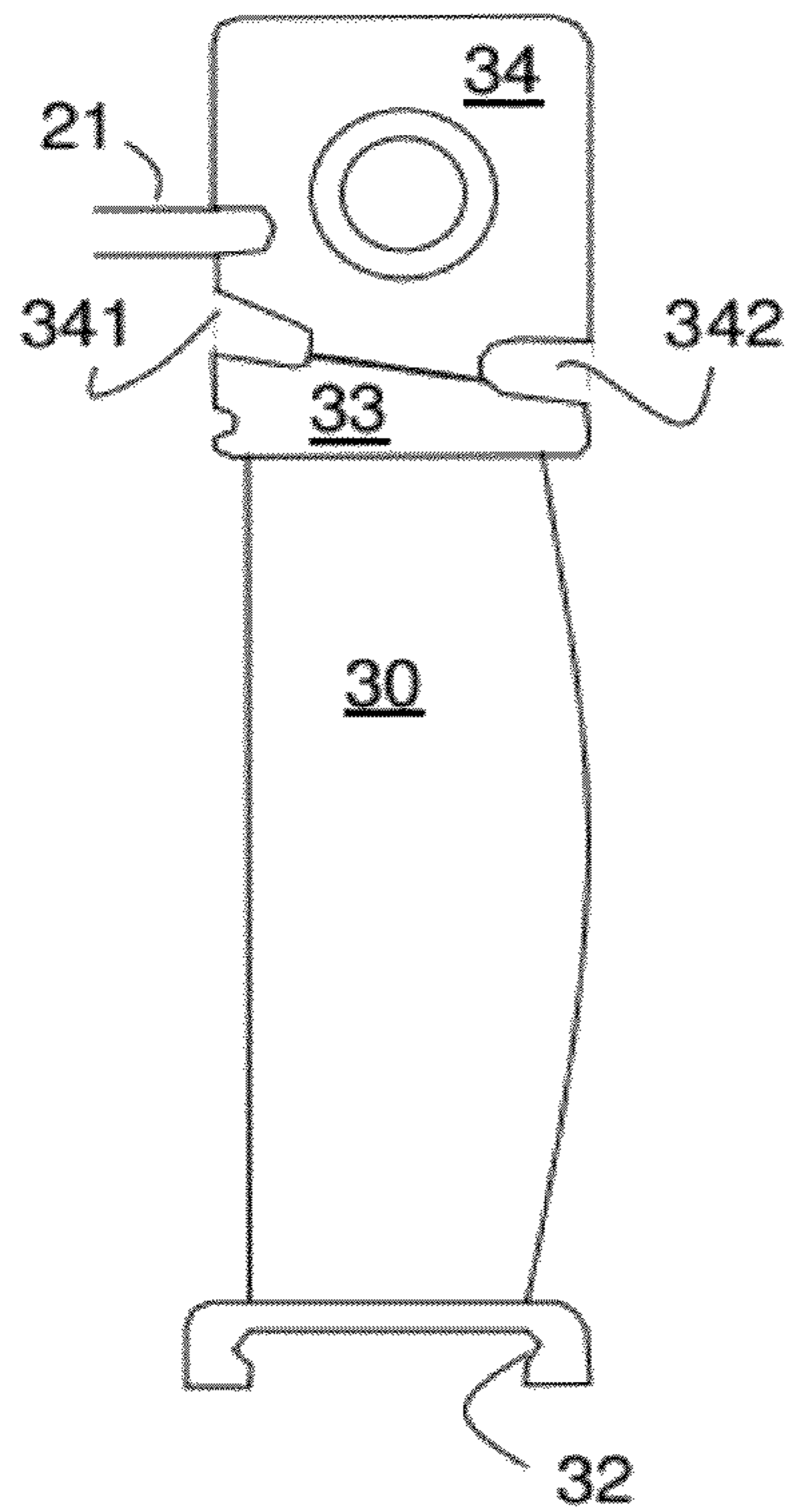
FIG. 2(Prior Art)
