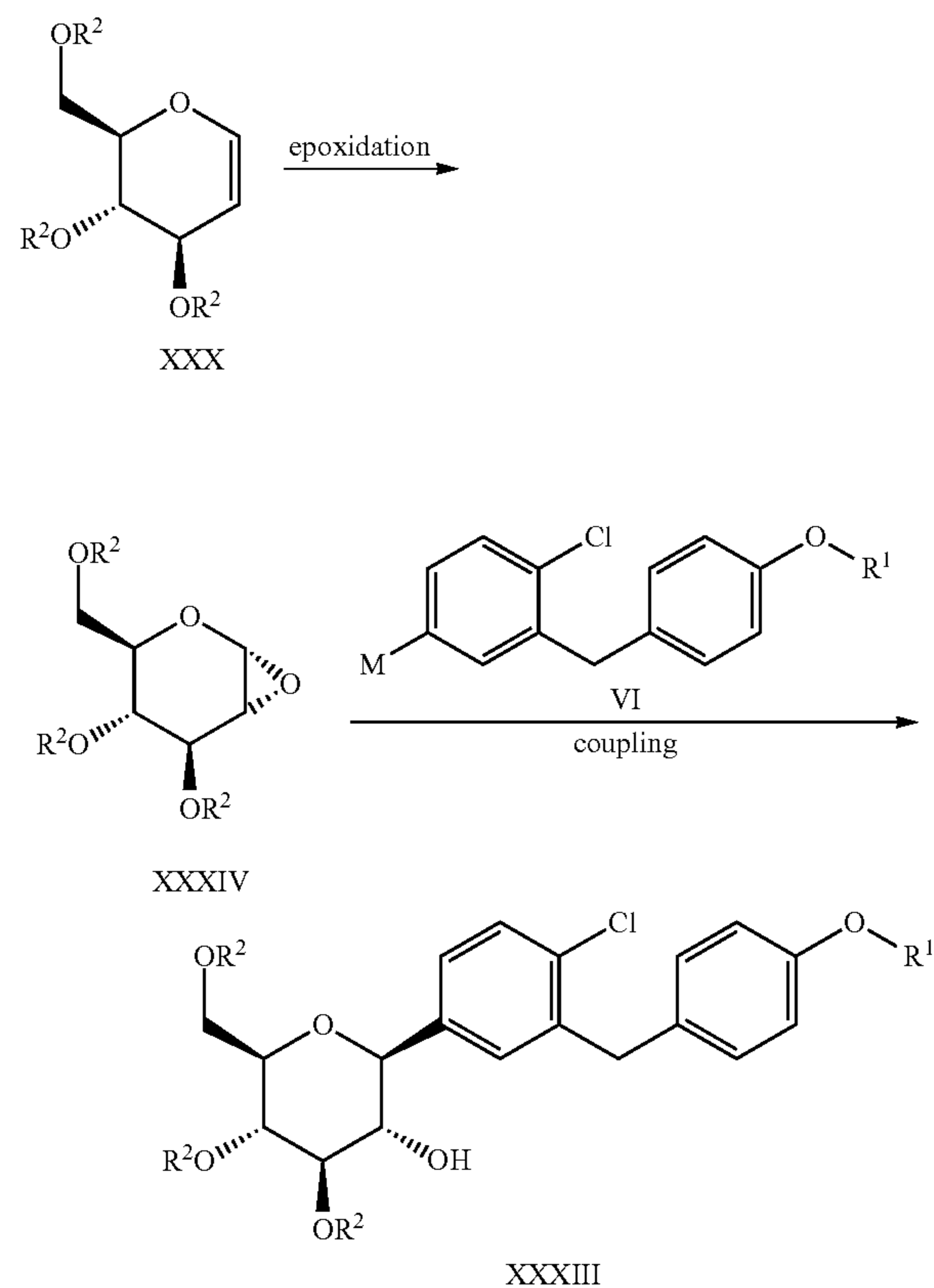
Scheme 2c: Synthesis of C-Glucosides - Approach 3
