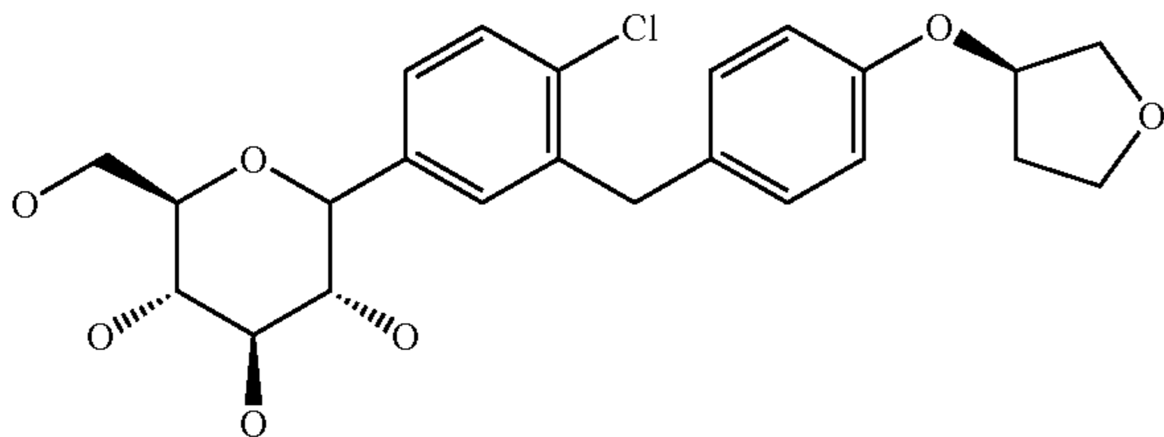
1-Chloro-4-(β-D-glucopyranos-1-yl)-2-(4-(R)-tetrahydrofuran-3-yloxy-benzyl)-benzene
