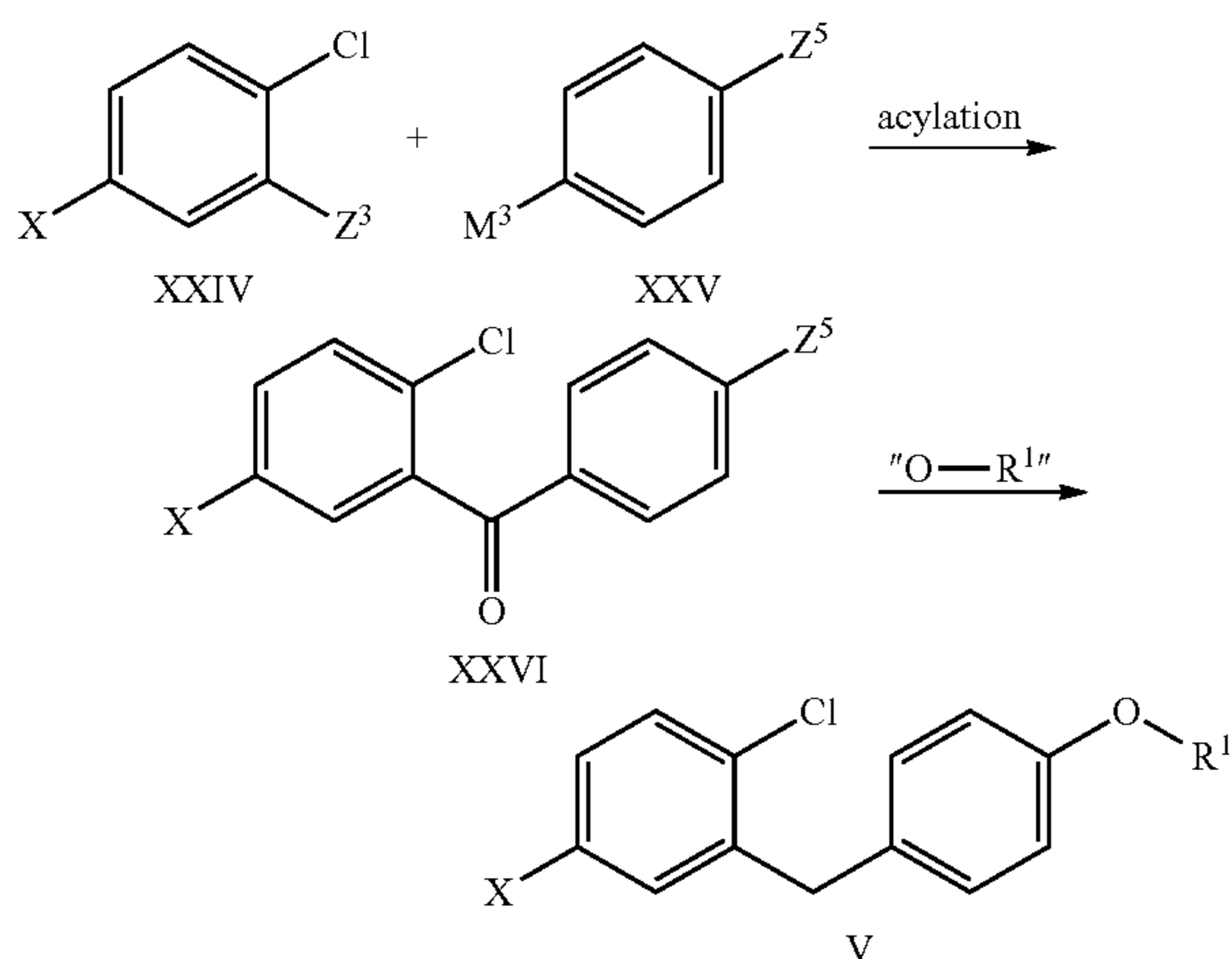
Scheme 10: Synthesis of Aglycon V - Approach 8
