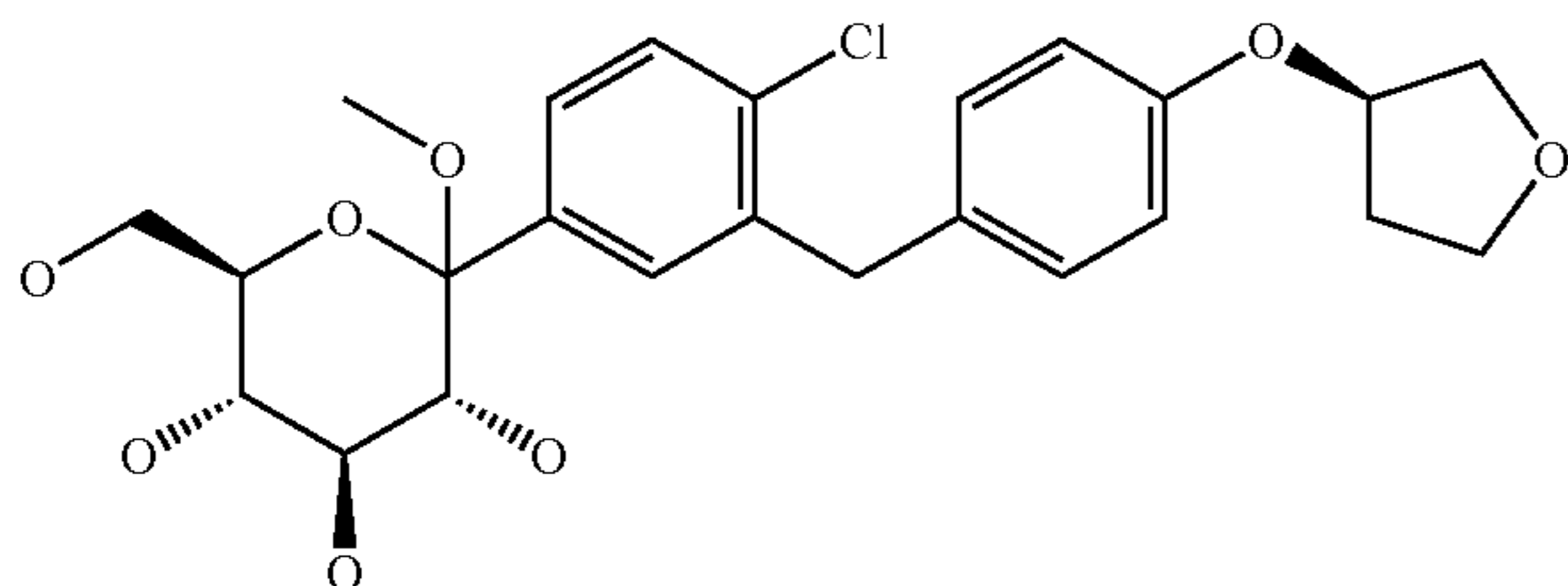
1-Chloro-4-(1-methoxy-D-glucopyranos-1-yl)-2-(4-(R)-tetrahydrofuran-3-yloxy-benzyl)-benzene
