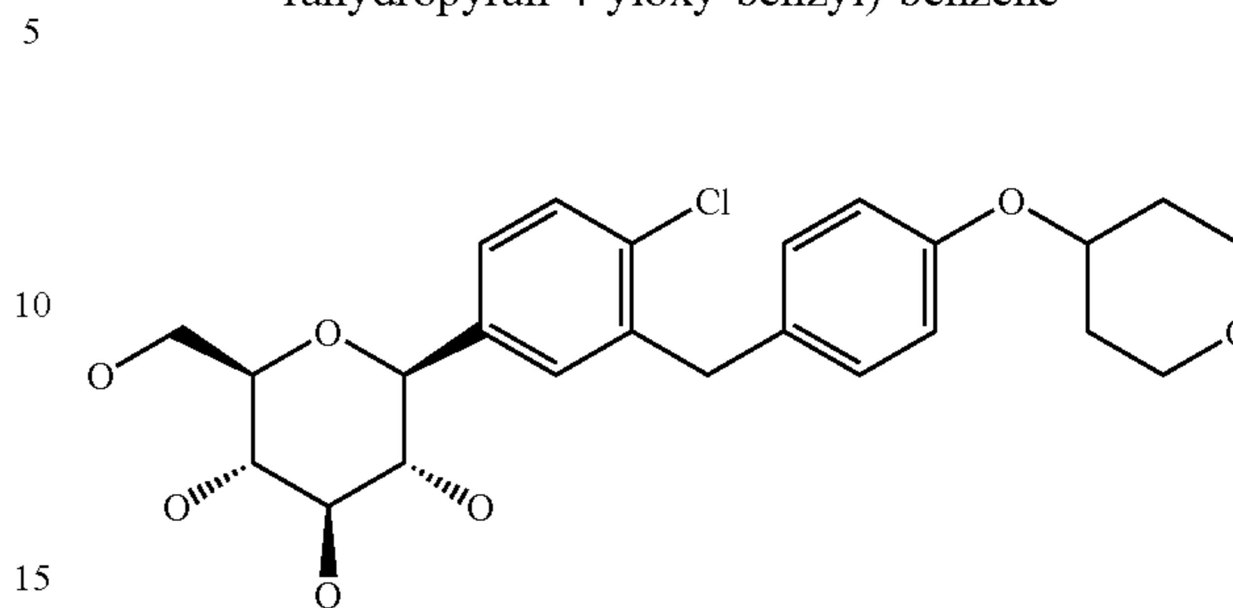
(3) 1-Chloro-4-(β-D-glucopyranos-1-yl)-2-(4-tetrahydrofuran-4-yloxy-benzyl)-benzene
