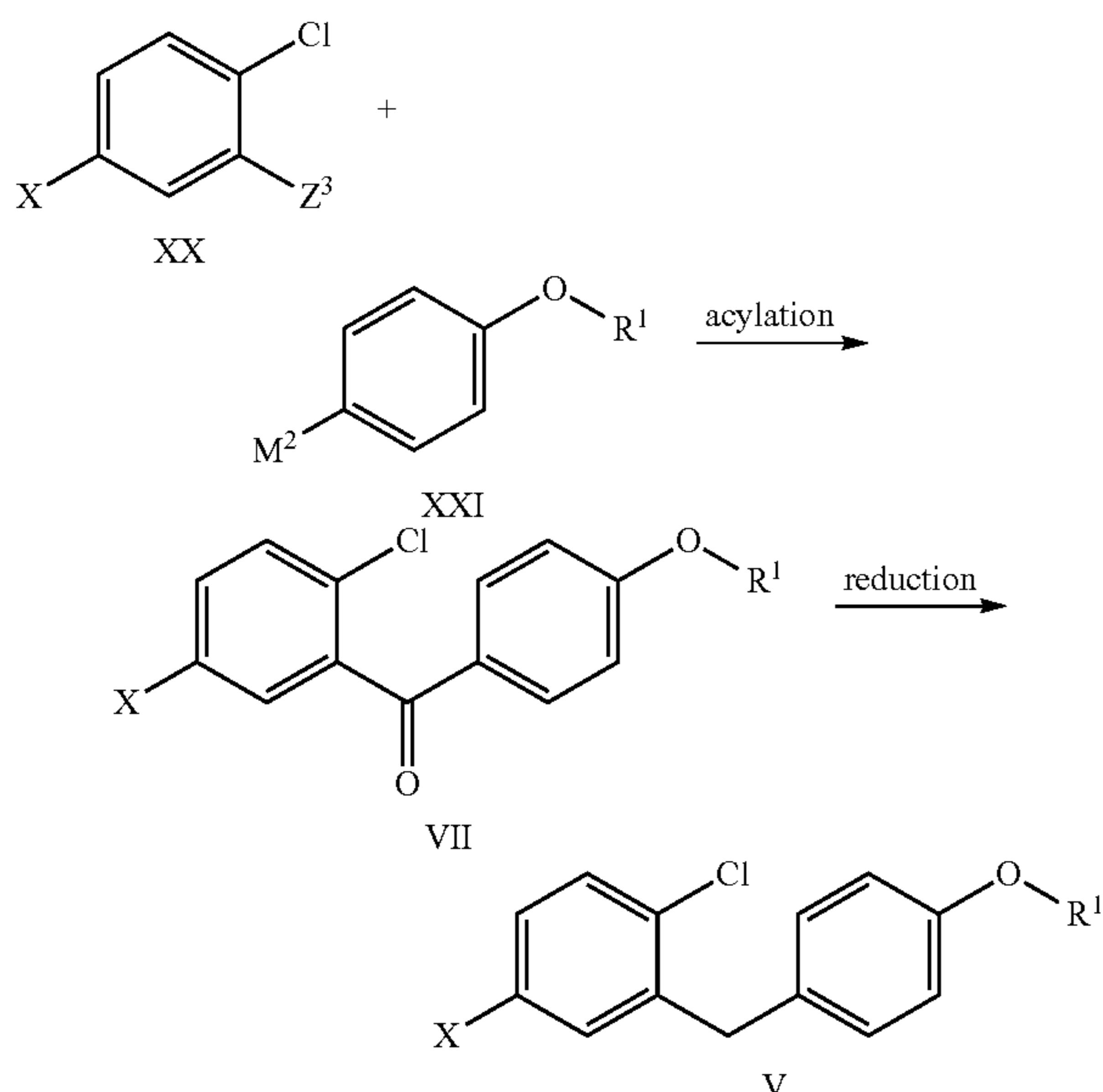
Scheme 8: Synthesis of Aglycon V - Approach 6
