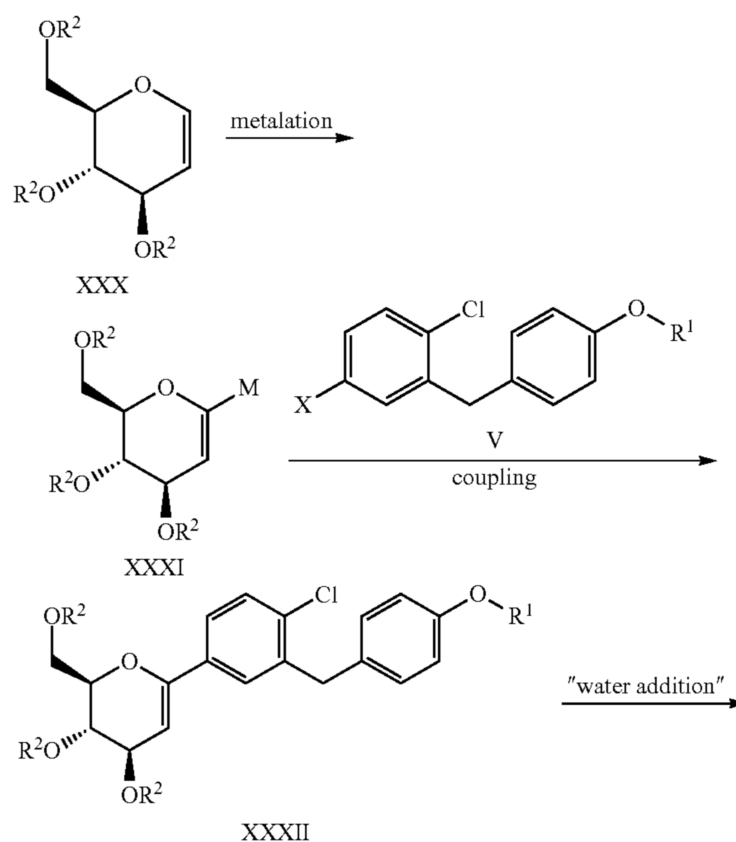
Scheme 2b: Synthesis of C-Glucosides - Approach 2
