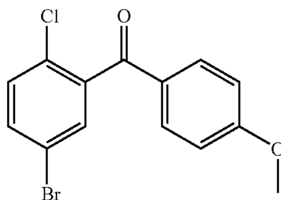
(5-bromo-2-chloro-phenyl)-(4-methoxy-phenyl)-methanone
