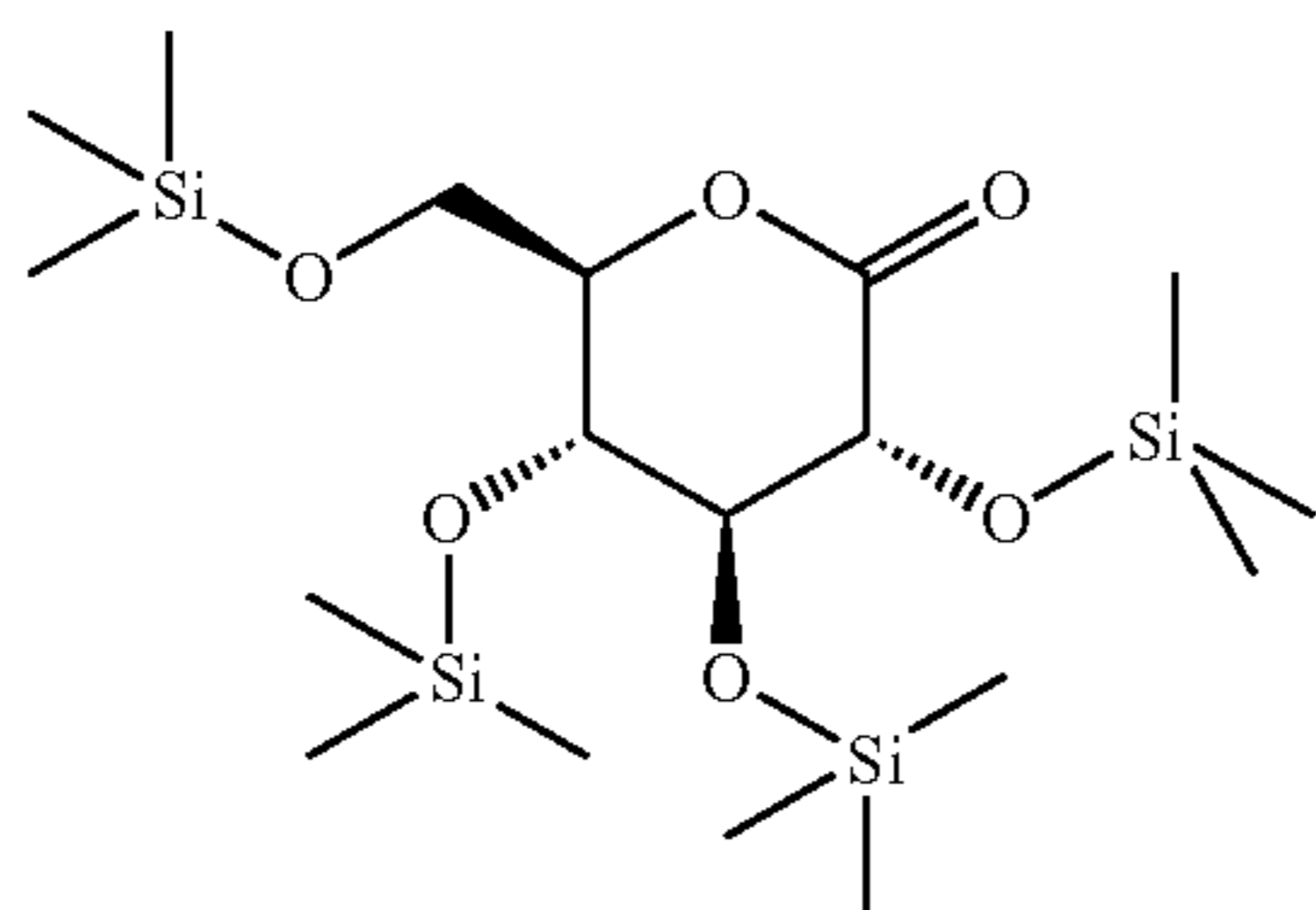
2,3,4,6-tetrakis-O-(trimethylsilyl)-D-glucopyranone
