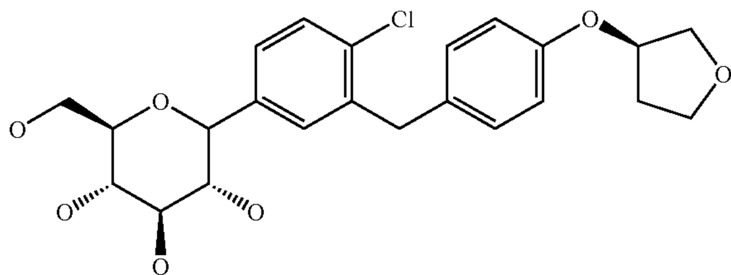
1-Chloro-4-(β-D-glucopyranos-1-yl)-2-(4-(R)-tetrahydrofuran-3-yloxy-benzyl)-benzene
