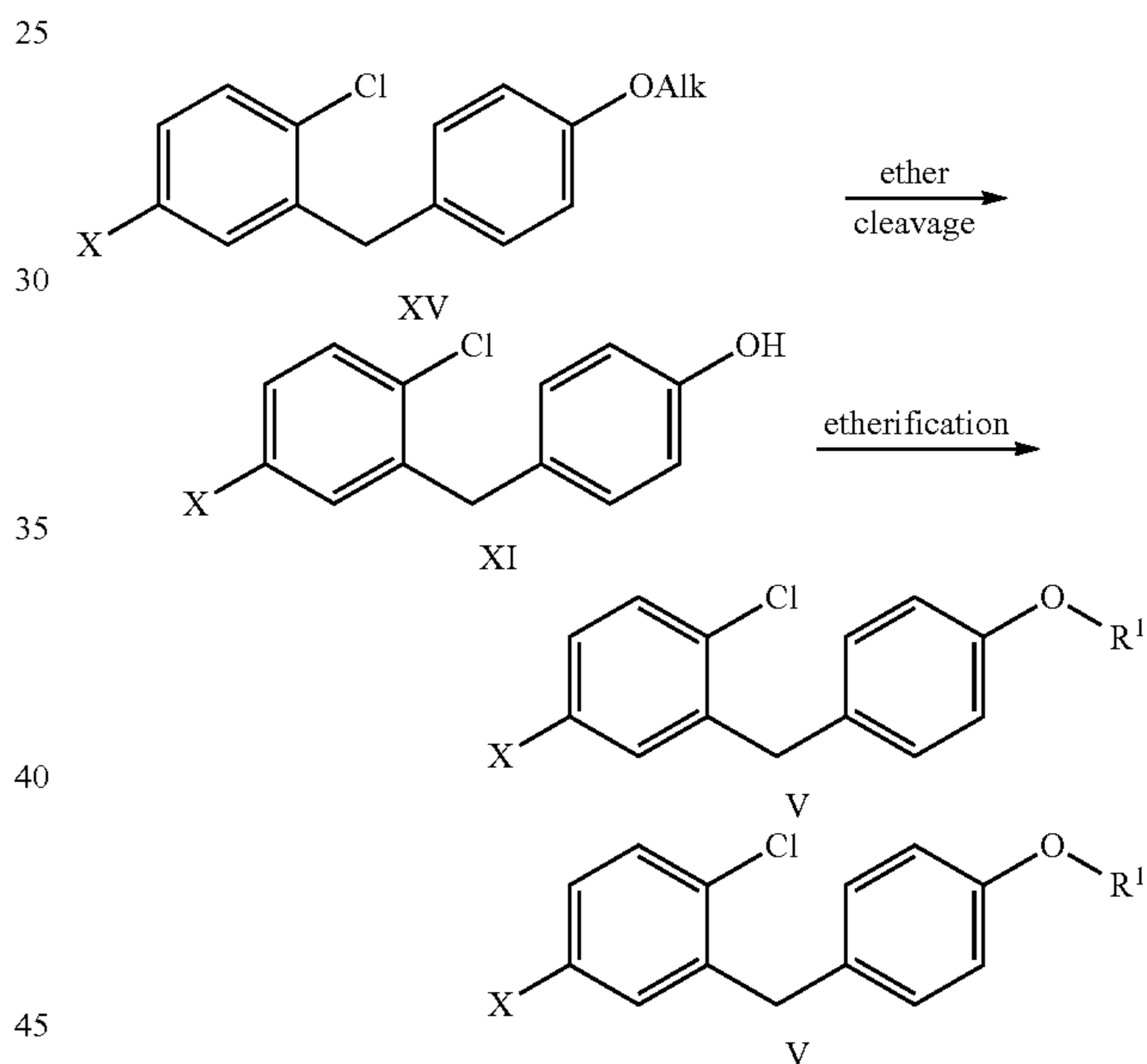
Scheme 4: Synthesis of Aglycon V - Approach 2
