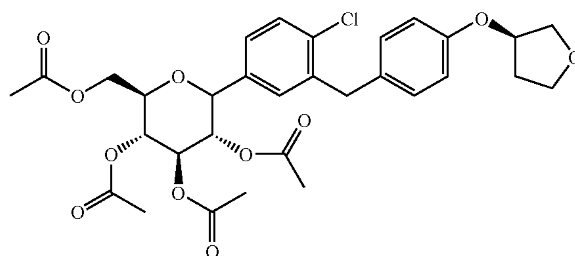
1-Chloro-4-(2,3,4,6-tetra-O-acetyl-D-glucopyranos-1-yl)-2-(4-(R)-tetrahydrofuran-3-yloxy-benzyl)-benzene
