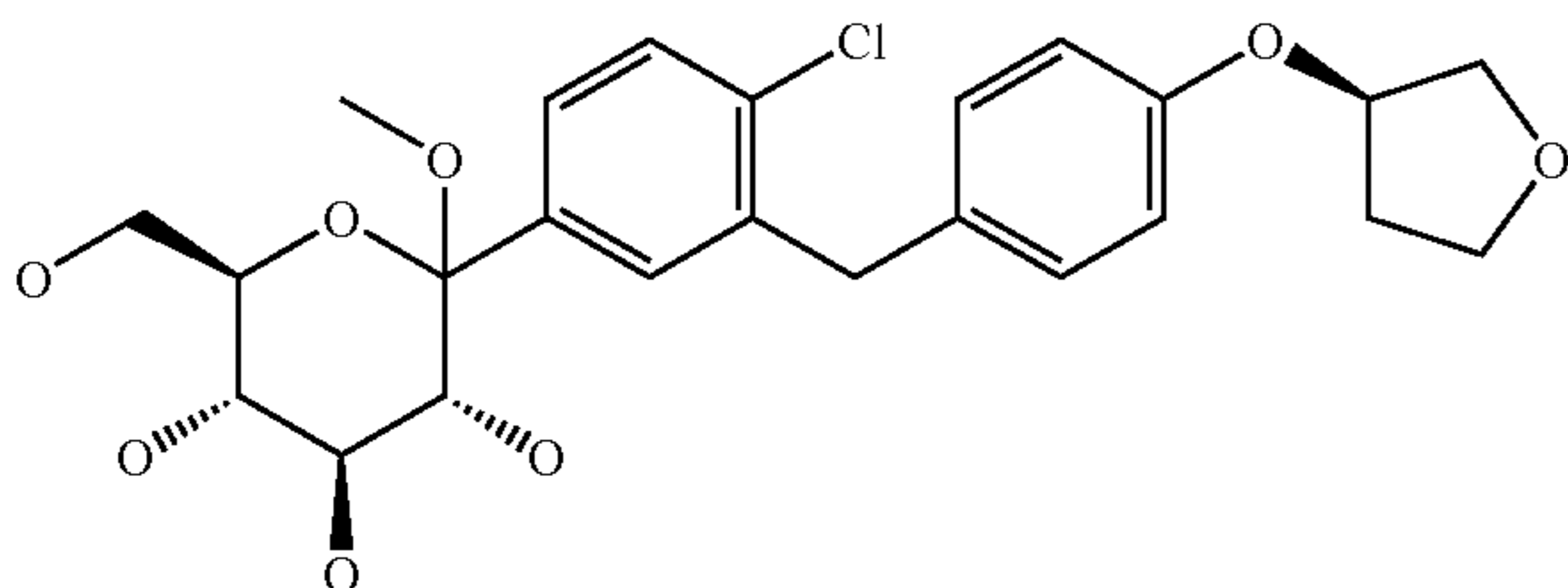
1-Chloro-4-(1-methoxy-D-glucopyranos-1-yl)-2-(4-(R)-tetrahydrofuran-3-yloxy-benzyl)-benzene
