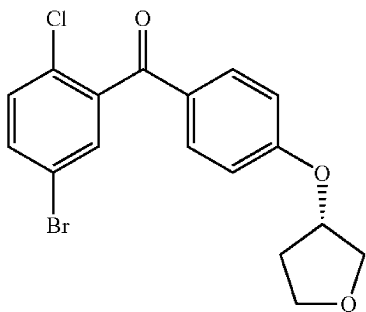
(5-bromo-2-chloro-phenyl)-(4-(S)-tetrahydrofuran-3-yloxy-phenyl)-methanone
