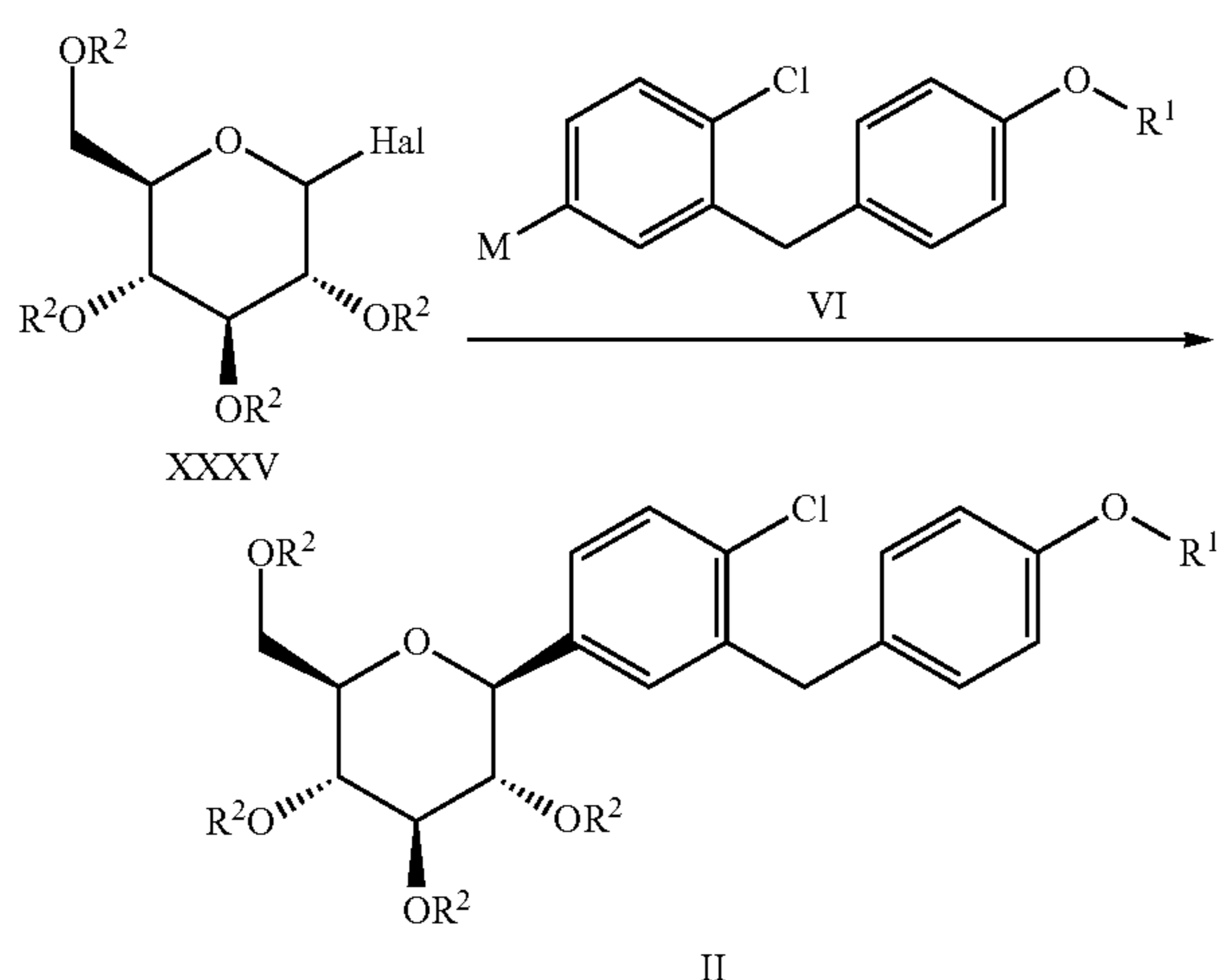
Scheme 2d: Synthesis of C-Glucoside - Approach 4
