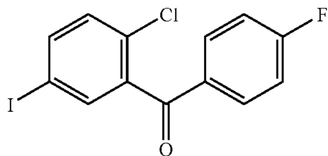
(2-Chloro-5-iodo-phenyl)-(4-fluoro-phenyl)-methanone
