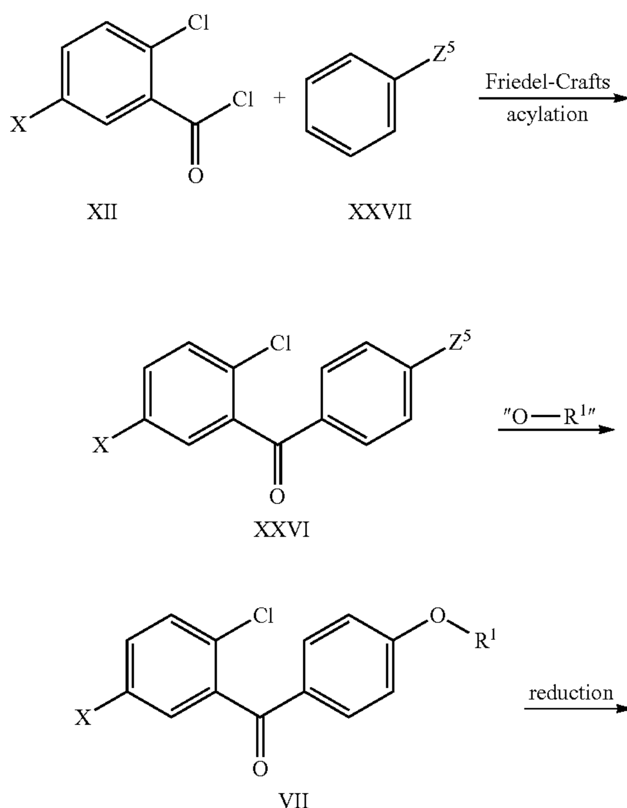
Scheme 11: Synthesis of Aglycon V - Preferred embodiment
