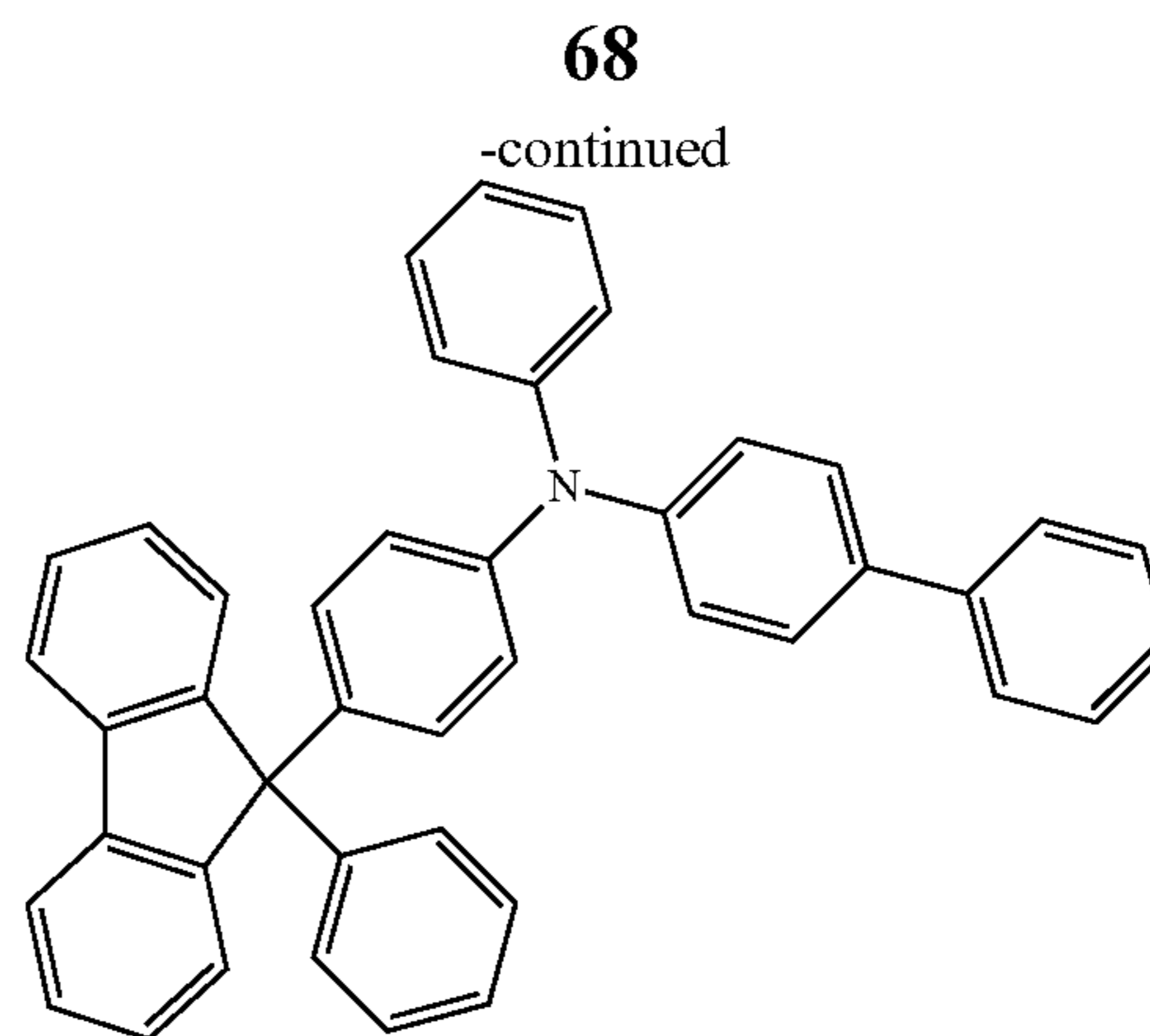
BPAFLP
