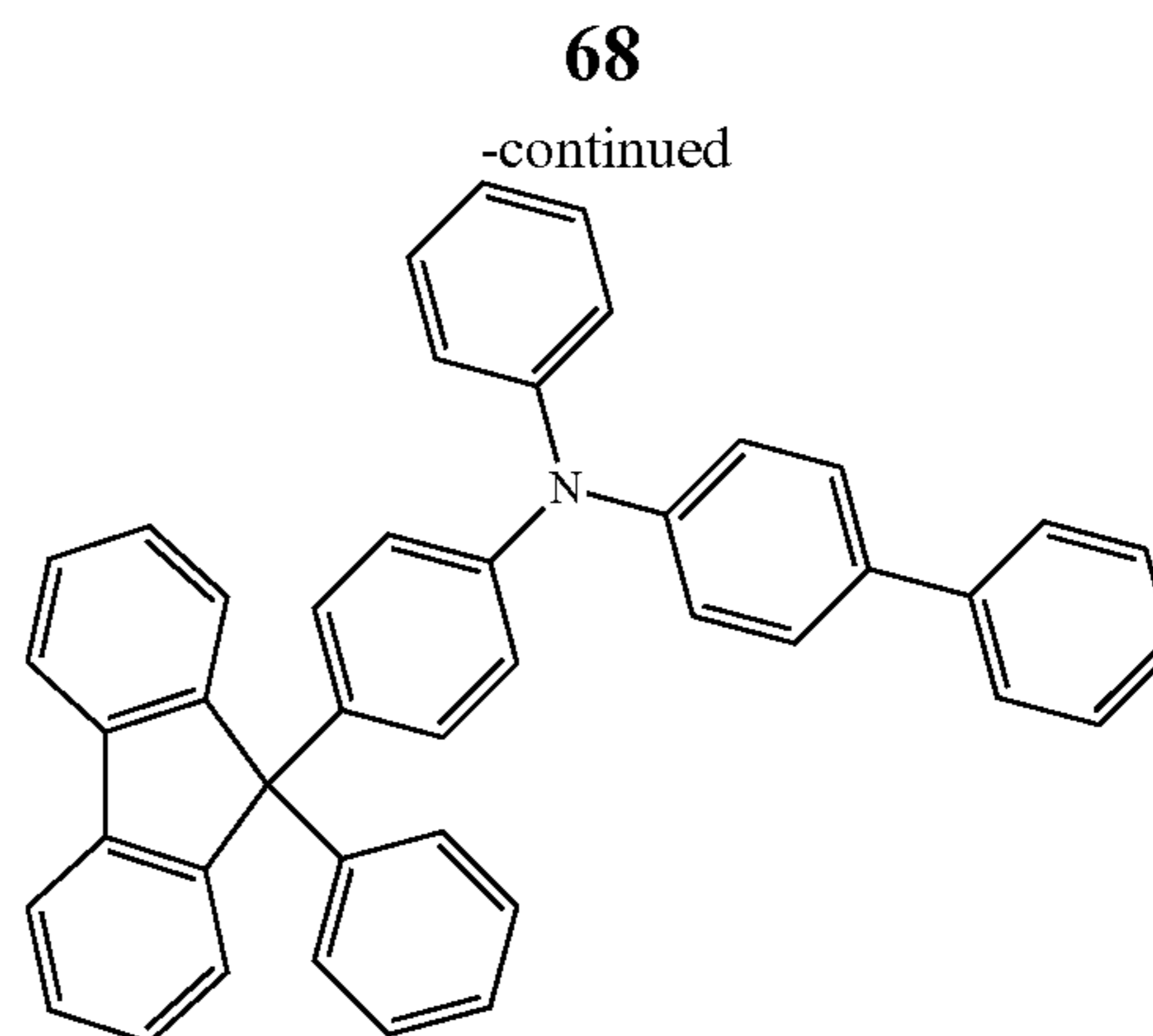
BPAFLP
