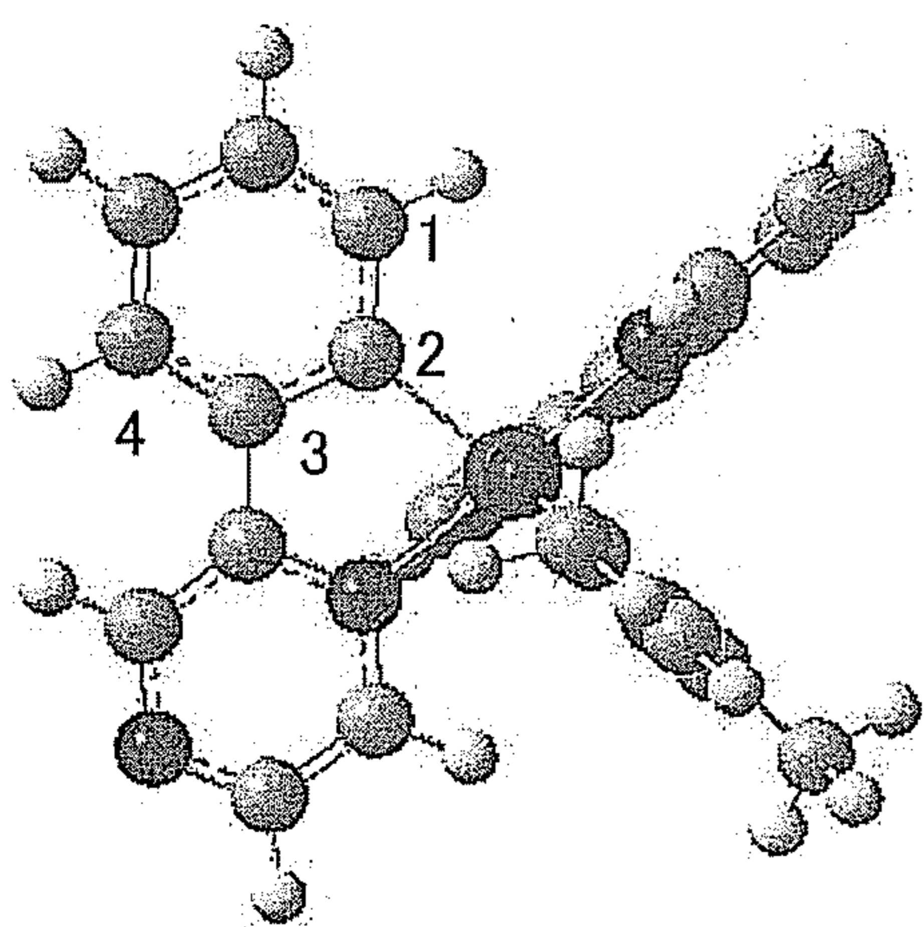
[\text{Ir}(\text{ppr})_2(\text{acac})]
