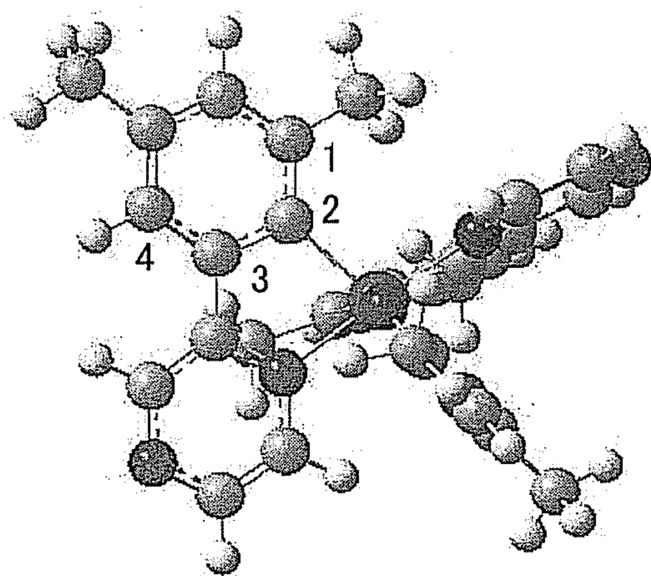
[\text{Ir}(\text{dmppr})_2(\text{acac})]
