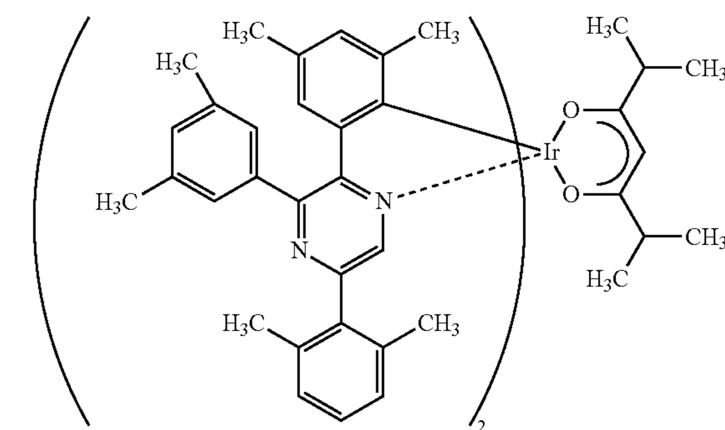
[Ir(dmdppr-dmp) 2 (dibm)]
