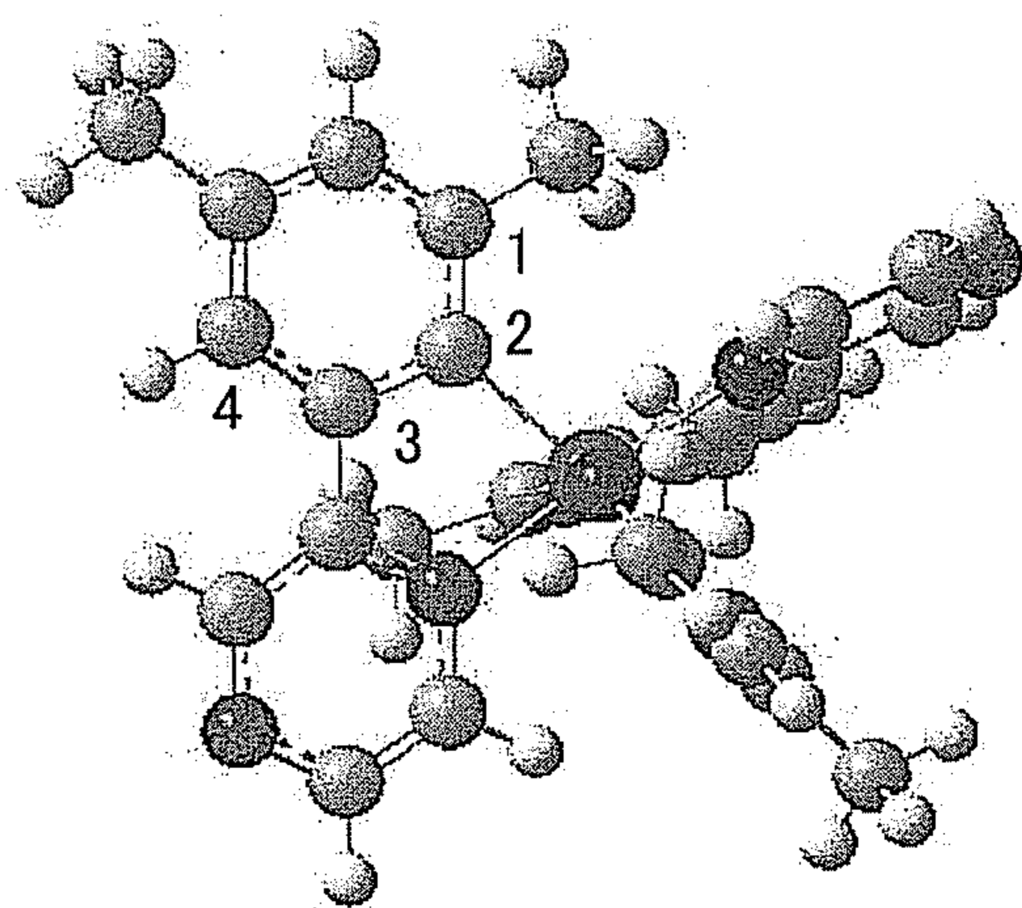
[\text{Ir}(\text{dmppr})_2(\text{acac})]
