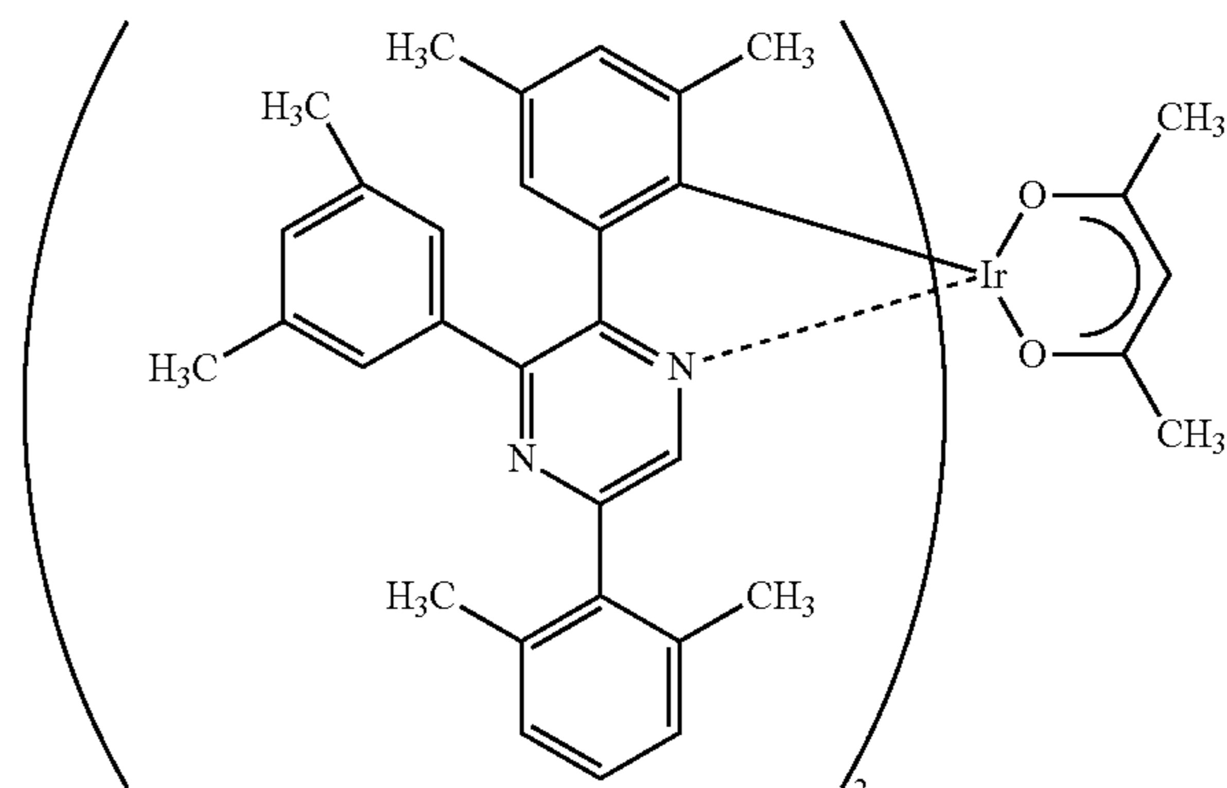
[Ir(dmdppr-dmp) 2 (acac)]
