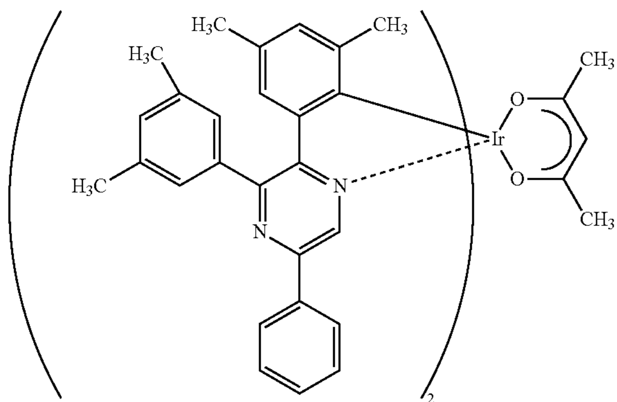
[Ir(dmdppr-P) 2 (acac)]
