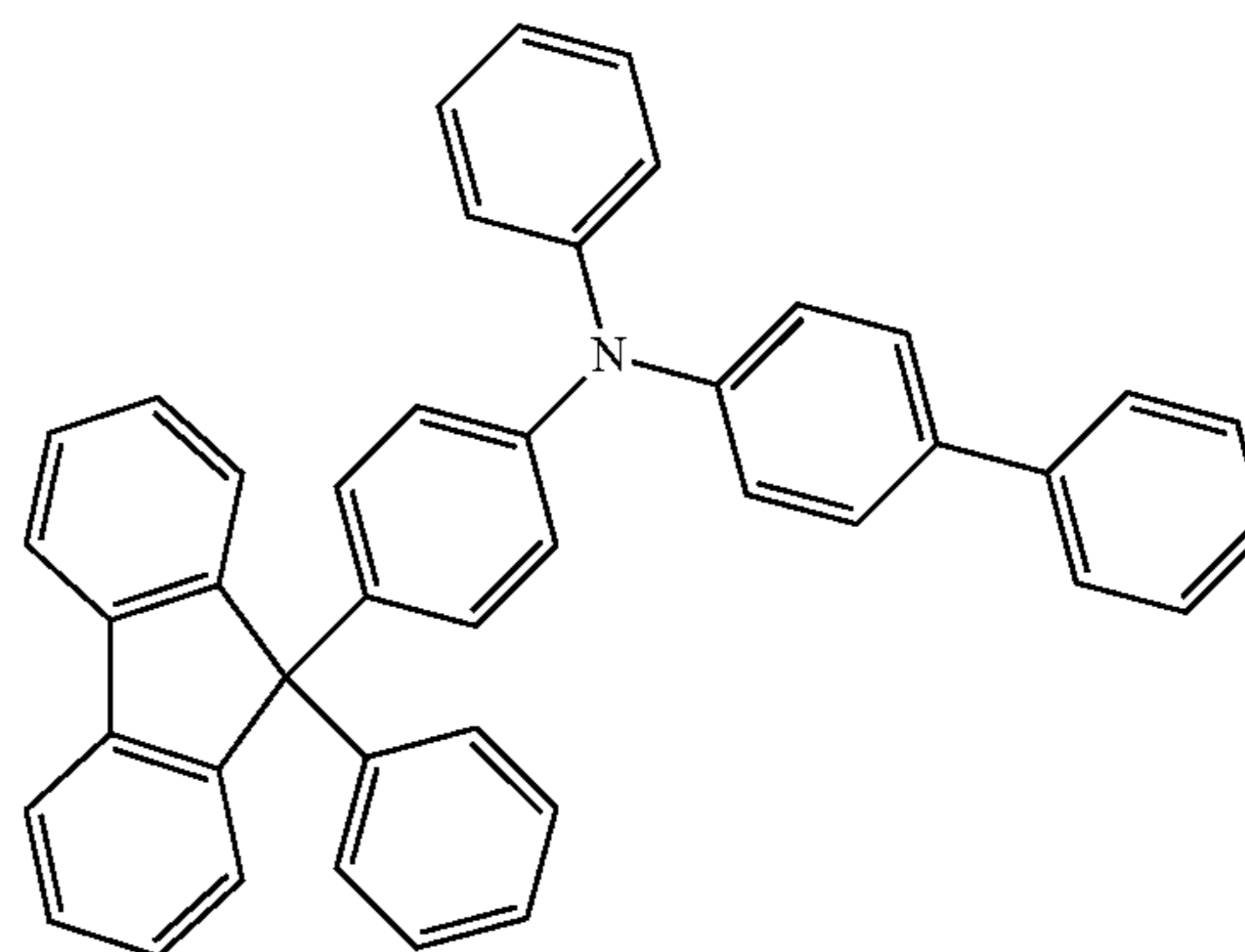
BPAFLP
