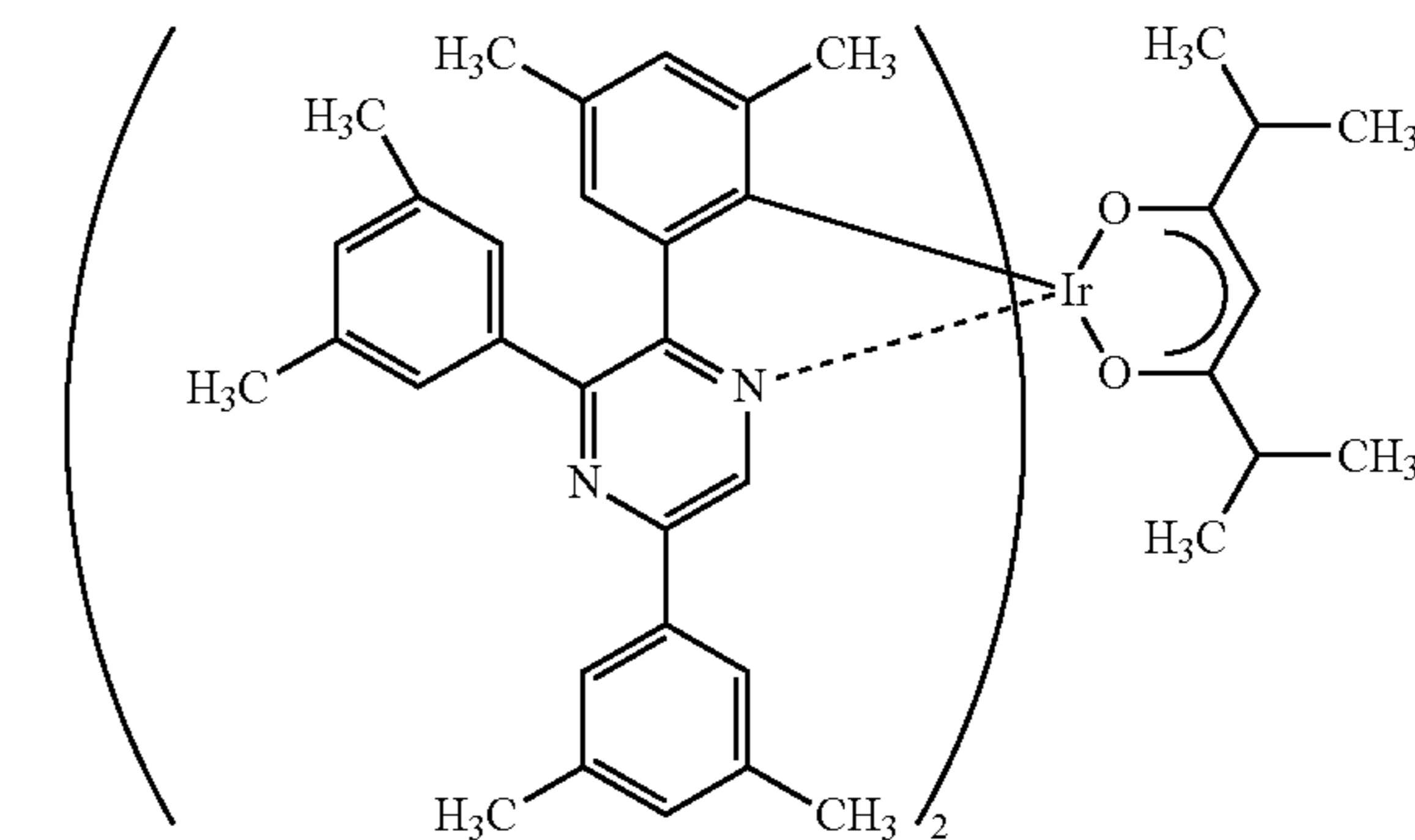
[Ir(dmdppr) 2 (dibm)]
