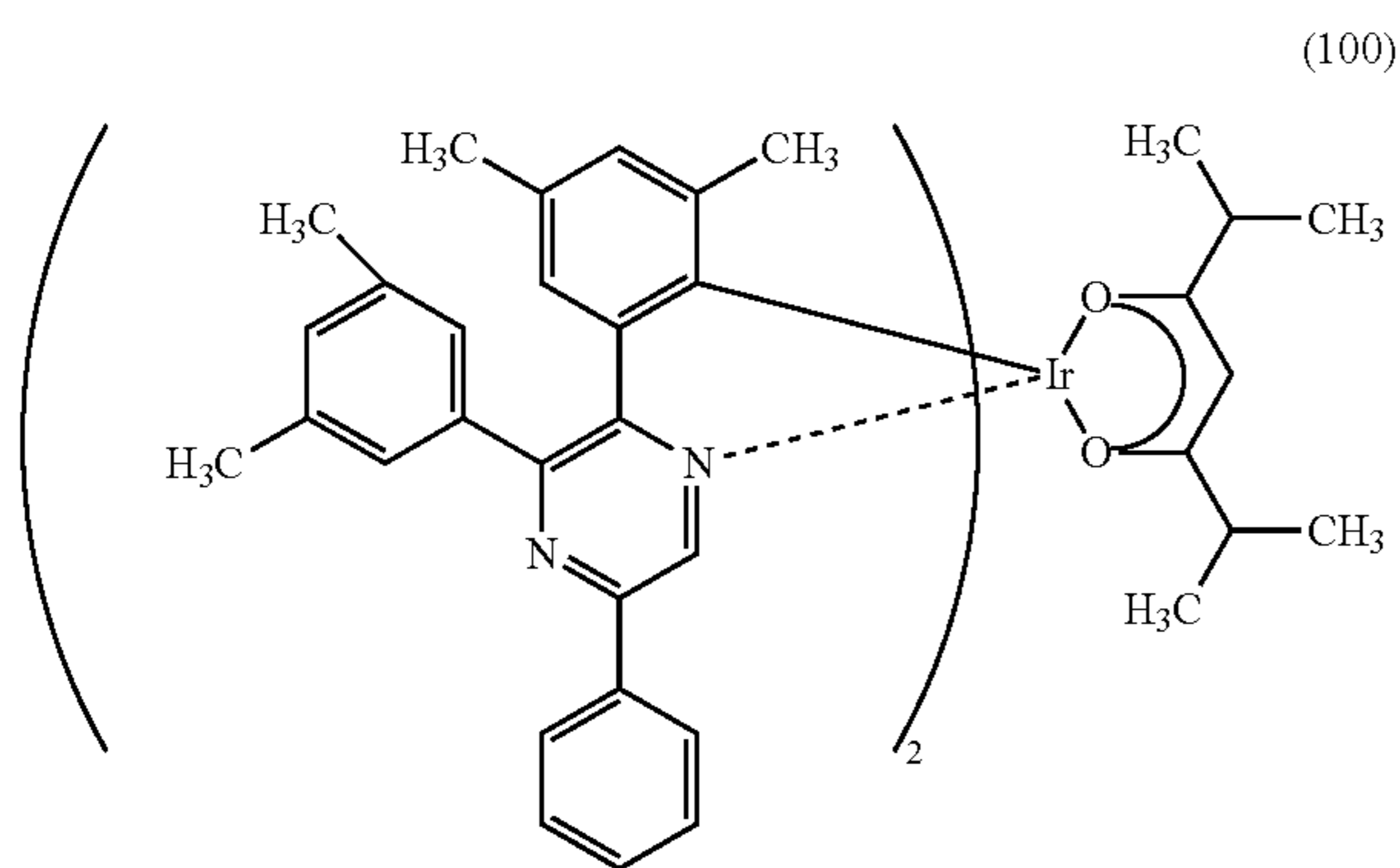
[Ir(dmdppr-P) 2 (dibm)]
