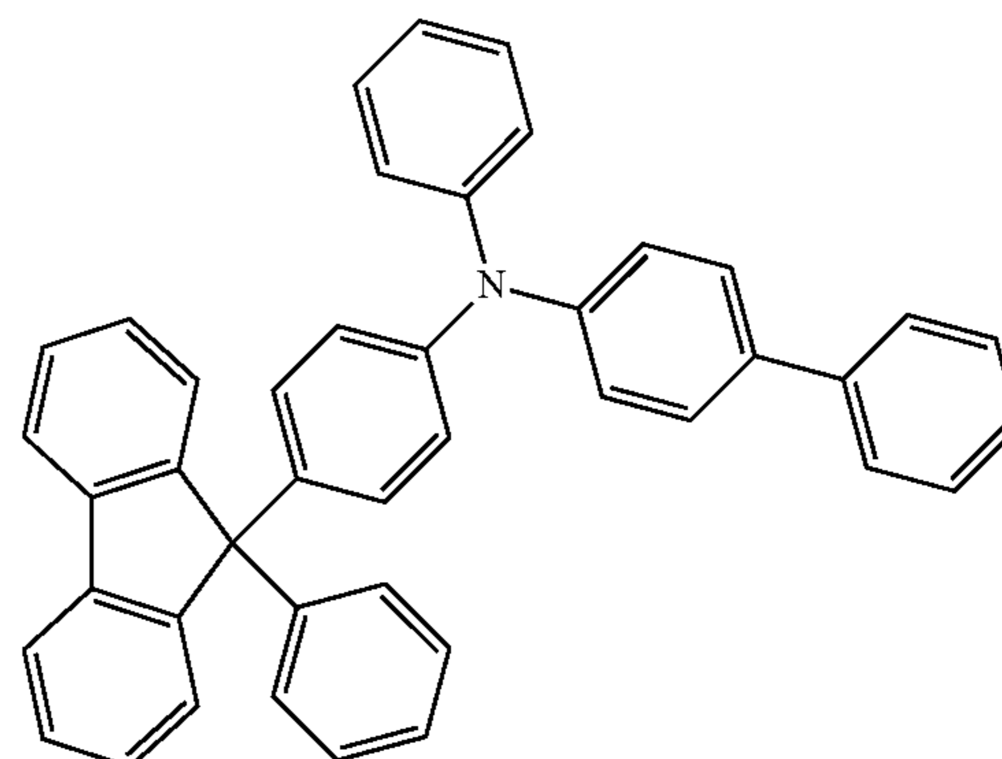
BPAFLP
