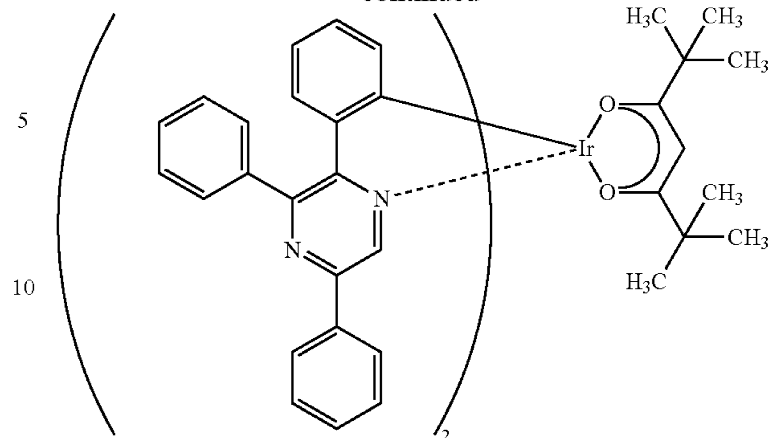
[Ir(tppr) 2 (dpm)]
