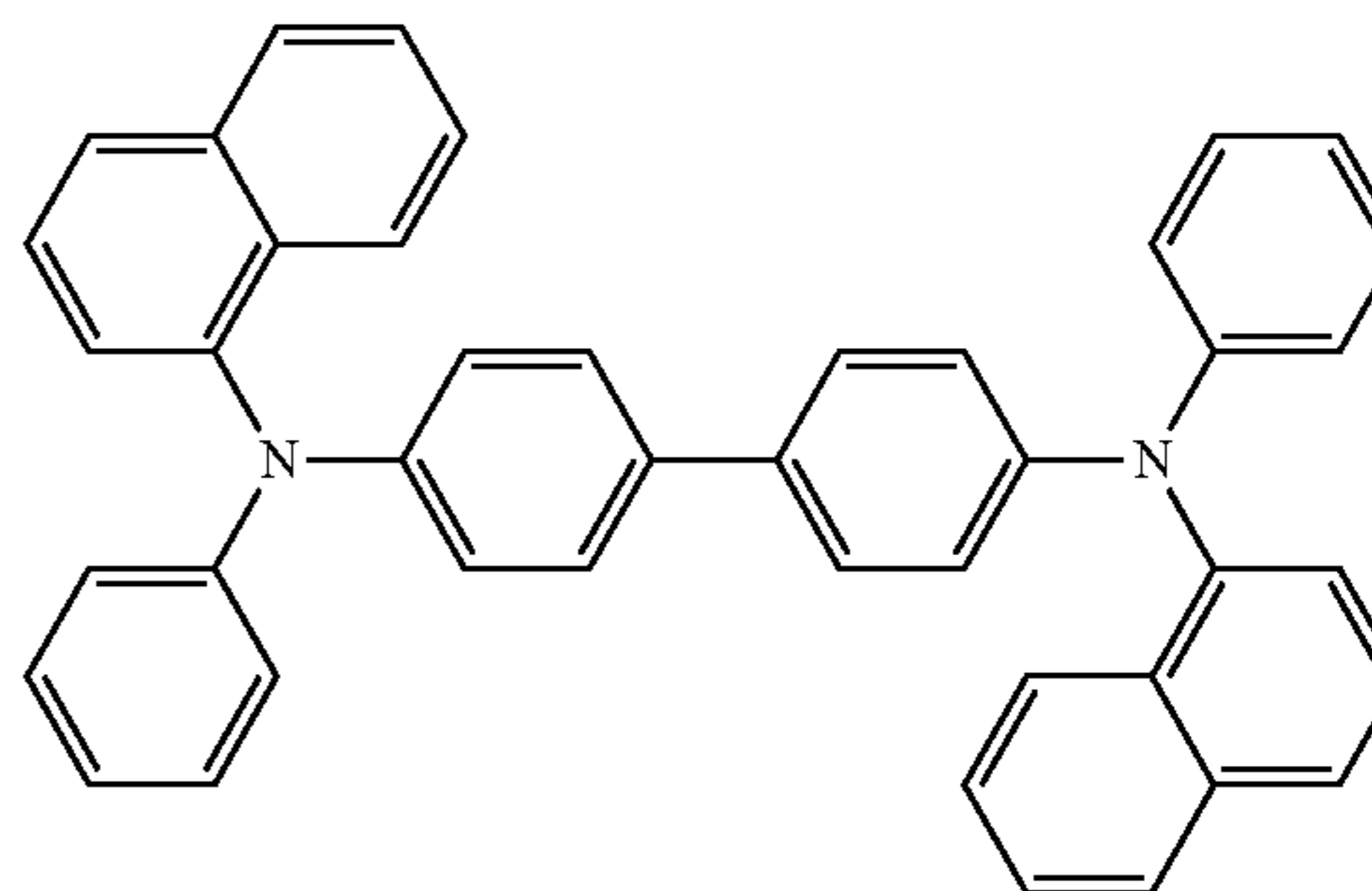
NPB
