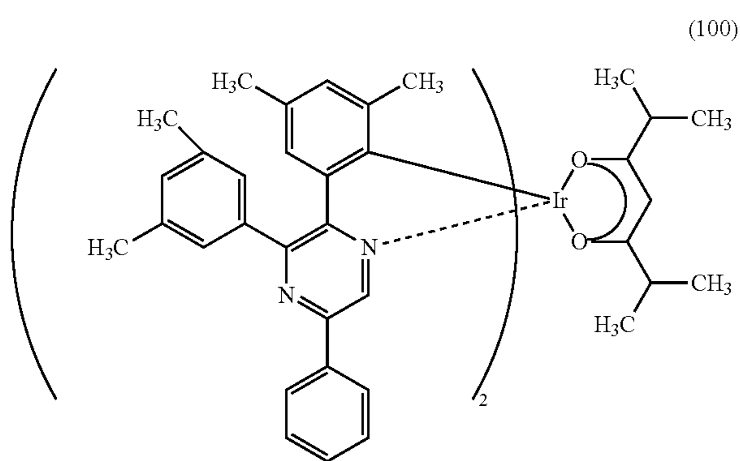
[Ir(dmdppr-P) 2 (dibm)]
