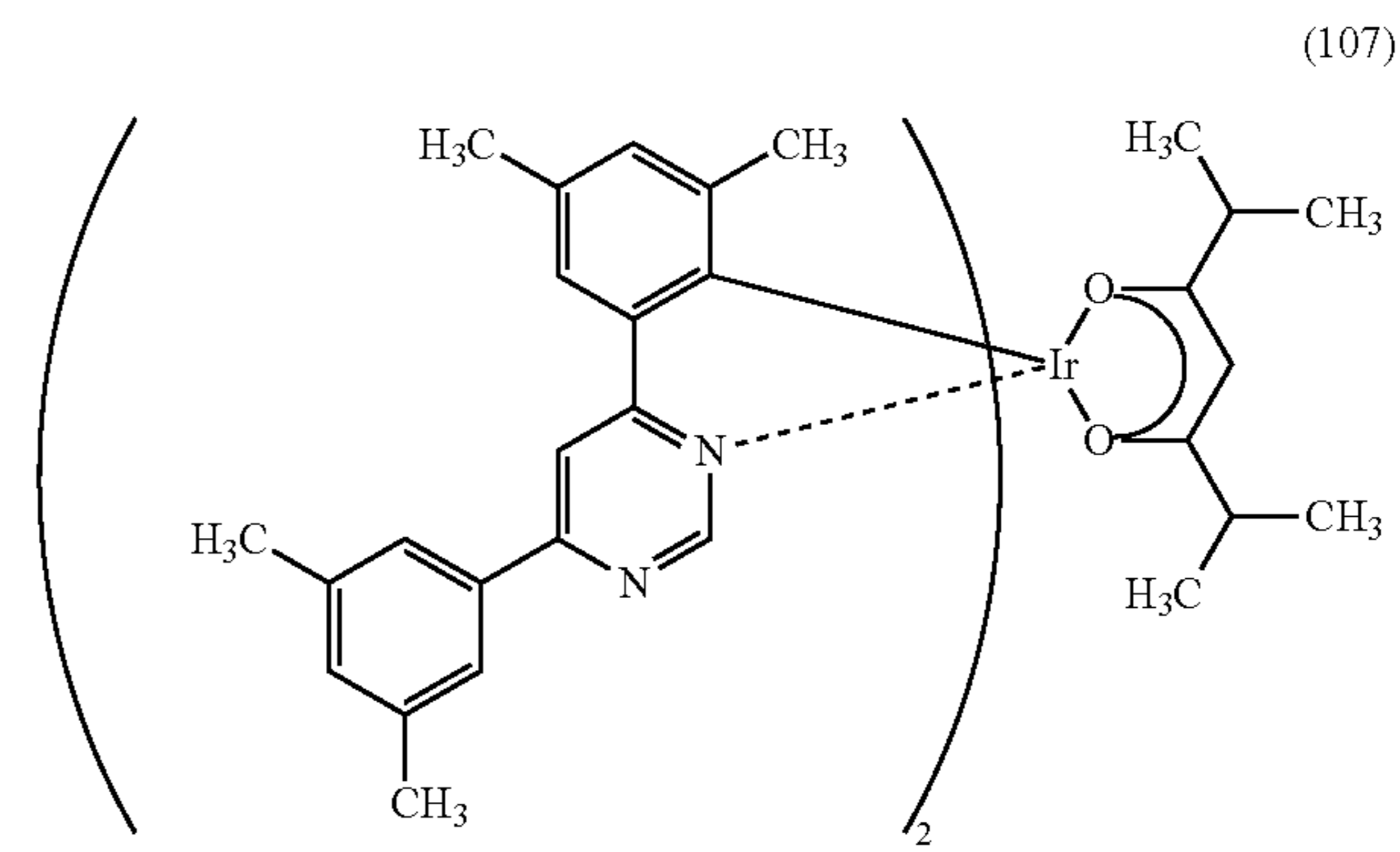
[Ir(dmdppm) 2 (dibm)]
