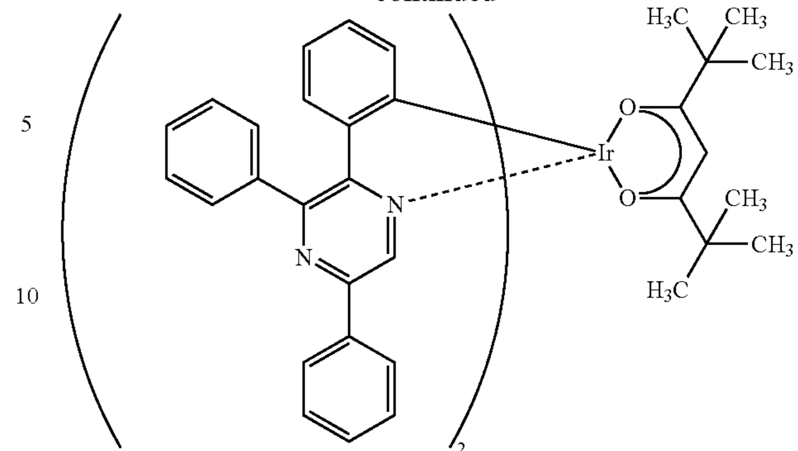
[Ir(tppr) 2 (dpm)]
