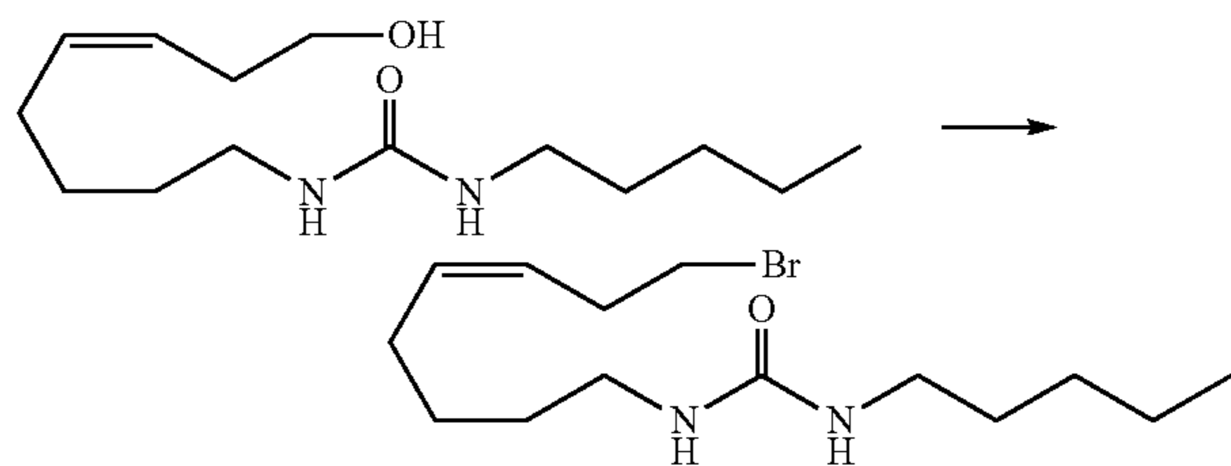
1-(8-Bromooct-5(Z)-enyl)-3-n-pentylurea
