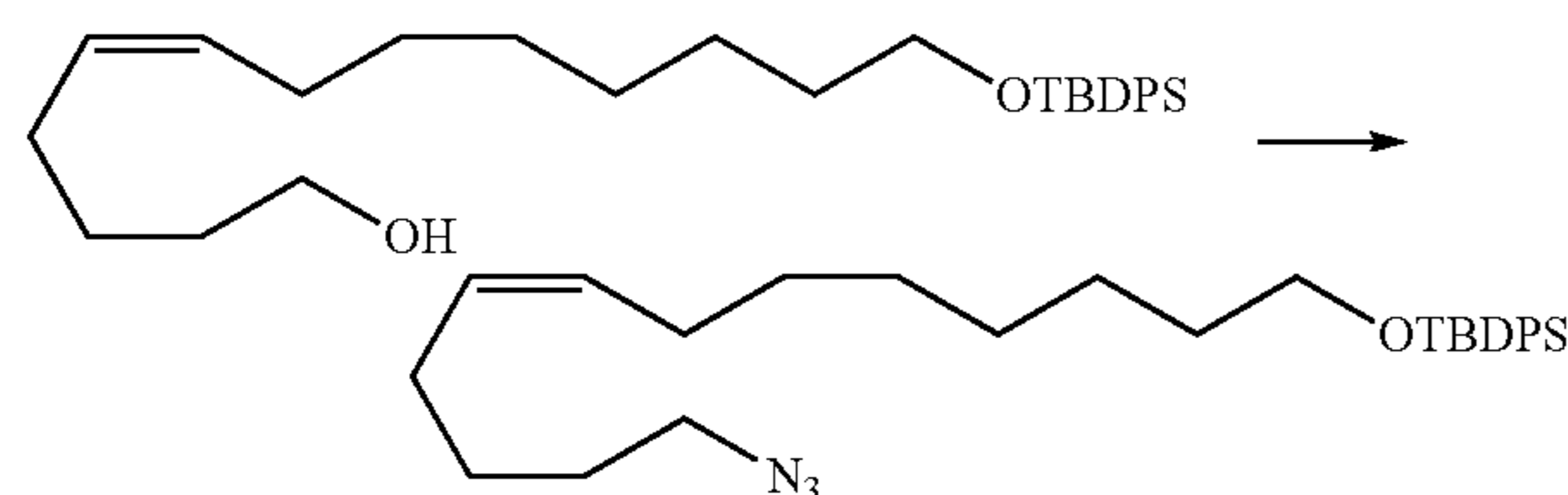
1-tert-Butyldiphenylsilyloxy-13-azidotridec-8(Z)-ene
