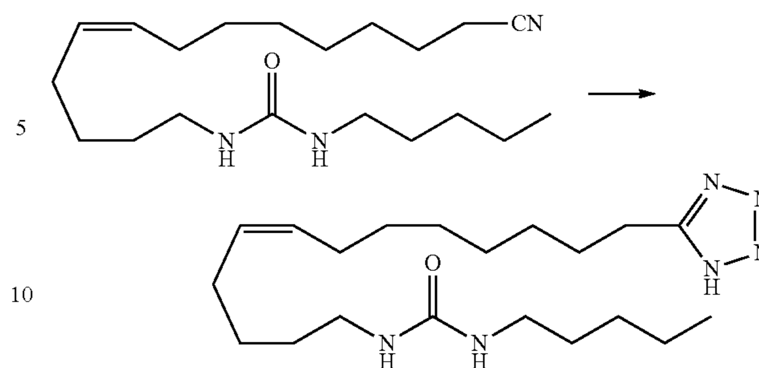
1-(13-(1H-Tetrazol-5-yl)tridec-5(Z)-enyl)-3-n-pentylurea (22)
