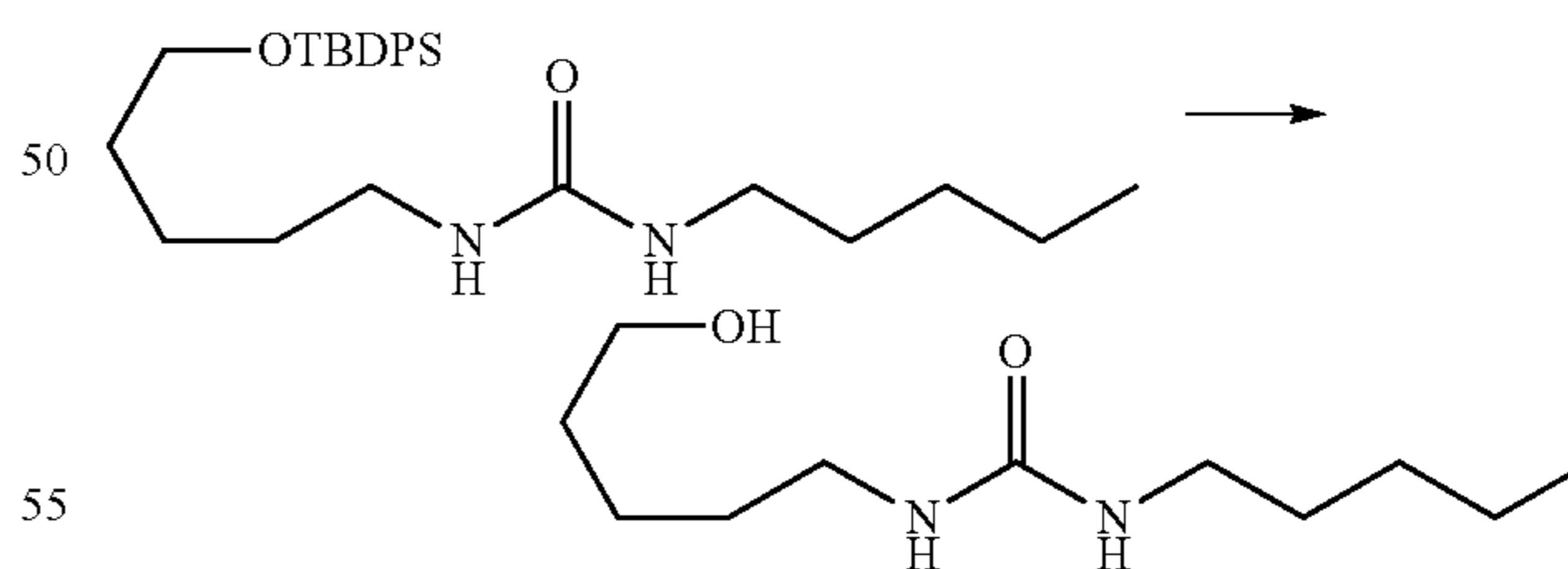
1-(5-Hydroxypentyl)-3-n-pentylurea
