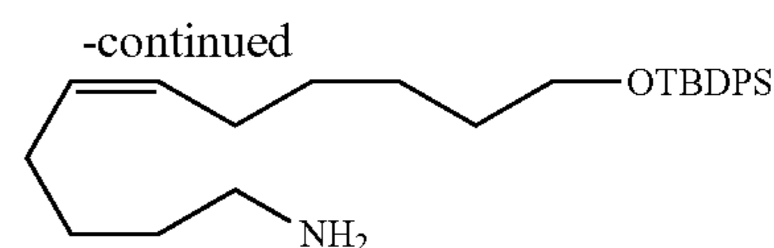
1-Amino-11-(tert-butyl-diphenylsilyloxy)undec-5(Z)-ene
