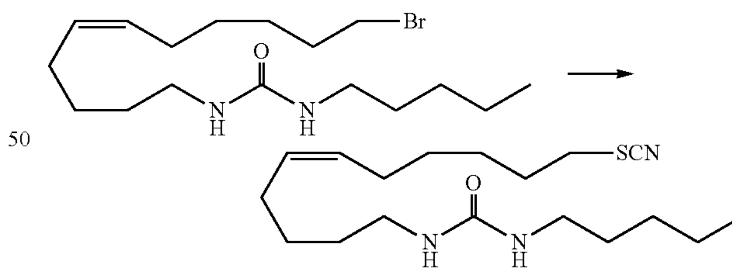
1-n-Pentyl-3-(11-thiocyanatoundec-5(Z)-enyl)urea
