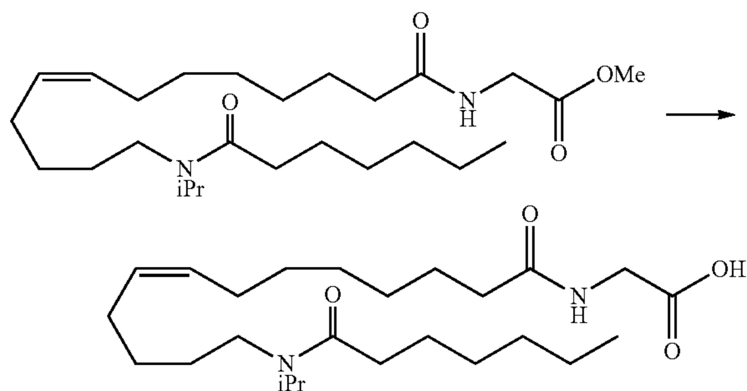
2-(13-(N-Isopropylheptanamido)tridec-8(Z)-enamido)acetic acid (5)
