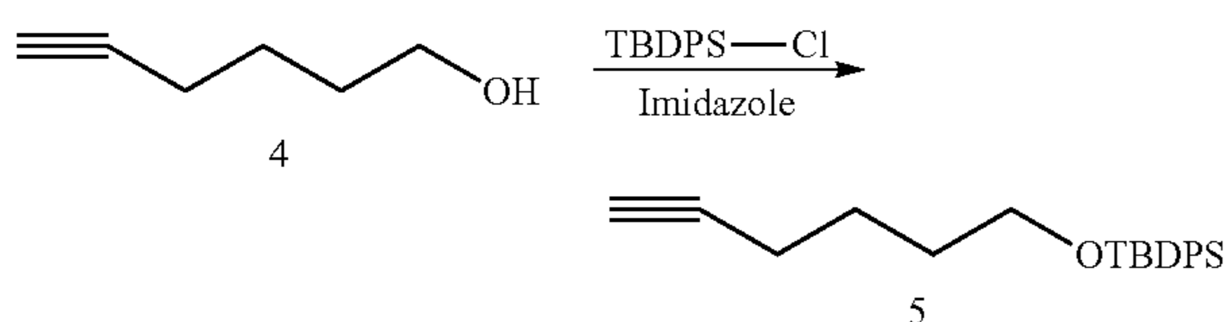
tert-Butyl(hex-5-yn-1-yloxy)diphenylsilane 3 (5)
