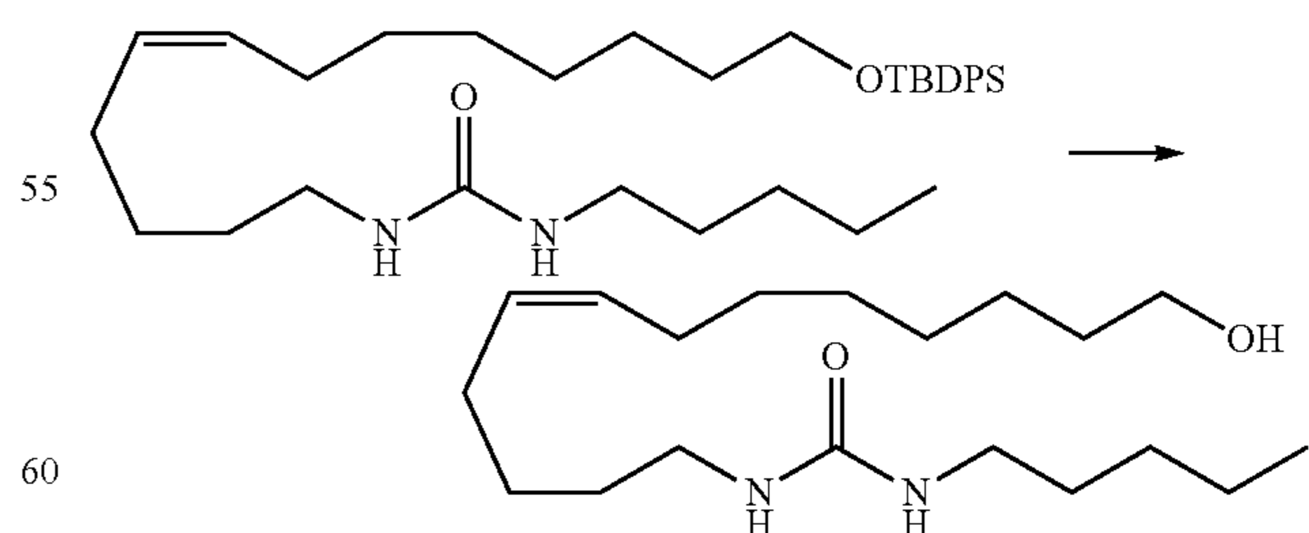
1-(13-Hydroxytridec-5(Z)-enyl)-3-n-pentylurea
