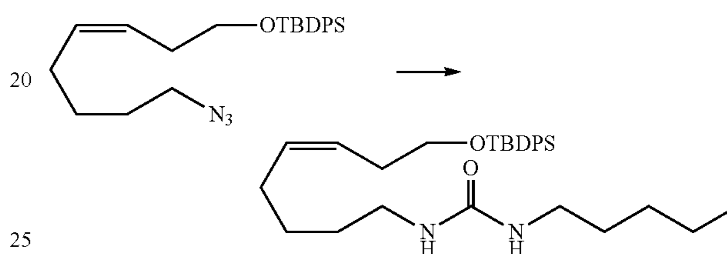
1-(8-(tert-Butyldiphenylsilyloxy)oct-5(Z)-enyl)-3-n-pentylurea
