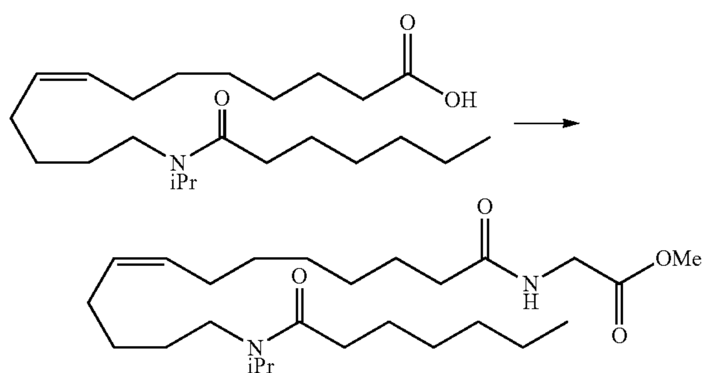
Methyl 2-(13-(N-Isopropylheptanamido)tridec-8(Z)-enamido)acetate
