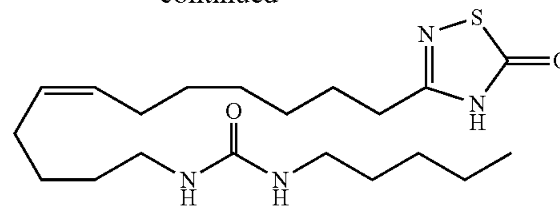
Analog 29
