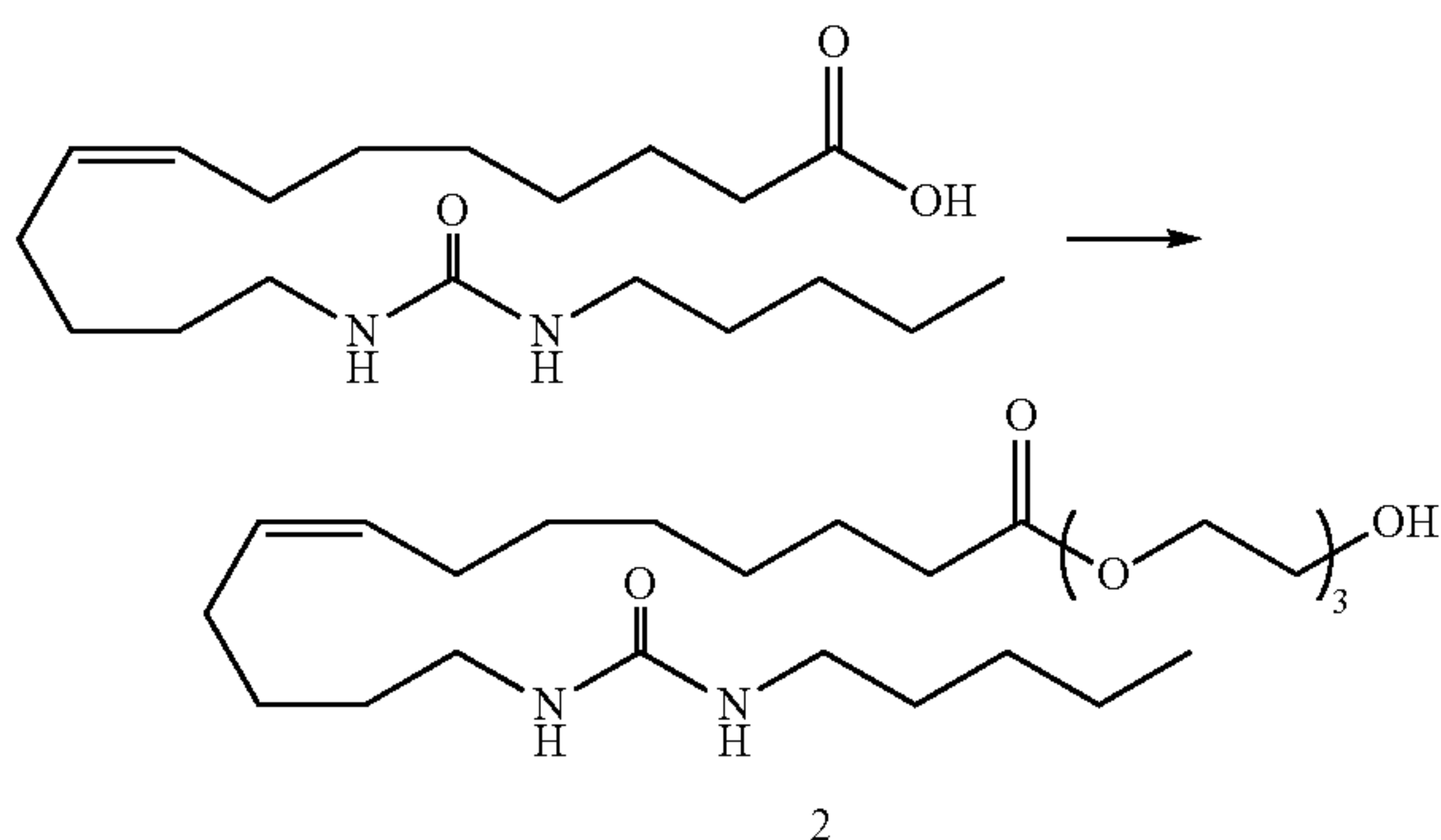
2-(2-(2-Hydroxyethoxy)ethoxy)ethyl 13-(3-n-pentylureido)tridec-8(Z)-enoate (2)
