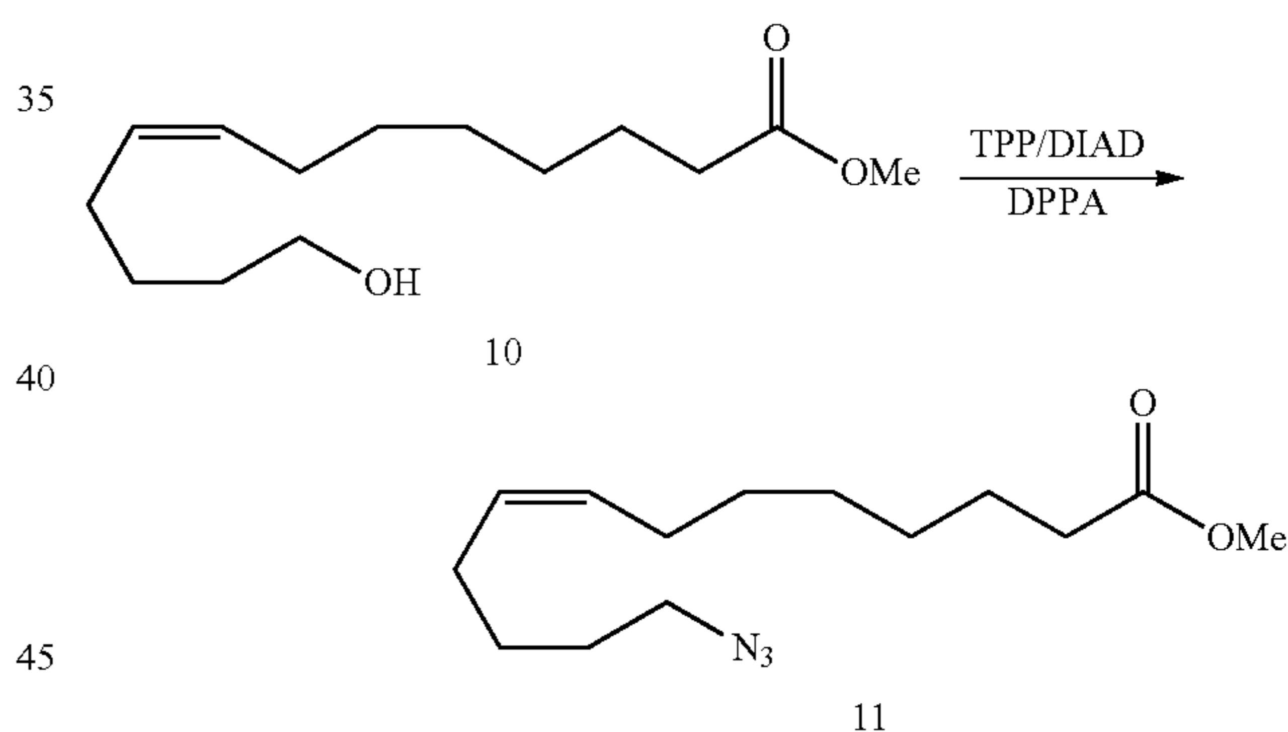
Methyl 13-azidotridec-8(Z)-enoate 5 (11)
