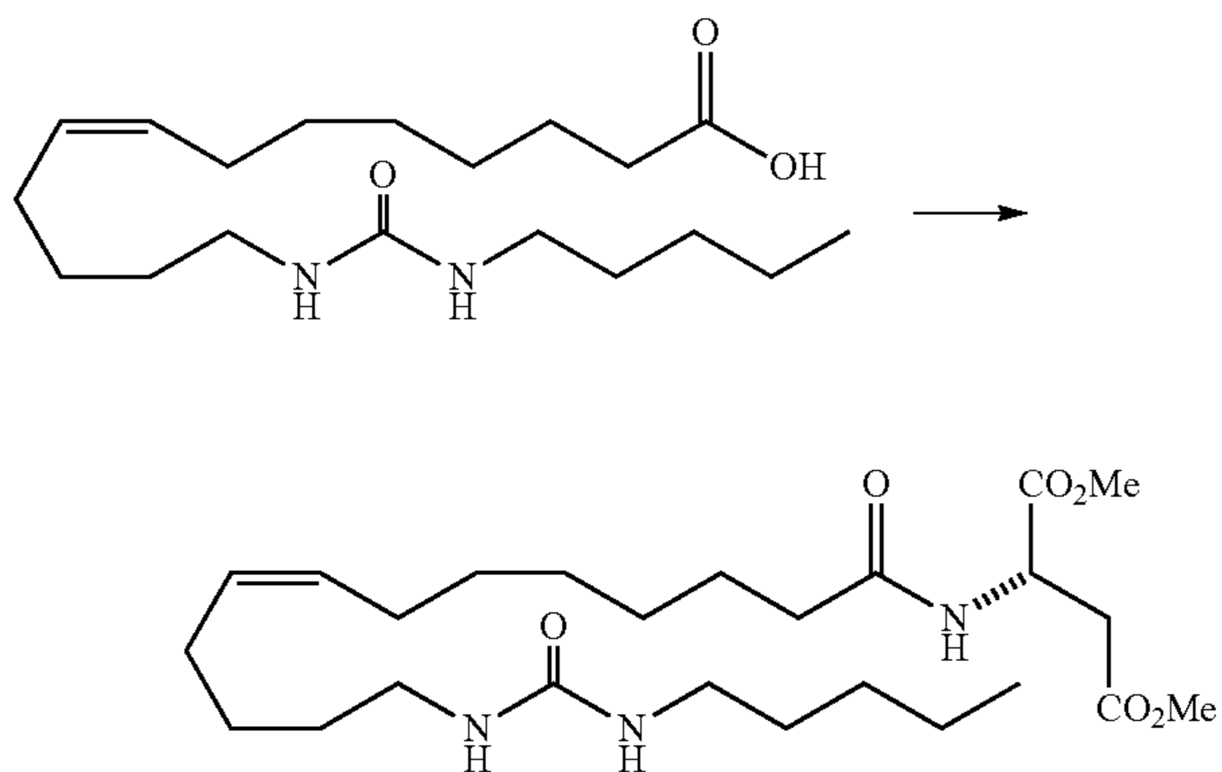
(S)-Dimethyl 2-(13-(3-n-pentylureido)tridec-8(Z)-enamido)succinate
