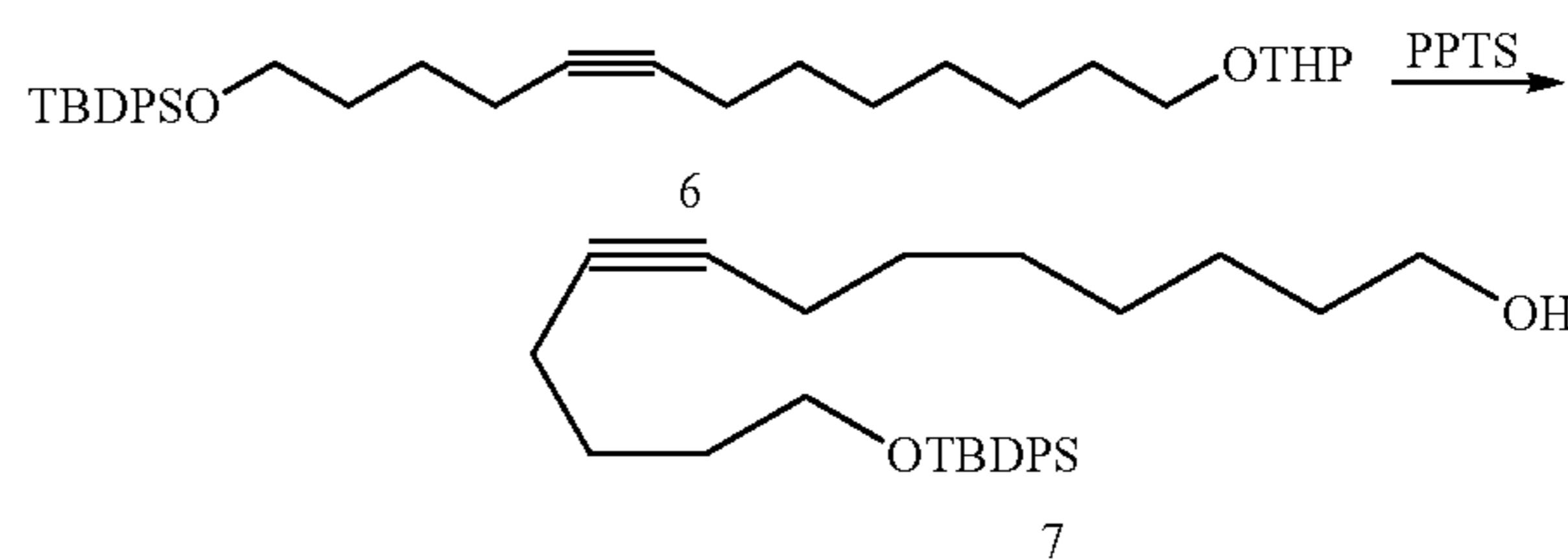
13-(tert-Butyldiphenylsilyloxy)tridec-8-yn-1-ol (7)
