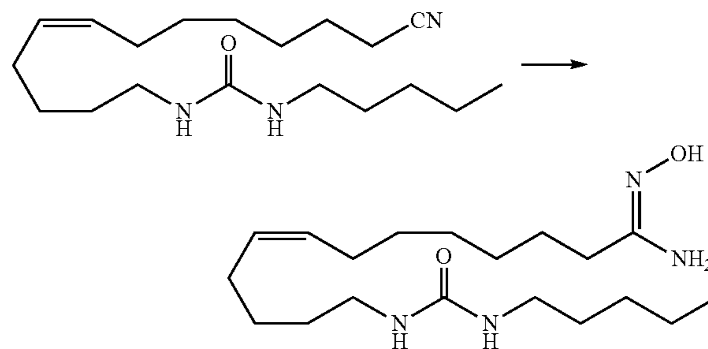
N'-Hydroxy-13-(3-n-pentylureido)tridec-8(Z)-enimidamide
