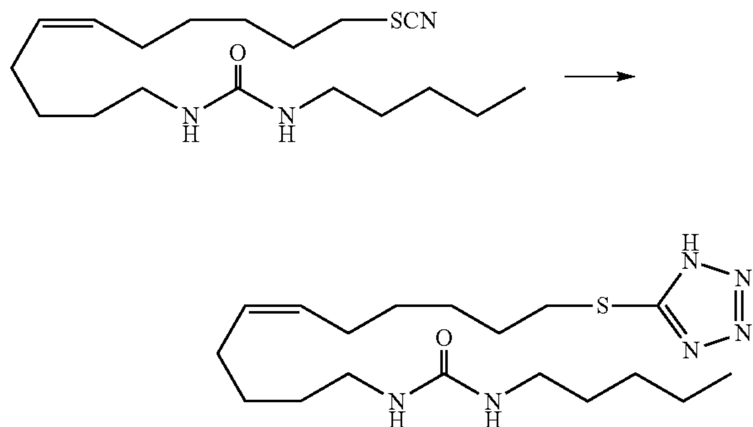
1-(11-(1H-Tetrazol-5-ylthio)undec-5(Z)-enyl)-3-pentylurea (15)
