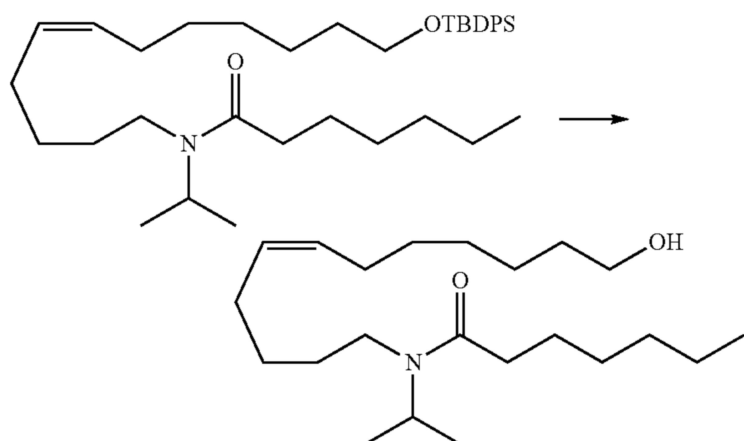
N-(12-Hydroxydodec-5(Z)-enyl)-N-isopropyl n-heptanamide
