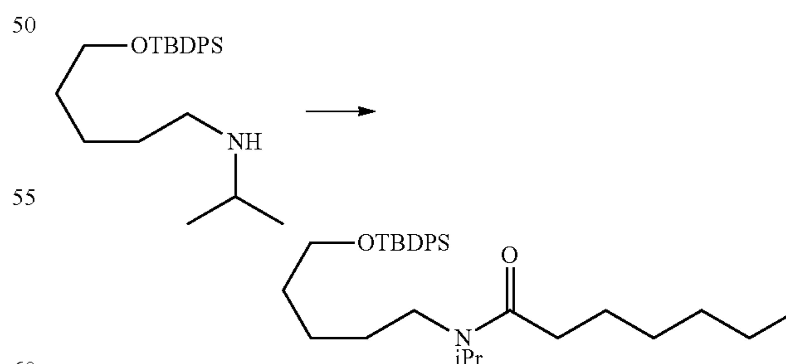
N-(5-(tert-Butyldiphenylsilyloxy)pentyl)-N-isopropylheptanamide
