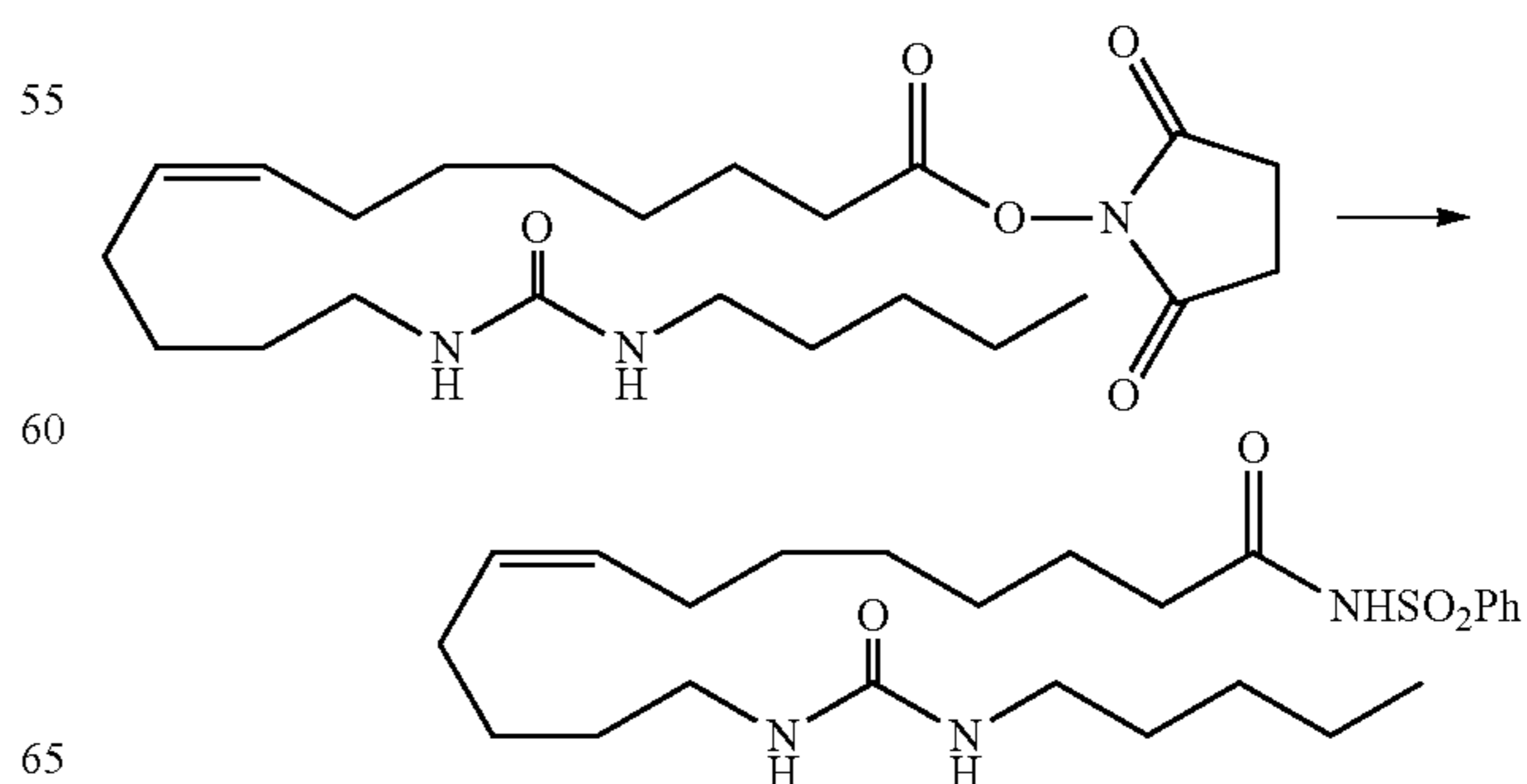
2-(2-(2-Hydroxyethoxy)ethoxy)ethyl 13-(N-isopropylheptanamido)tridec-8(Z)-enoate (1)
