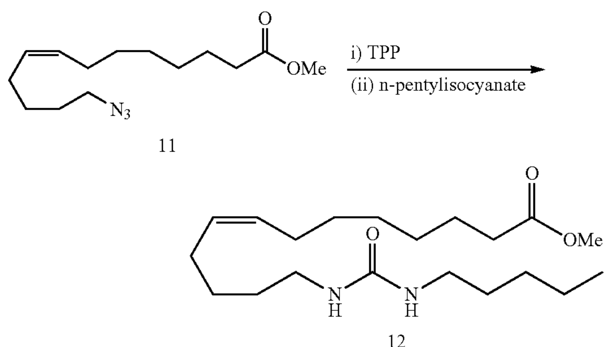
Methyl 13-(3-pentylureido)tridec-8(Z)-enoate 6 (12)
