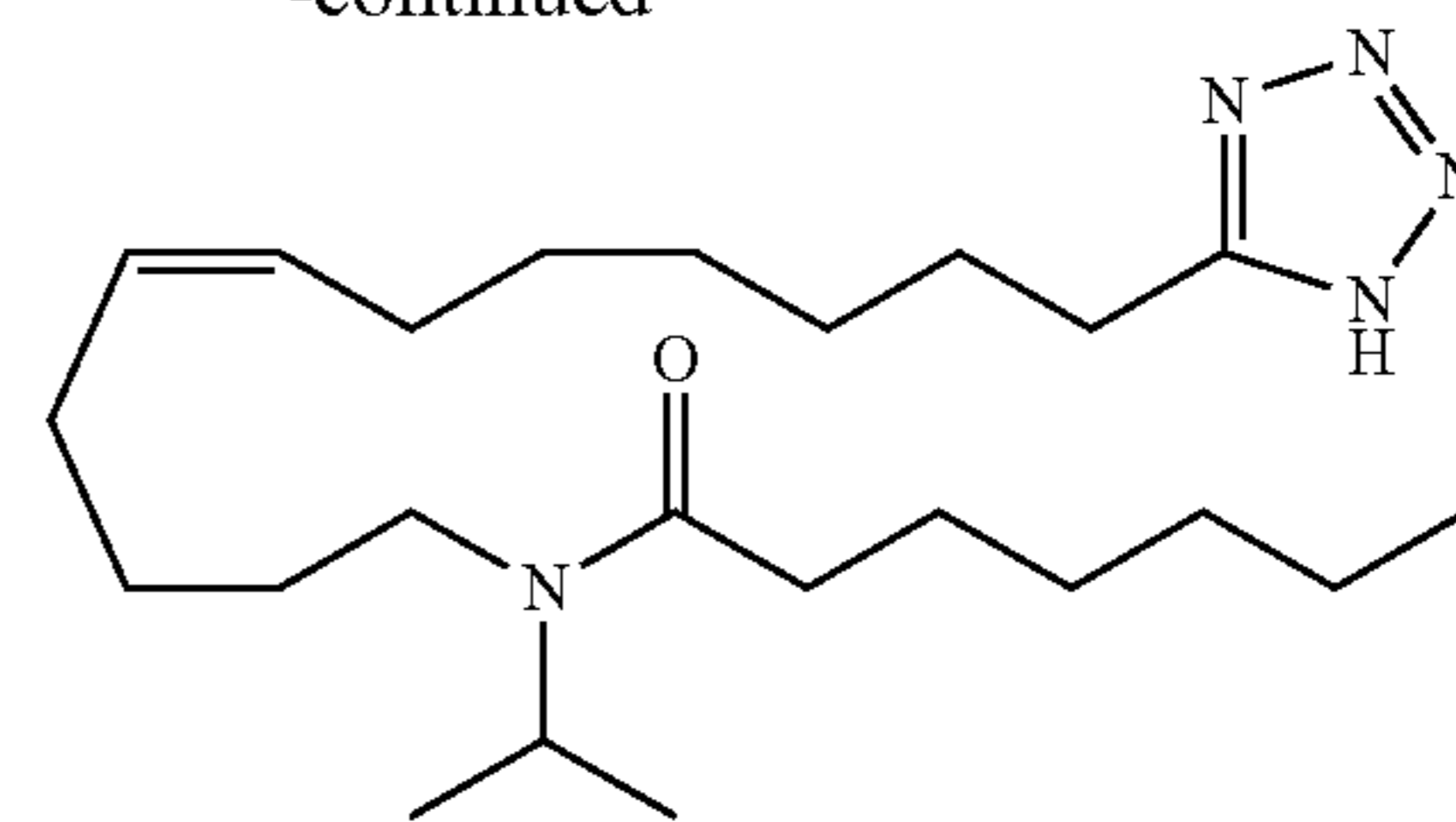
Analog 19
