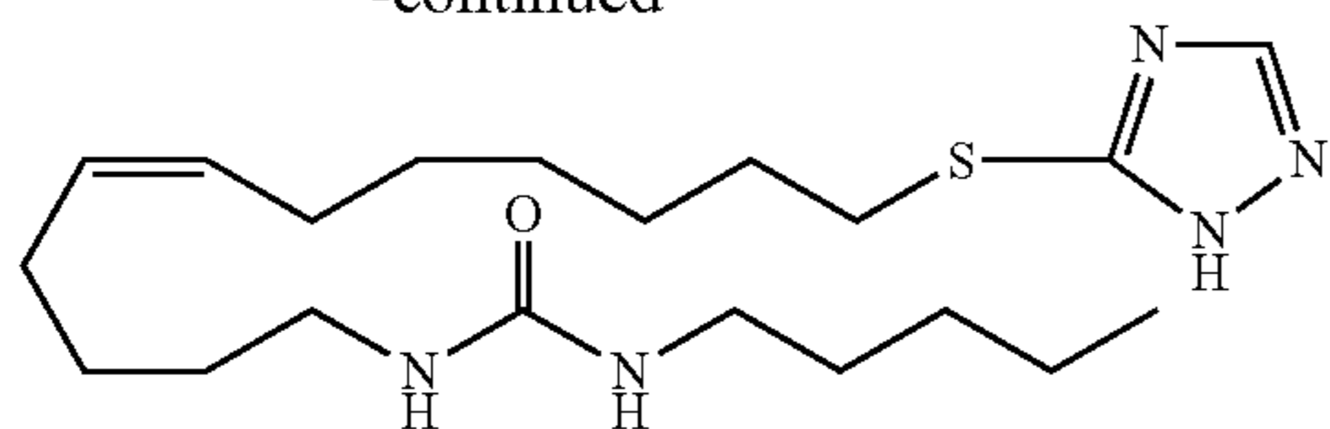
Analog 16
