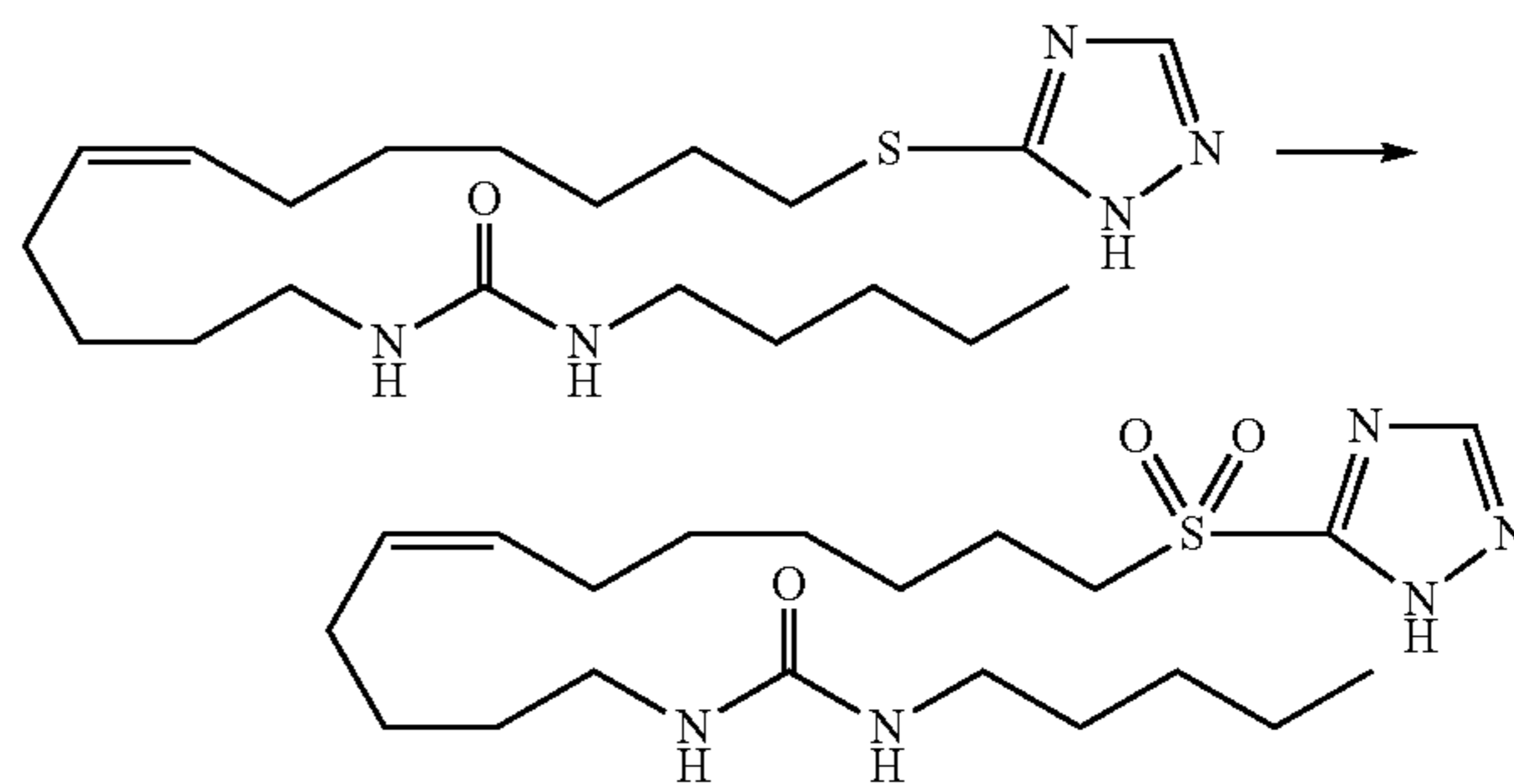
Analog 18
