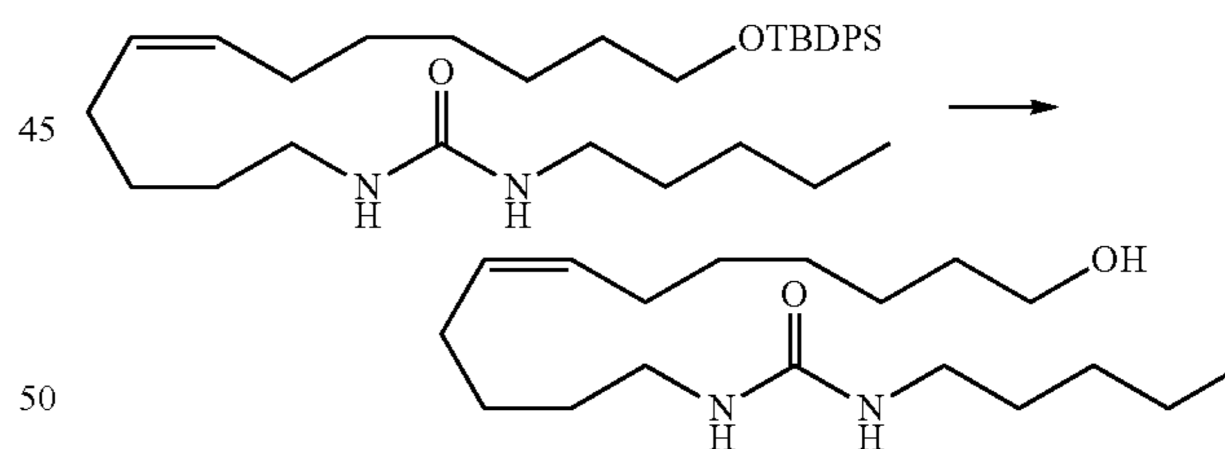
1-(12-Hydroxydodec-5(Z)-enyl)-3-n-pentylurea
