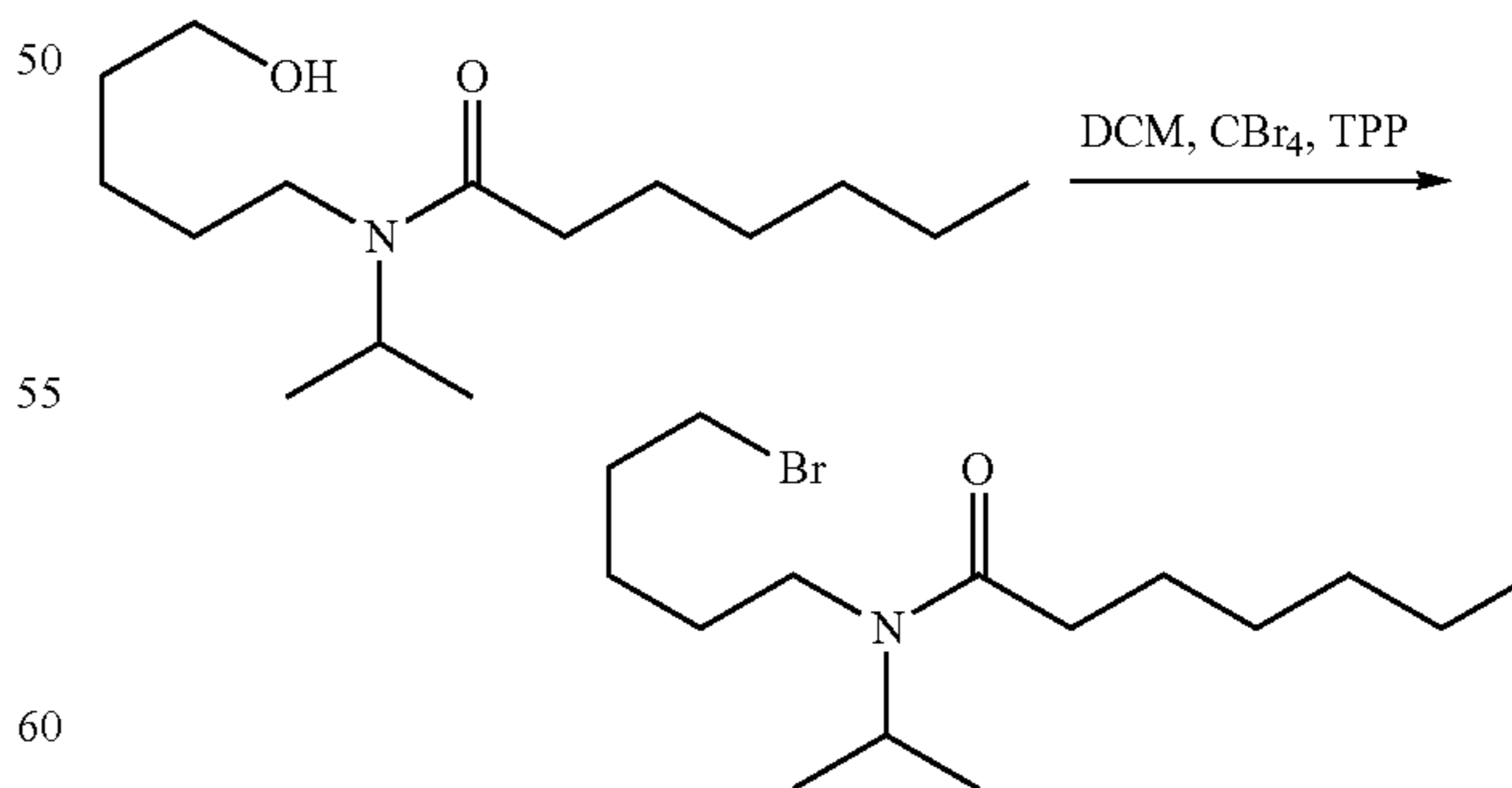
N-(5-Bromopentyl)-N-isopropylheptanamide (7)
