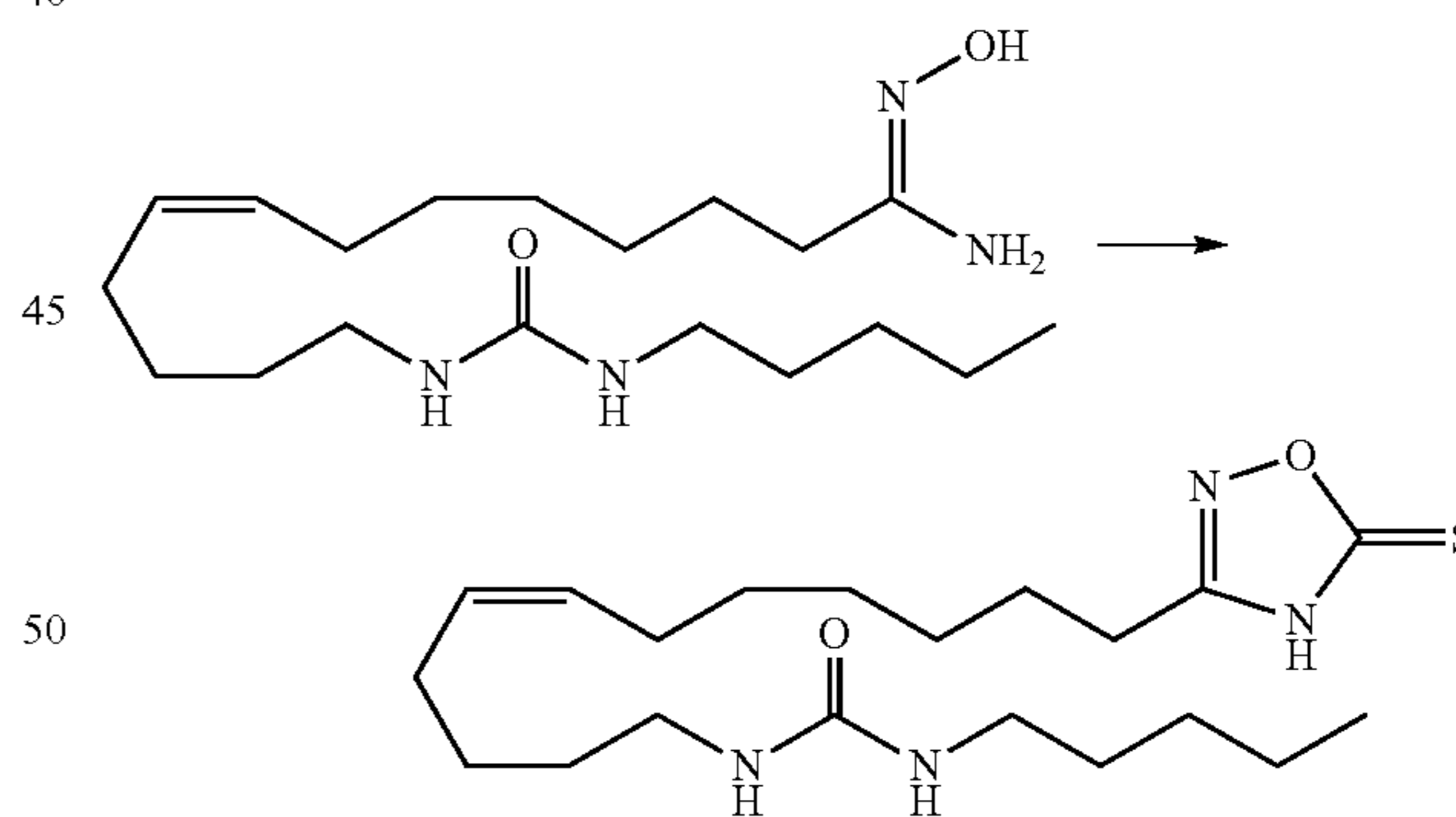
Analog 28
