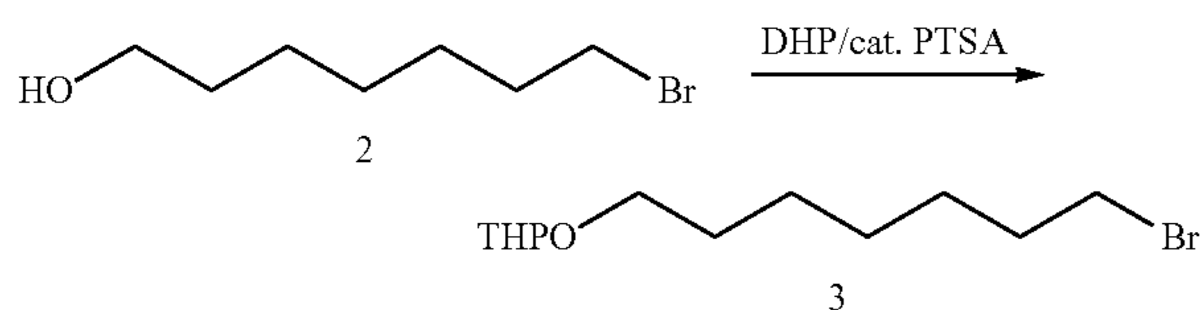
2-(7-Bromoheptyloxy)tetrahydro-2H-pyran 2 (3)
