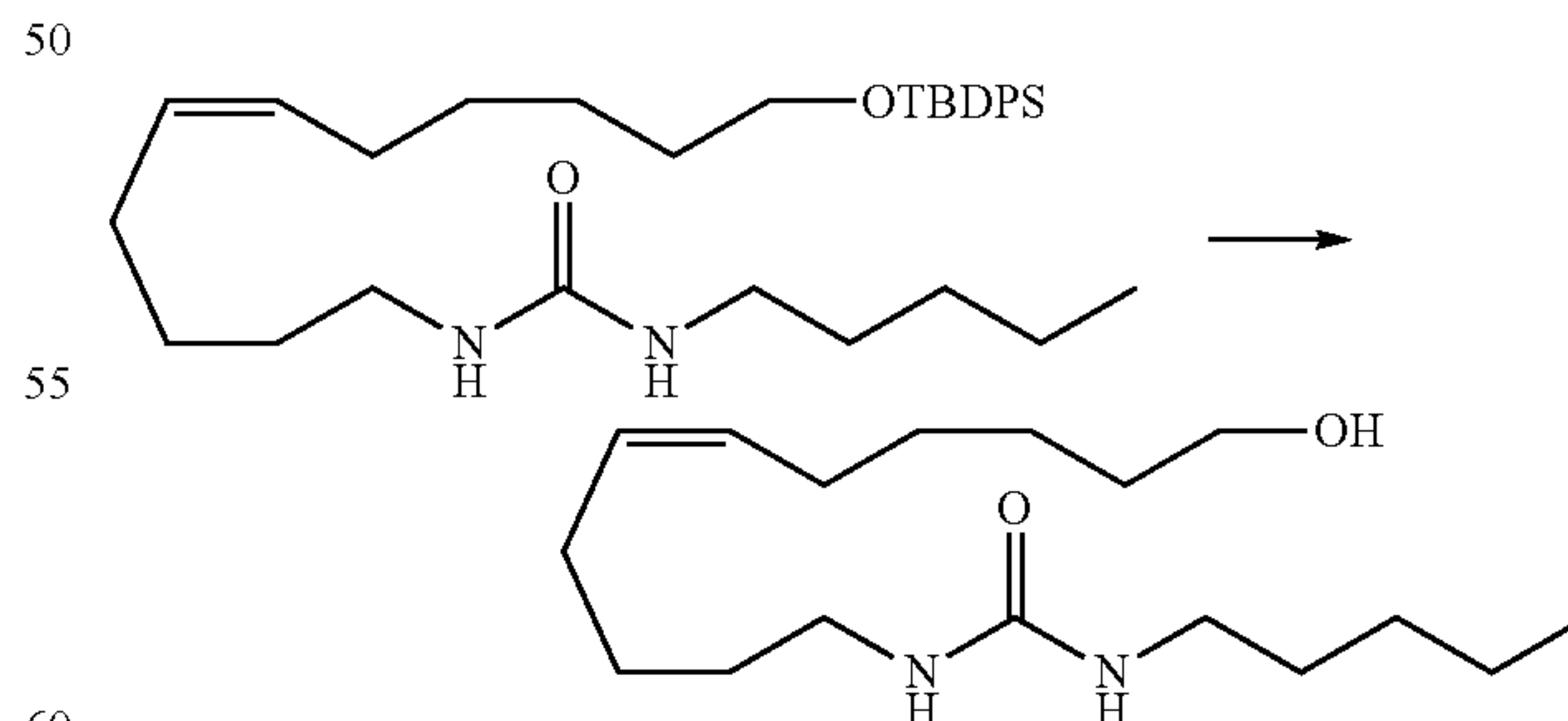
1-(11-Hydroxyundec-5(Z)-enyl)-3-n-pentylurea
