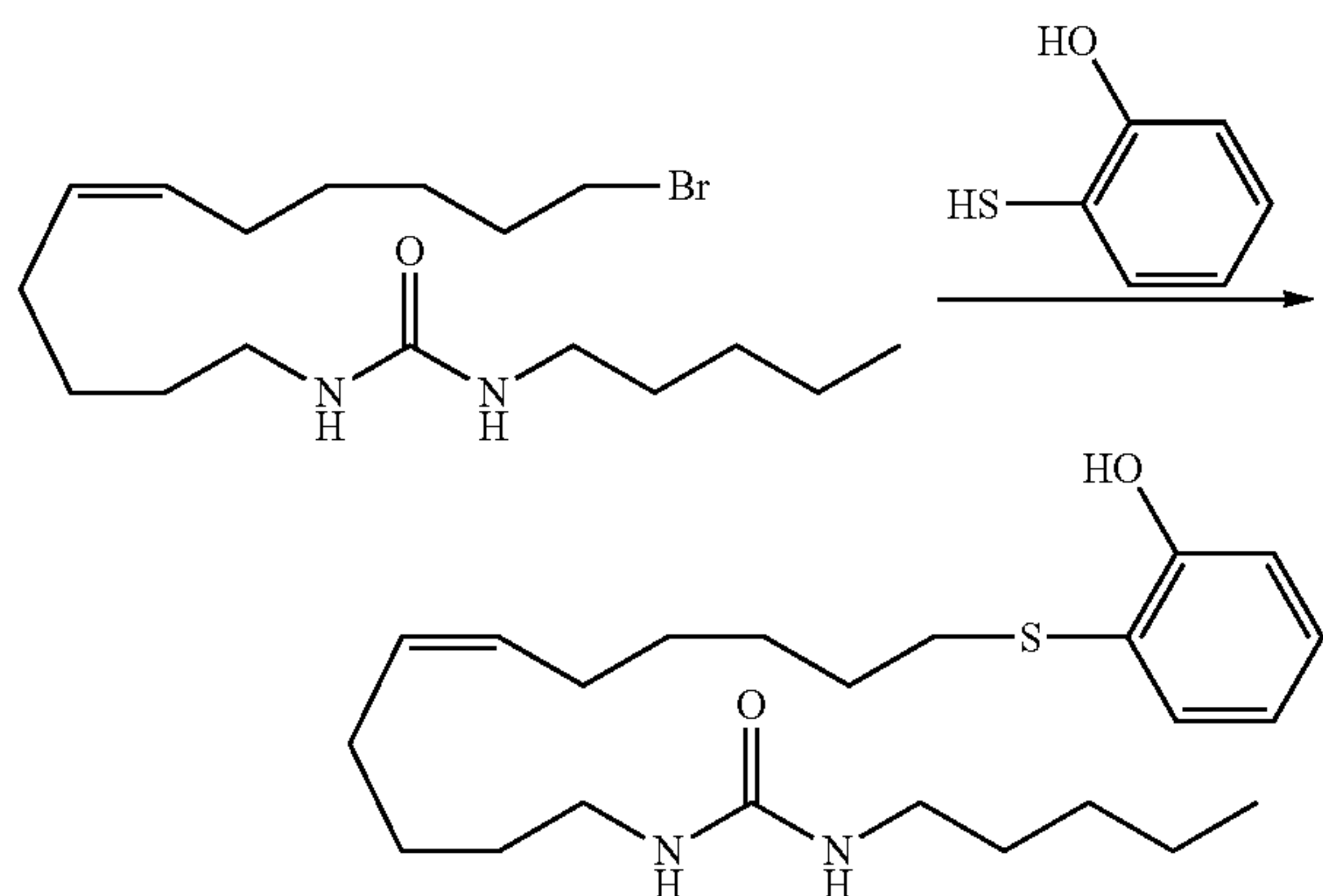
1-(11-(2-Hydroxyphenylthio)undec-5(Z)-enyl)-3-n-pentylurea (13)
