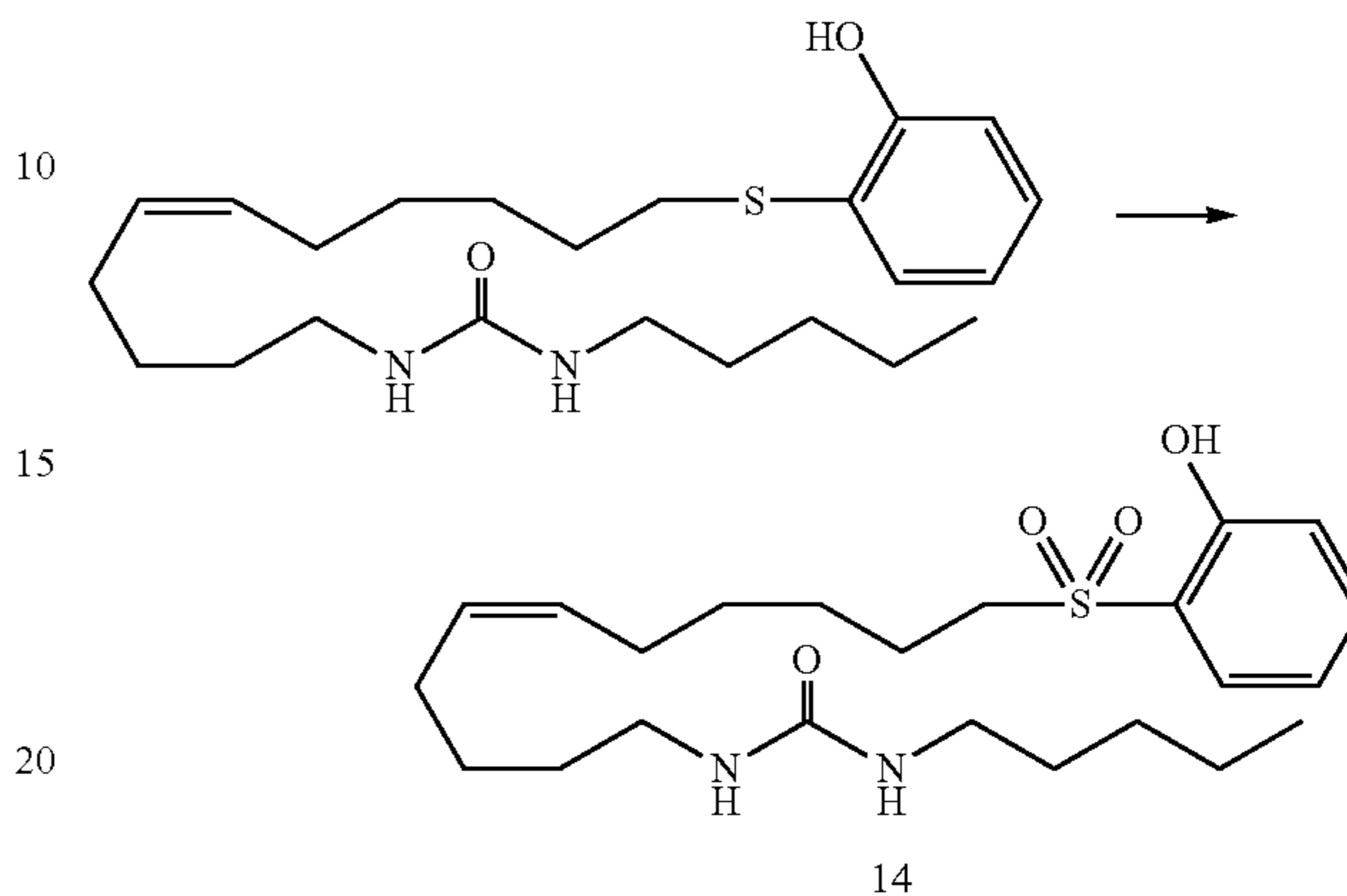
1-(11-(2-Hydroxyphenylsulfonyl)undec-5(Z)-enyl)-3-n-pentylurea (14)
