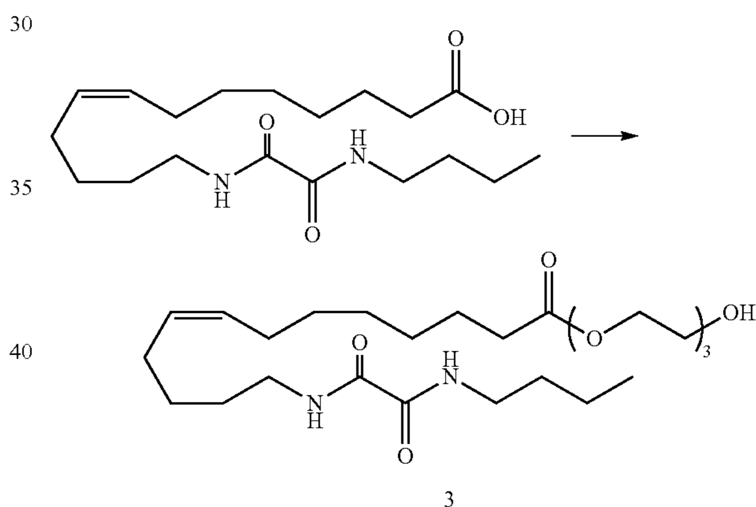
2-(2-(2-Hydroxyethoxy)ethoxy)ethyl 13-(2-(n-butylamino)-2-oxoacetamido)tridec-8(Z)-enoate (3)
