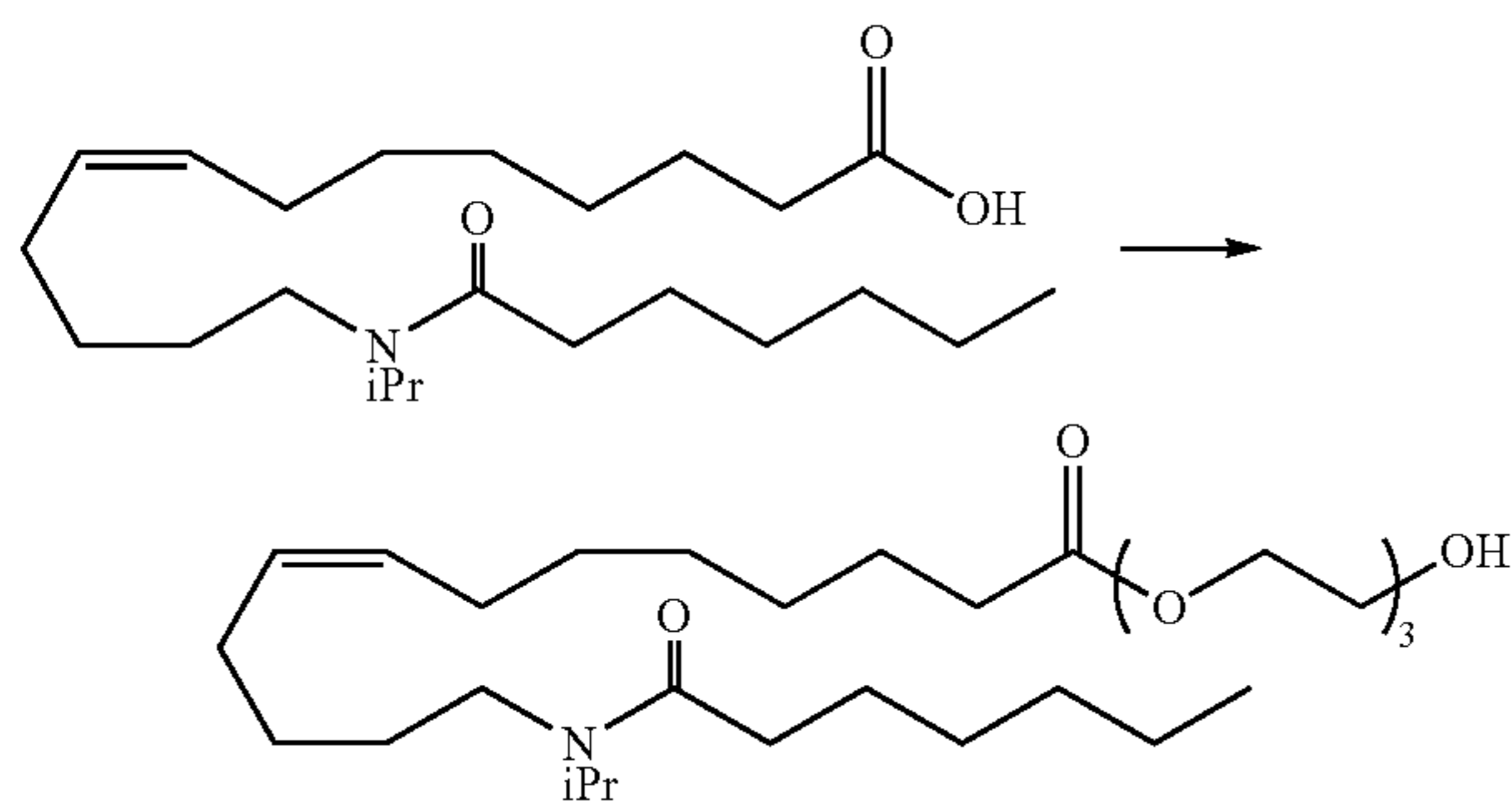
2-(2-(2-Hydroxyethoxy)ethoxy)ethyl 13-(N-isopropylheptanamido)tridec-8(Z)-enoate (1)
