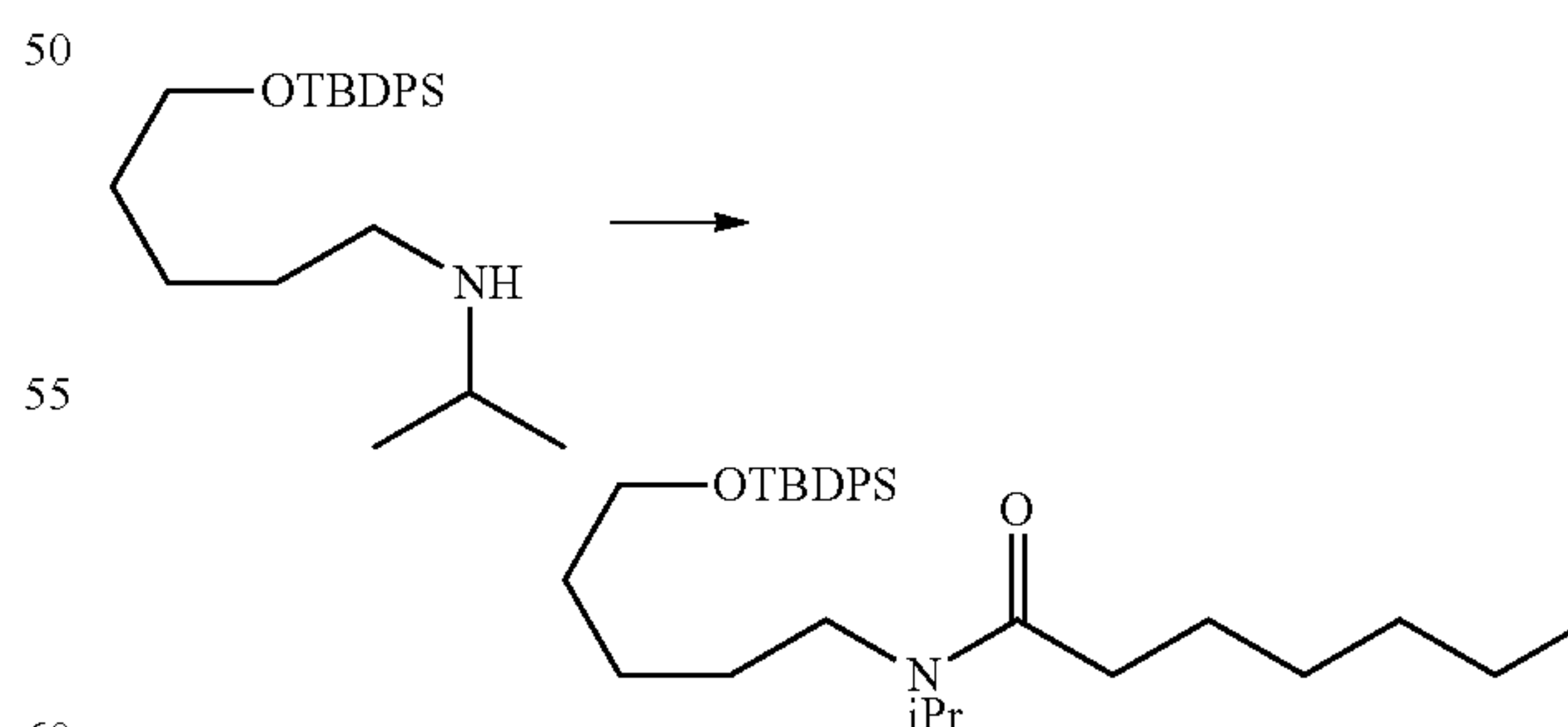
N-(5-(tert-Butyldiphenylsilyloxy)pentyl)-N-isopropylheptanamide
