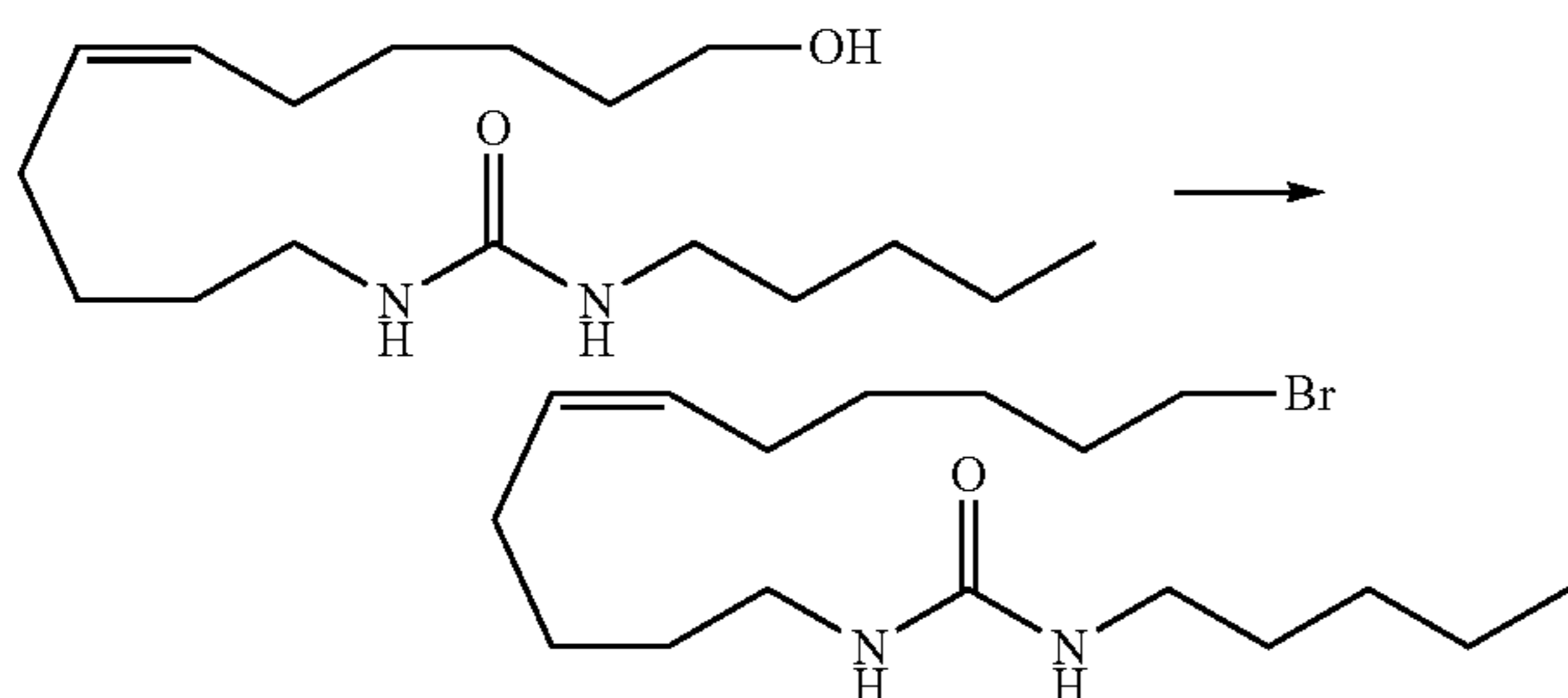
1-(11-Bromoundec-5(Z)-enyl)-3-n-pentylurea
