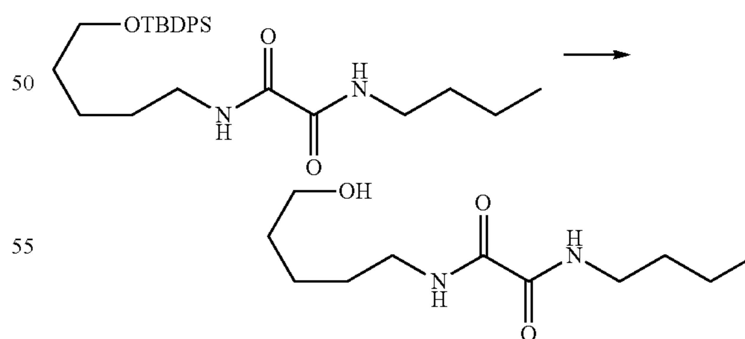
N 1 -n-Butyl-N 2 -(5-hydroxypentyl)oxalamide
