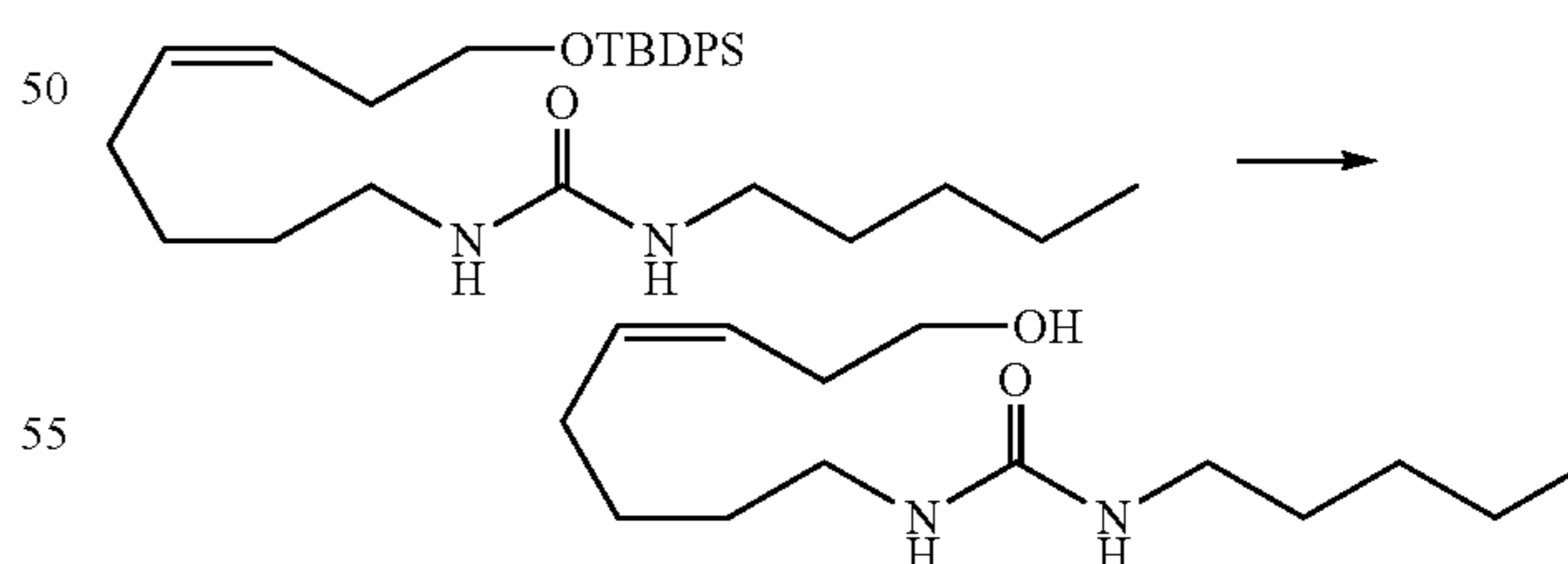
1-(8-Hydroxyoct-5(Z)-enyl)-3-n-pentylurea
