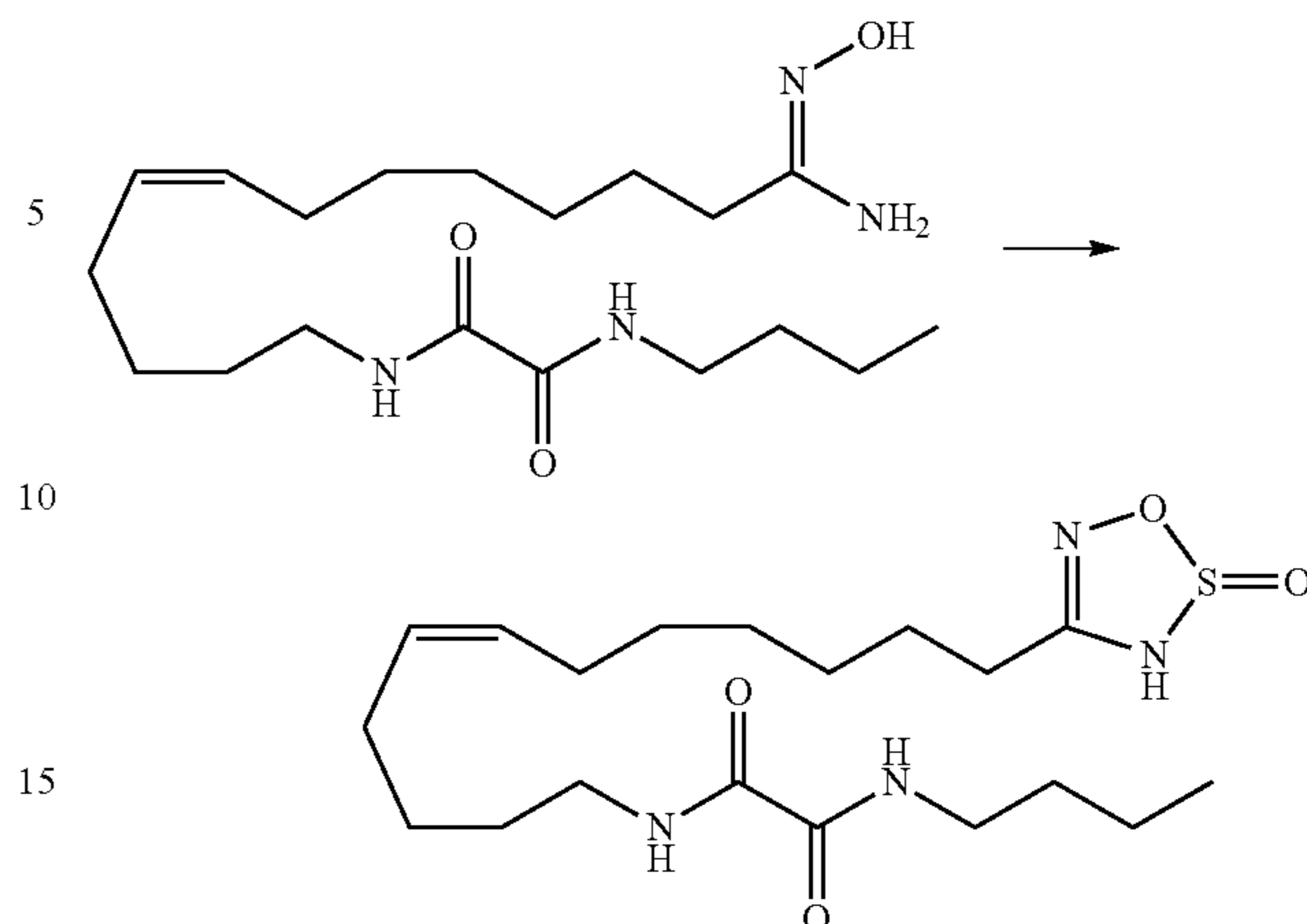
Analog 27
