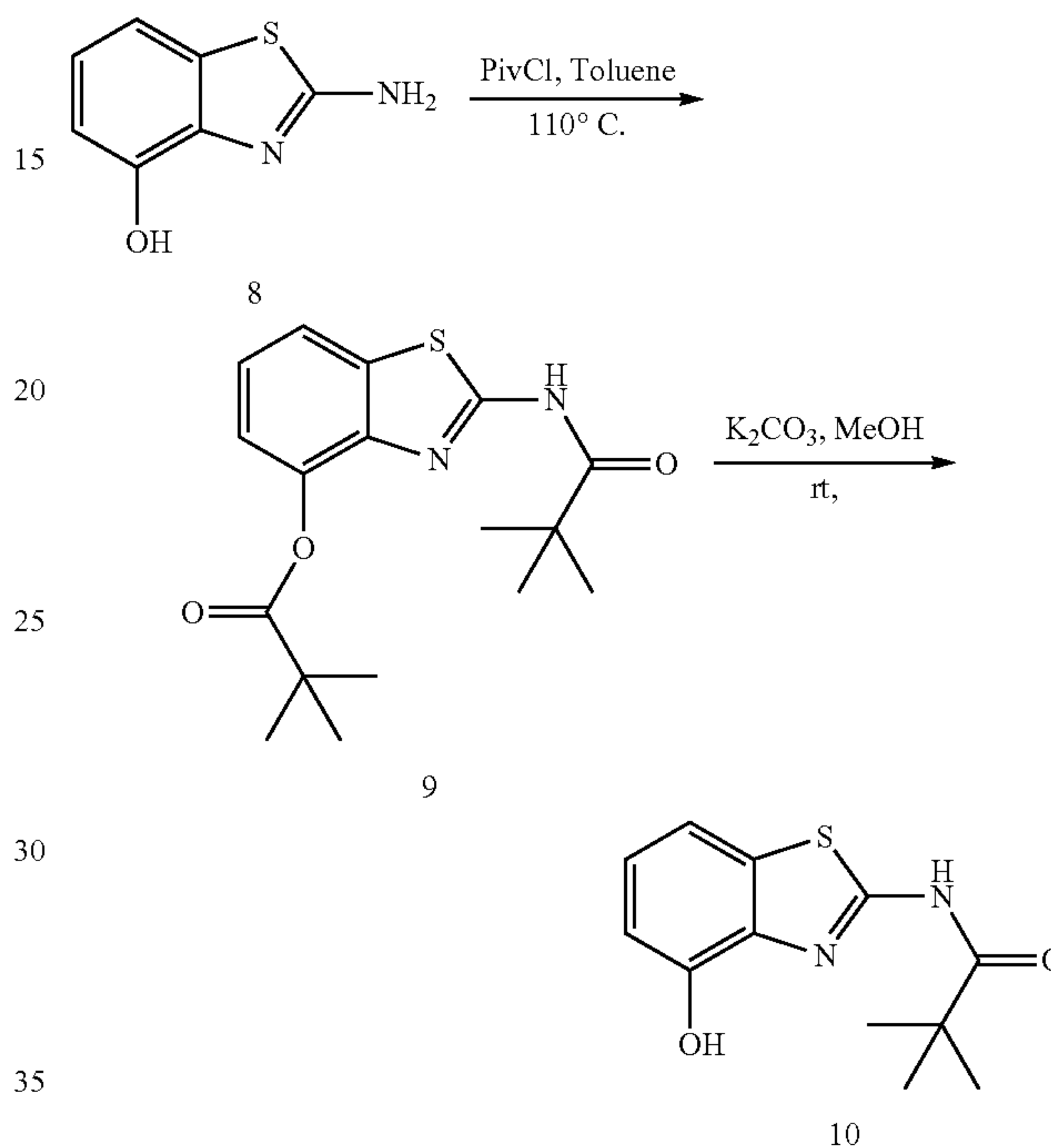
N-(4-hydroxybenzo[d]thiazol-2-yl)pivalamide (10)
