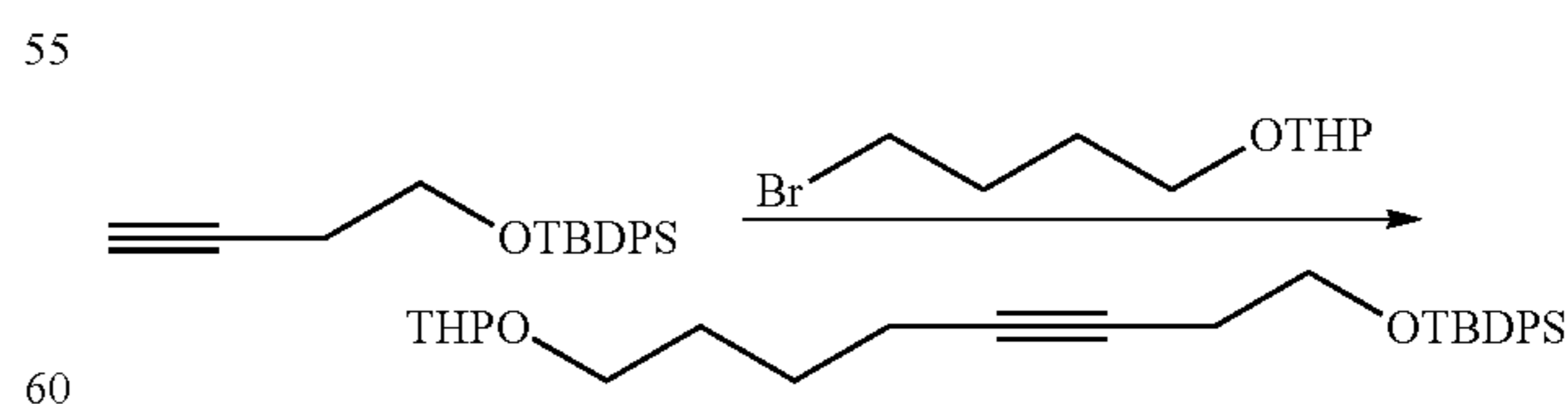
1-(tert-Butyldiphenylsilyloxy)-8-(tetrahydro-2H-pyran-2-yloxy)oct-3-yne
