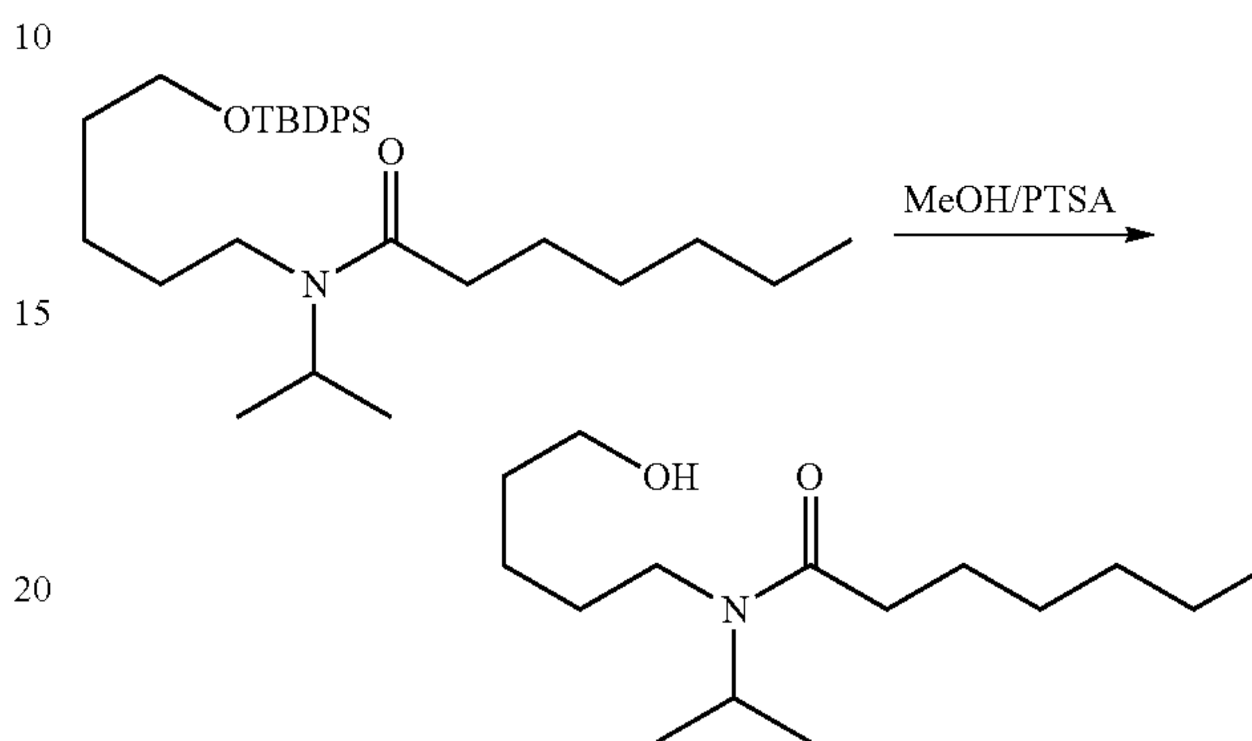
N-(5-hydroxypentyl)-N-isopropylheptanamide (6)
