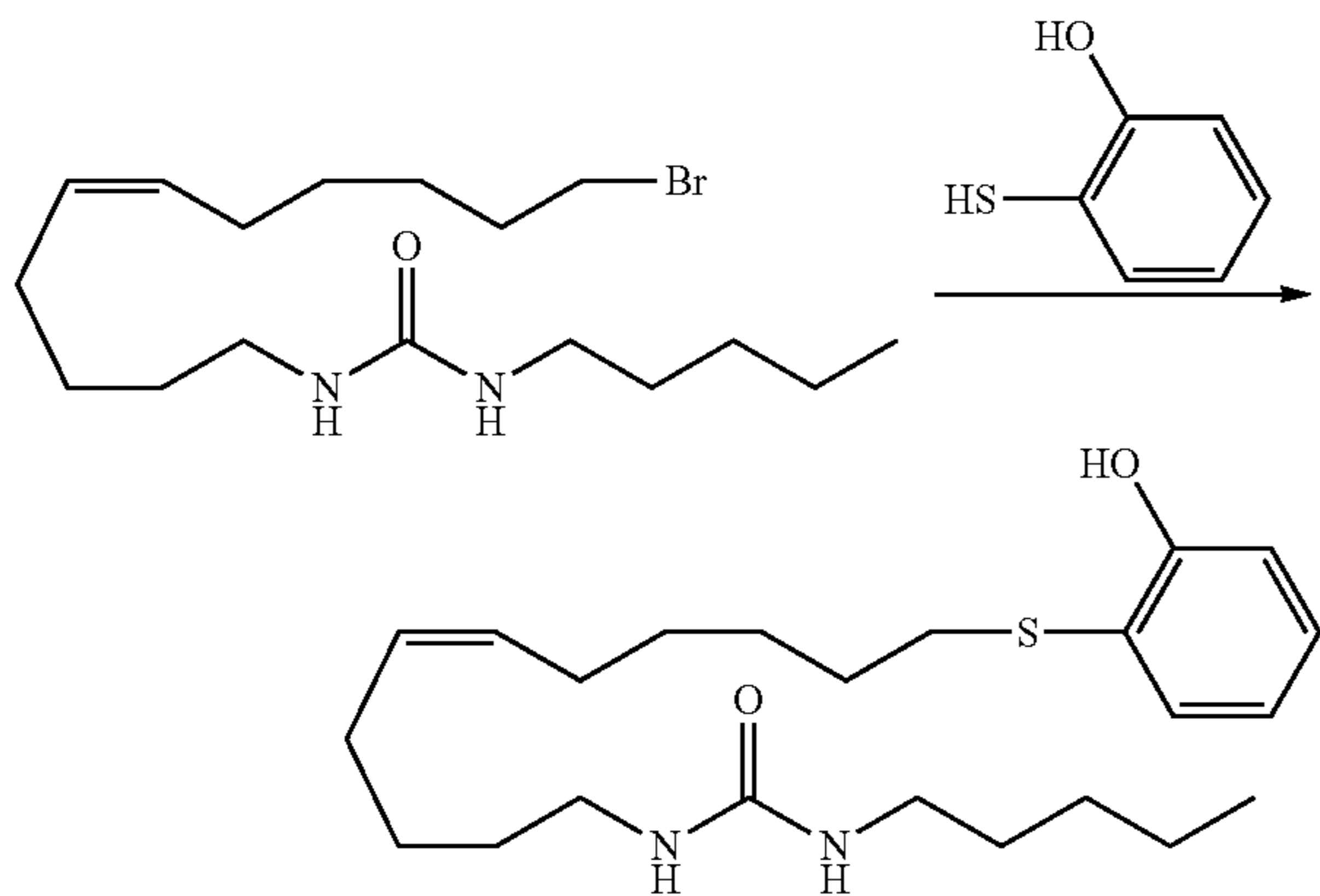
1-(11-(2-Hydroxyphenylthio)undec-5(Z)-enyl)-3-n-pentylurea (13)
