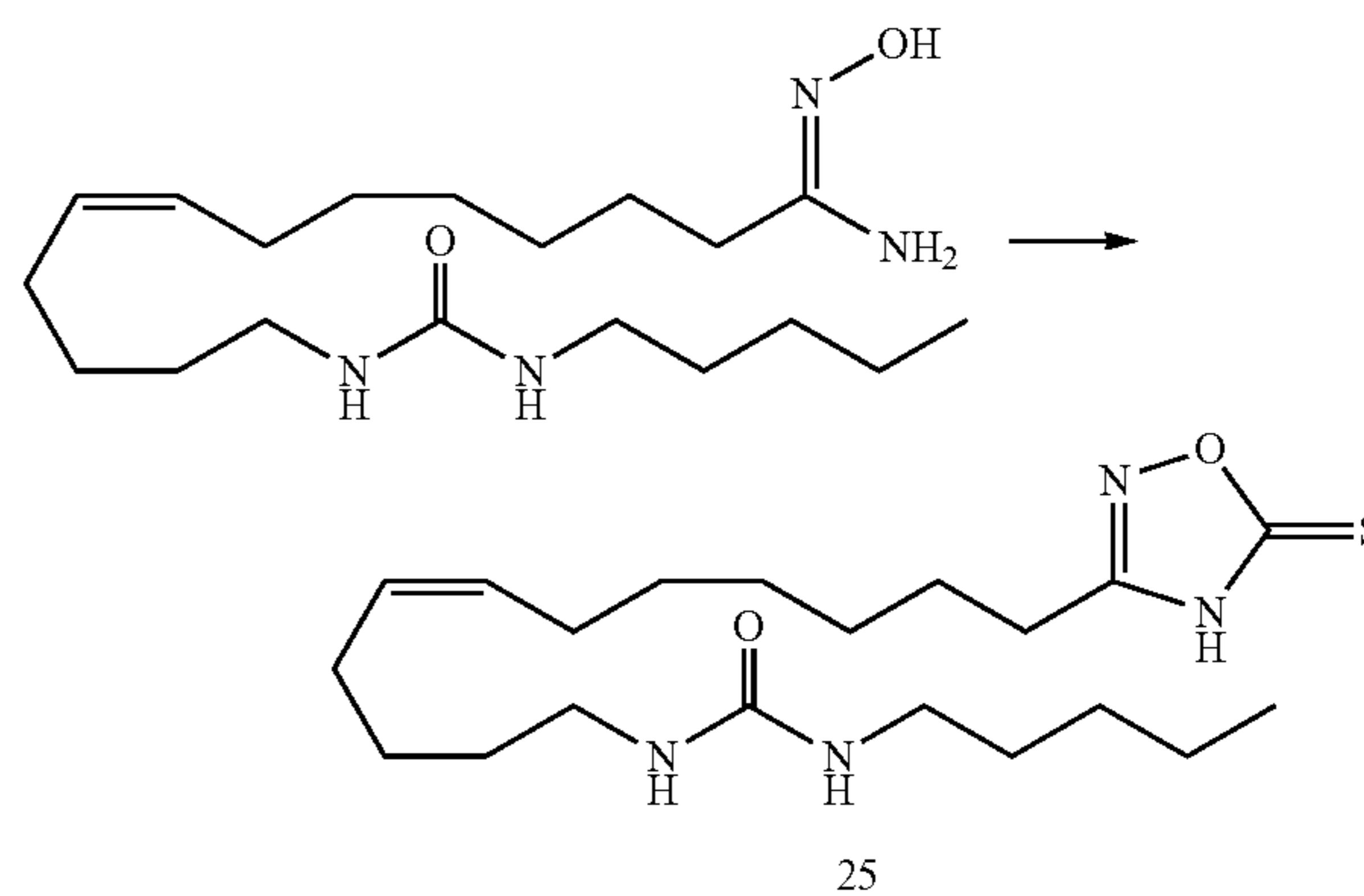
Analog 25
