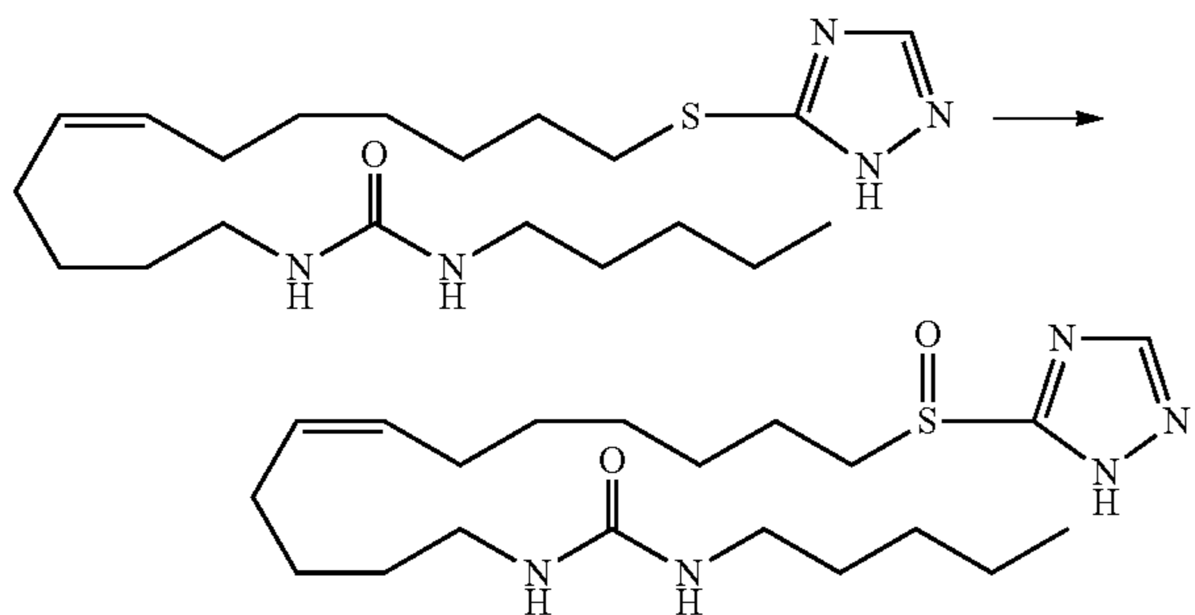
Analog 17
