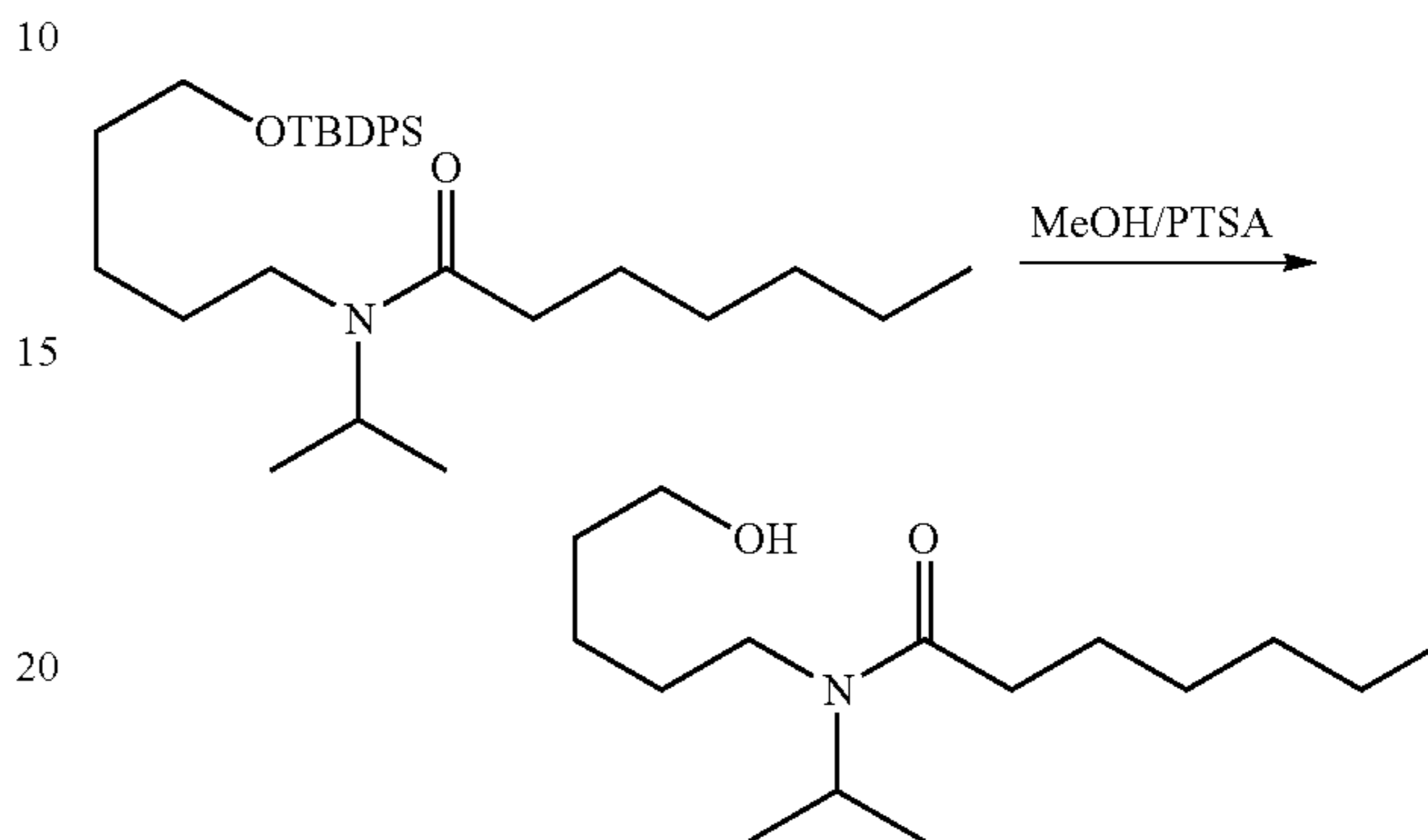
N-(5-hydroxypentyl)-N-isopropylheptanamide (6)
