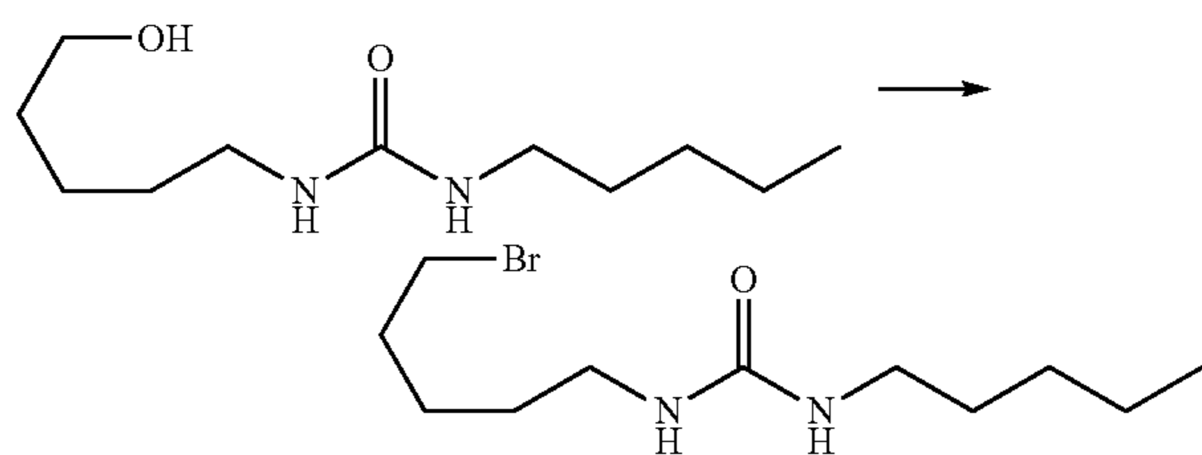
1-(5-Bromopentyl)-3-n-pentylurea
