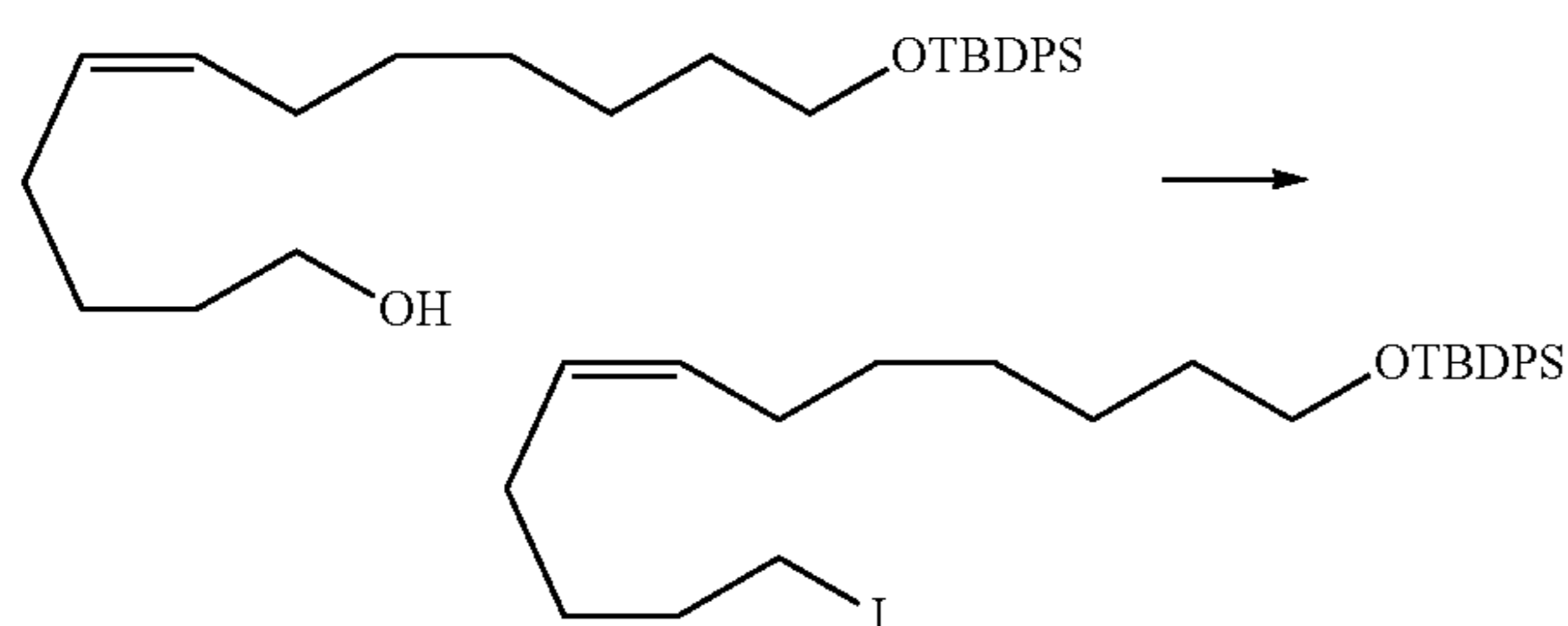
1-(tert-Butyldiphenylsilyloxy-12-Iodododec-7(Z)-ene
