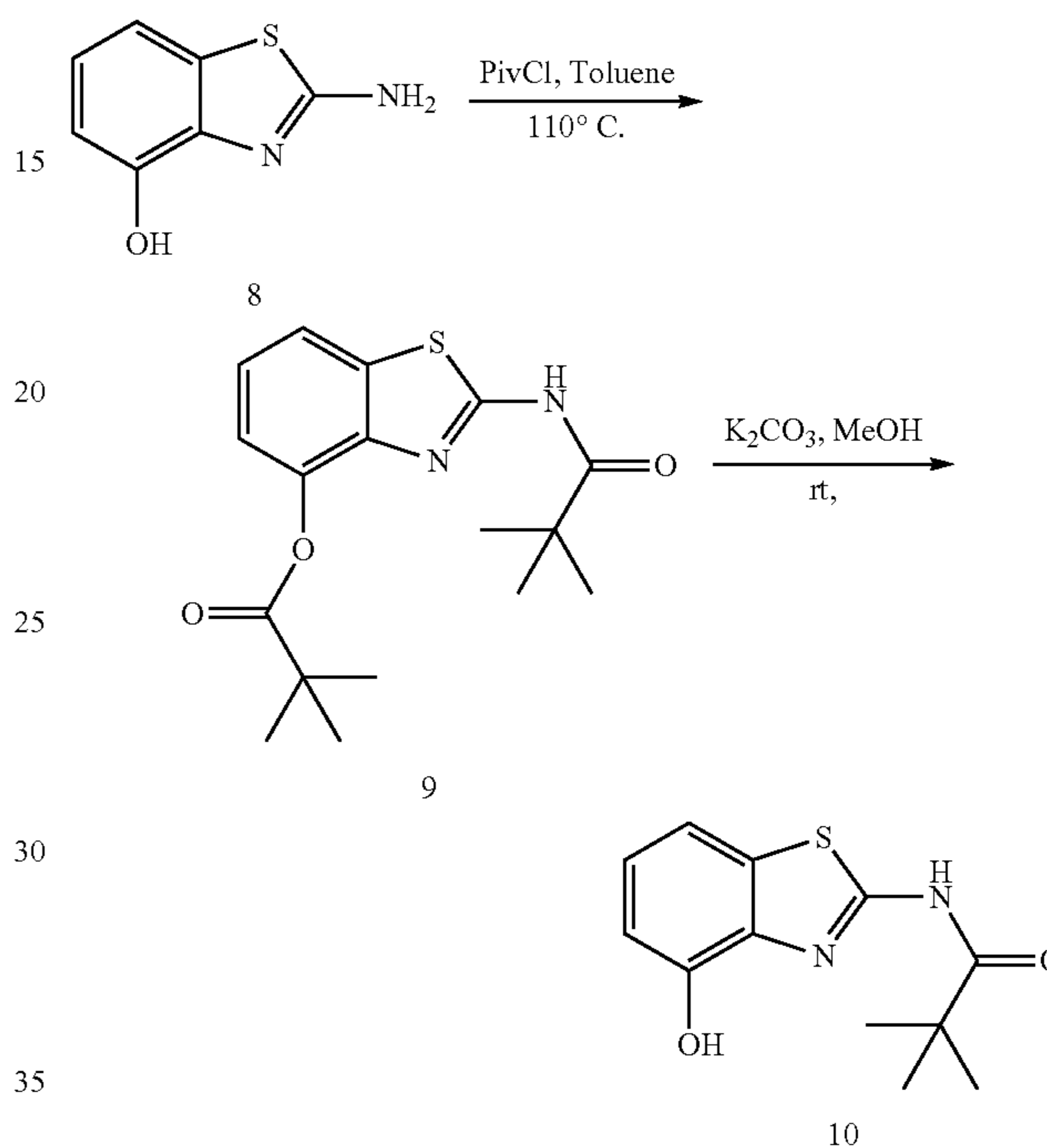
N-(4-hydroxybenzo[d]thiazol-2-yl)pivalamide (10)
