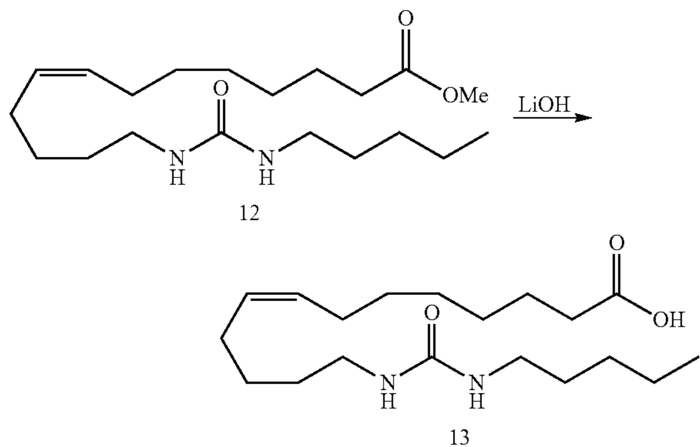
Methyl 13-(3-pentylureido)tridec-8(Z)-enoic acid 7 (13)
