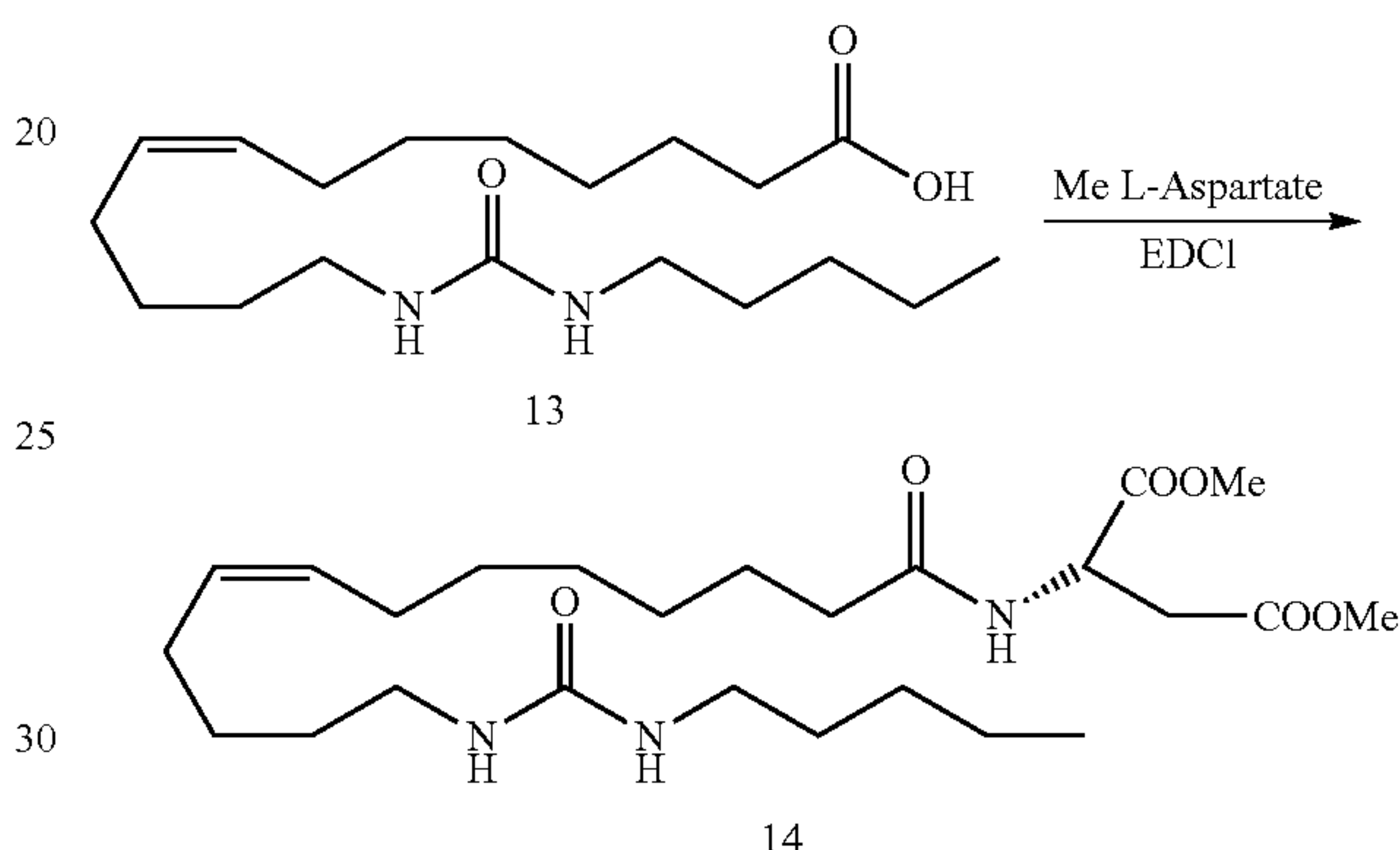
(S)-2-(13-(3-Pentylureido)tridec-8(Z)-enamido)succinate (14)
