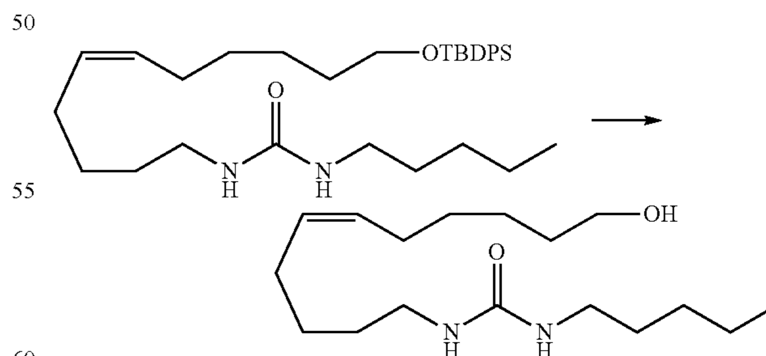
1-(11-Hydroxyundec-5(Z)-enyl)-3-n-pentylurea
