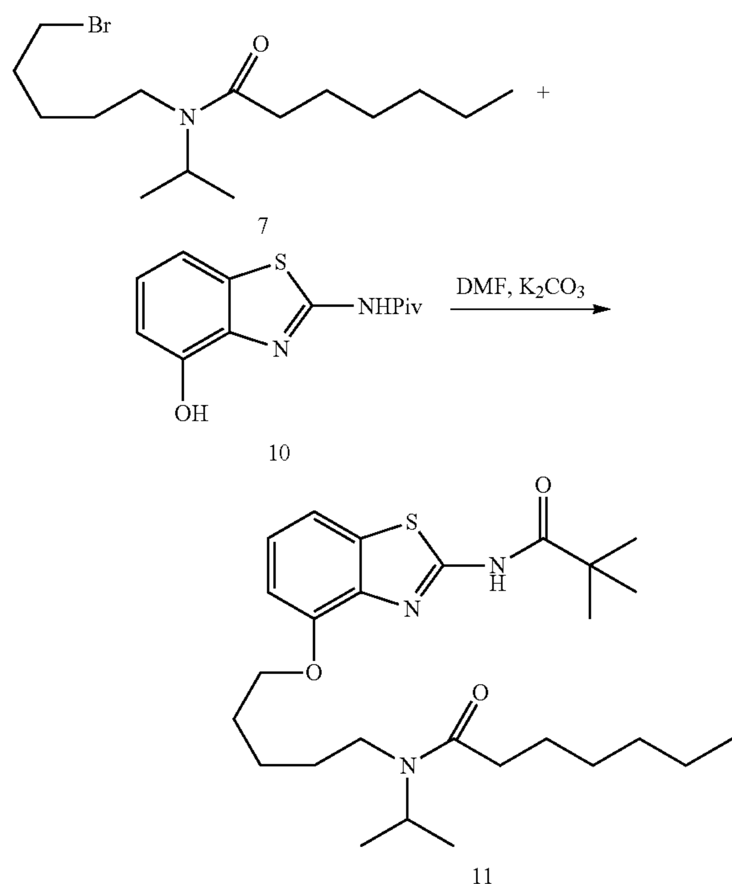
Isopropyl-N-(5-(2-pivalamidobenzo[d]thiazol-4-yloxy)pentyl)heptanamide (11)
