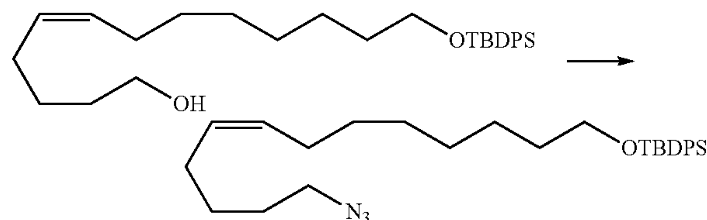
1-tert-Butyldiphenylsilyloxy-13-azidotridec-8(Z)-ene
