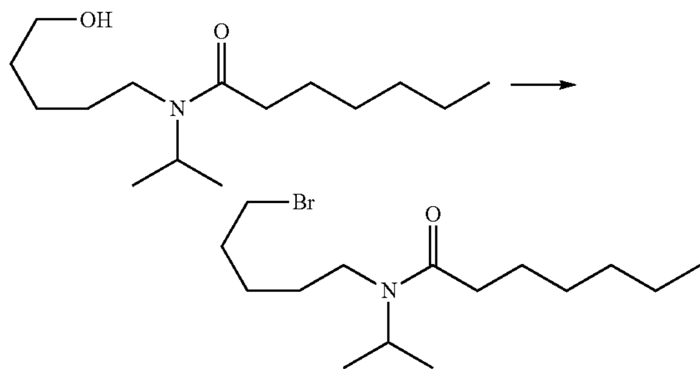
N-(5-Bromopentyl)-N-isopropylheptanamide
