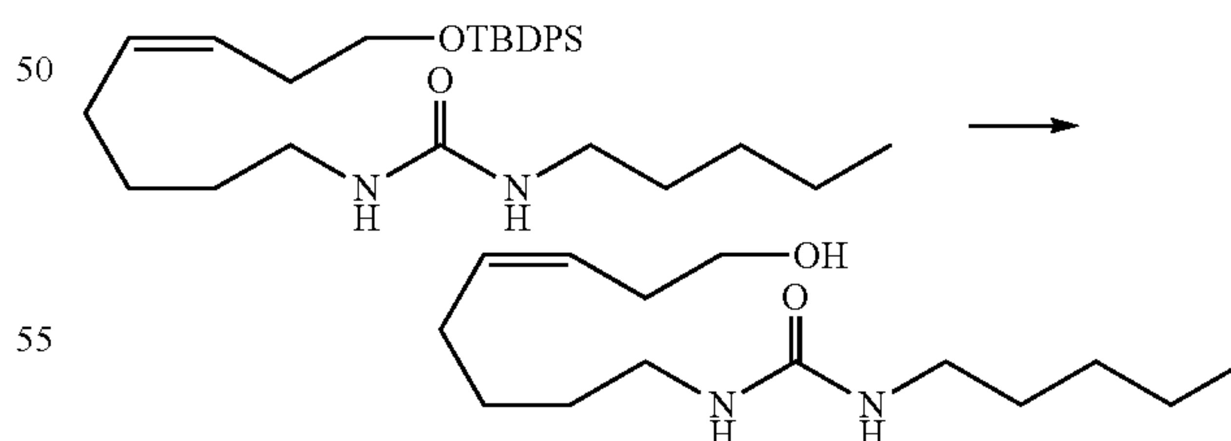
1-(8-Hydroxyoct-5(Z)-enyl)-3-n-pentylurea
