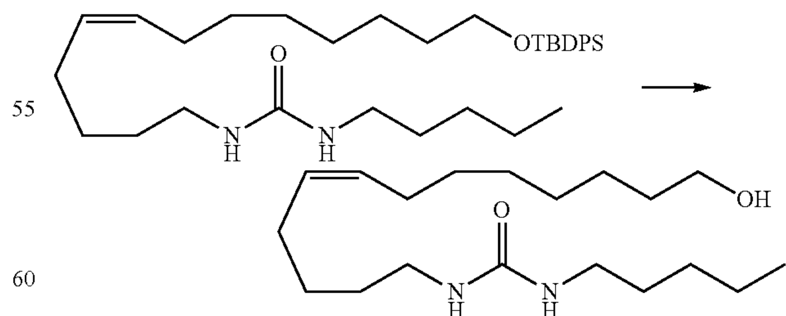
1-(13-Hydroxytridec-5(Z)-enyl)-3-n-pentylurea
