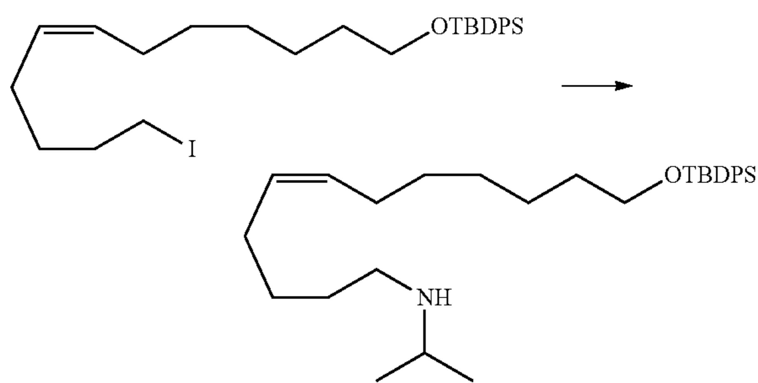
1-(tert-Butyldiphenylsilyloxy-12-N-isopropylamino-dodec-7(Z)-ene
