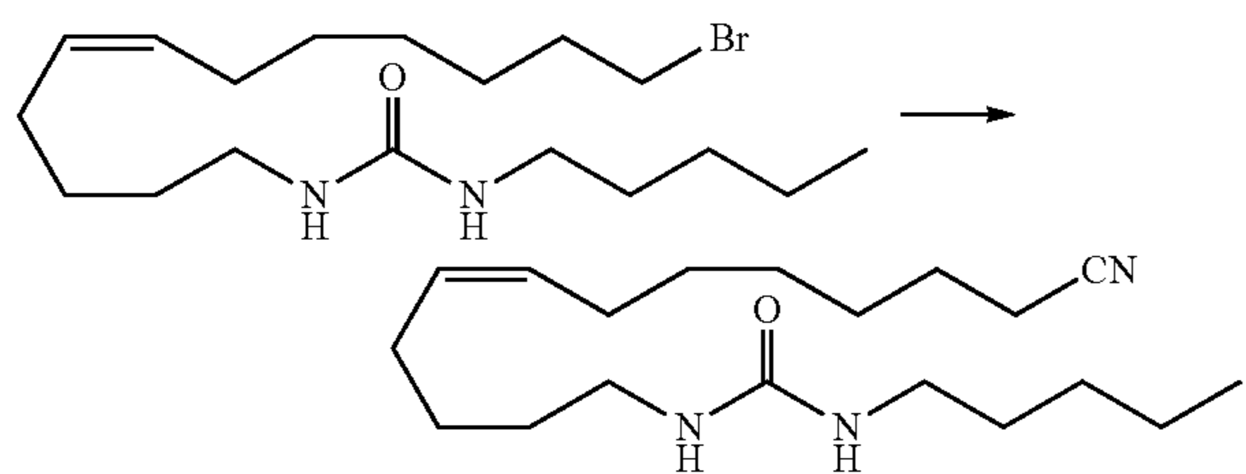
1-(12-Cyanododec-5(Z)-enyl)-3-n-pentylurea
