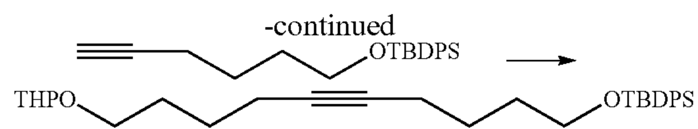
1-(Tetrahydro-2H-pyran-2-yloxy)-100-(tert-butyl-diphenylsilyloxy)dec-5-yne
