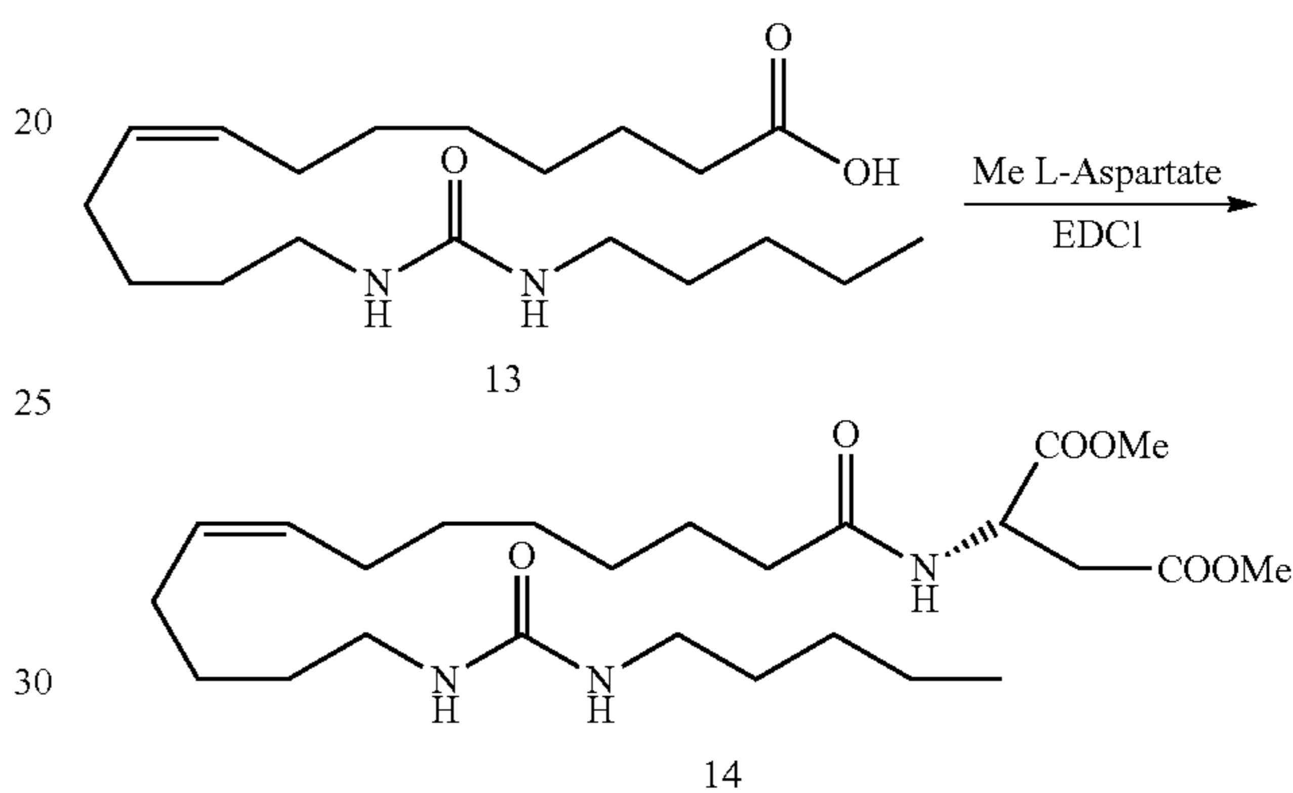
(S)-2-(13-(3-Pentylureido)tridec-8(Z)-enamido)succinate (14)
