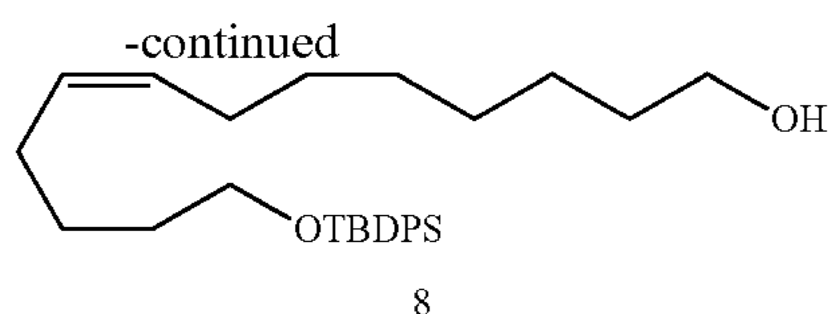
13-(tert-Butyldiphenylsilyloxy)tridec-8(Z)-en-1-ol (8)
