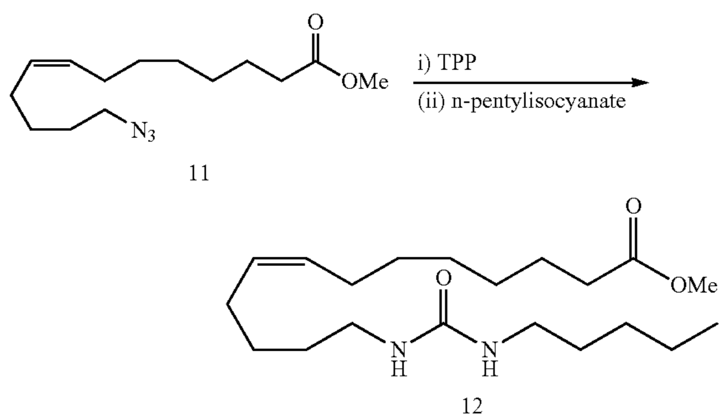
Methyl 13-(3-pentylureido)tridec-8(Z)-enoate 6 (12)
