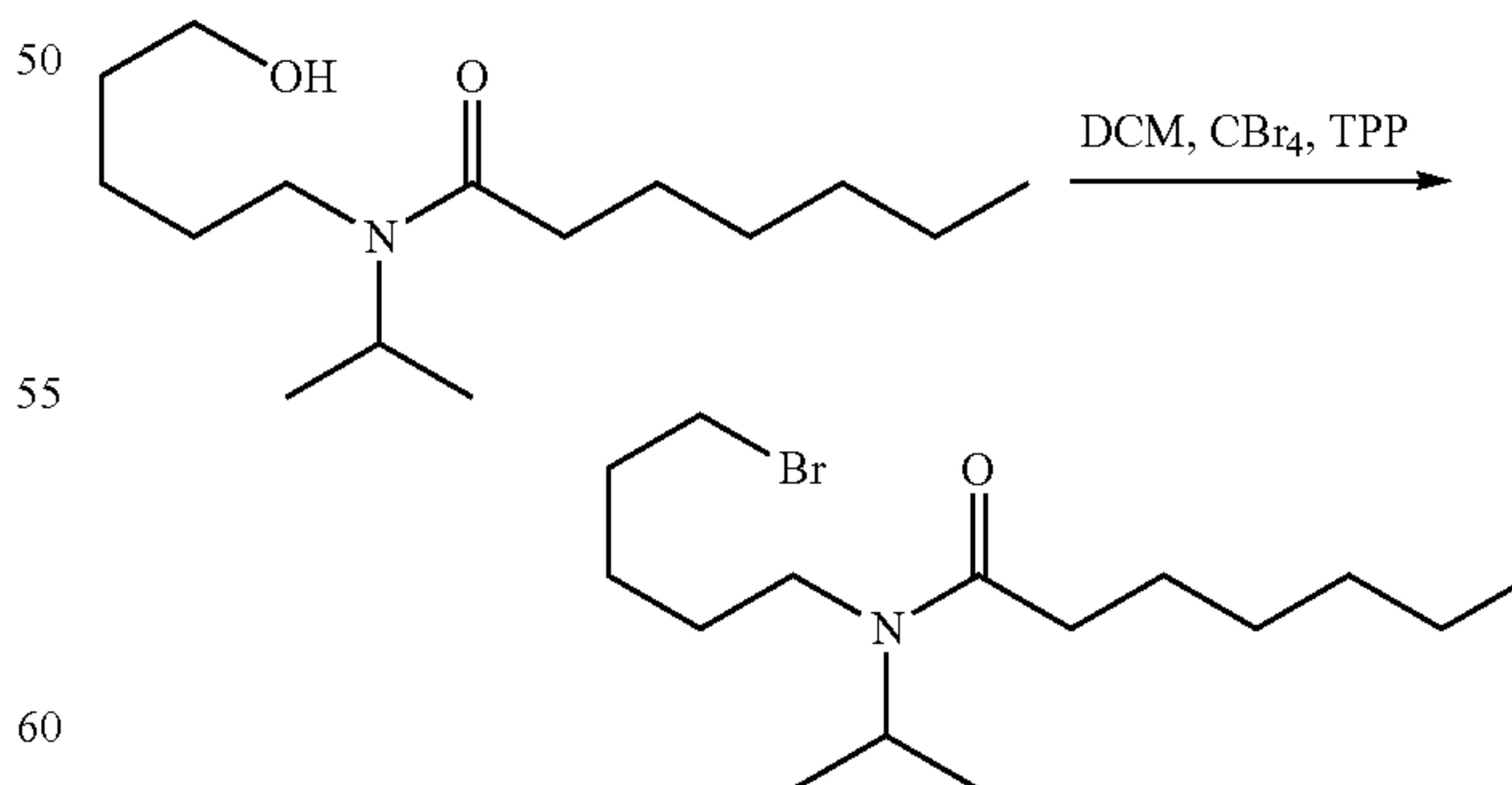
N-(5-Bromopentyl)-N-isopropylheptanamide (7)
