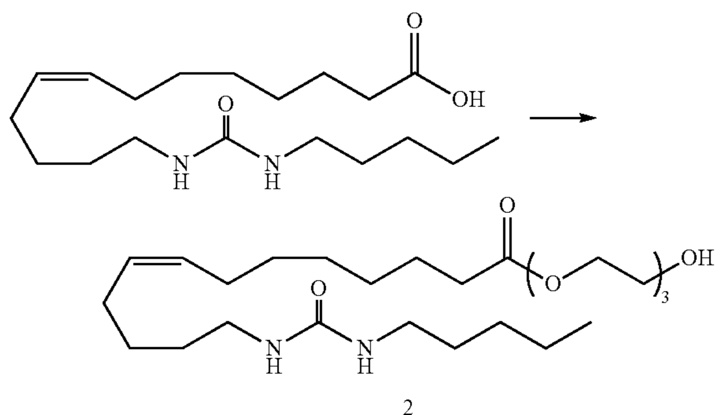
2-(2-(2-Hydroxyethoxy)ethoxy)ethyl 13-(3-n-pentylureido)tridec-8(Z)-enoate (2)
