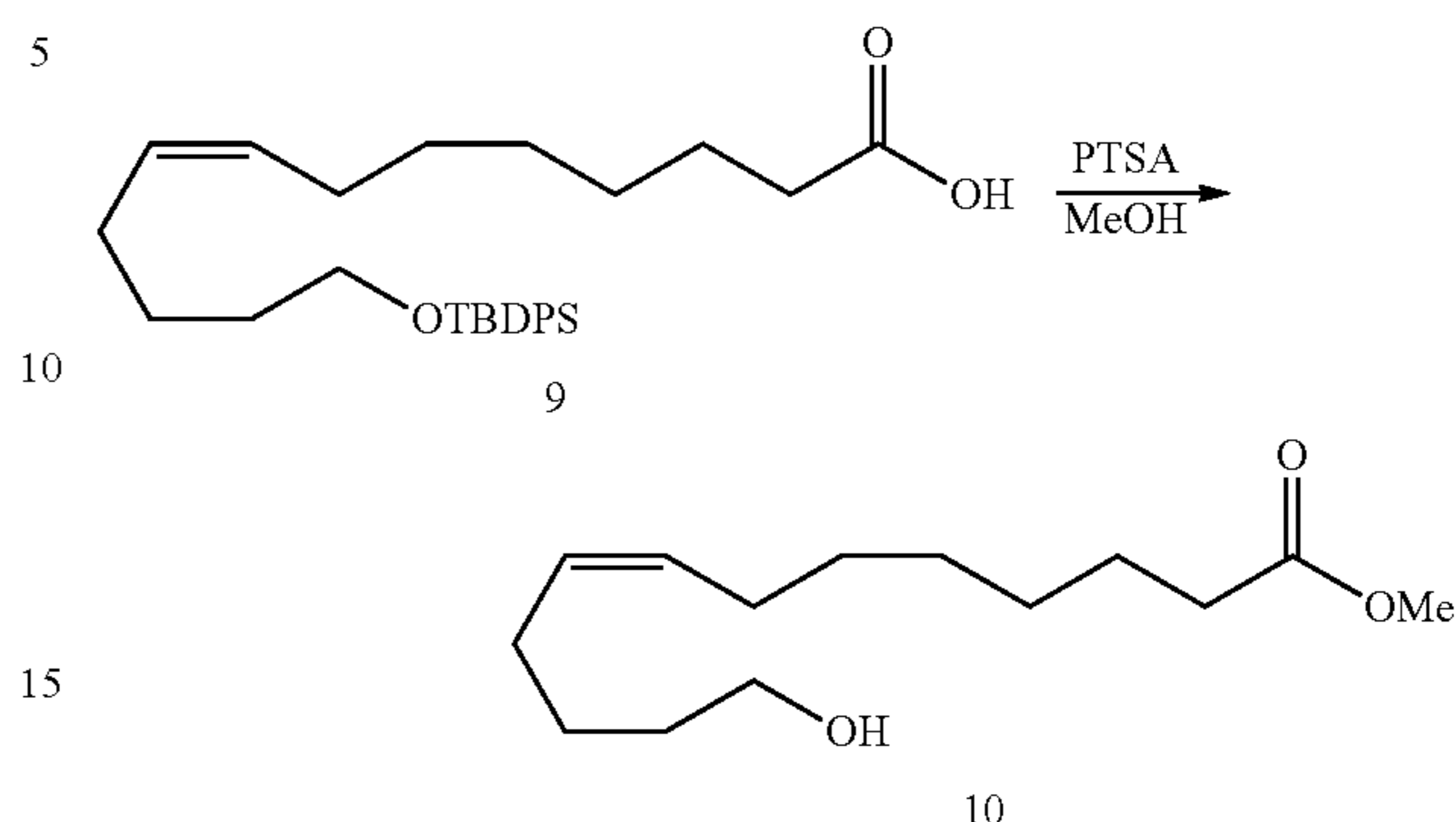
Methyl β-hydroxytridec-8(Z)-enoate 4 (10)
