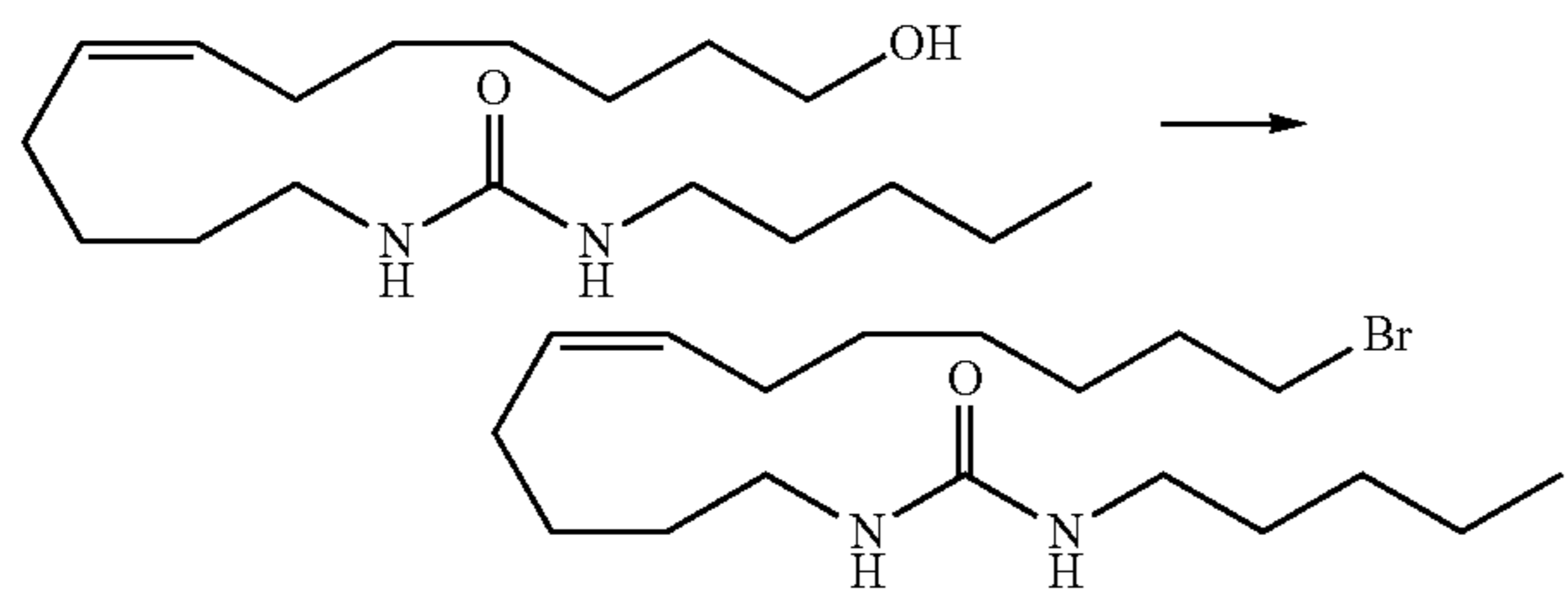
1-(12-Bromododec-5(Z)-enyl)-3-n-pentylurea
