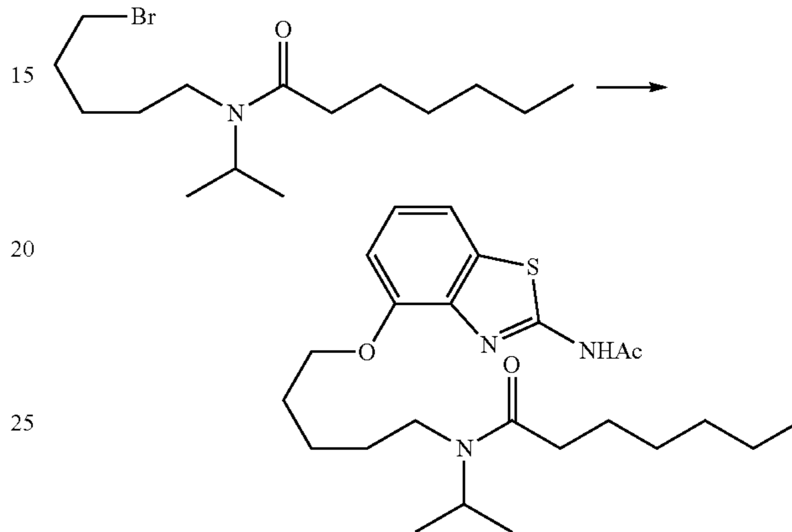
N-(5-(2-Acetamidobenzo[d]thiazol-4-yloxy)pentyl)-N-isopropylheptanamide (30)
