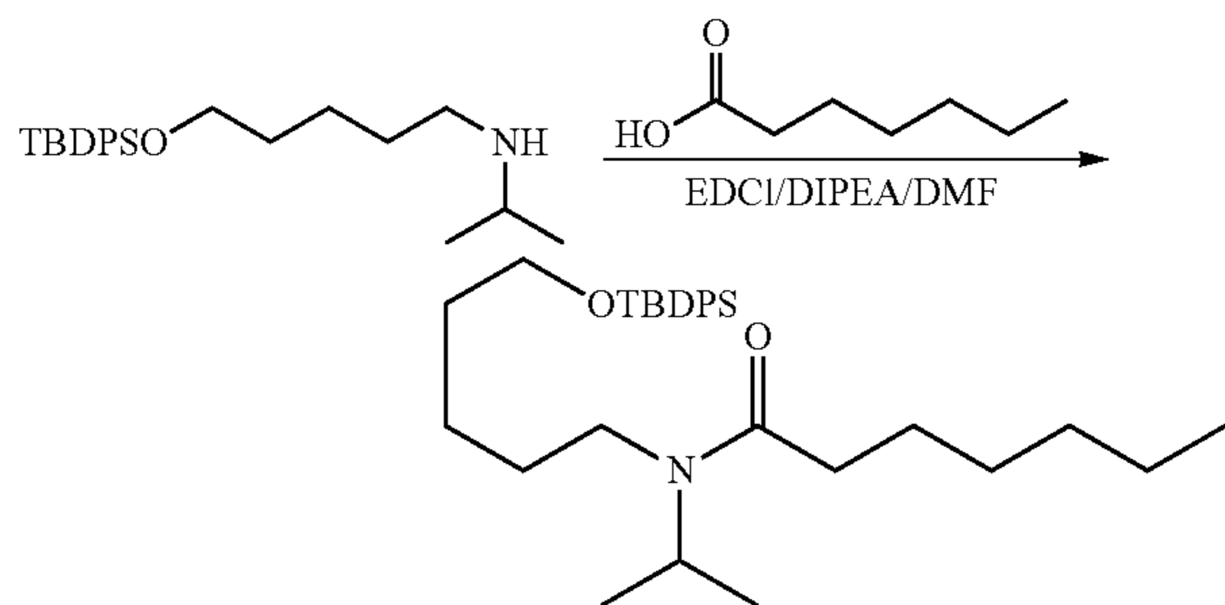
N-(5-(tert-Butyldiphenylsilyloxy)pentyl)-N-isopropylheptanamide (5)
