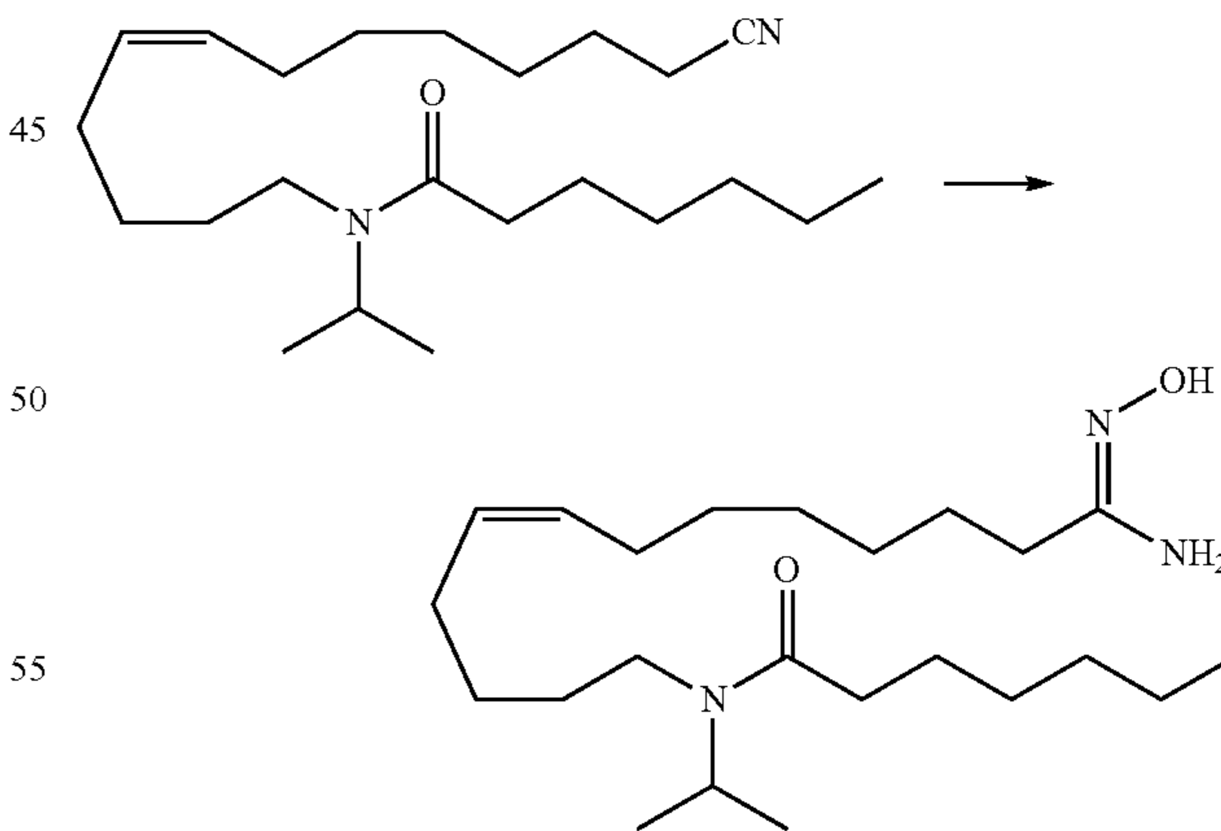
N-(13-Amino-13-(hydroxyimino)tridec-5(Z)-enyl)-N-isopropyl-n-heptanamide
