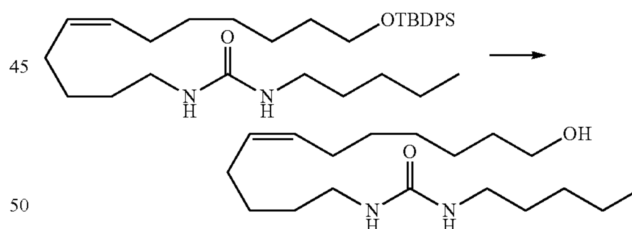
1-(12-Hydroxydodec-5(Z)-enyl)-3-n-pentylurea
