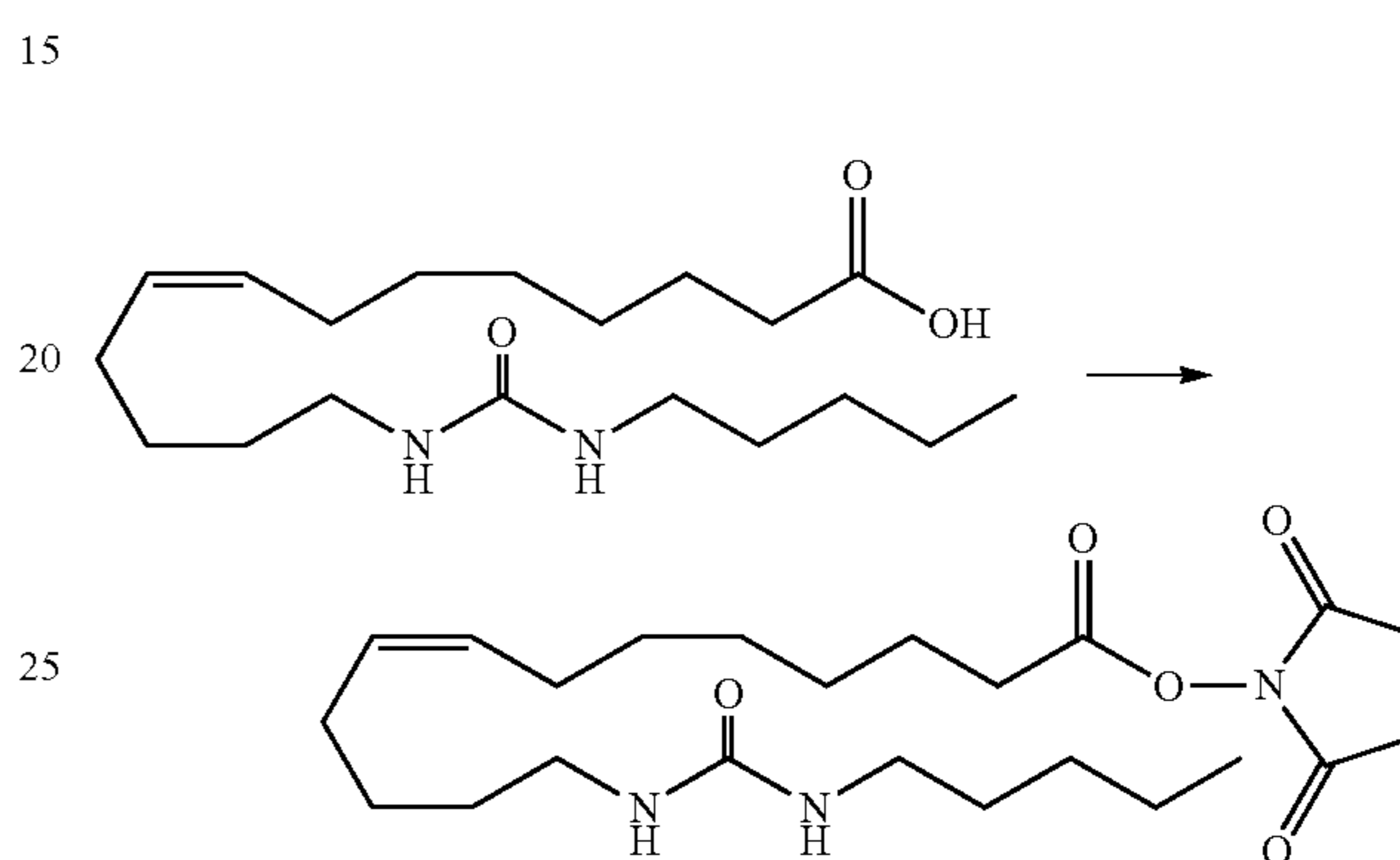
N-Hydroxysuccinimidyl 13-(3-n-pentylureido)tridec-8(Z)-enoate
